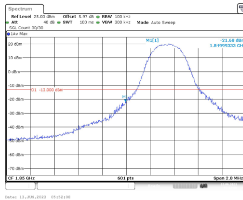
Band25-5MHz-QPSK-26065-1RB#0
