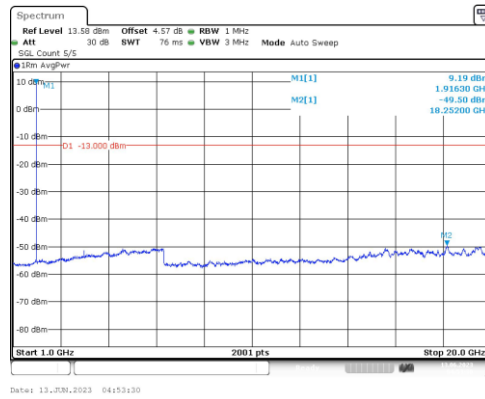
Band25-1.4MHz-16QAM-26683-1RB#0-Range4:1000~20000MHz
