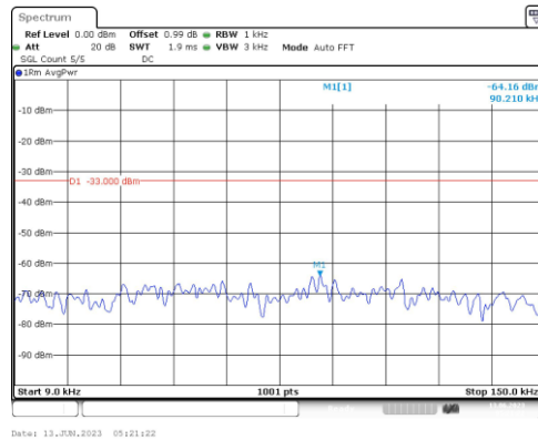
Band25-3MHz-QPSK-26055-1RB#0-Range1:0.009~0.15MHz
