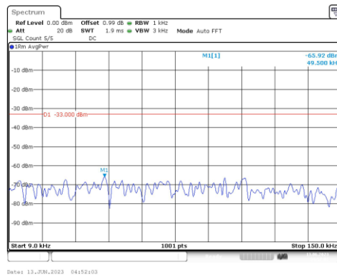
Band25-1.4MHz-QPSK-26683-1RB#0-Range1:0.009~0.15MHz
