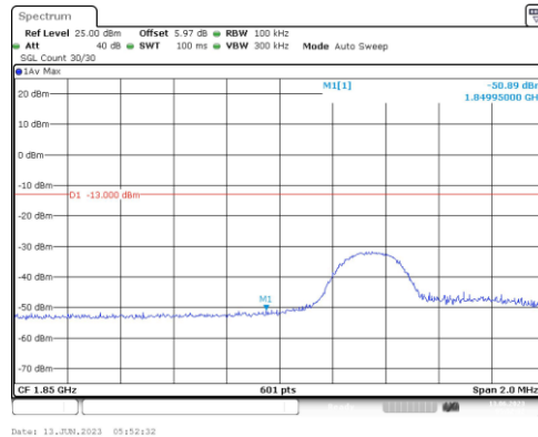
Band25-5MHz-QPSK-26065-1RB#24
