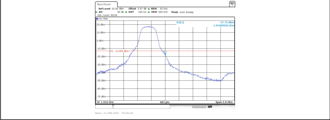
Band25-3MHz-16QAM-26675-1RB#0
