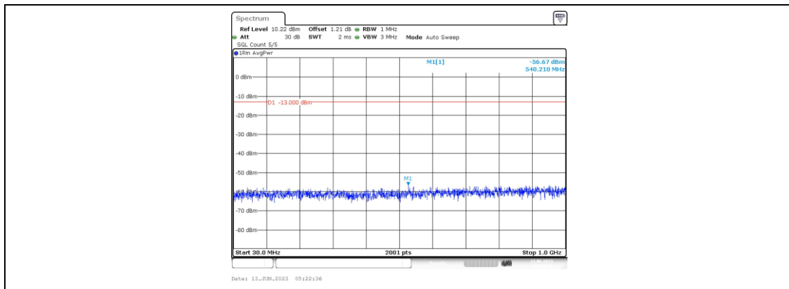
Band25-3MHz-16QAM-26055-1RB#0-Range3:30~1000MHz
