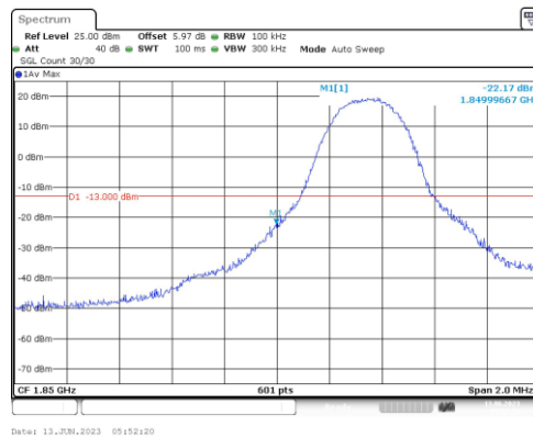
Band25-5MHz-16QAM-26065-1RB#0
