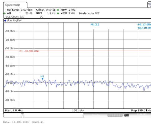
Band25-10MHz-QPSK-26365-1RB#0-Range1:0.009~0.15MHz
