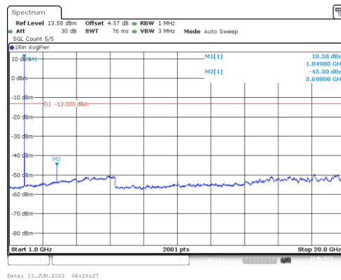
Band25-10MHz-16QAM-26090-1RB#0-Range4:1000~20000MHz
