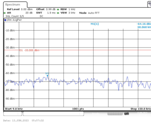
Band25-5MHz-16QAM-26365-1RB#0-Range1:0.009~0.15MHz
