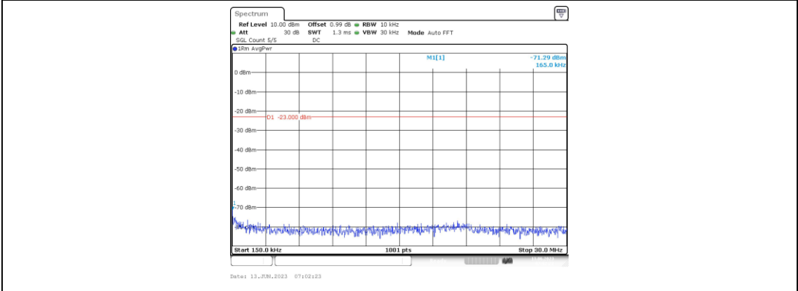
Band25-15MHz-16QAM-26115-1RB#0-Range2:0.15~30MHz
