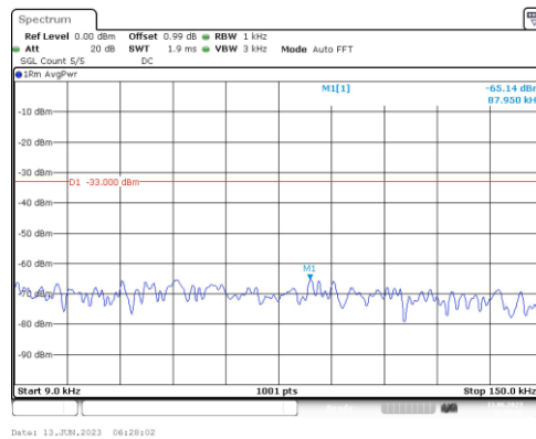
Band25-10MHz-QPSK-26090-1RB#0-Range1:0.009~0.15MHz
