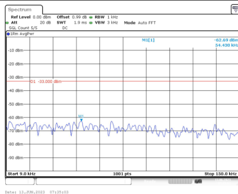
Band25-20MHz-QPSK-26140-1RB#0-Range1:0.009~0.15MHz
