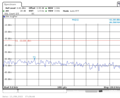
Band25-20MHz-QPSK-26365-1RB#0-Range1:0.009~0.15MHz
