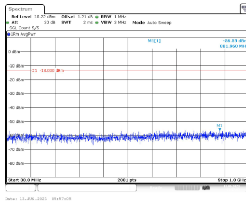
Band25-5MHz-QPSK-26365-1RB#0-Range3:30~1000MHz
