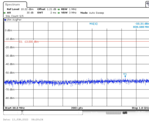
Band25-10MHz-QPSK-26090-1RB#0-Range3:30~1000MHz
