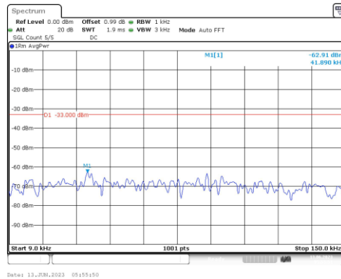
Band25-5MHz-16QAM-26065-1RB#0-Range1:0.009~0.15MHz
