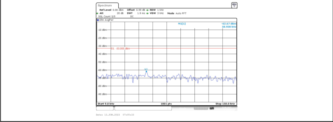
Band25-15MHz-16QAM-26615-1RB#0-Range1:0.009~0.15MHz
