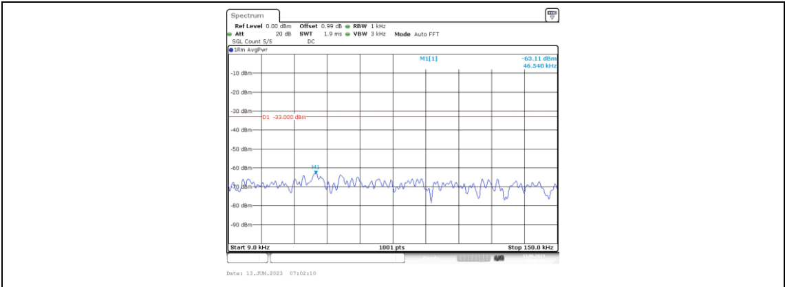
Band25-15MHz-16QAM-26115-1RB#0-Range1:0.009~0.15MHz
