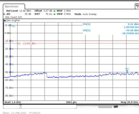
Band25-15MHz-16QAM-26615-1RB#0-Range4:1000~20000MHz
