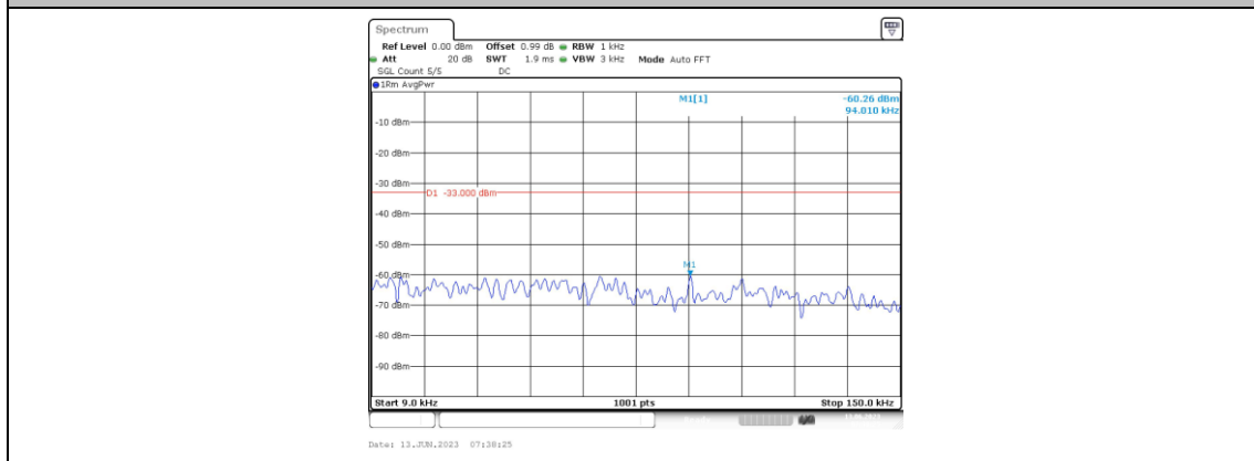
Band25-20MHz-QPSK-26590-1RB#0-Range1:0.009~0.15MHz
