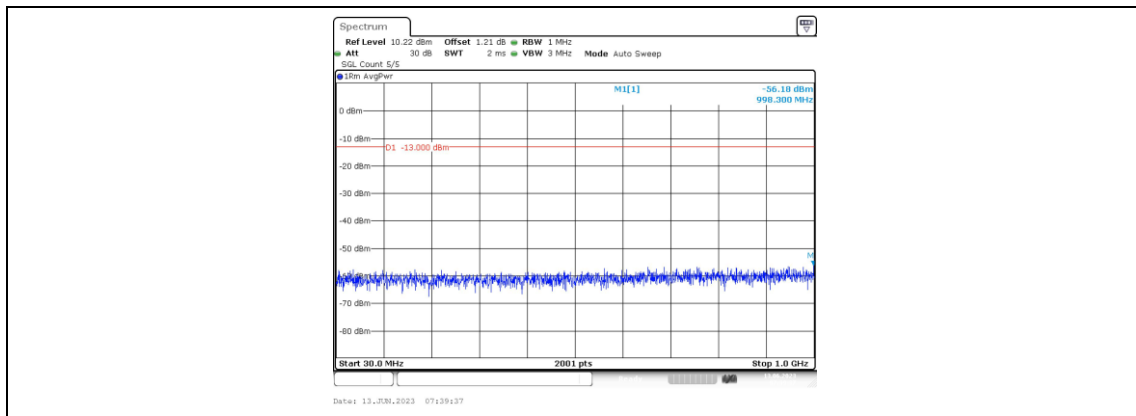
Band25-20MHz-16QAM-26590-1RB#0-Range3:30~1000MHz
