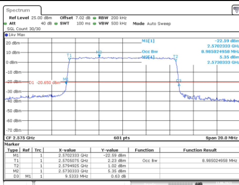
Band38-10MHz-QPSK-37800-50RB#0-8.985
