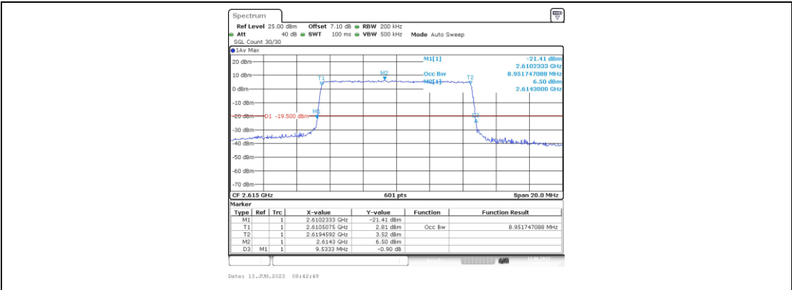
Band38-10MHz-QPSK-38200-50RB#0-8.952
