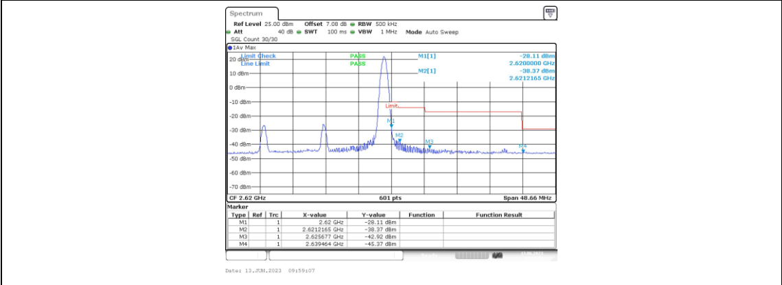
Band38-20MHz-16QAM-38150-1RB#99
