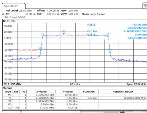
Band38-10MHz-QPSK-38000-50RB#0-8.985
