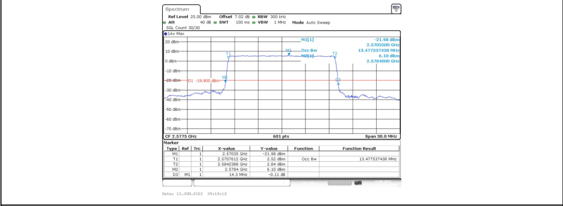
Band38-15MHz-QPSK-37825-75RB#0-13.478
