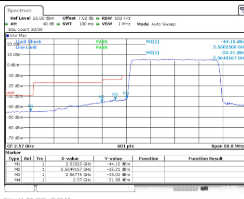
Band38-20MHz-16QAM-37850-100RB#0
