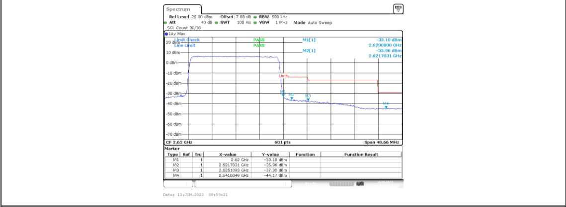
Band38-20MHz-QPSK-38150-100RB#0
