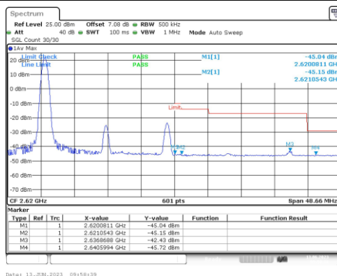
Band38-20MHz-16QAM-38150-1RB#0
