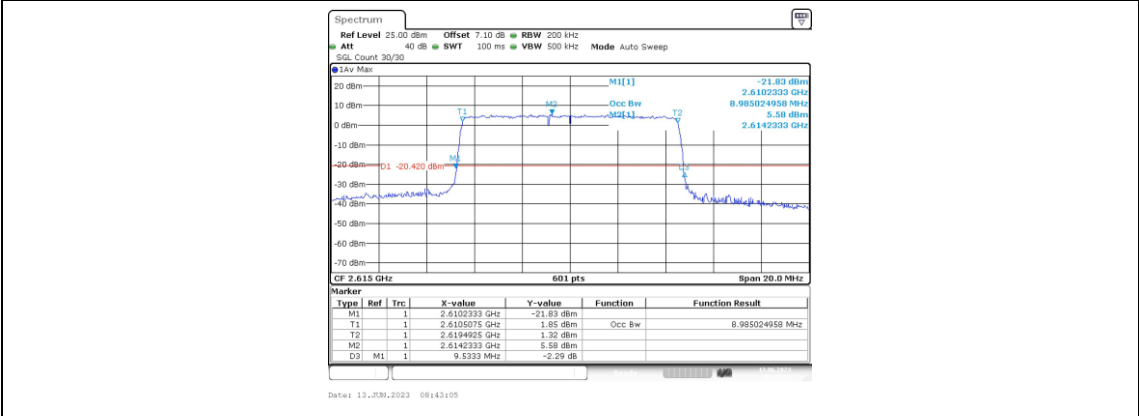
Band38-10MHz-16QAM-38200-50RB#0-8.985
