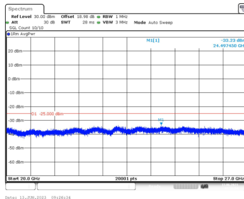
Band38-15MHz-QPSK-38000-1RB#0-Range5:20000~27000MHz
