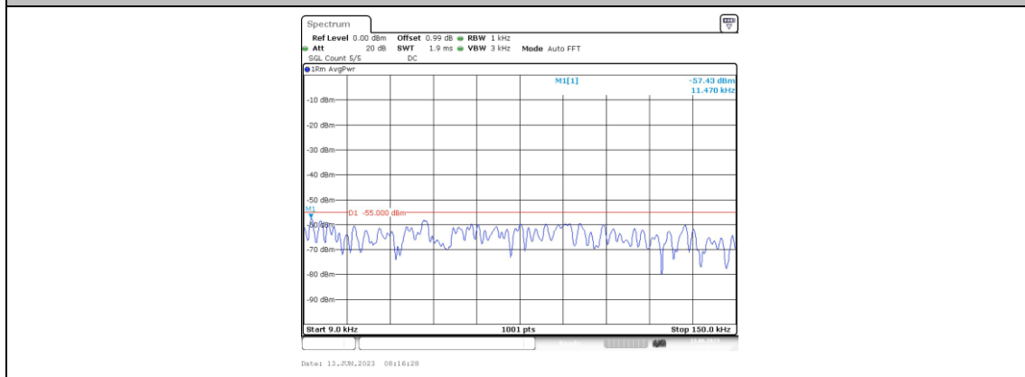
Band38-5MHz-16QAM-38225-1RB#0-Range1:0.009~0.15MHz
