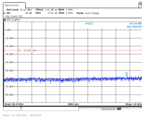
Band38-15MHz-16QAM-37825-1RB#0-Range3:30~1000MHz
