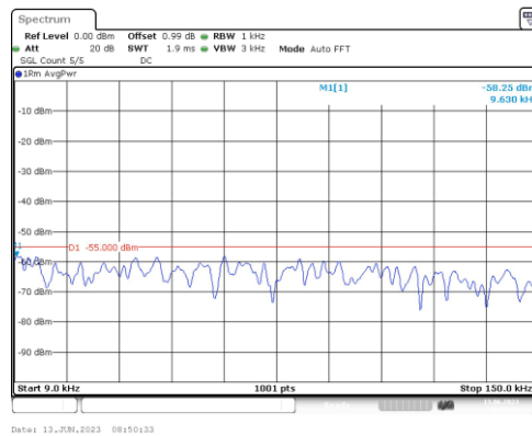
Band38-10MHz-16QAM-38000-1RB#0-Range1:0.009~0.15MHz
