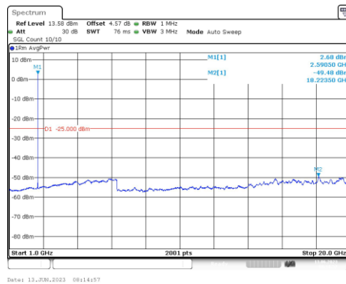
Band38-5MHz-16QAM-38000-1RB#0-Range4:1000~20000MHz
