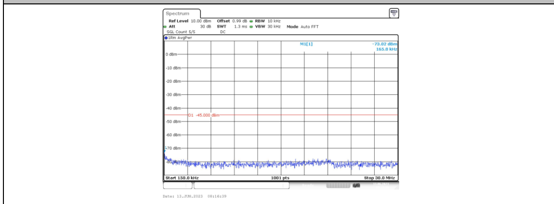
Band38-5MHz-16QAM-38225-1RB#0-Range2:0.15~30MHz
