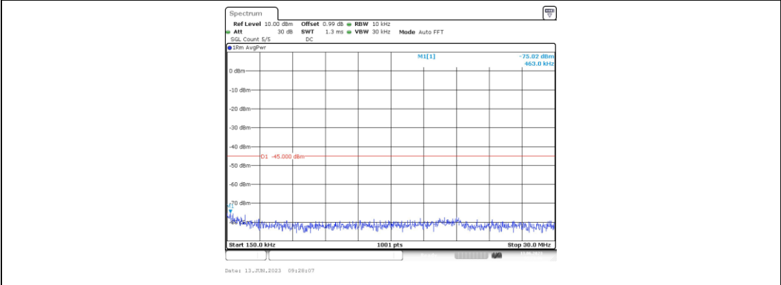
Band38-15MHz-QPSK-38175-1RB#0-Range2:0.15~30MHz
