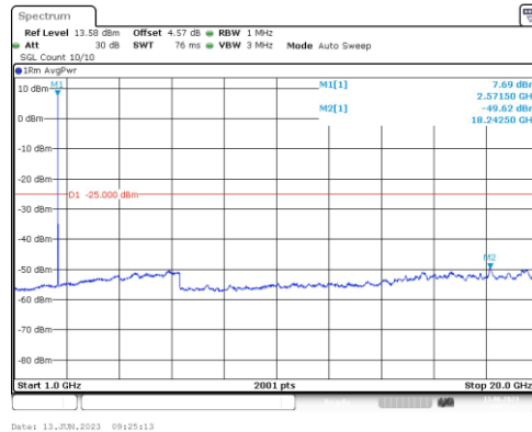
Band38-15MHz-16QAM-37825-1RB#0-Range4:1000~20000MHz
