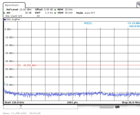
Band38-10MHz-16QAM-38000-1RB#0-Range2:0.15~30MHz
