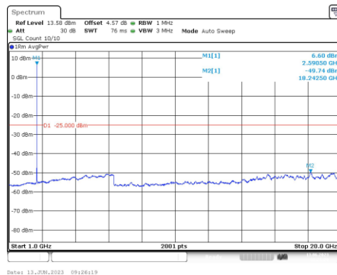
Band38-15MHz-QPSK-38000-1RB#0-Range4:1000~20000MHz
