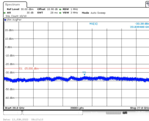
Band38-5MHz-16QAM-38000-1RB#0-Range5:20000~27000MHz
