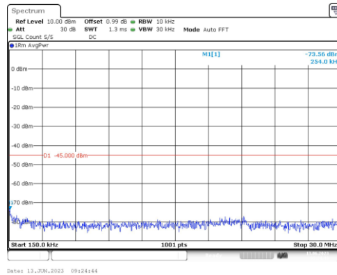
Band38-15MHz-16QAM-37825-1RB#0-Range2:0.15~30MHz
