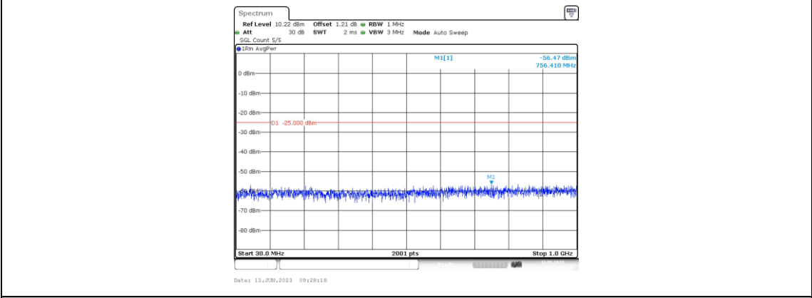
Band38-15MHz-QPSK-38175-1RB#0-Range3:30~1000MHz
