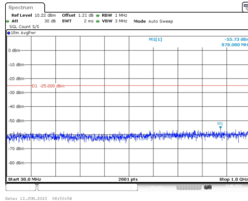
Band38-10MHz-16QAM-38000-1RB#0-Range3:30~1000MHz
