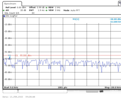
Band38-15MHz-16QAM-38000-1RB#0-Range1:0.009~0.15MHz
