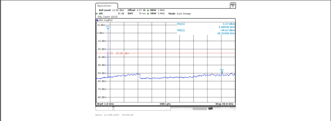
Band38-15MHz-16QAM-38175-1RB#0-Range4:1000~20000MHz
