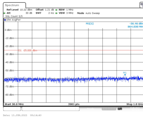
Band38-5MHz-16QAM-38000-1RB#0-Range3:30~1000MHz
