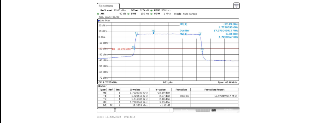
Band4-20MHz-QPSK-20175-100RB#0-17.97
