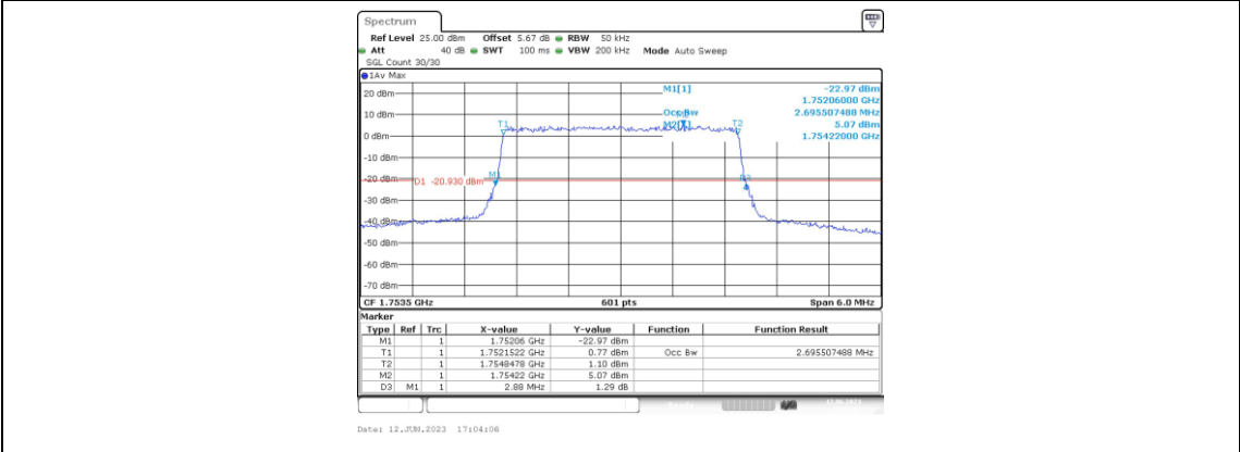
Band4-3MHz-16QAM-20385-15RB#0-2.696
