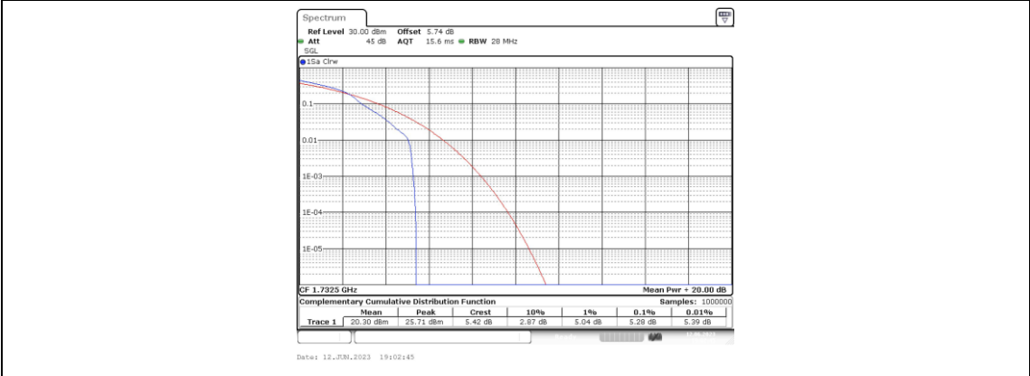
Band4-15MHz-16QAM-20175-1RB#0
