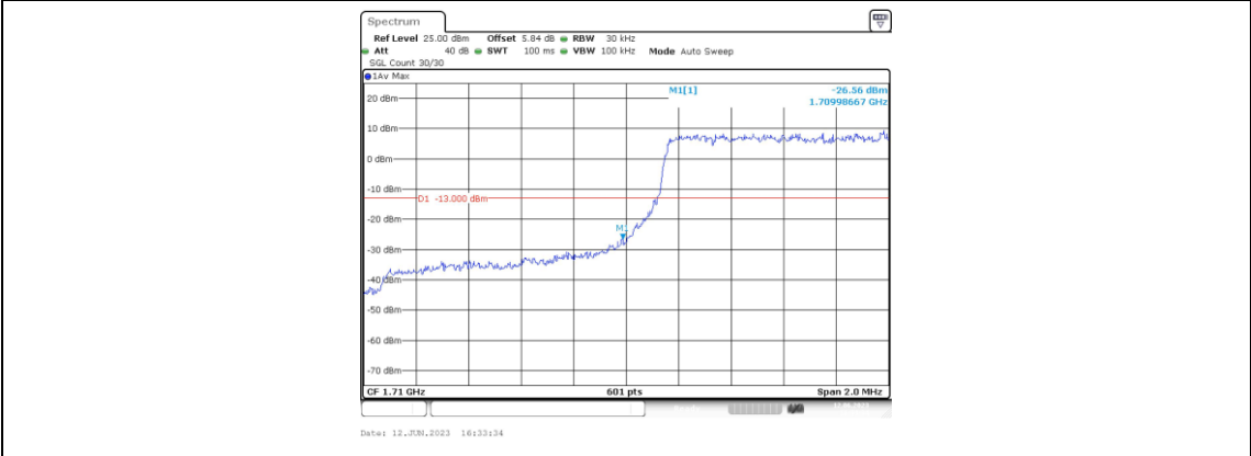
Band4-1.4MHz-QPSK-19957-6RB#0
