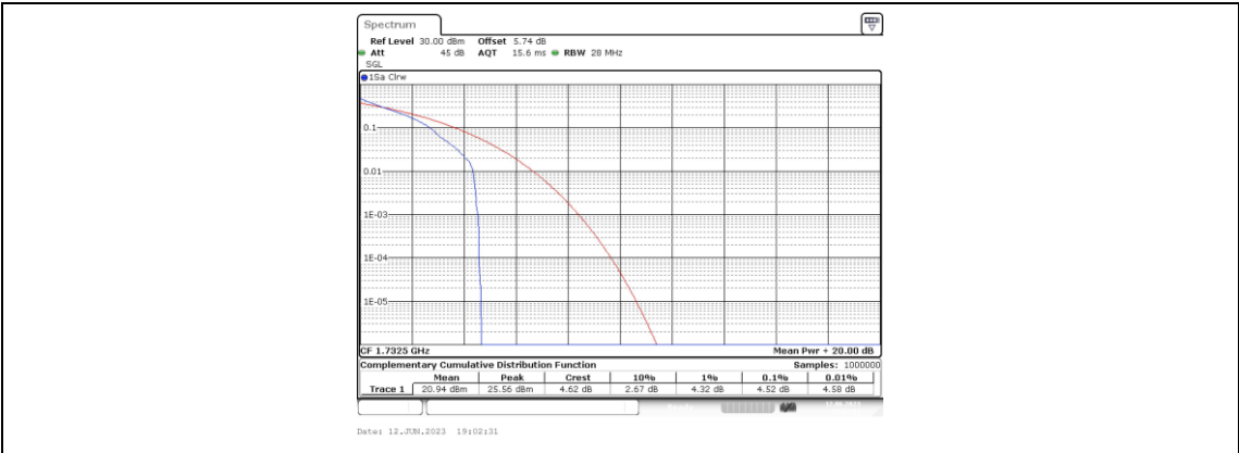
Band4-15MHz-QPSK-20175-1RB#0
