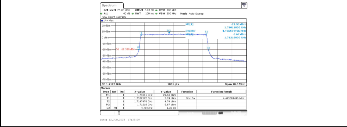
Band4-5MHz-QPSK-19975-25RB#0-4.496
