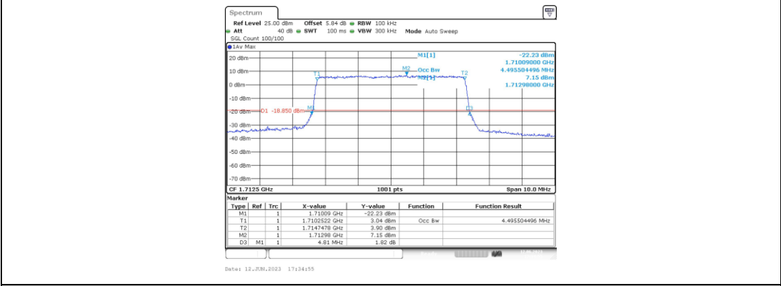
Band4-5MHz-QPSK-19975-25RB#0-4.496
