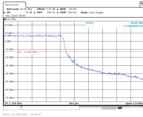
Band4-1.4MHz-QPSK-20393-6RB#0
