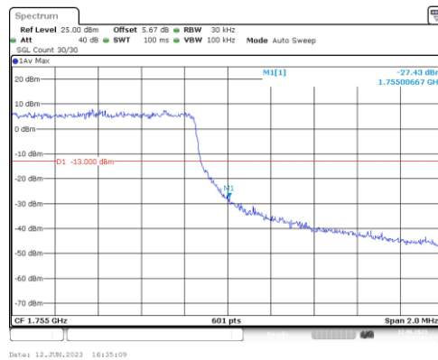
Band4-1.4MHz-16QAM-20393-6RB#0
