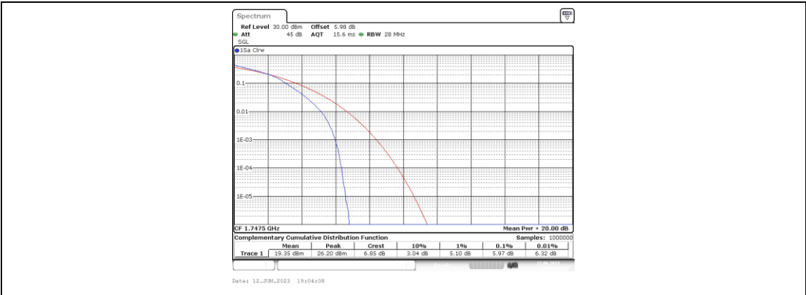
Band4-15MHz-16QAM-20325-75RB#0
