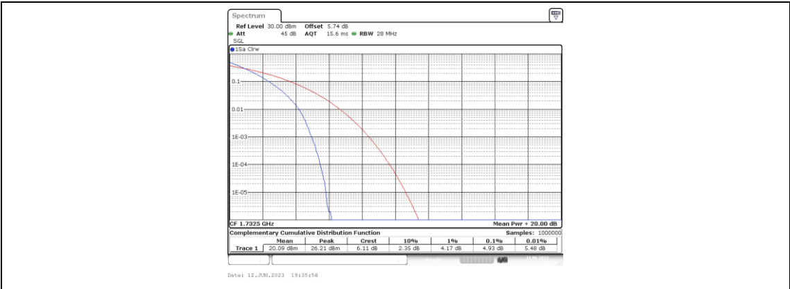
Band4-20MHz-QPSK-20175-100RB#0
