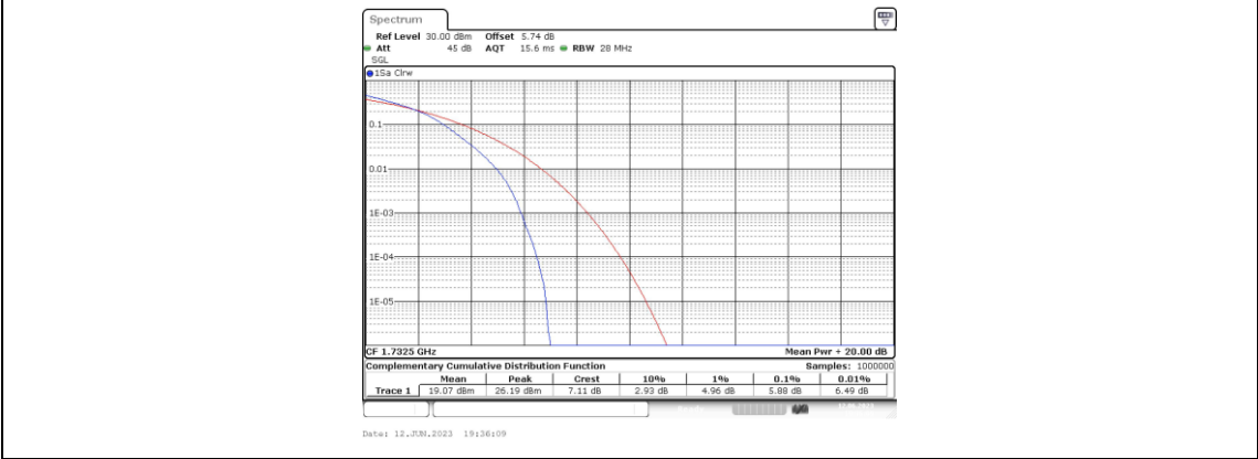
Band4-20MHz-16QAM-20175-100RB#0
