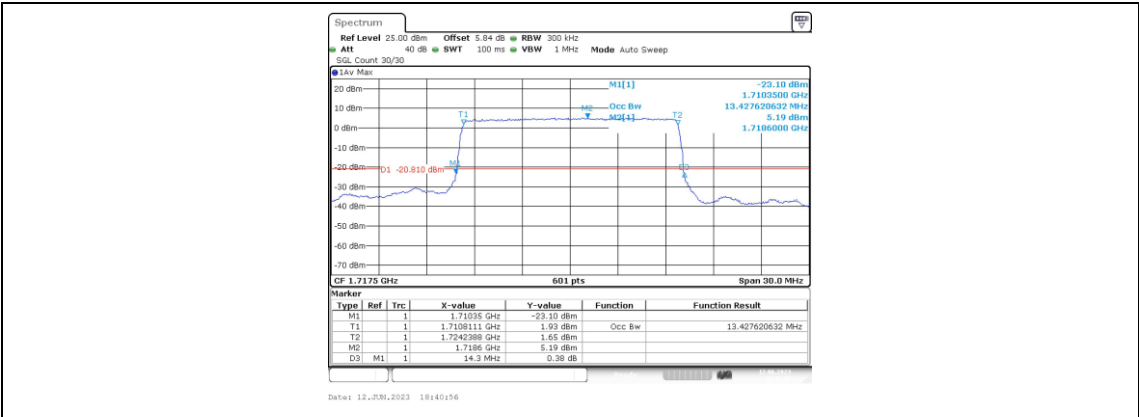
Band4-15MHz-QPSK-20025-75RB#0-13.428
