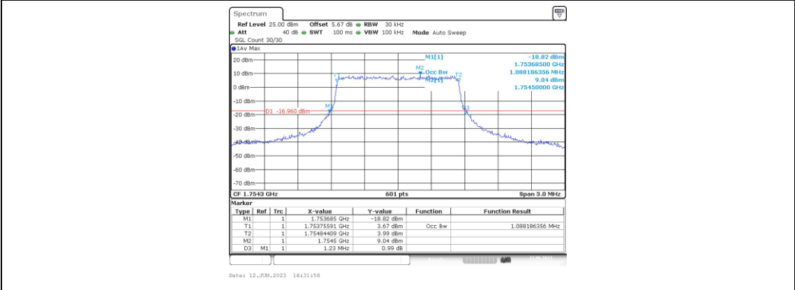
Band4-1.4MHz-QPSK-20393-6RB#0-1.088
