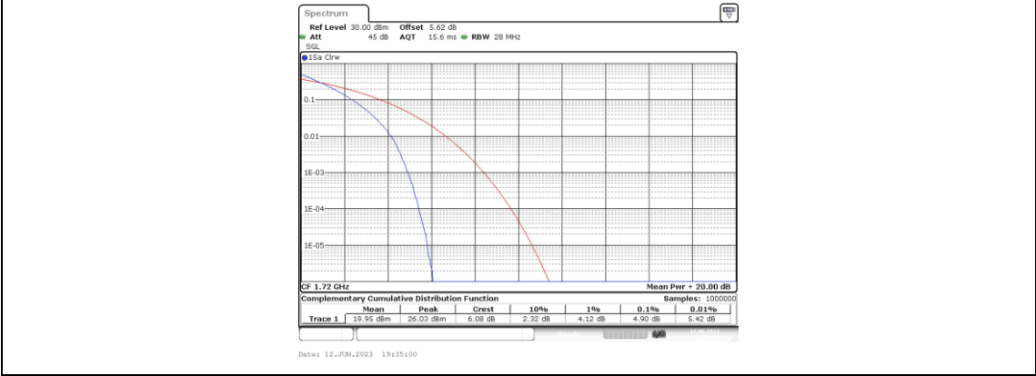
Band4-20MHz-16QAM-20050-1RB#0
