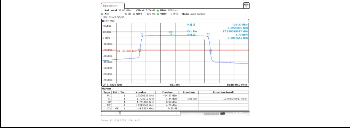
Band4-20MHz-16QAM-20175-100RB#0-17.97
