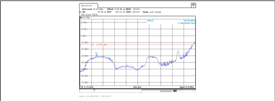
Band4-1.4MHz-16QAM-19957-1RB#5
