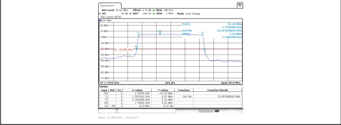
Band4-15MHz-QPSK-20175-75RB#0-13.428
