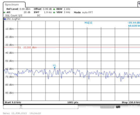
Band4-10MHz-QPSK-20175-1RB#0-Range1:0.009~0.15MHz
