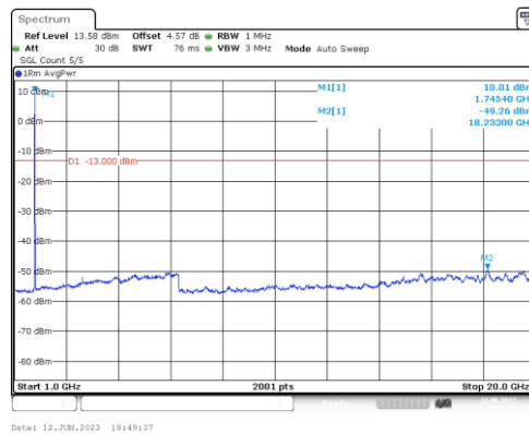
Band4-15MHz-QPSK-20325-1RB#0-Range4:1000~20000MHz
