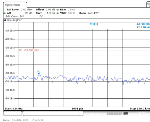
Band4-5MHz-16QAM-20175-1RB#0-Range1:0.009~0.15MHz
