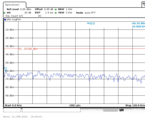
Band4-10MHz-QPSK-20350-1RB#0-Range1:0.009~0.15MHz
