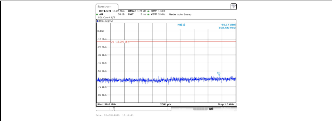
Band4-3MHz-16QAM-20175-1RB#0-Range3:30~1000MHz
