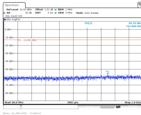
Band4-5MHz-QPSK-20375-1RB#0-Range3:30~1000MHz
