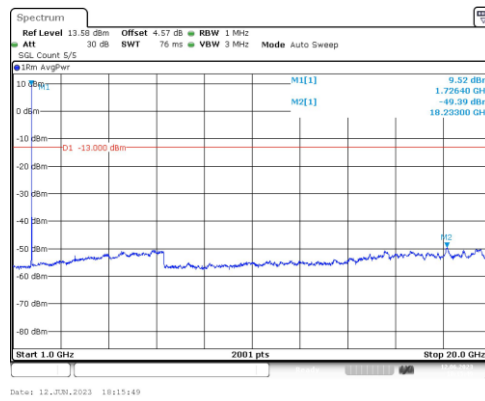
Band4-10MHz-16QAM-20175-1RB#0-Range4:1000~20000MHz
