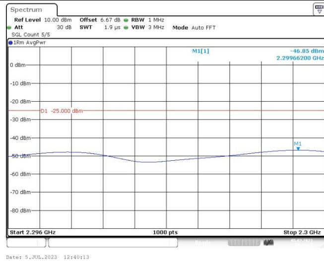
Band40-10MHz-QPSK-38750-1RB#0-Range8:2300~2304MHz
