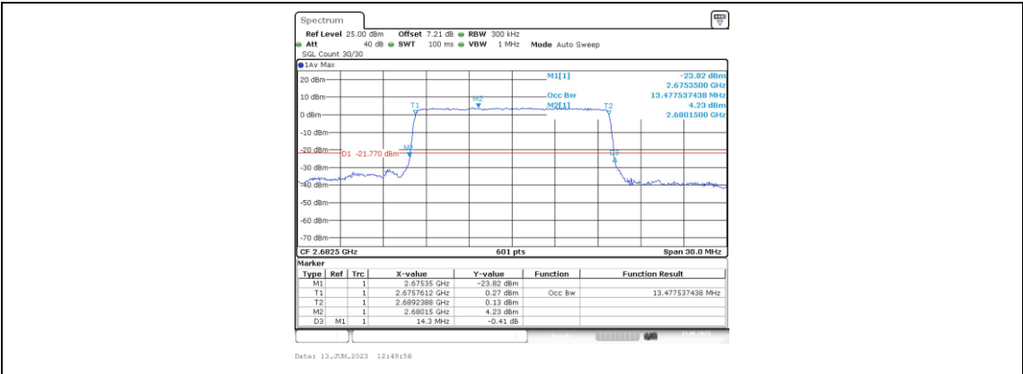
Band41-15MHz-16QAM-41515-75RB#0-13.478
