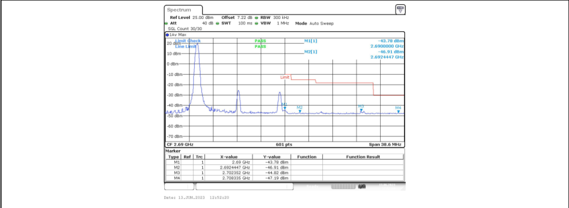
Band41-15MHz-16QAM-41515-1RB#0
