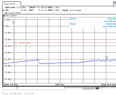
Band41-15MHz-16QAM-41515-1RB#0-Range4:1000~20000MHz
