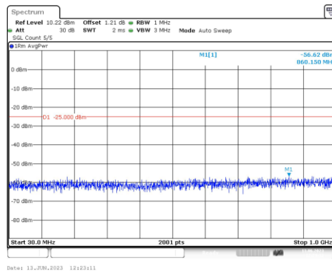
Band41-10MHz-QPSK-41540-1RB#0-Range3:30~1000MHz
