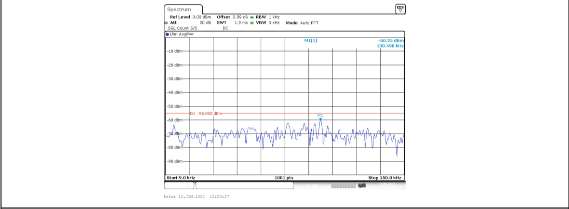
Band41-10MHz-QPSK-40620-1RB#0-Range1:0.009~0.15MHz
