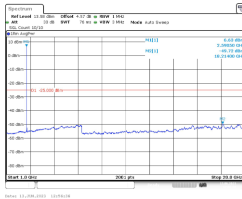
Band41-15MHz-QPSK-40620-1RB#0-Range4:1000~20000MHz
