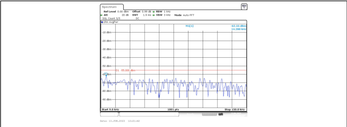
Band41-10MHz-16QAM-40620-1RB#0-Range1:0.009~0.15MHz
