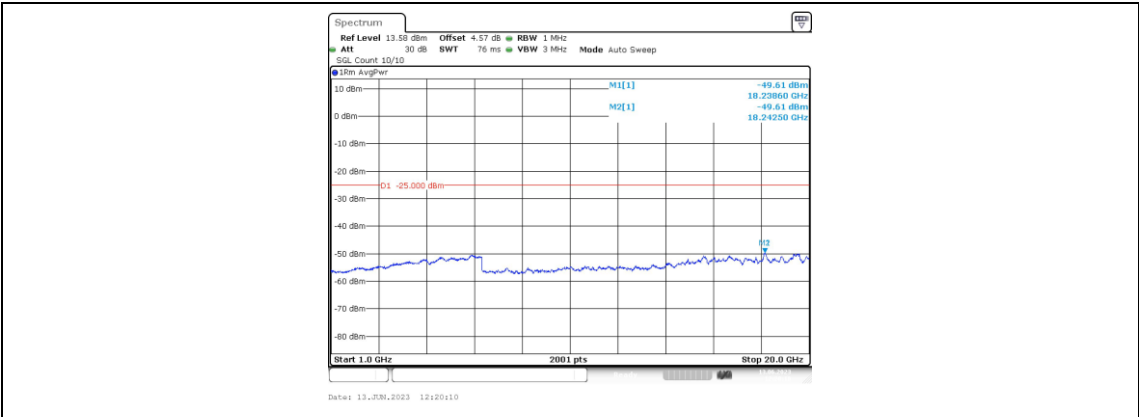
Band41-10MHz-16QAM-39700-1RB#0-Range4:1000~20000MHz
