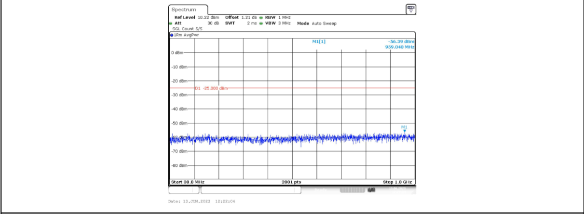
Band41-10MHz-16QAM-40620-1RB#0-Range3:30~1000MHz
