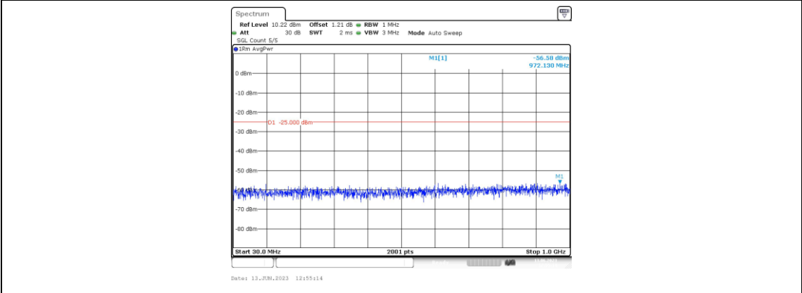
Band41-15MHz-16QAM-39725-1RB#0-Range3:30~1000MHz
