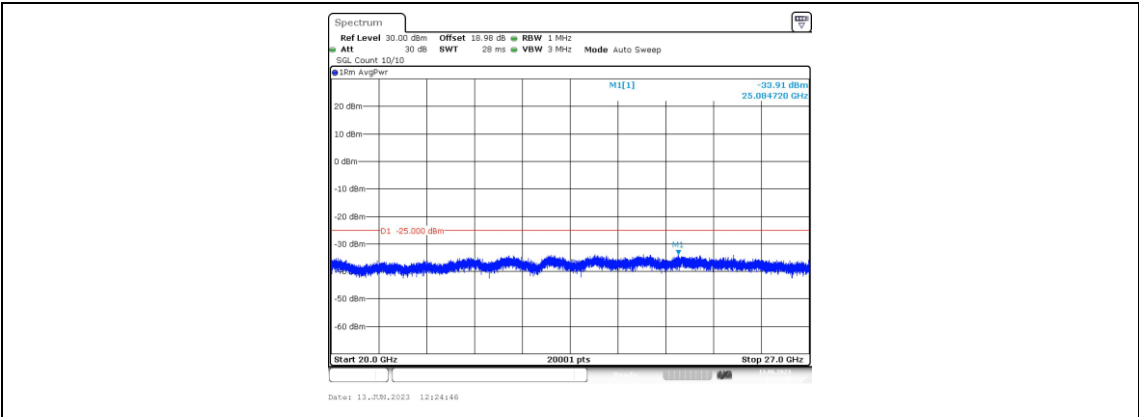
Band41-10MHz-16QAM-41540-1RB#0-Range5:20000~27000MHz
