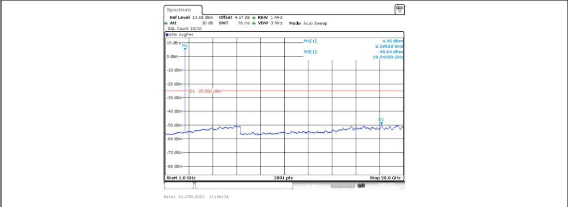
Band41-5MHz-16QAM-40620-1RB#0-Range4:1000~20000MHz
