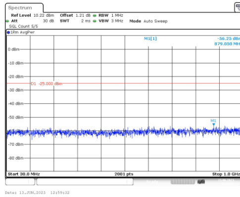
Band41-15MHz-16QAM-41515-1RB#0-Range3:30~1000MHz
