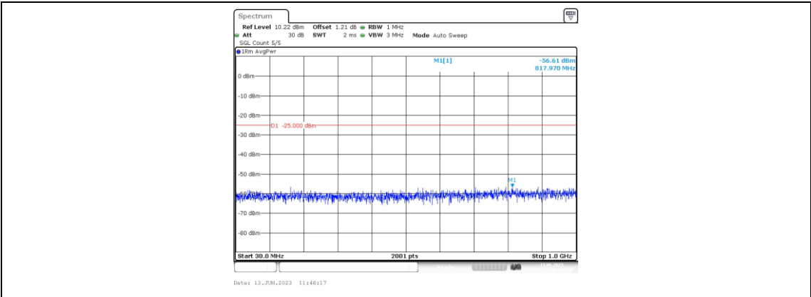
Band41-5MHz-16QAM-40620-1RB#0-Range3:30~1000MHz
