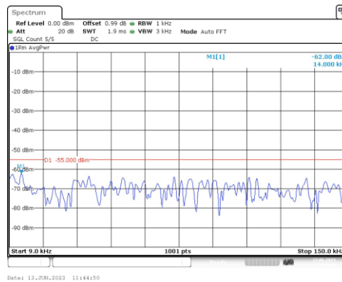
Band41-5MHz-QPSK-40620-1RB#0-Range1:0.009~0.15MHz
