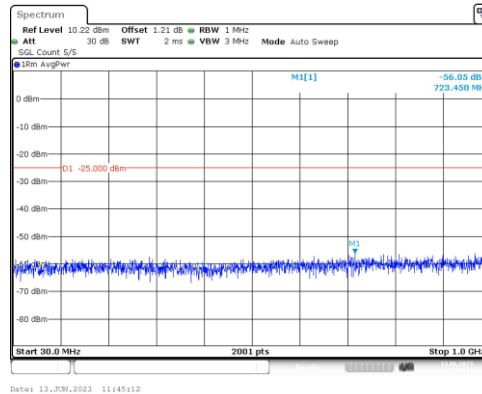
Band41-5MHz-QPSK-40620-1RB#0-Range3:30~1000MHz
