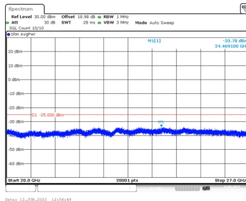
Band41-15MHz-QPSK-40620-1RB#0-Range5:20000~27000MHz
