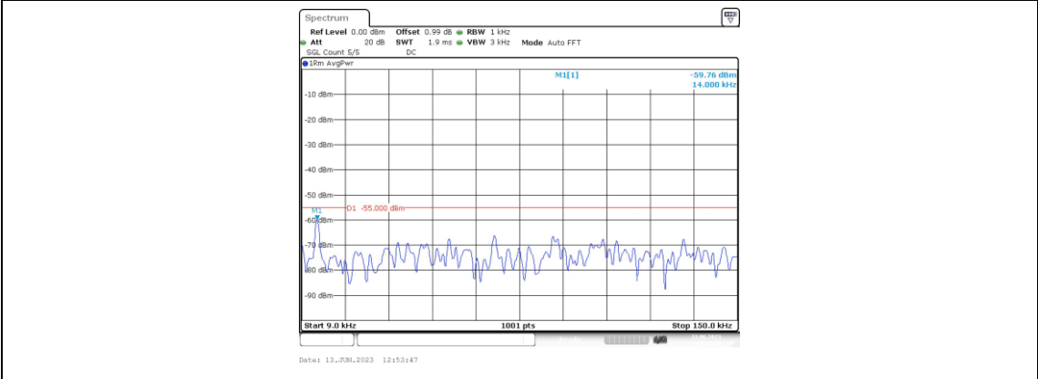
Band41-15MHz-QPSK-39725-1RB#0-Range1:0.009~0.15MHz
