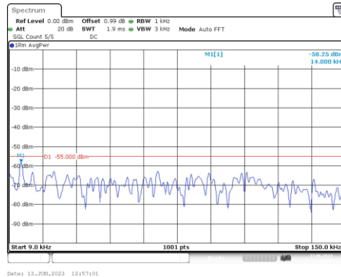
Band41-15MHz-16QAM-40620-1RB#0-Range1:0.009~0.15MHz
