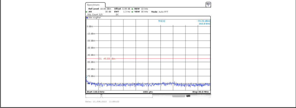
Band41-5MHz-16QAM-41565-1RB#0-Range2:0.15~30MHz
