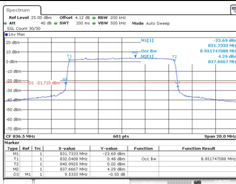
Band5-10MHz-QPSK-20525-50RB#0-8.952
