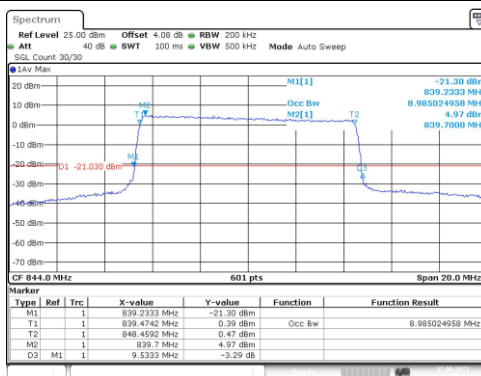
Band5-10MHz-QPSK-20600-50RB#0-8.985
