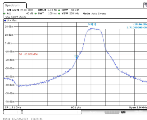
Band66-3MHz-QPSK-131987-1RB#0
