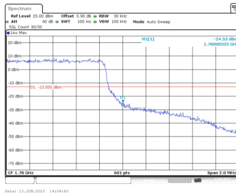
Band66-1.4MHz-16QAM-132665-6RB#0
