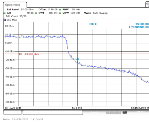
Band66-1.4MHz-QPSK-132665-6RB#0
