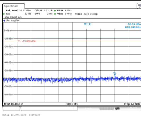
Band66-1.4MHz-16QAM-131979-1RB#0-Range3:30~1000MHz
