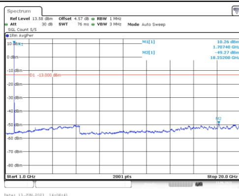
Band66-1.4MHz-16QAM-131979-1RB#0-Range4:1000~20000MHz
