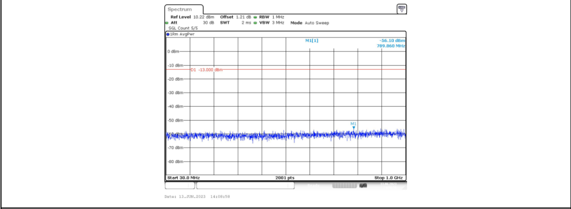
Band66-1.4MHz-QPSK-132665-1RB#0-Range3:30~1000MHz
