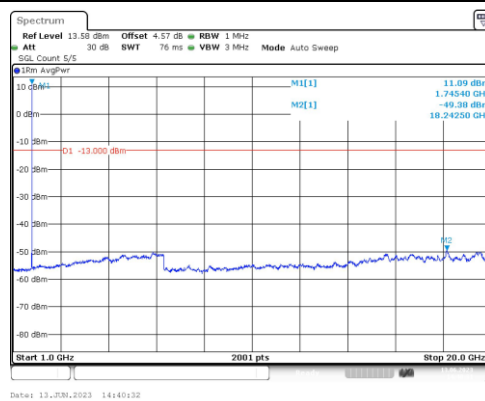
Band66-3MHz-QPSK-132322-1RB#0-Range4:1000~20000MHz
