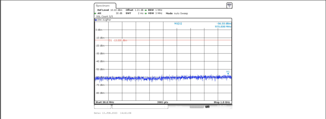
Band66-3MHz-16QAM-132322-1RB#0-Range3:30~1000MHz
