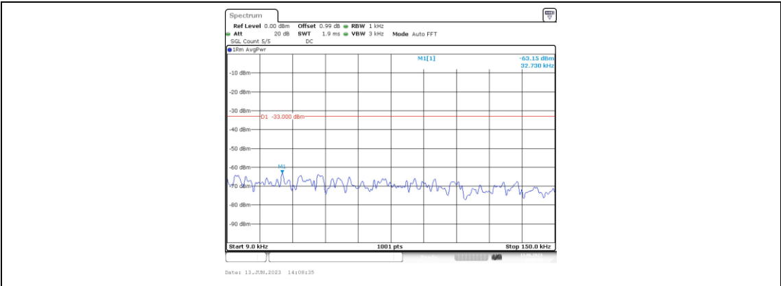
Band66-1.4MHz-QPSK-132665-1RB#0-Range1:0.009~0.15MHz
