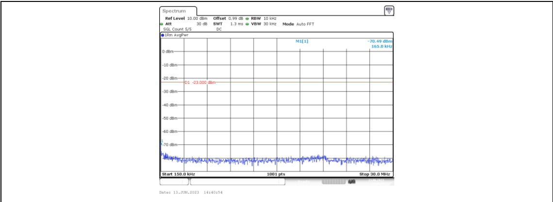
Band66-3MHz-16QAM-132322-1RB#0-Range2:0.15~30MHz
