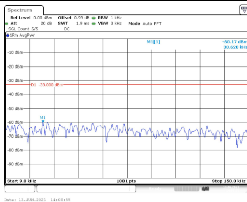
Band66-1.4MHz-QPSK-132322-1RB#0-Range1:0.009~0.15MHz
