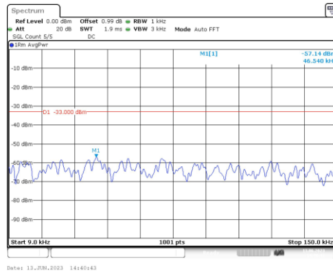
Band66-3MHz-16QAM-132322-1RB#0-Range1:0.009~0.15MHz
