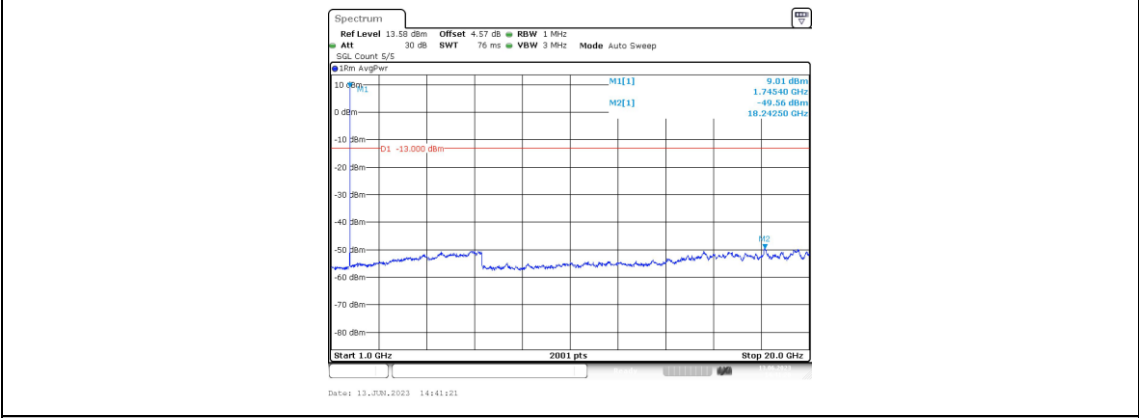
Band66-3MHz-16QAM-132322-1RB#0-Range4:1000~20000MHz
