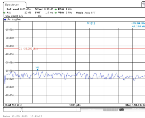
Band66-5MHz-16QAM-131997-1RB#0-Range1:0.009~0.15MHz
