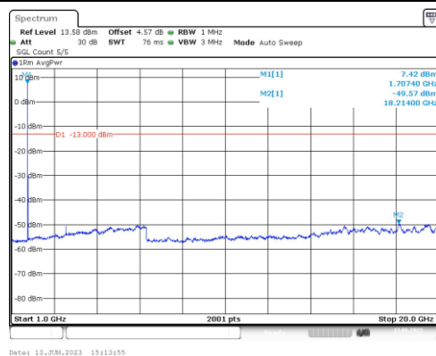
Band66-5MHz-16QAM-131997-1RB#0-Range4:1000~20000MHz
