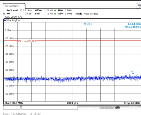
Band66-5MHz-16QAM-132322-1RB#0-Range3:30~1000MHz
