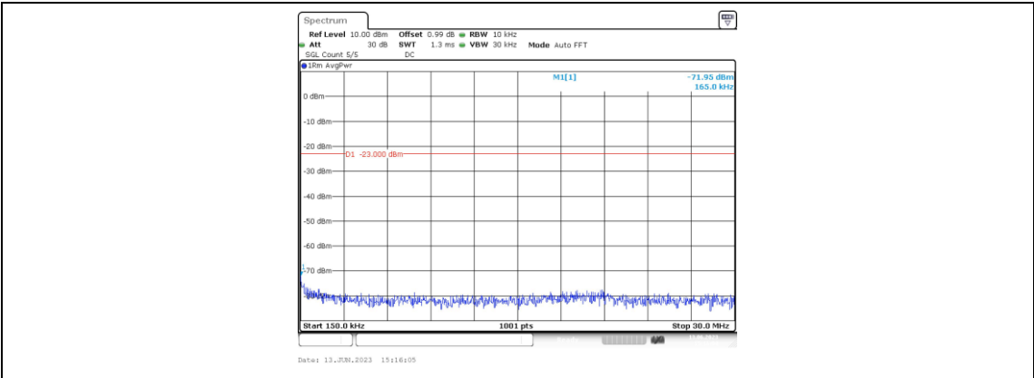
Band66-5MHz-QPSK-132647-1RB#0-Range2:0.15~30MHz
