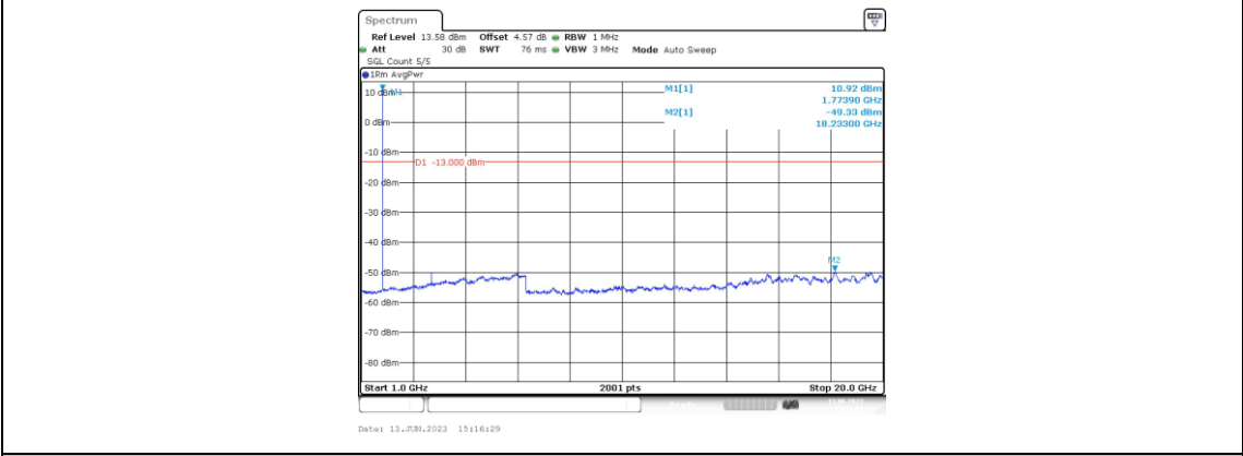
Band66-5MHz-QPSK-132647-1RB#0-Range4:1000~20000MHz
