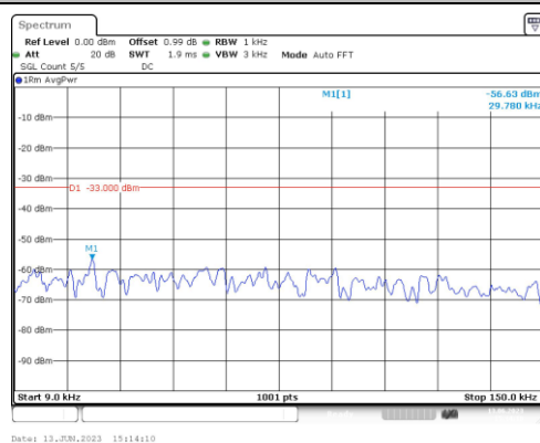
Band66-5MHz-QPSK-132322-1RB#0-Range1:0.009~0.15MHz
