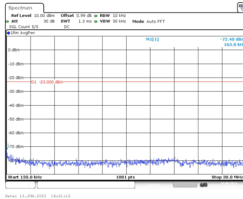
Band66-15MHz-16QAM-132047-1RB#0-Range2:0.15~30MHz
