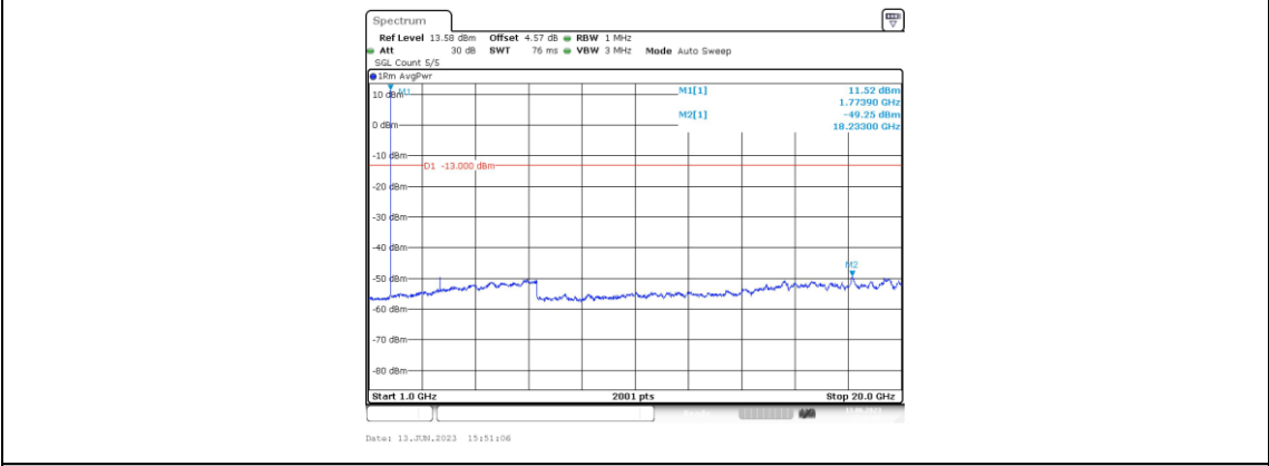
Band66-10MHz-16QAM-132622-1RB#0-Range4:1000~20000MHz
