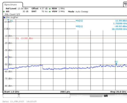
Band66-15MHz-QPSK-132322-1RB#0-Range4:1000~20000MHz
