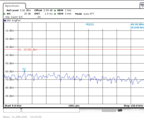
Band66-5MHz-QPSK-132647-1RB#0-Range1:0.009~0.15MHz
