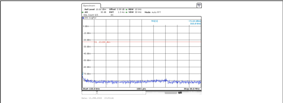
Band66-10MHz-16QAM-132622-1RB#0-Range2:0.15~30MHz
