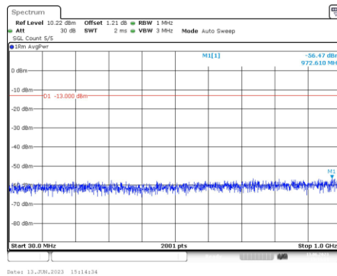
Band66-5MHz-QPSK-132322-1RB#0-Range3:30~1000MHz
