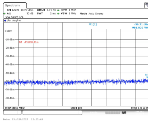
Band66-15MHz-QPSK-132597-1RB#0-Range3:30~1000MHz
