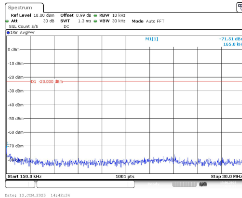
Band66-3MHz-16QAM-132657-1RB#0-Range2:0.15~30MHz
