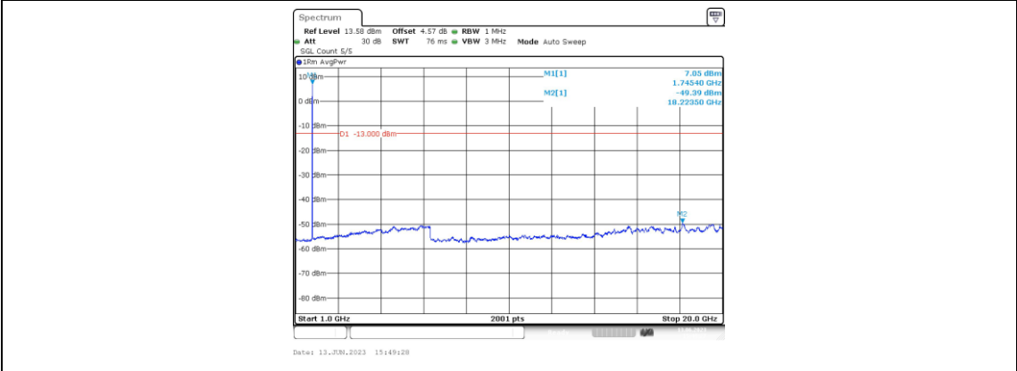
Band66-10MHz-16QAM-132322-1RB#0-Range4:1000~20000MHz
