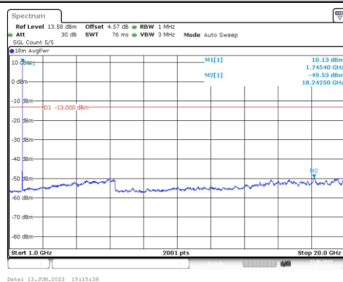
Band66-5MHz-16QAM-132322-1RB#0-Range4:1000~20000MHz
