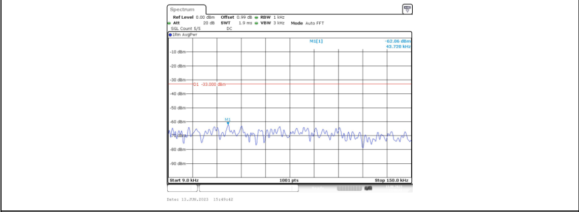
Band66-10MHz-QPSK-132622-1RB#0-Range1:0.009~0.15MHz
