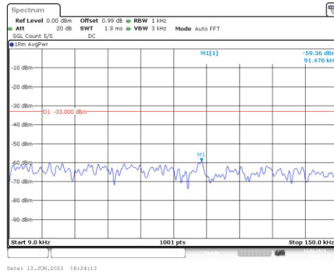
Band66-15MHz-16QAM-132597-1RB#0-Range1:0.009~0.15MHz
