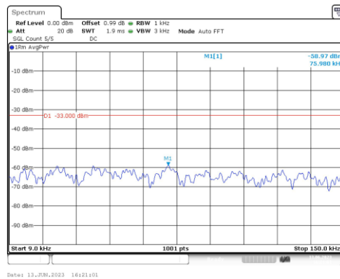
Band66-15MHz-16QAM-132047-1RB#0-Range1:0.009~0.15MHz
