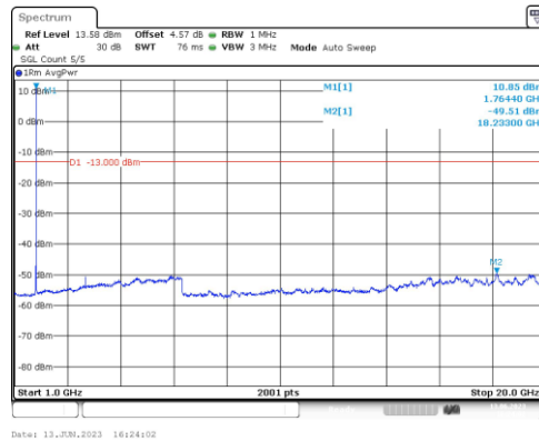
Band66-15MHz-QPSK-132597-1RB#0-Range4:1000~20000MHz
