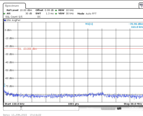
Band66-5MHz-QPSK-132322-1RB#0-Range2:0.15~30MHz
