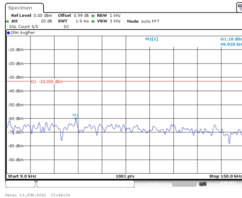
Band66-10MHz-QPSK-132322-1RB#0-Range1:0.009~0.15MHz
