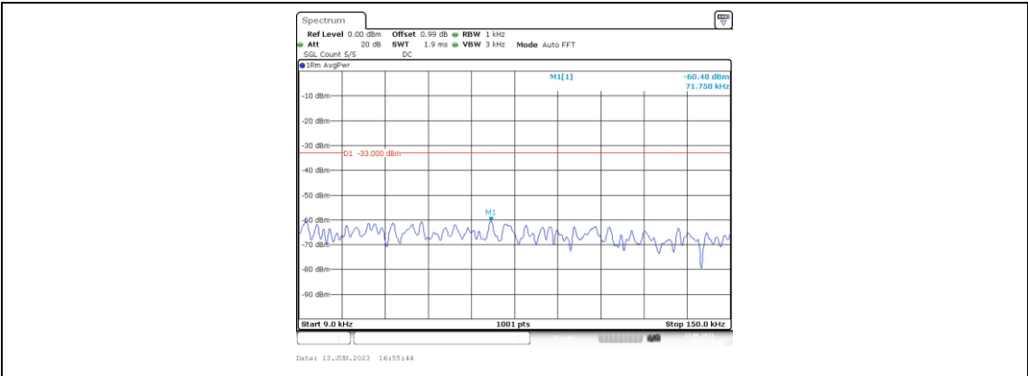
Band66-20MHz-QPSK-132322-1RB#0-Range1:0.009~0.15MHz
