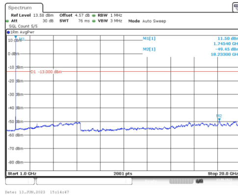
Band66-5MHz-QPSK-132322-1RB#0-Range4:1000~20000MHz
