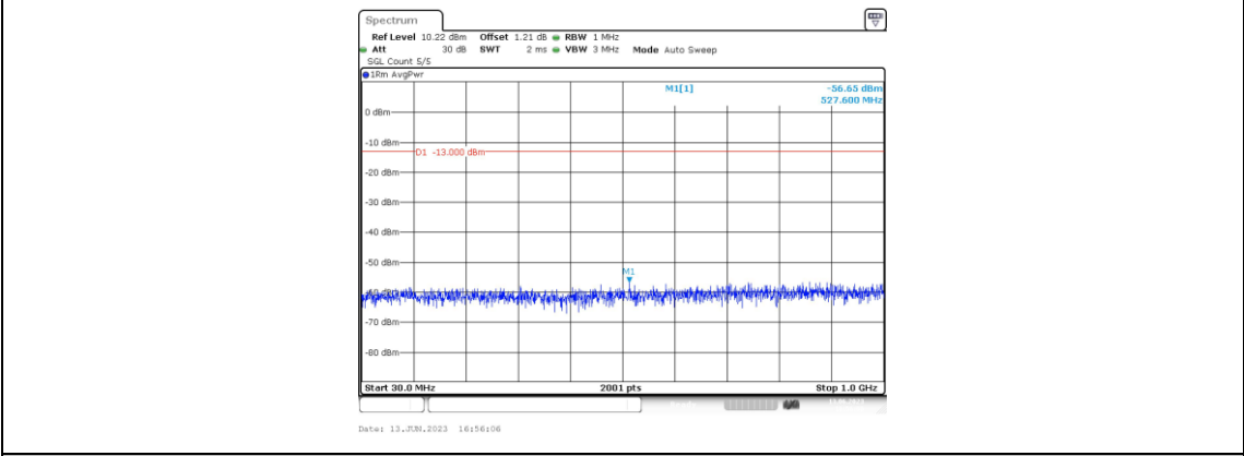
Band66-20MHz-QPSK-132322-1RB#0-Range3:30~1000MHz
