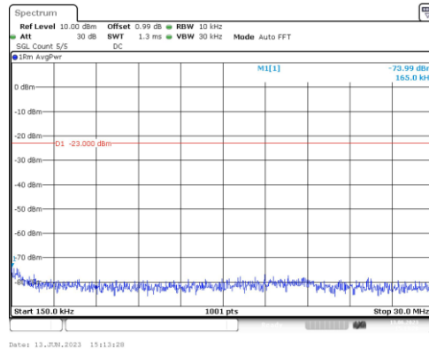
Band66-5MHz-16QAM-131997-1RB#0-Range2:0.15~30MHz
