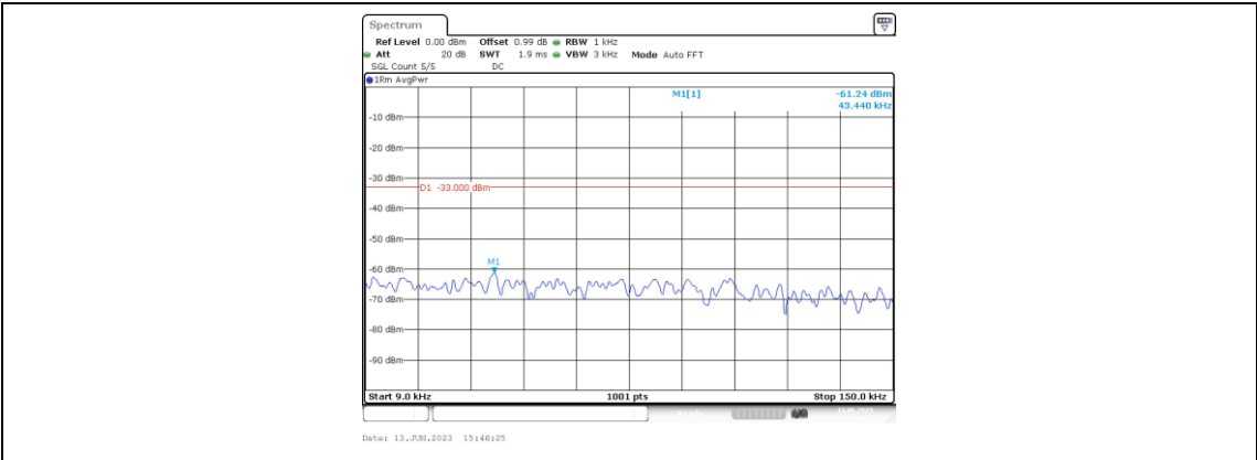
Band66-10MHz-QPSK-132022-1RB#0-Range1:0.009~0.15MHz
