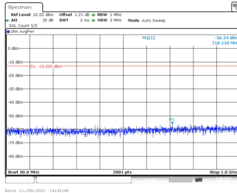
Band66-3MHz-16QAM-132657-1RB#0-Range3:30~1000MHz
