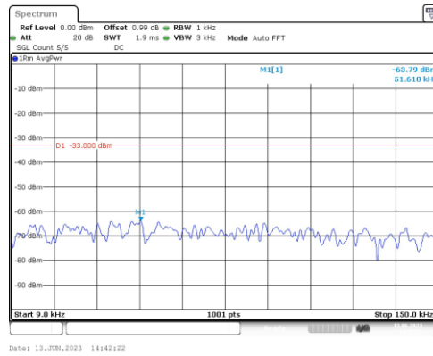
Band66-3MHz-16QAM-132657-1RB#0-Range1:0.009~0.15MHz
