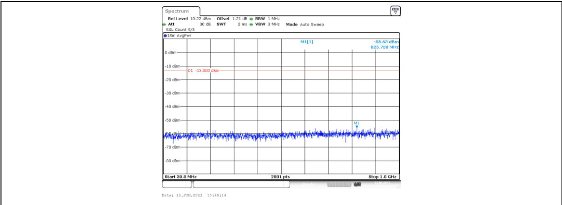
Band66-10MHz-16QAM-132322-1RB#0-Range3:30~1000MHz
