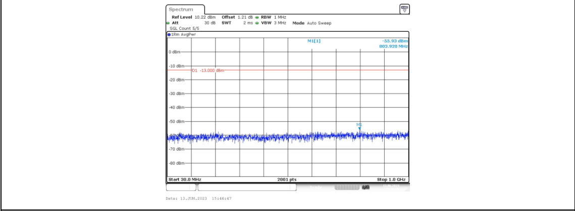
Band66-10MHz-QPSK-132022-1RB#0-Range3:30~1000MHz
