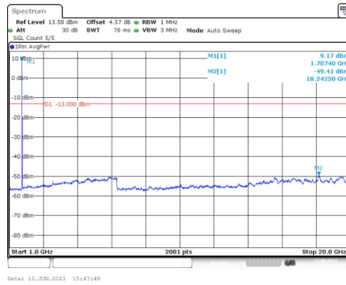
Band66-10MHz-16QAM-132022-1RB#0-Range4:1000~20000MHz
