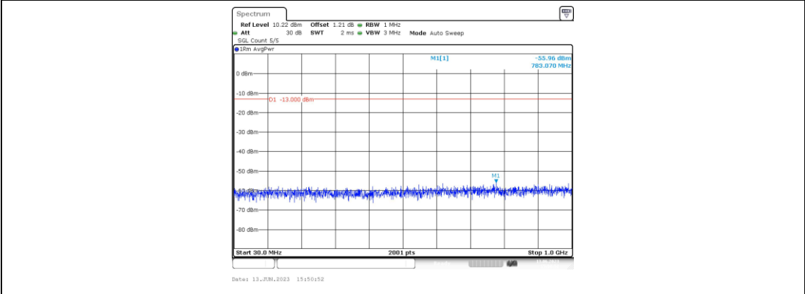
Band66-10MHz-16QAM-132622-1RB#0-Range3:30~1000MHz
