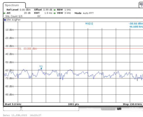
Band66-15MHz-16QAM-132322-1RB#0-Range1:0.009~0.15MHz
