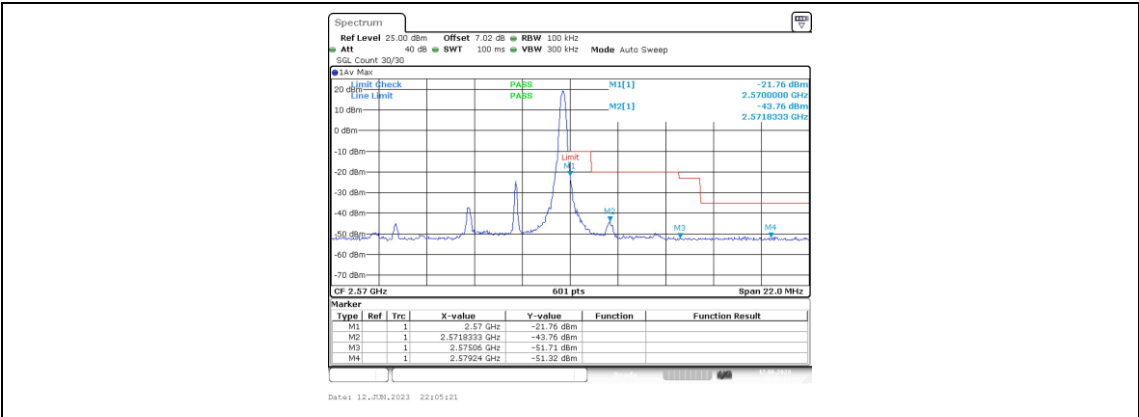
Band7-5MHz-16QAM-21425-1RB#24
