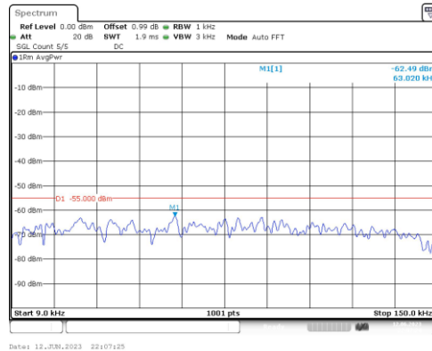
Band7-5MHz-16QAM-20775-1RB#0-Range1:0.009~0.15MHz
