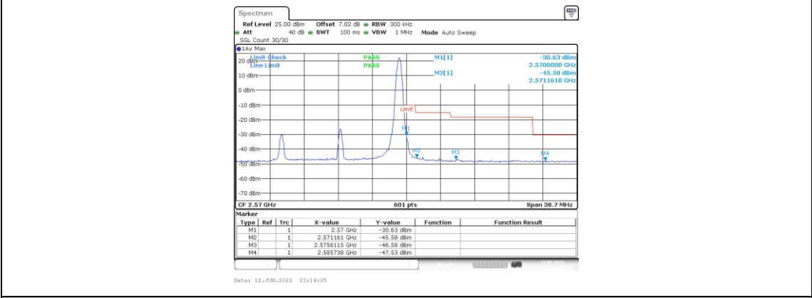
Band7-15MHz-QPSK-21375-1RB#74
