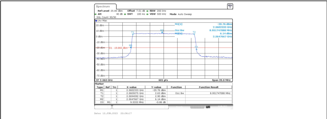
Band7-10MHz-QPSK-21400-50RB#0-8.952
