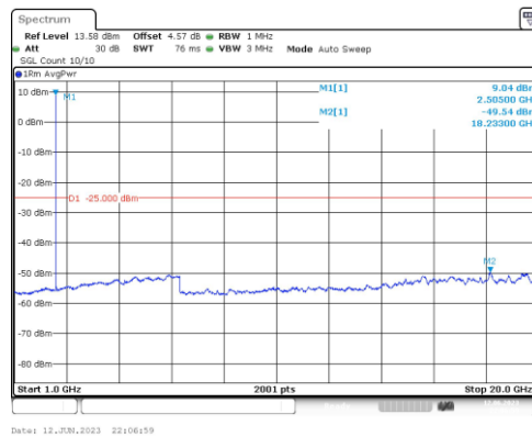
Band7-5MHz-QPSK-20775-1RB#0-Range4:1000~20000MHz
