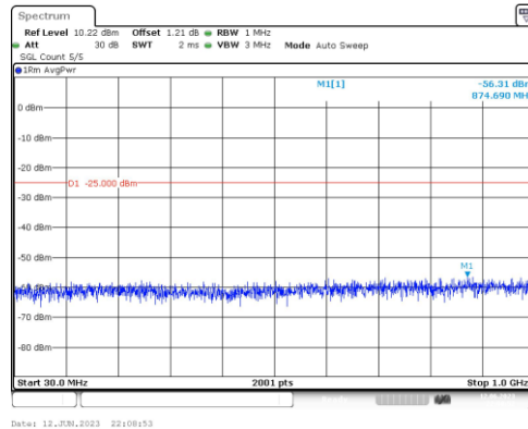
Band7-5MHz-QPSK-21100-1RB#0-Range3:30~1000MHz
