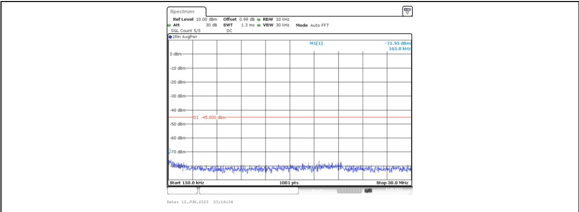
Band7-15MHz-16QAM-20825-1RB#0-Range2:0.15~30MHz
