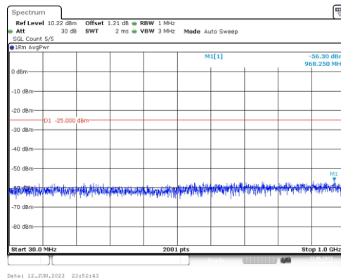
Band7-20MHz-QPSK-21100-1RB#0-Range3:30~1000MHz
