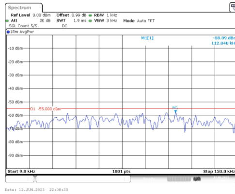
Band7-5MHz-QPSK-21100-1RB#0-Range1:0.009~0.15MHz
