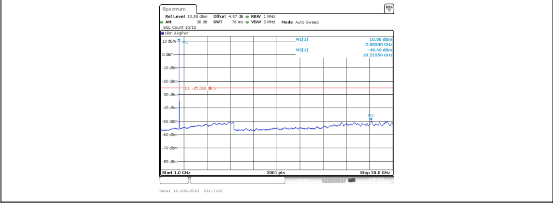
Band7-15MHz-16QAM-20825-1RB#0-Range4:1000~20000MHz
