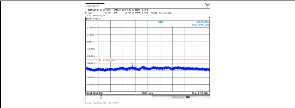
Band7-10MHz-16QAM-21400-1RB#0-Range5:20000~27000MHz
