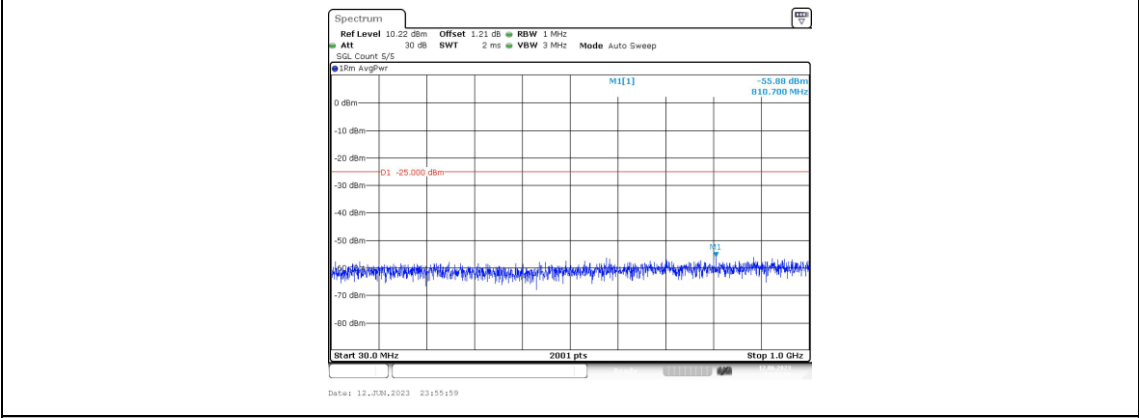
Band7-20MHz-16QAM-21350-1RB#0-Range3:30~1000MHz
