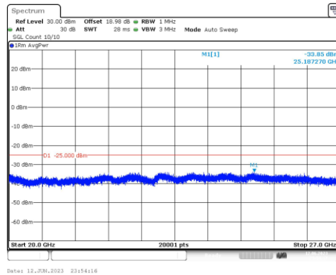
Band7-20MHz-16QAM-21100-1RB#0-Range5:20000~27000MHz
