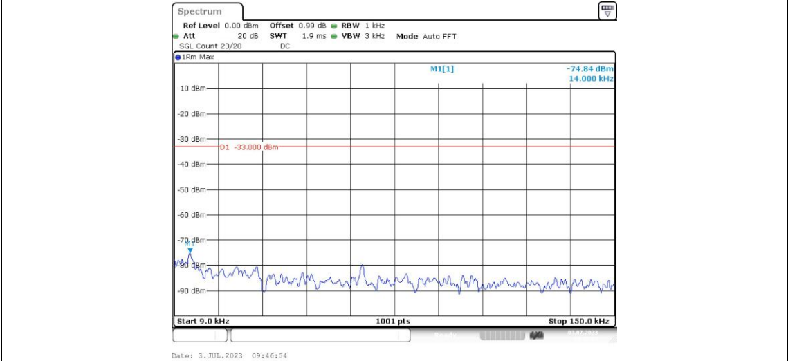
Band5-4183-1-0.009~0.15MHz
