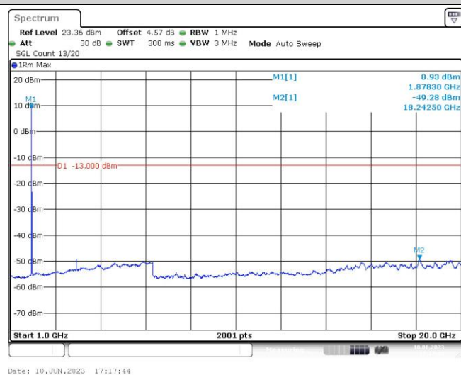
Band2-9400-4-1000~20000MHz
