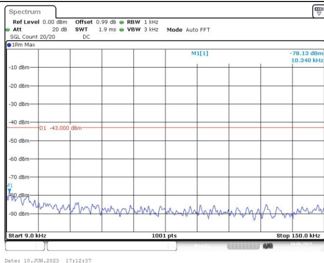
Band2-9262-3-0.009~0.15MHz
