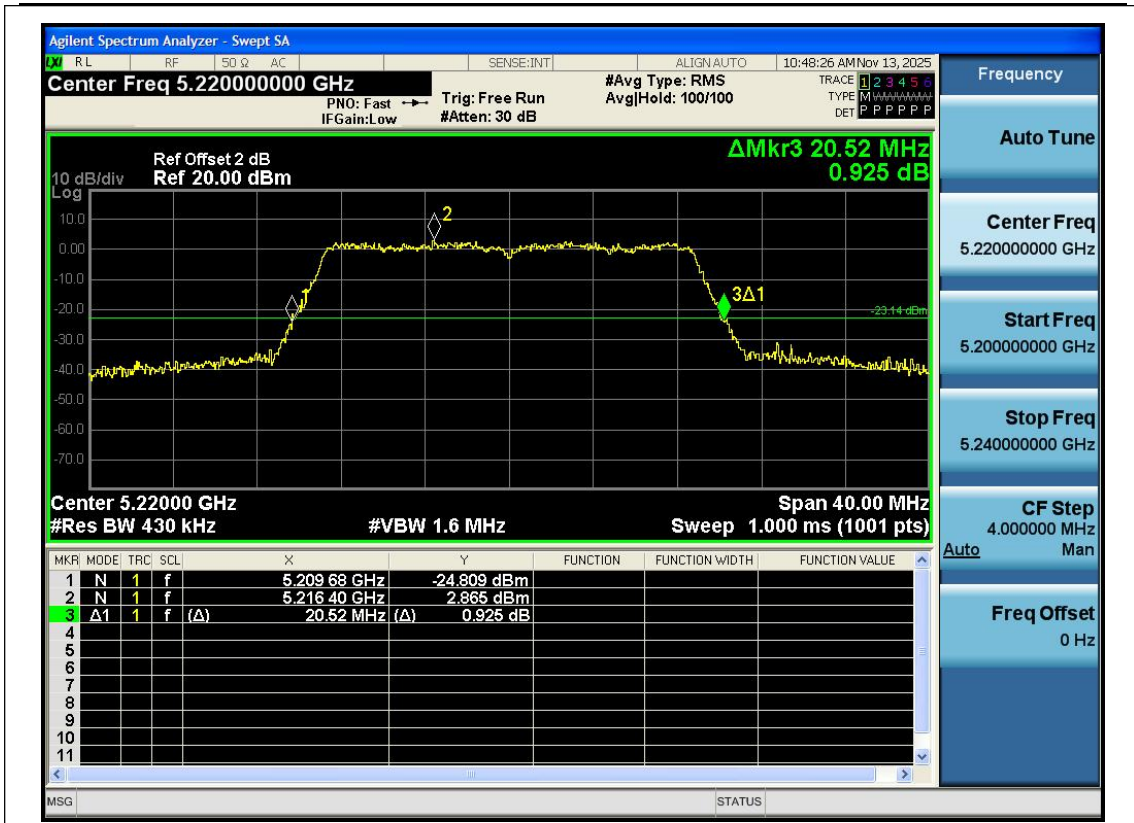
11AC20SISO-Ant1-5220
