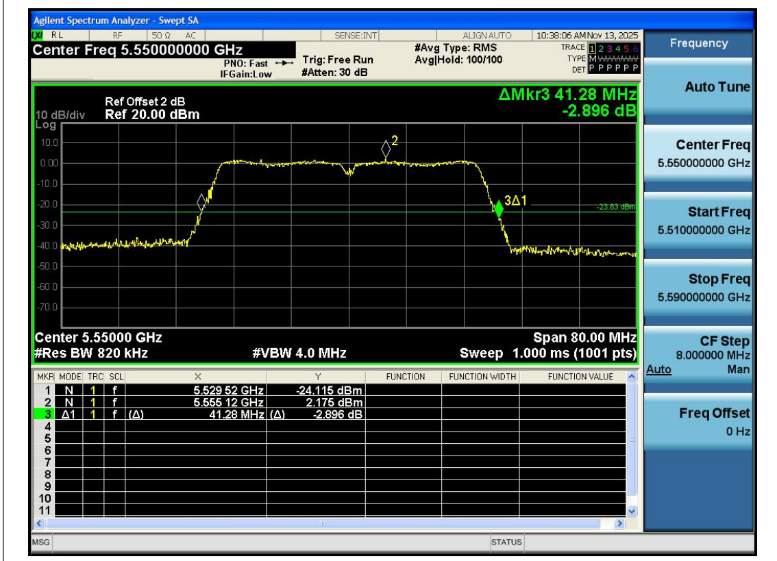
11N40SISO-Ant1-5550
