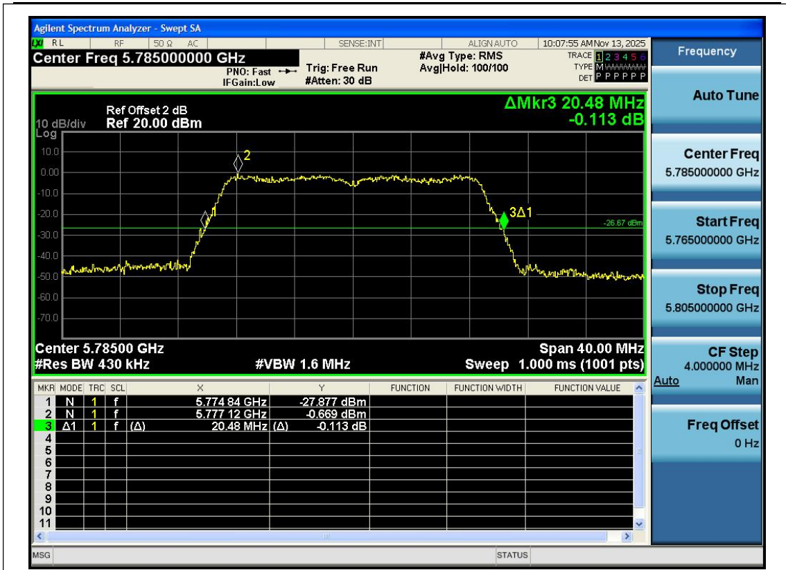
11N20SISO-Ant1-5785
