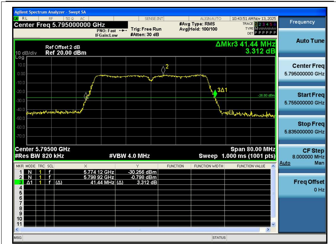
11N40SISO-Ant1-5795
