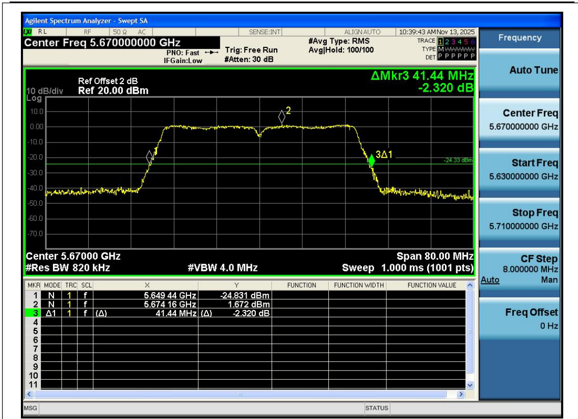
11N40SISO-Ant1-5670
