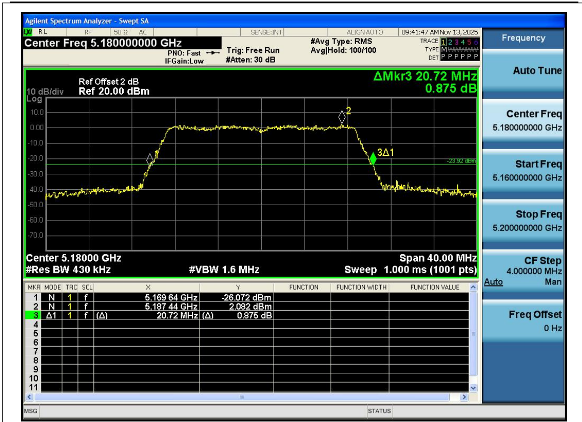
11N20SISO-Ant1-5180
