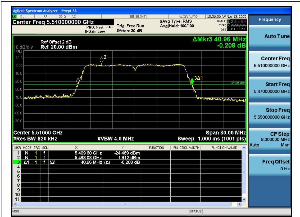
11N40SISO-Ant1-5510
