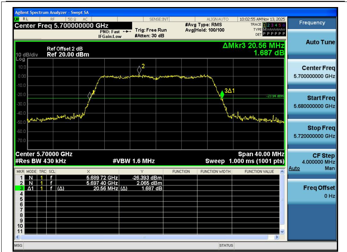
11N20SISO-Ant1-5700
