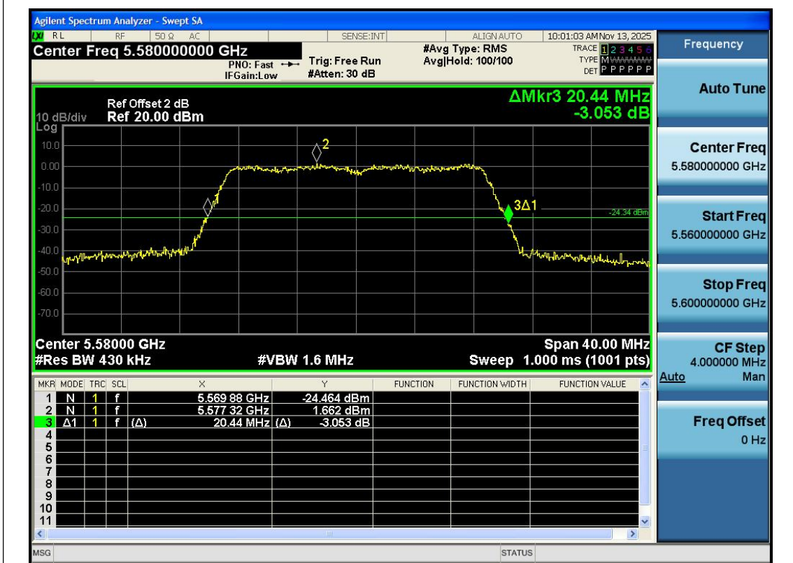
11N20SISO-Ant1-5580
