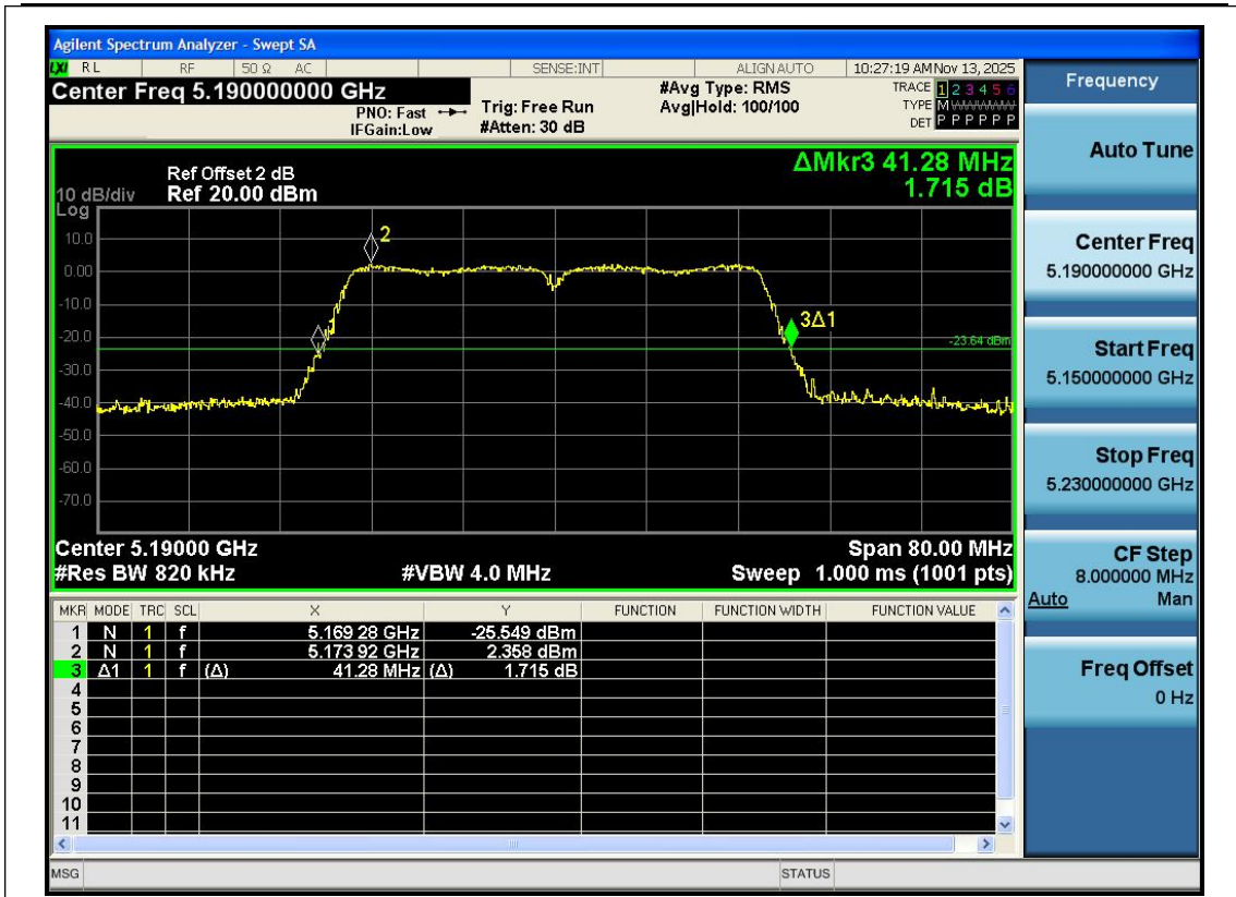
11N40SISO-Ant1-5190
