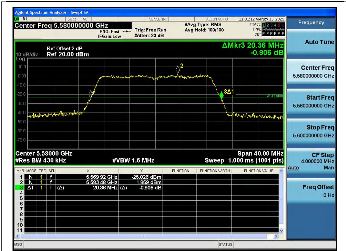
11AC20SISO-Ant1-5580
