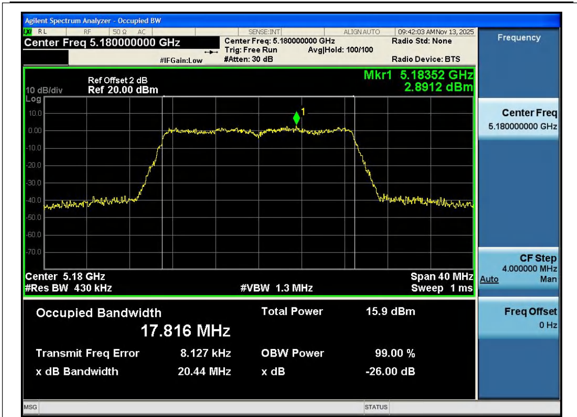
11N20SISO-Ant1-5180
