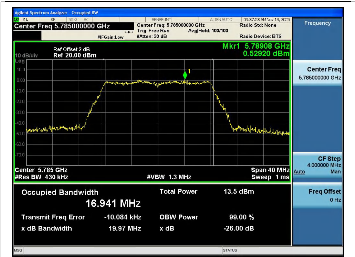
11A-Ant1-5785
