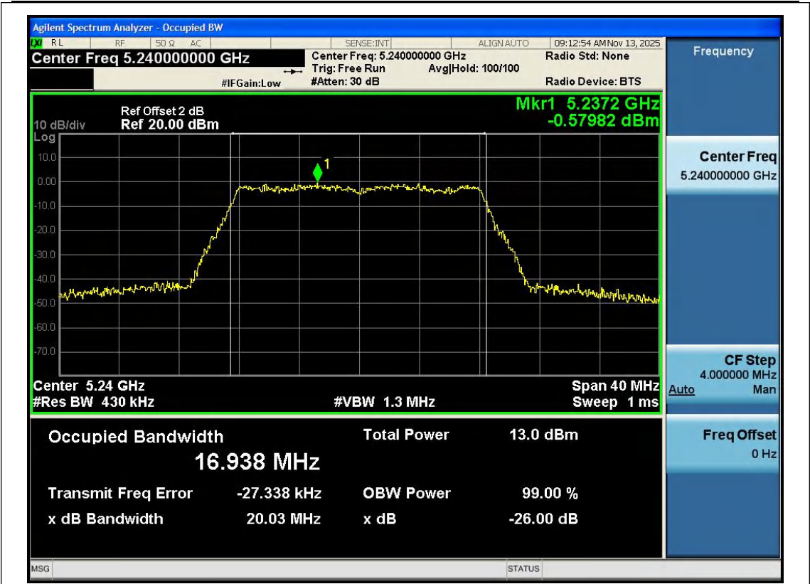
11A-Ant1-5240
