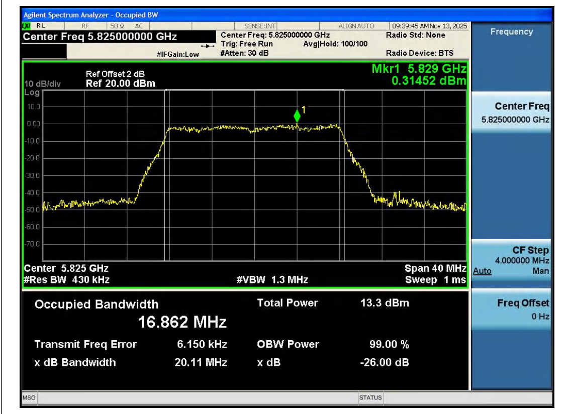
11A-Ant1-5825
