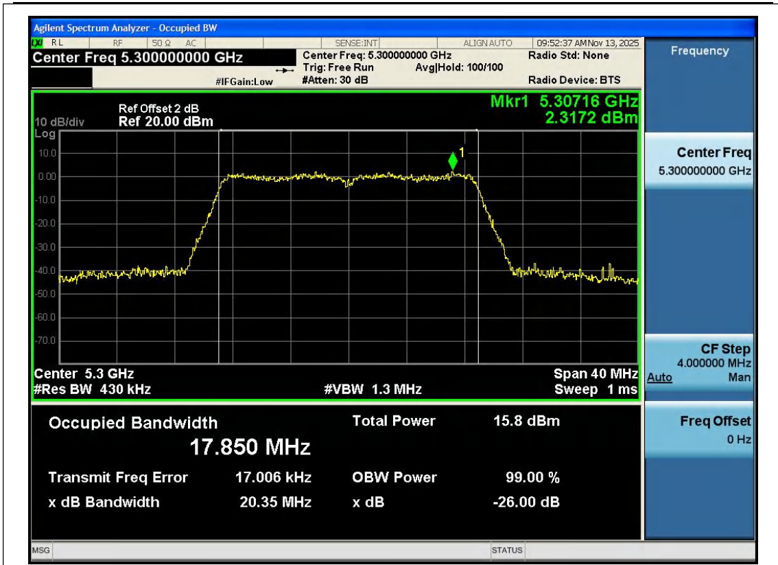
11N20SISO-Ant1-5300
