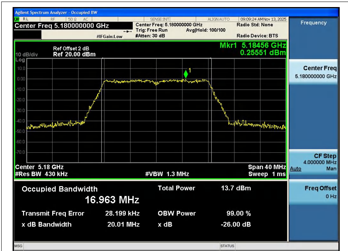
11A-Ant1-5180
