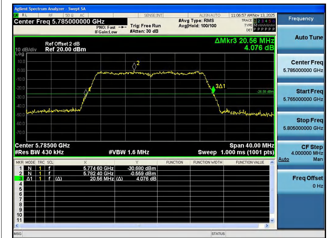
11AC20SISO-Ant1-5785
