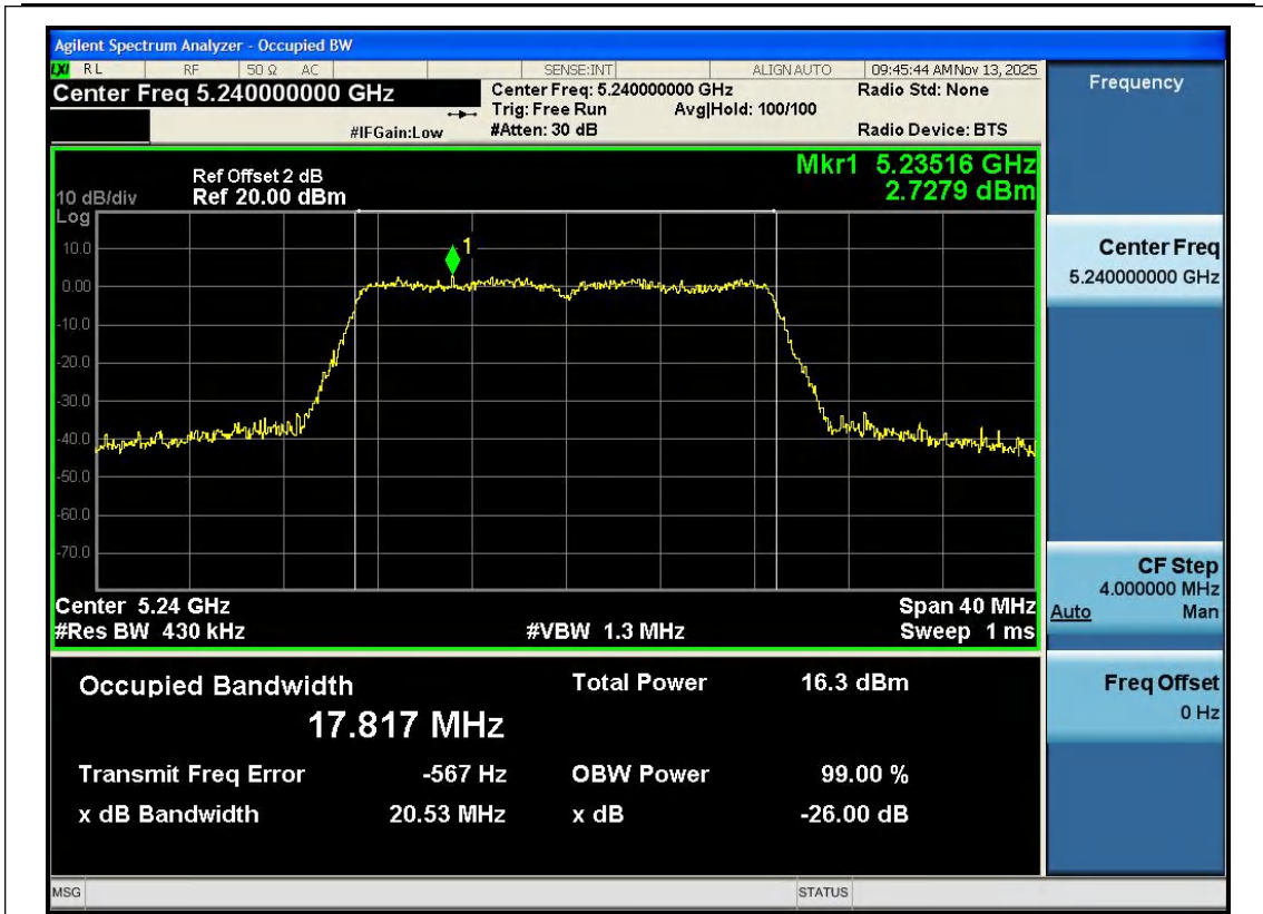
11N20SISO-Ant1-5240
