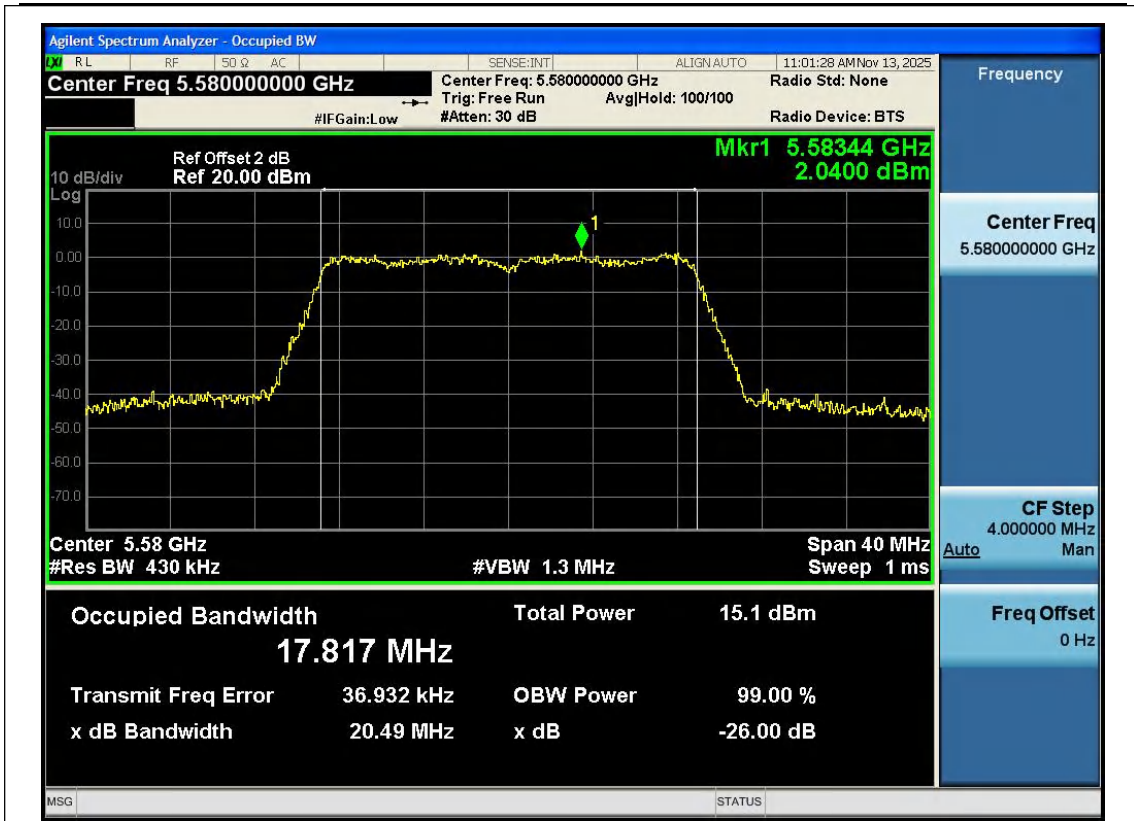
11AC20SISO-Ant1-5580
