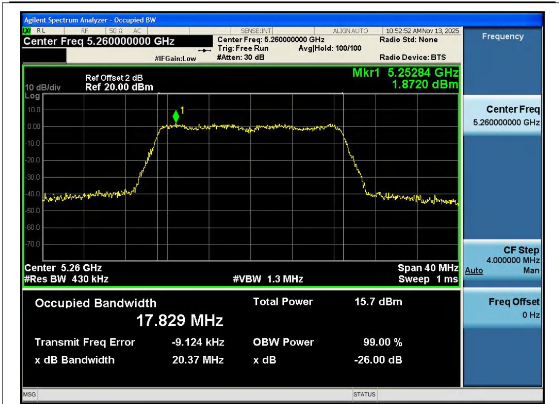
11AC20SISO-Ant1-5260
