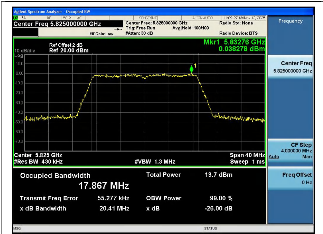
11AC20SISO-Ant1-5825
