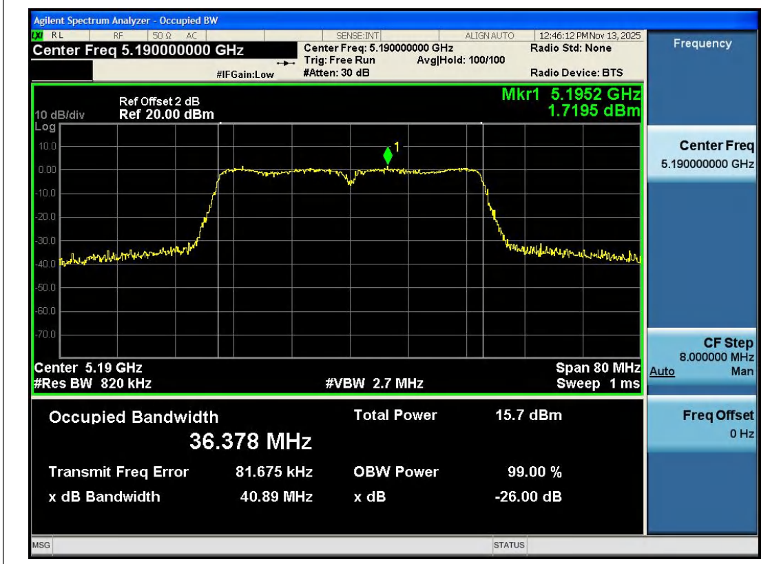
11AC40SISO-Ant1-5190
