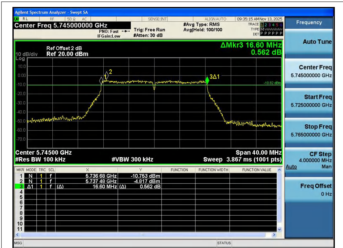
11A-Ant1-5745-PASS
