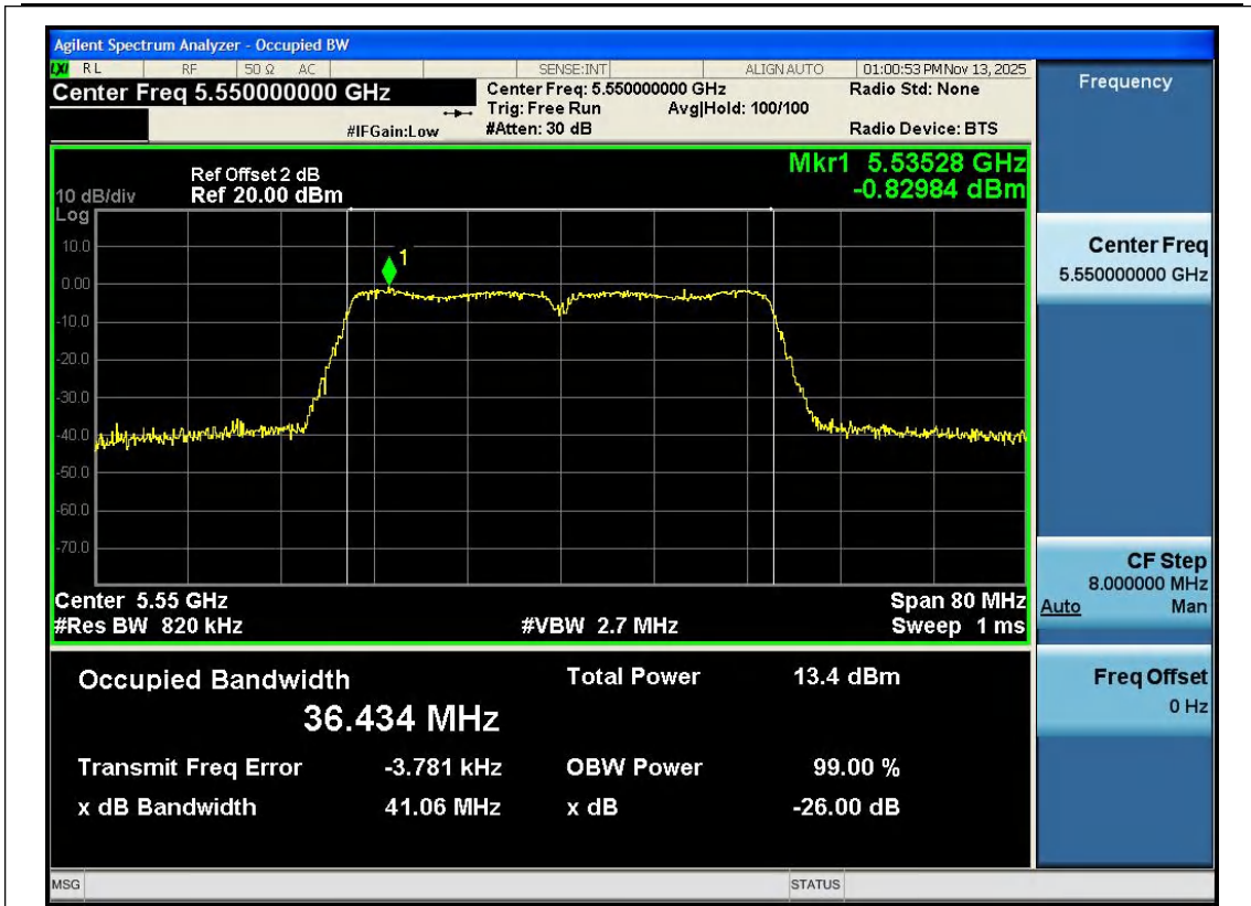
11AC40SISO-Ant1-5550
