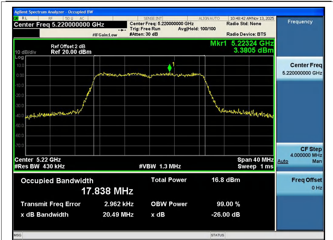
11AC20SISO-Ant1-5220
