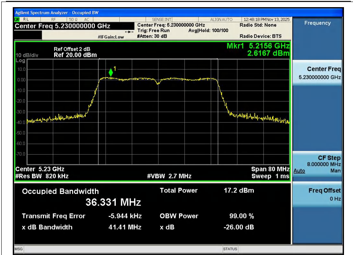
11AC40SISO-Ant1-5230
