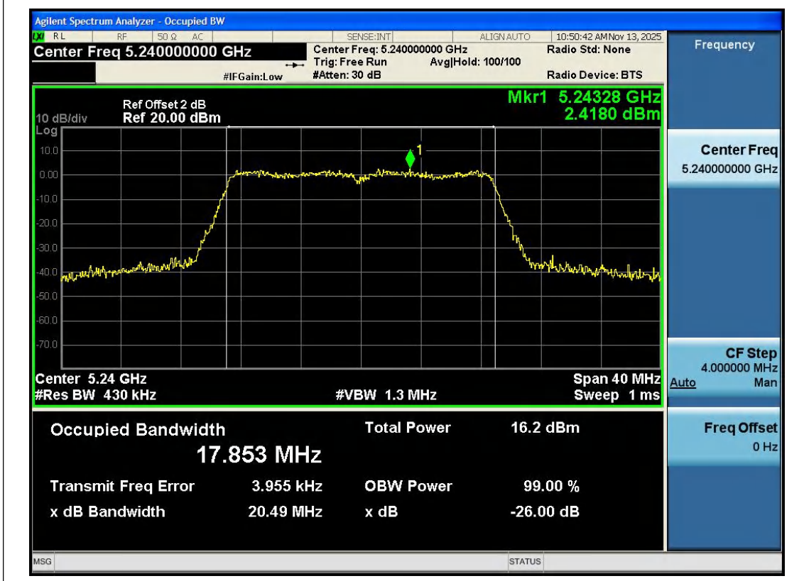
11AC20SISO-Ant1-5240
