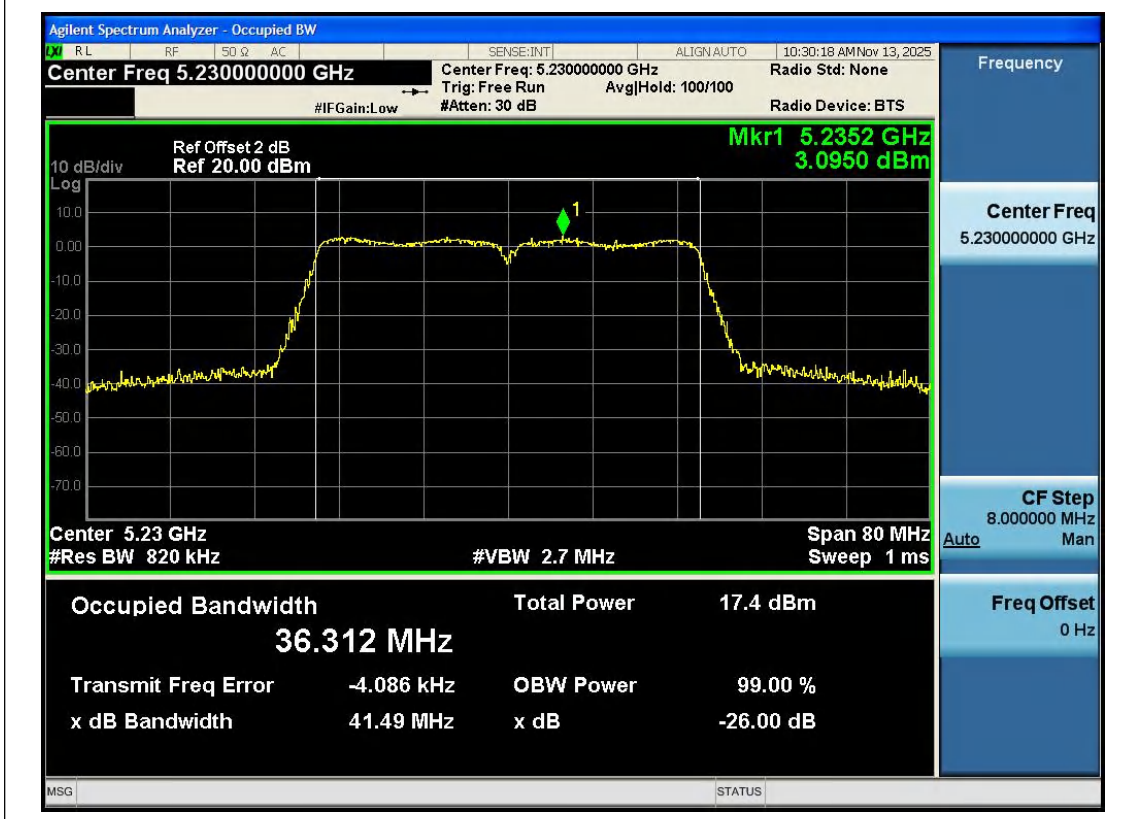
11N40SISO-Ant1-5230
