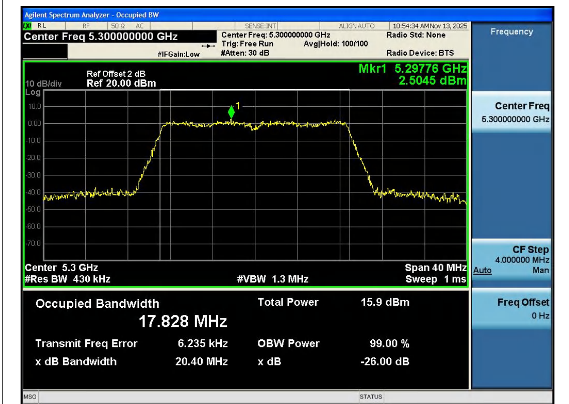
11AC20SISO-Ant1-5300
