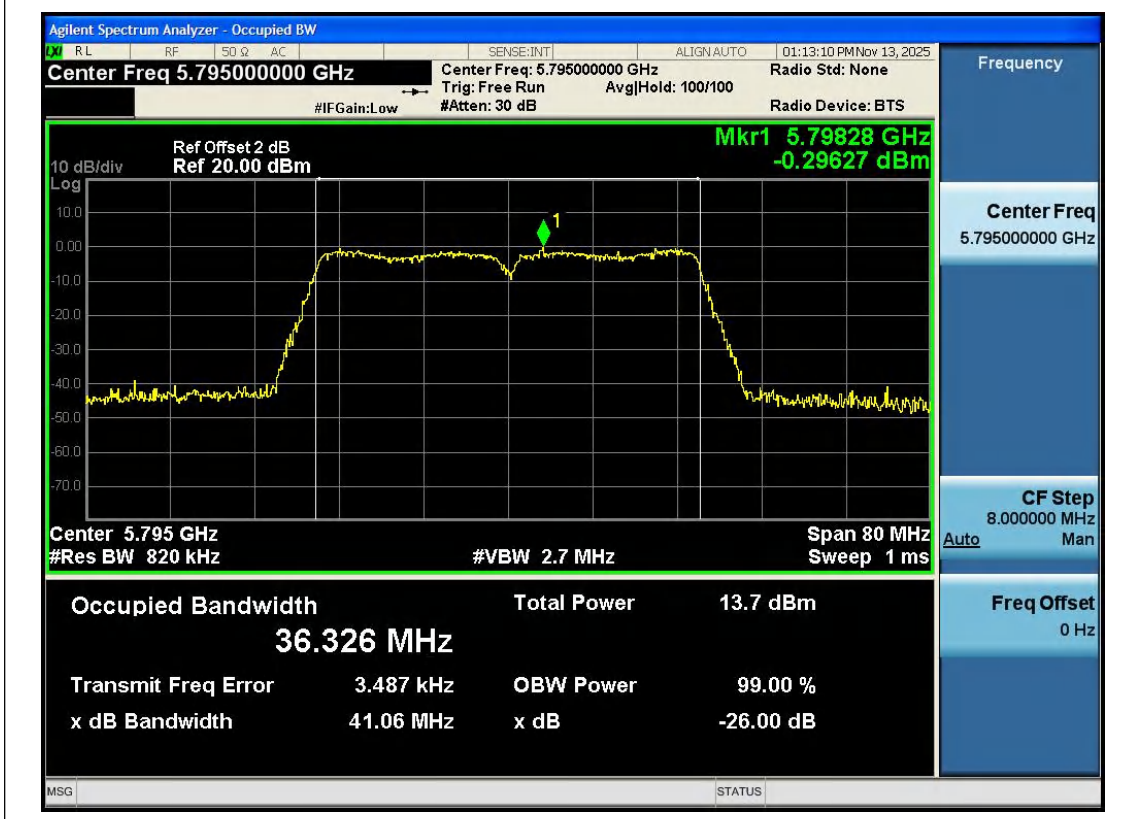
11AC40SISO-Ant1-5795
