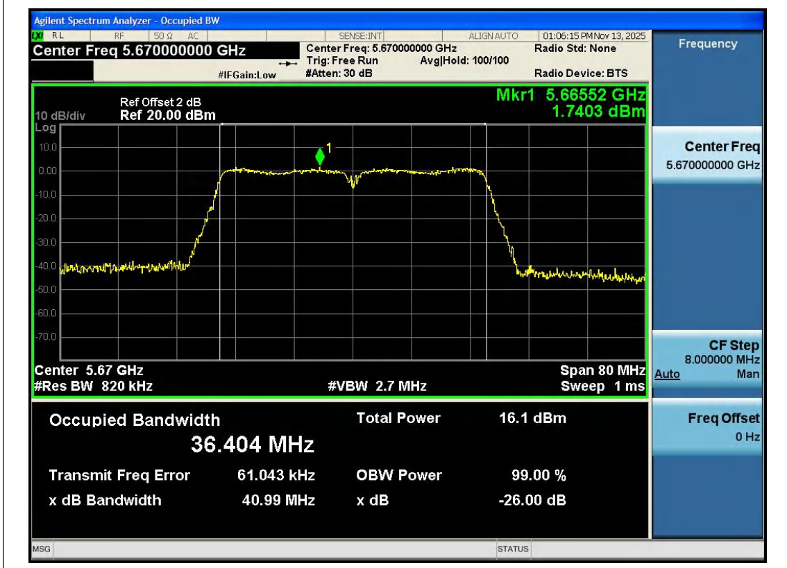
11AC40SISO-Ant1-5670
