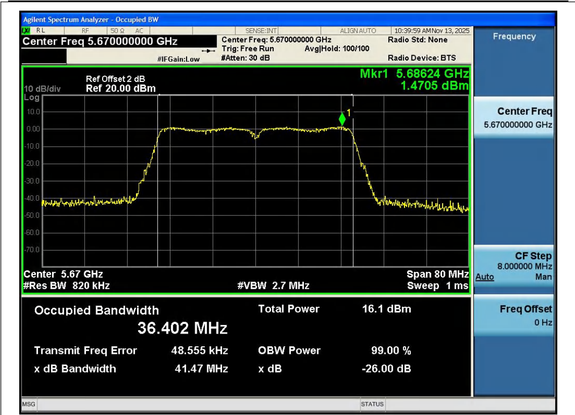
11N40SISO-Ant1-5670
