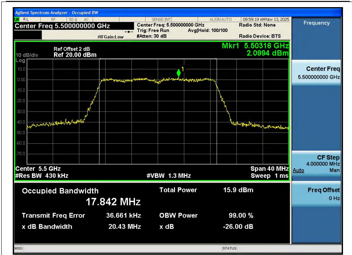
11N20SISO-Ant1-5500
