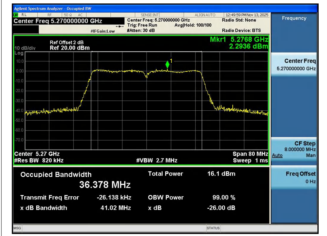
11AC40SISO-Ant1-5270
