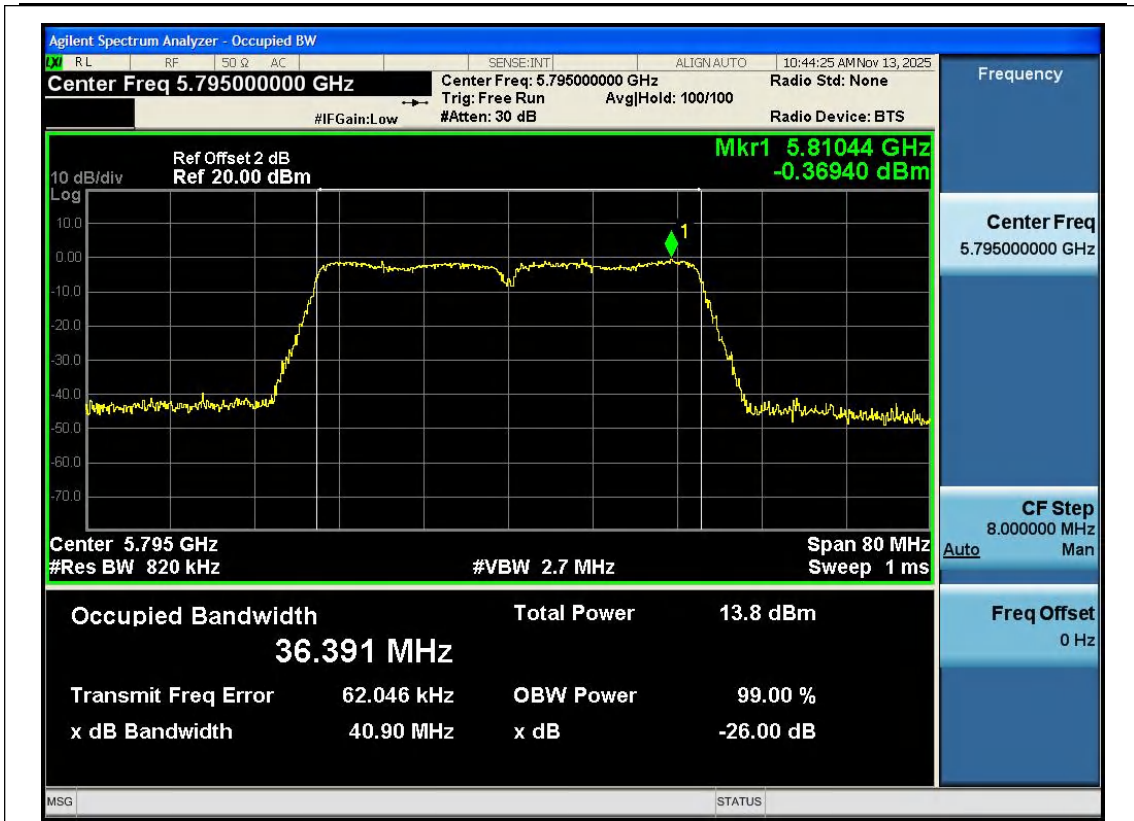
11N40SISO-Ant1-5795
