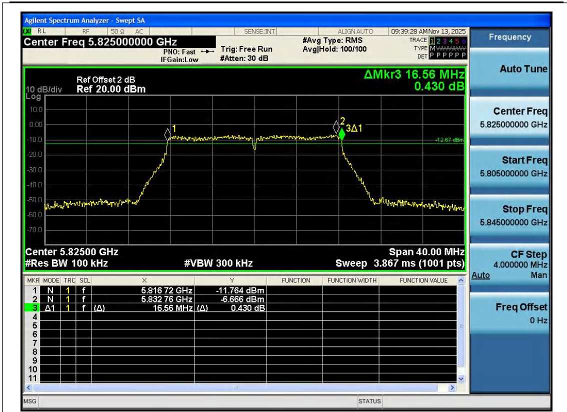
11A-Ant1-5825-PASS
