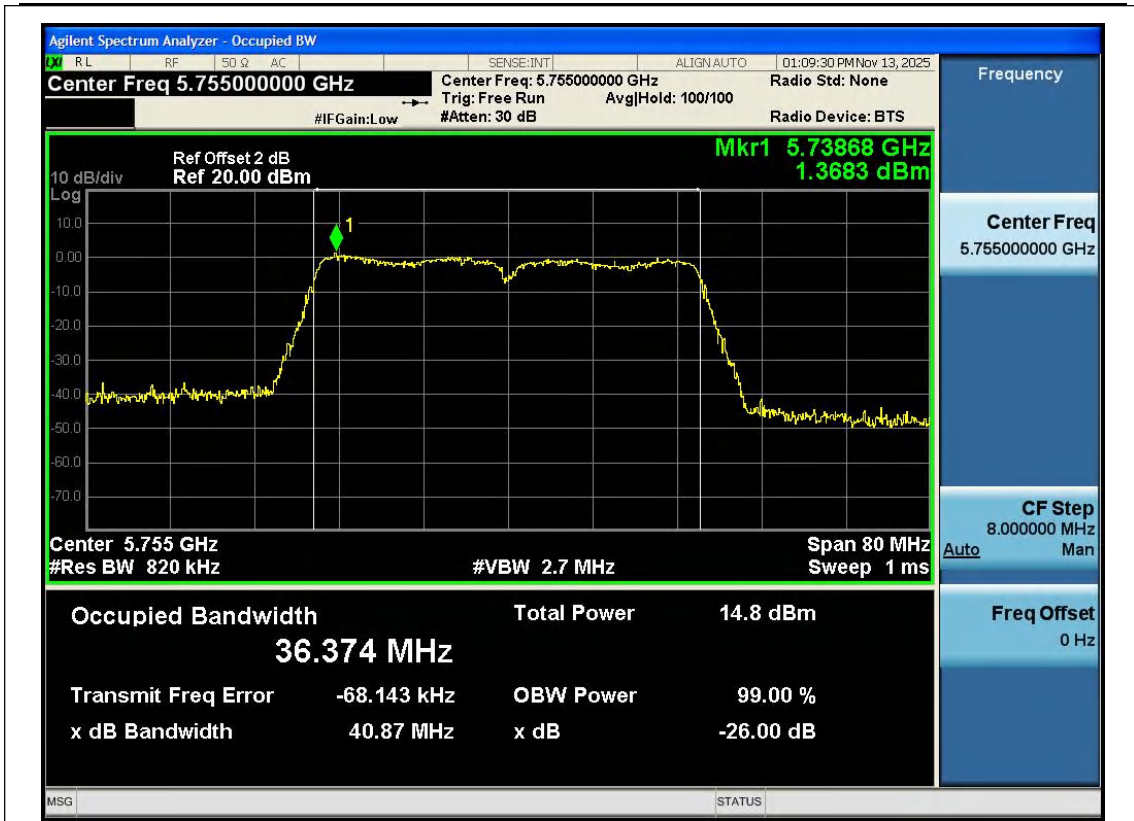
11AC40SISO-Ant1-5755
