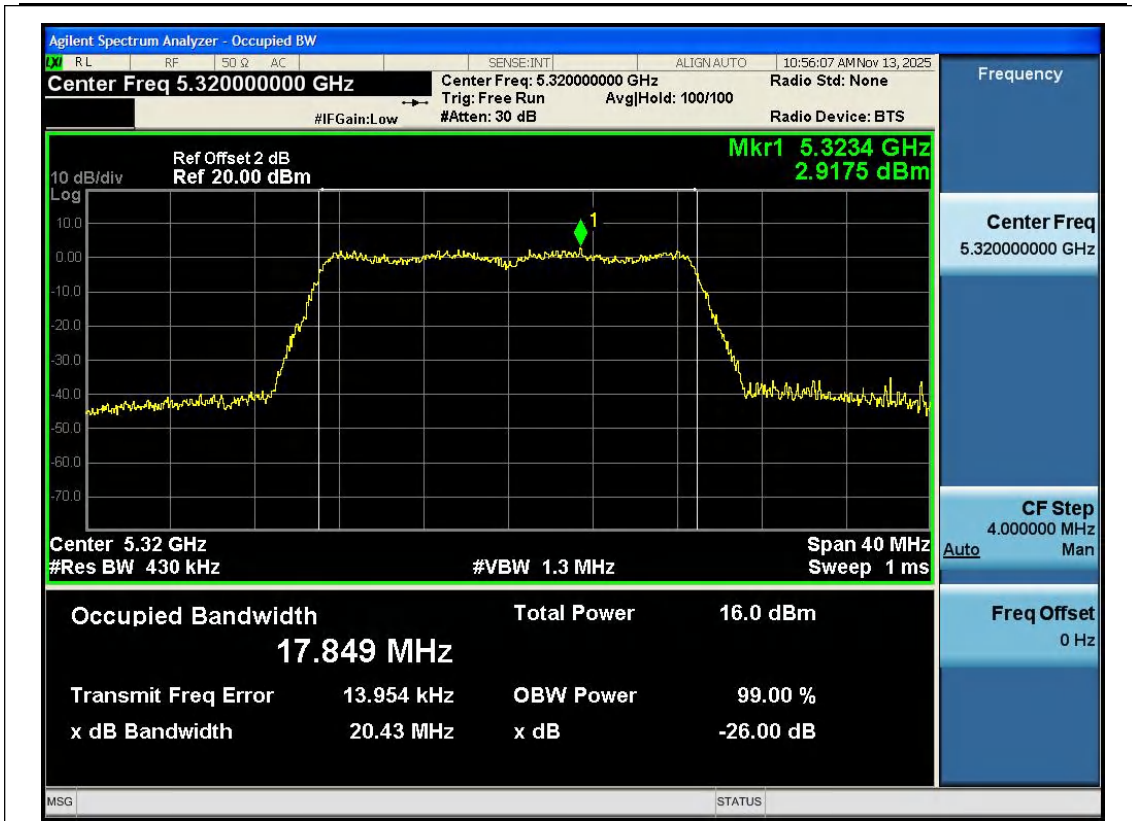
11AC20SISO-Ant1-5320
