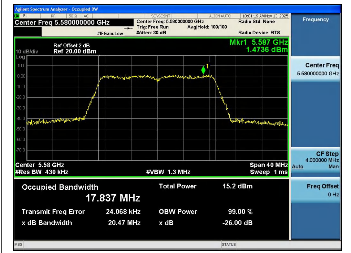
11N20SISO-Ant1-5580
