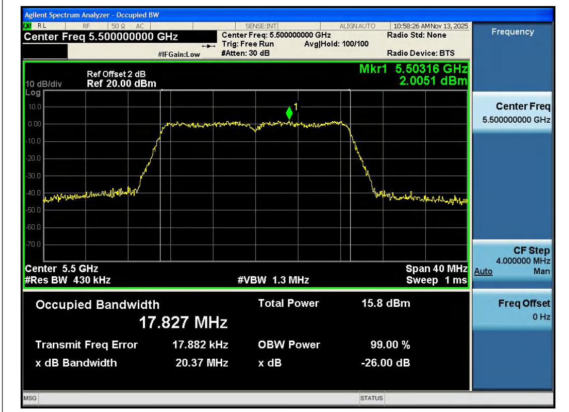
11AC20SISO-Ant1-5500
