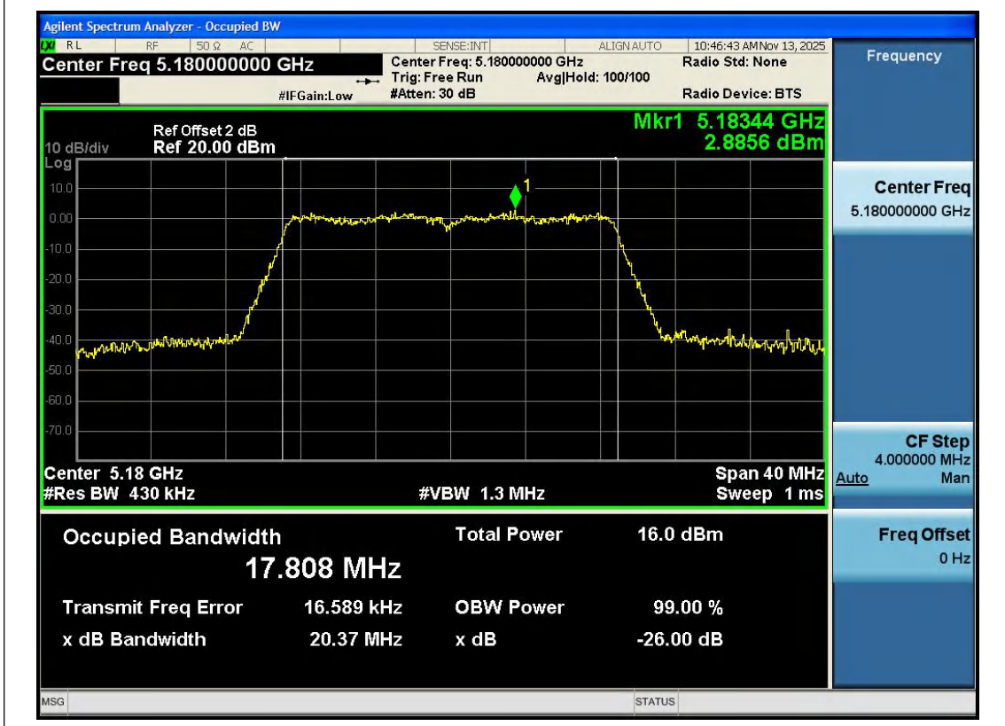
11AC20SISO-Ant1-5180
