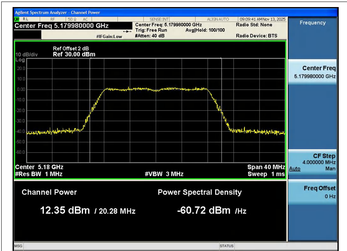
11A-Ant1-5180-PASS
