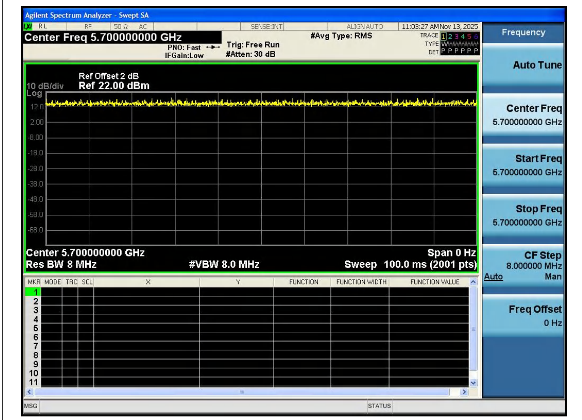
NTNV-11AC20SISO-Ant1-5700
