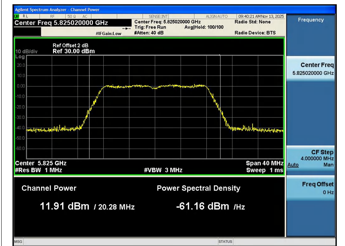
11A-Ant1-5825-PASS
