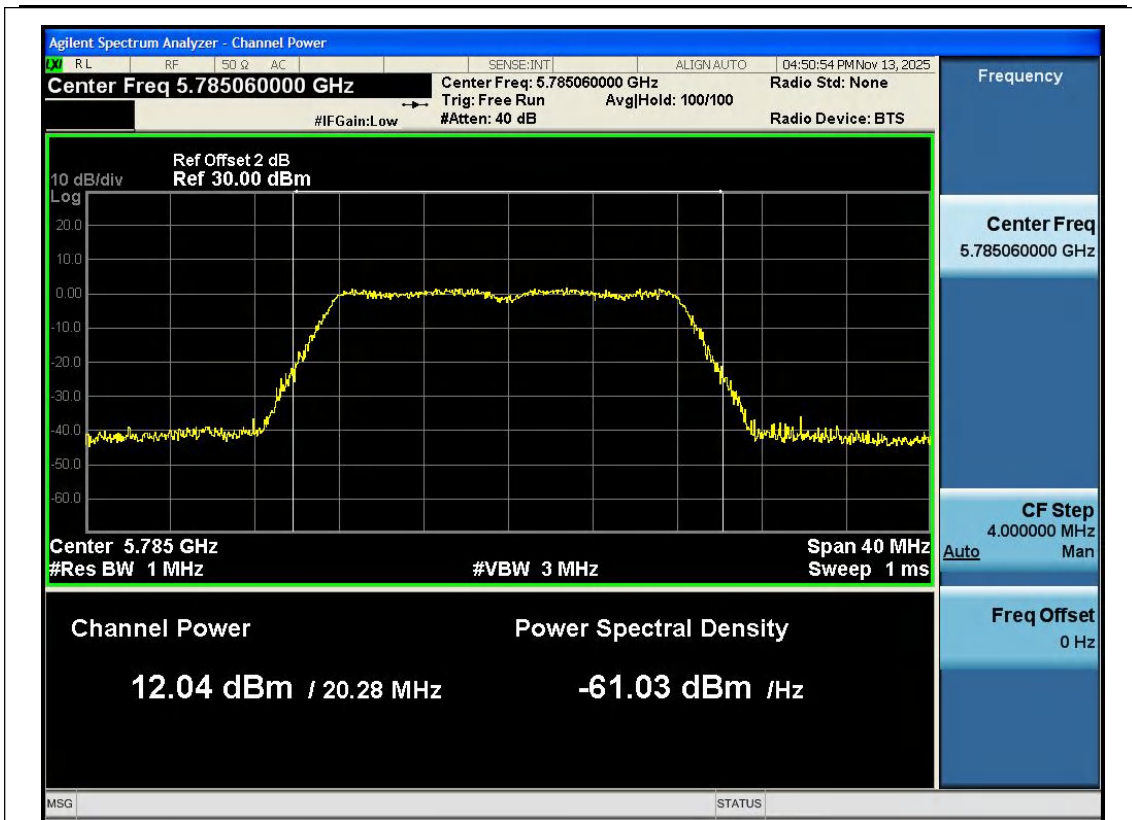
11A-Ant1-5785-PASS
