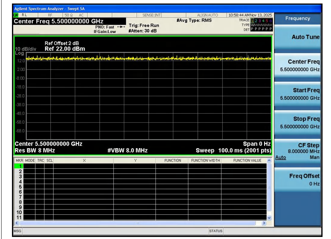
NTNV-11AC20SISO-Ant1-5500
