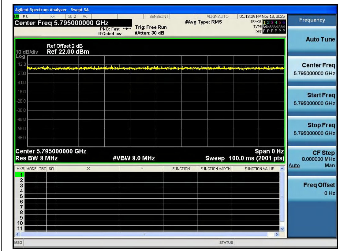
NTNV-11AC40SISO-Ant1-5795
