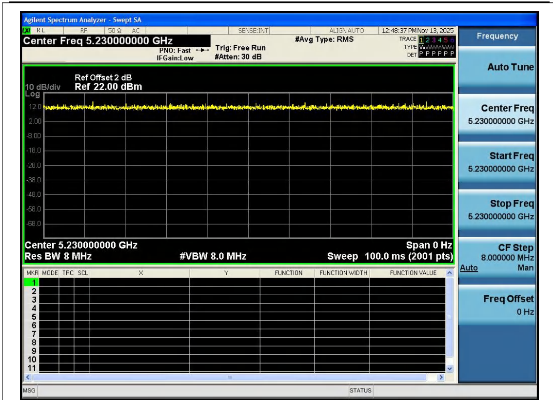
NTNV-11AC40SISO-Ant1-5230
