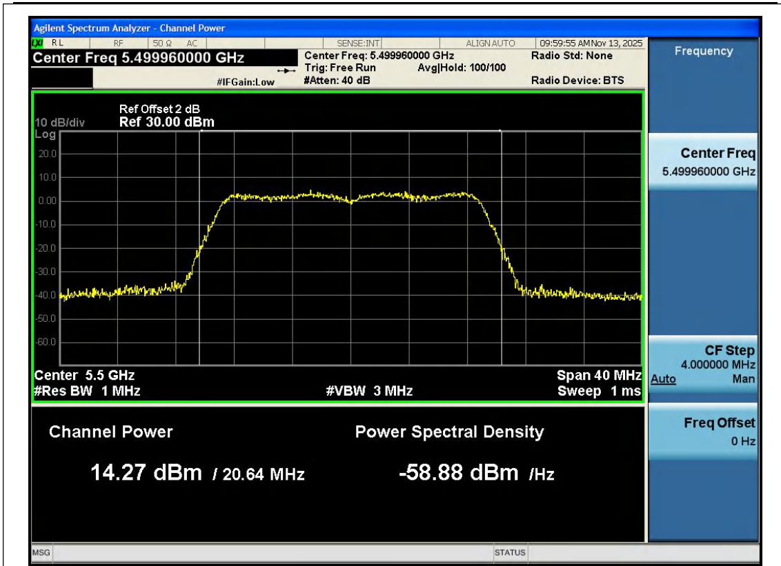
11N20SISO-Ant1-5500-PASS
