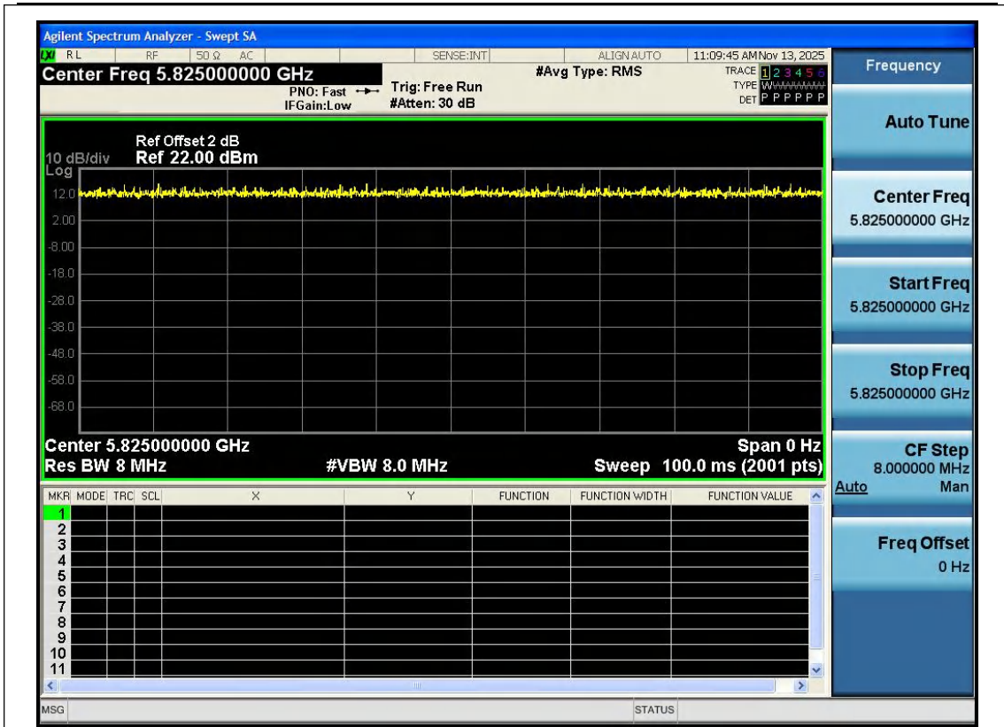
NTNV-11AC20SISO-Ant1-5825
