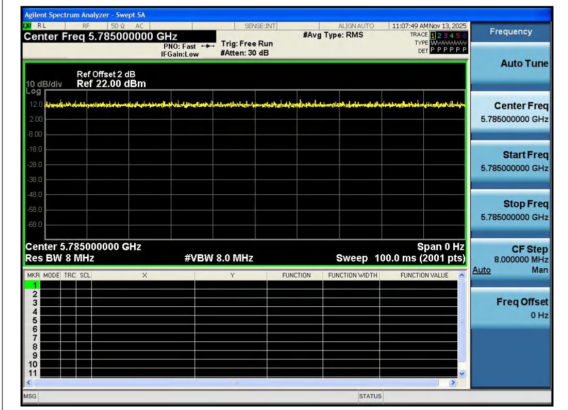
NTNV-11AC20SISO-Ant1-5785
