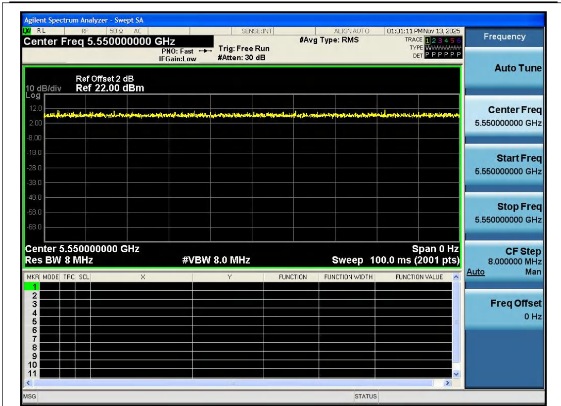
NTNV-11AC40SISO-Ant1-5550
