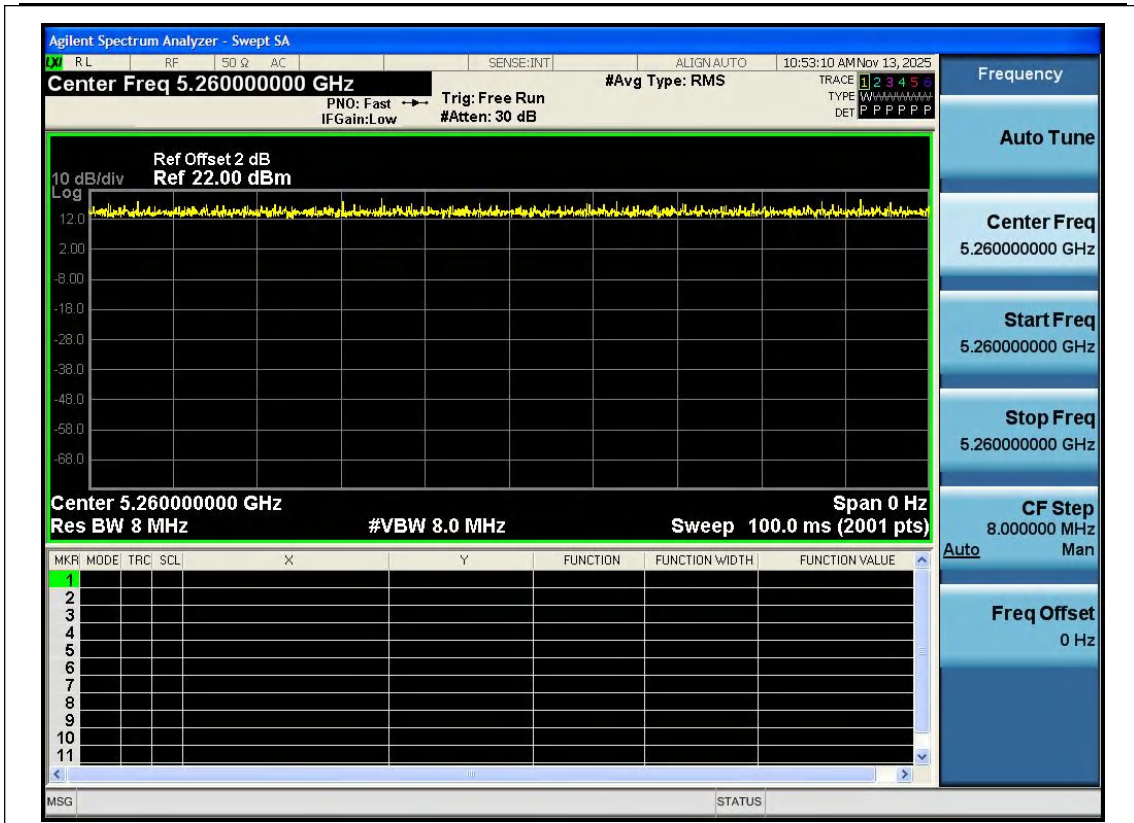
NTNV-11AC20SISO-Ant1-5260
