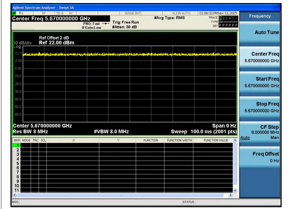
NTNV-11AC40SISO-Ant1-5670
