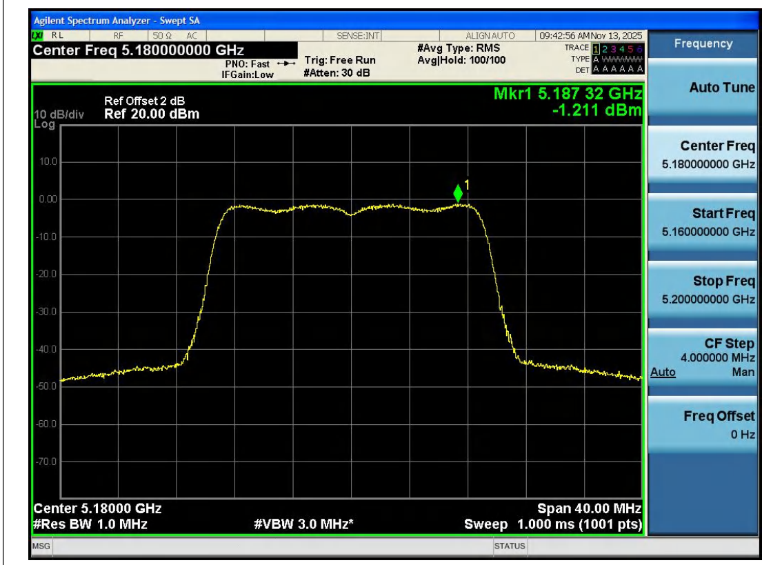
11N20SISO-Ant1-5180-PASS
