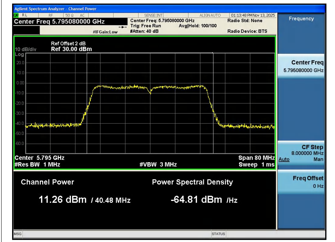
11AC40SISO-Ant1-5795-PASS
