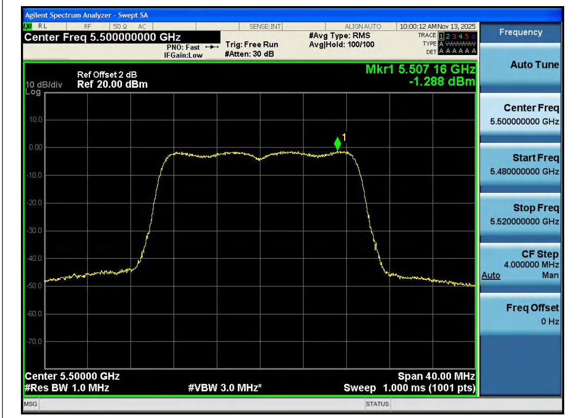
11N20SISO-Ant1-5500-PASS
