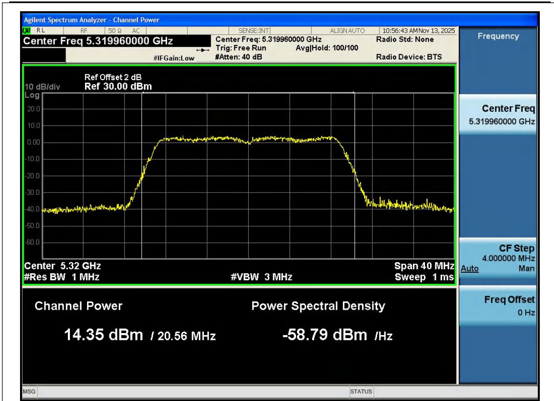
11AC20SISO-Ant1-5320-PASS
