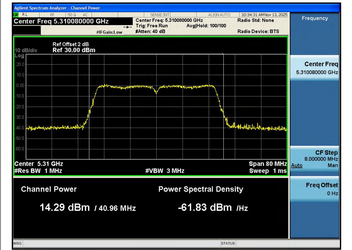
11N40SISO-Ant1-5310-PASS
