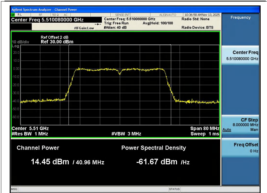
11N40SISO-Ant1-5510-PASS
