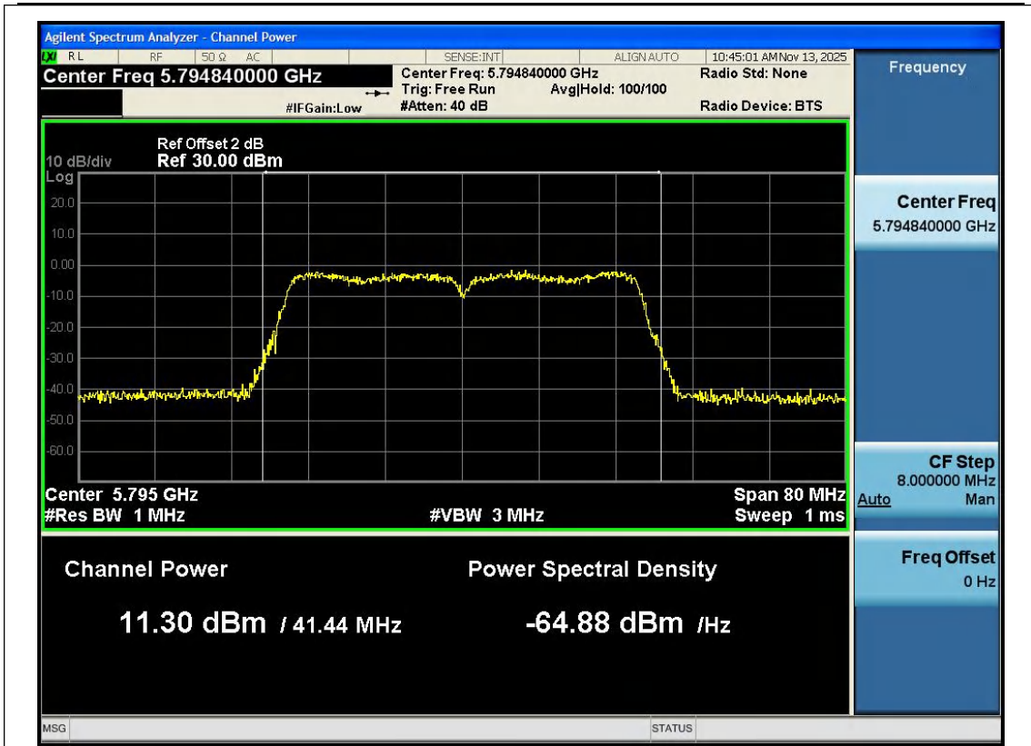
11N40SISO-Ant1-5795-PASS
