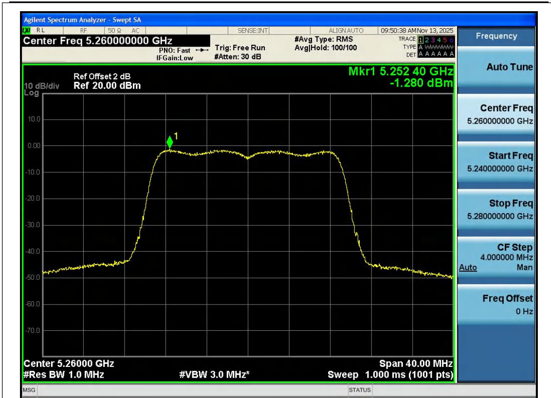
11N20SISO-Ant1-5260-PASS
