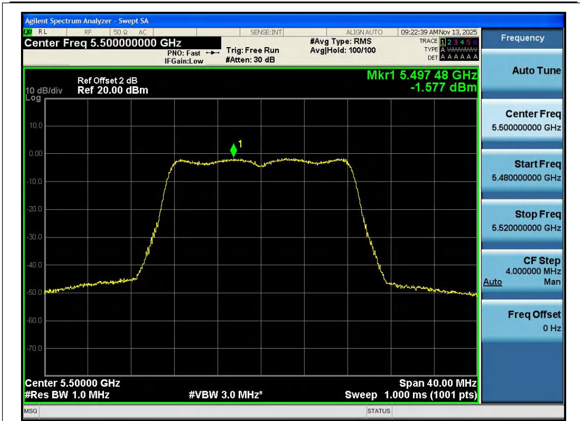
11A-Ant1-5500-PASS
