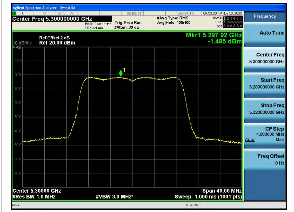
11N20SISO-Ant1-5300-PASS
