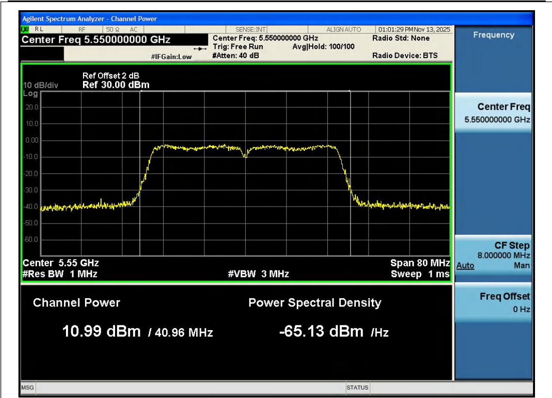
11AC40SISO-Ant1-5550-PASS
