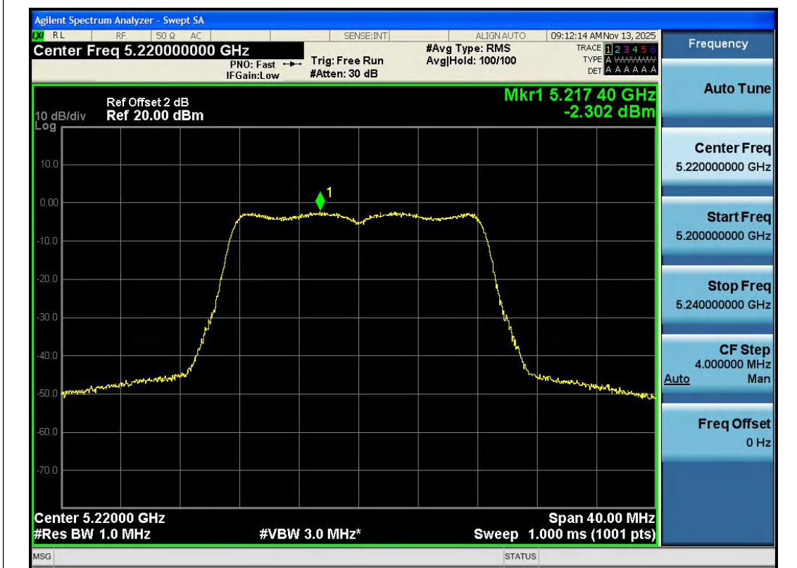
11A-Ant1-5220-PASS
