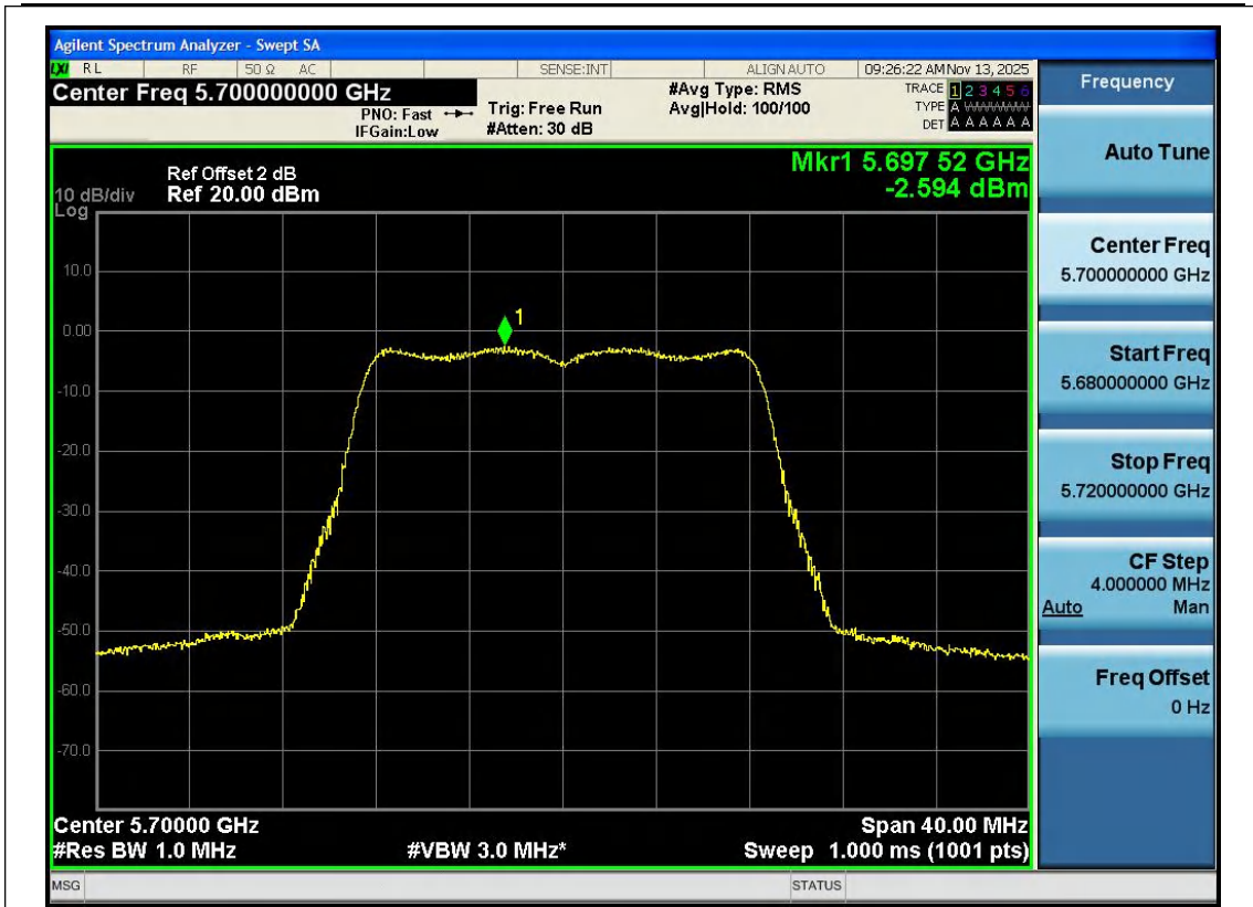
11A-Ant1-5700-PASS
