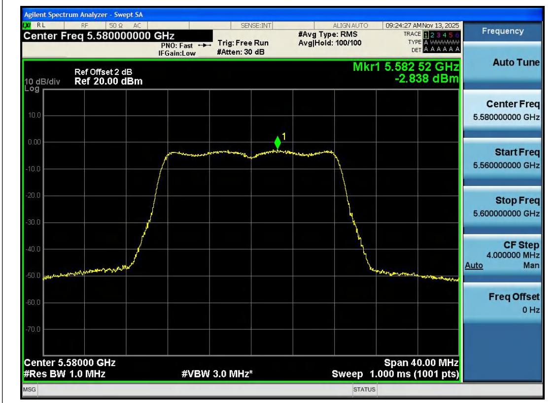
11A-Ant1-5580-PASS
