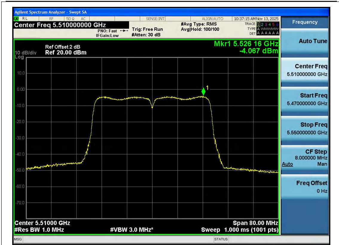
11N40SISO-Ant1-5510-PASS
