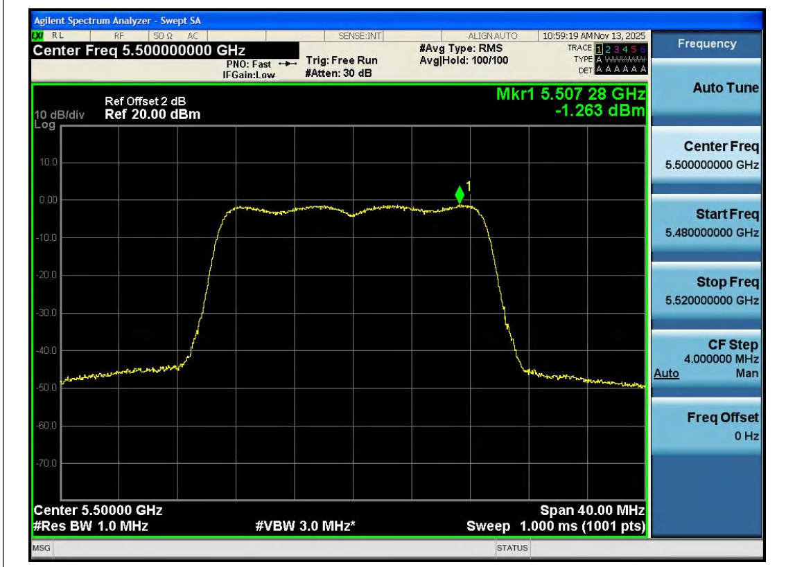
11AC20SISO-Ant1-5500-PASS
