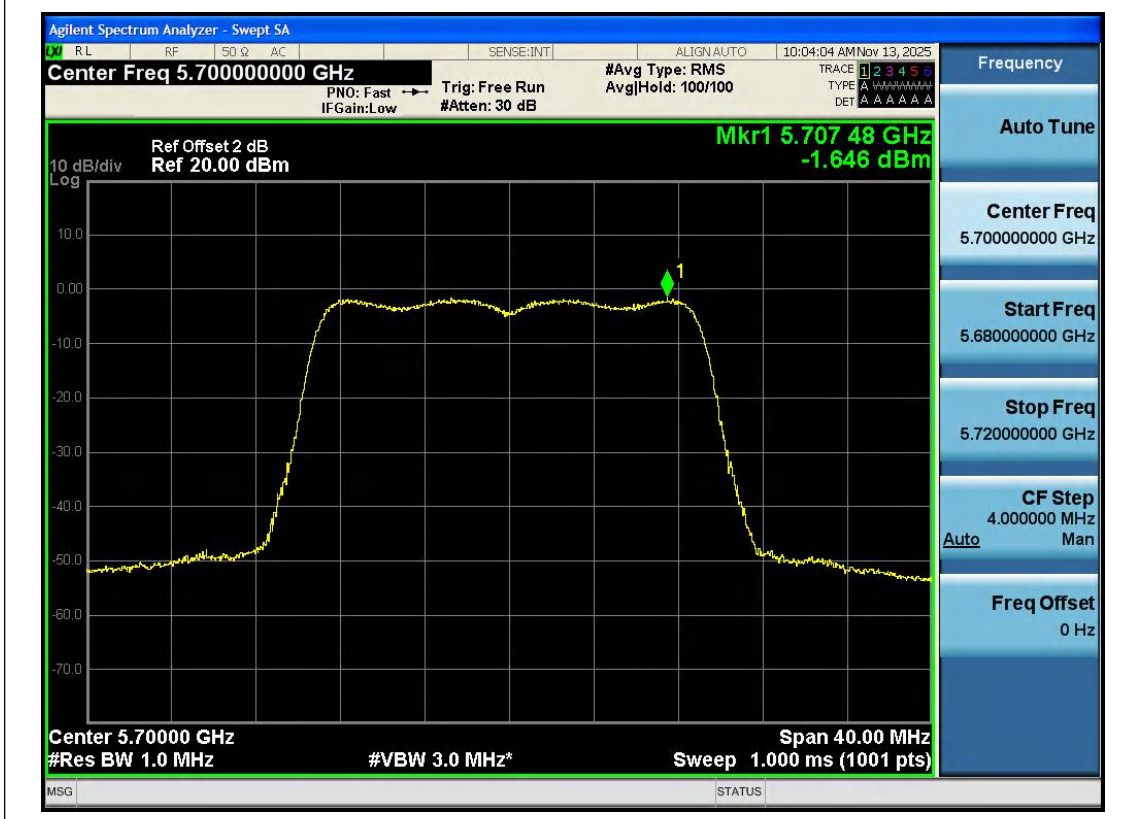
11N20SISO-Ant1-5700-PASS
