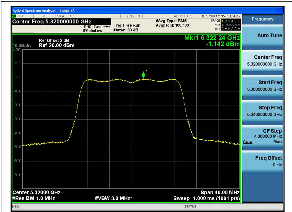
11AC20SISO-Ant1-5320-PASS
