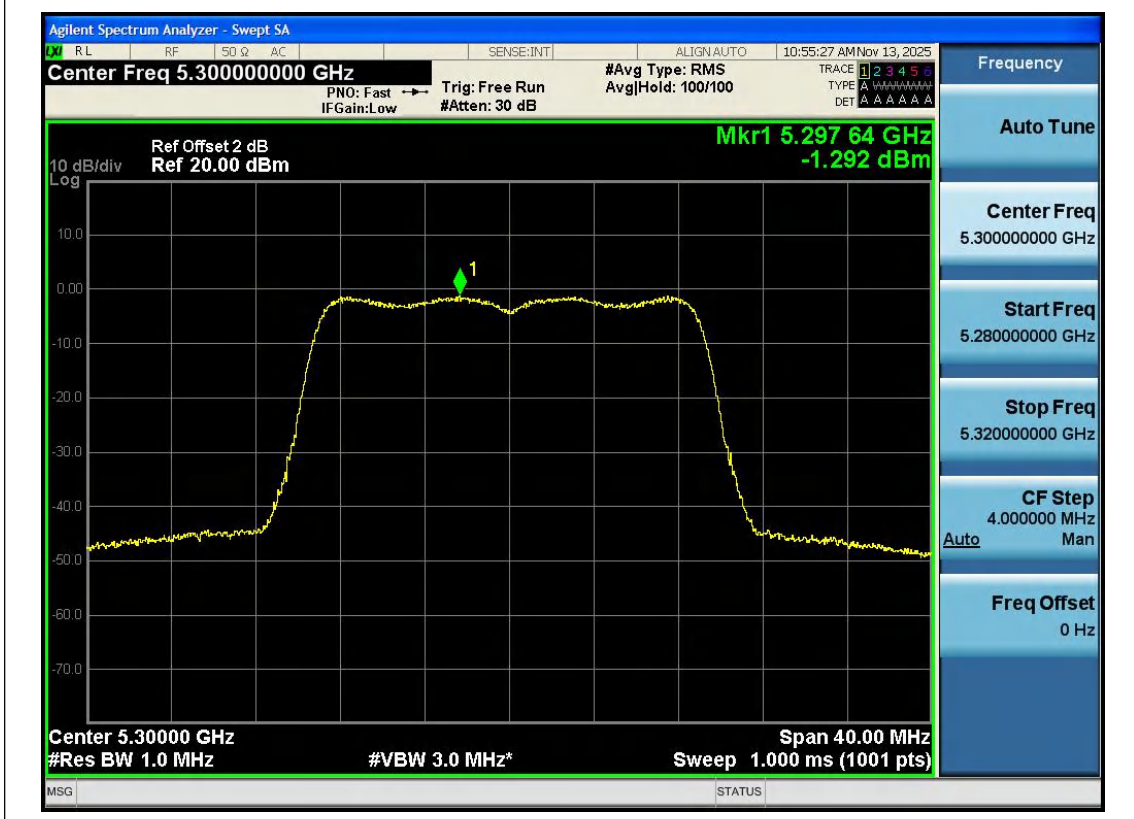
11AC20SISO-Ant1-5300-PASS
