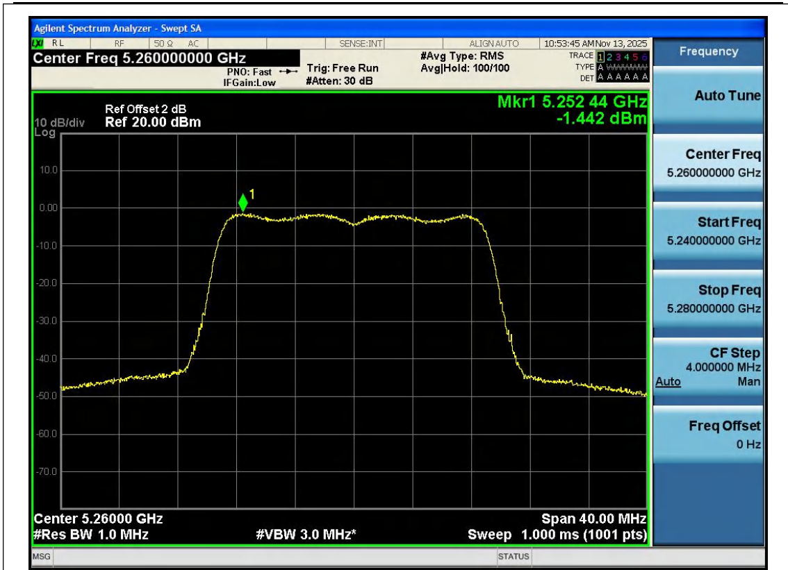
11AC20SISO-Ant1-5260-PASS
