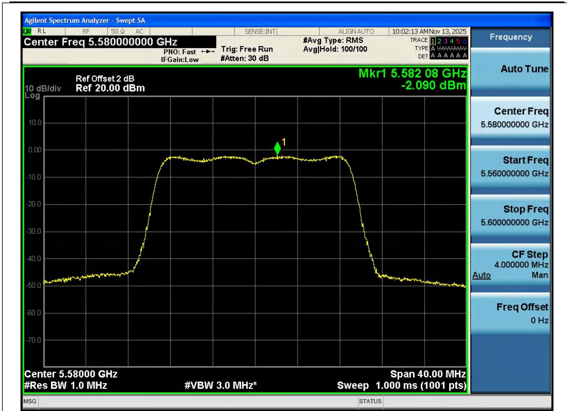
11N20SISO-Ant1-5580-PASS
