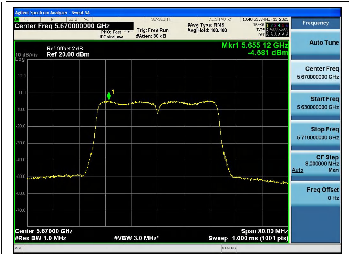
11N40SISO-Ant1-5670-PASS
