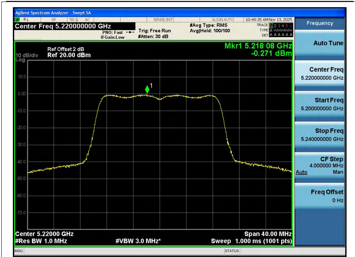
11AC20SISO-Ant1-5220-PASS
