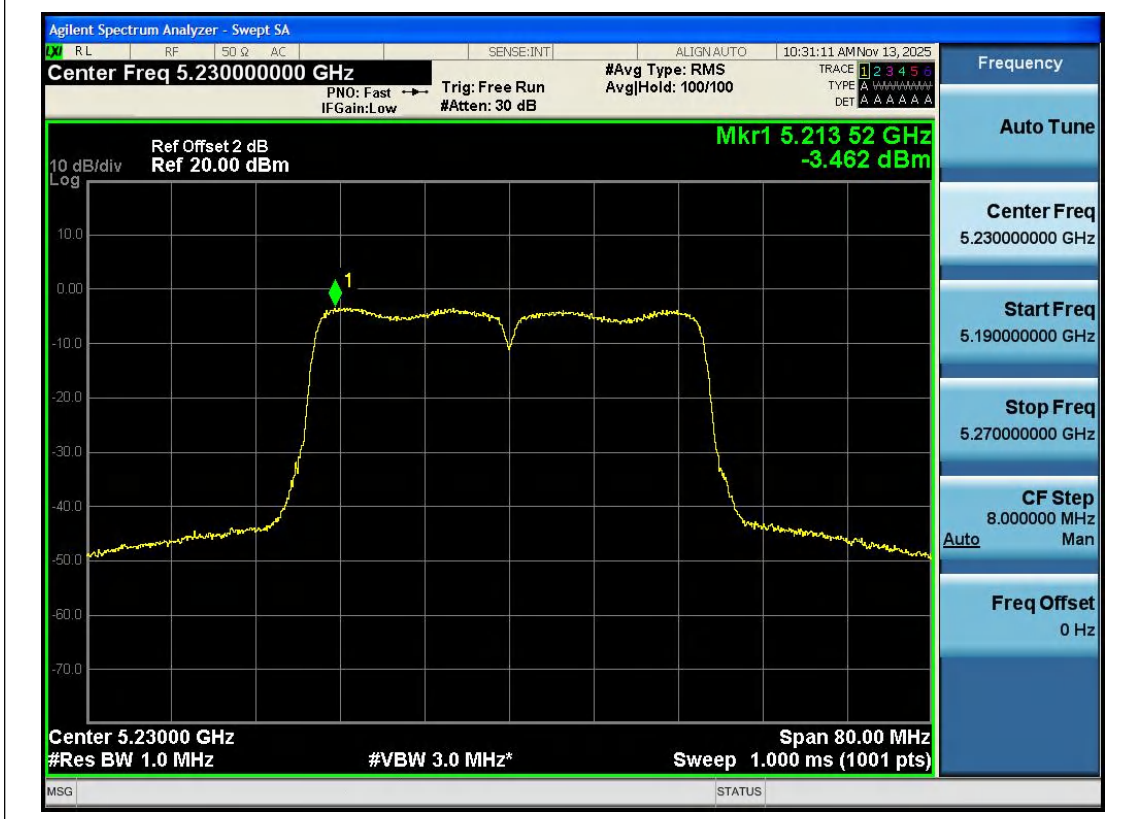
11N40SISO-Ant1-5230-PASS
