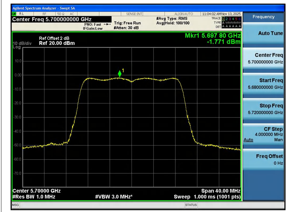
11AC20SISO-Ant1-5700-PASS
