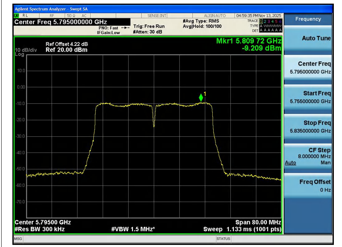
11N40SISO-Ant1-5795-PASS
