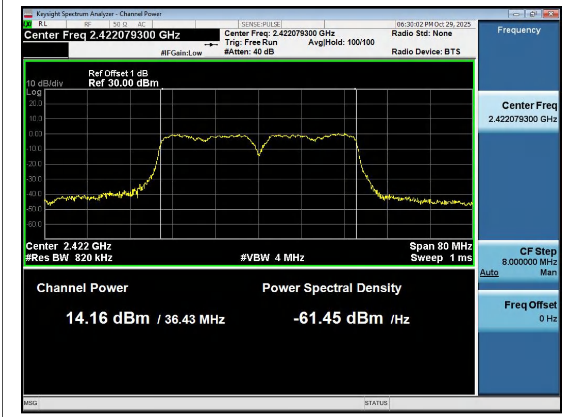
11N40SISO-Ant1-2422-PASS
