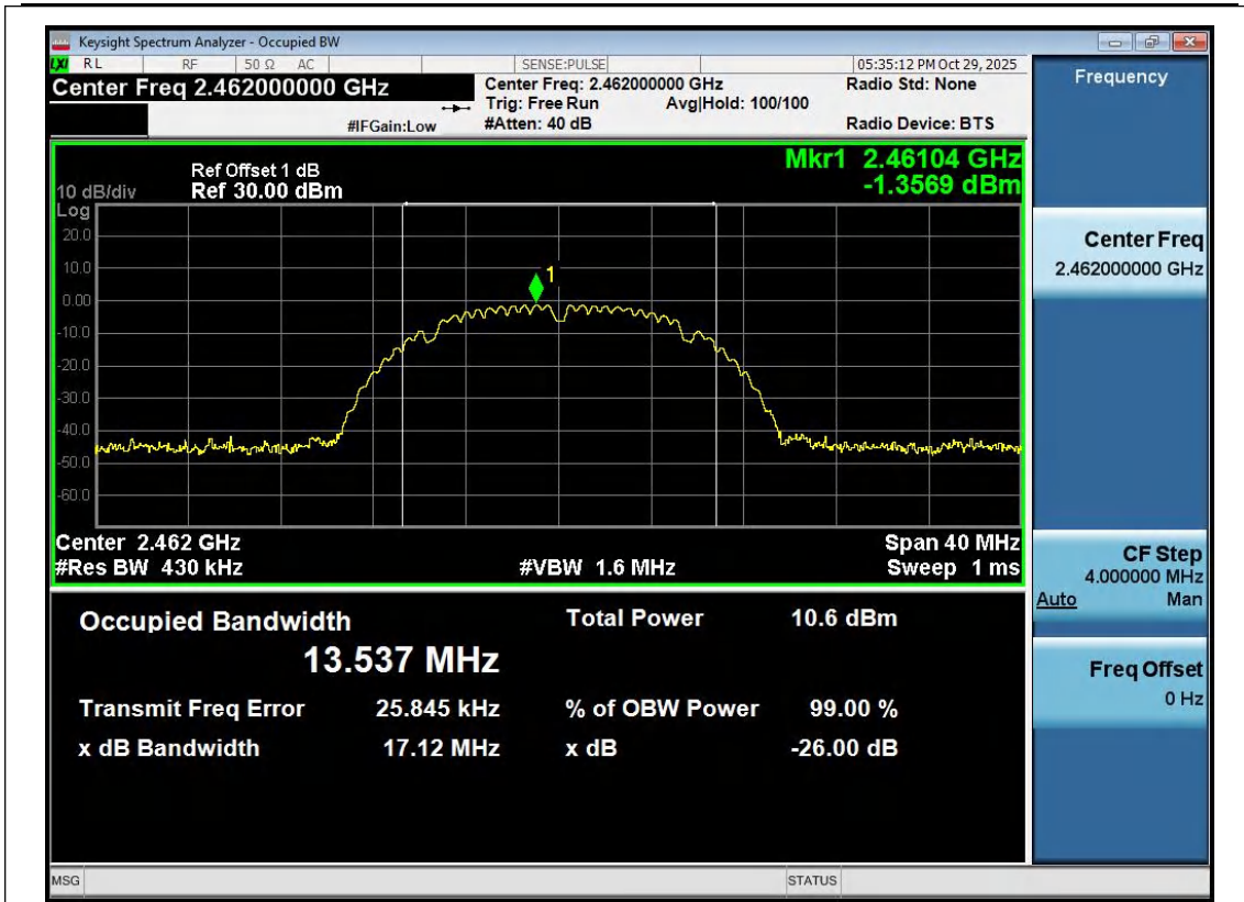
11B-Ant1-2462
