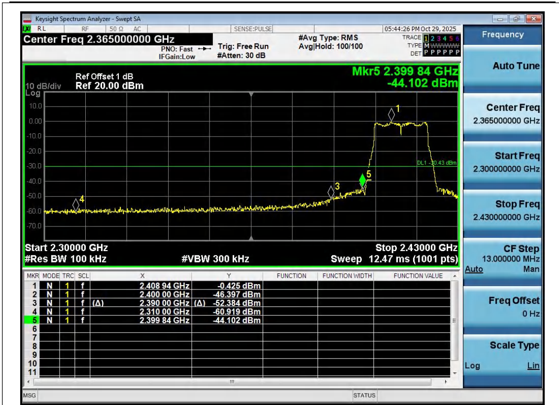
11G-Ant1-2412-PASS
