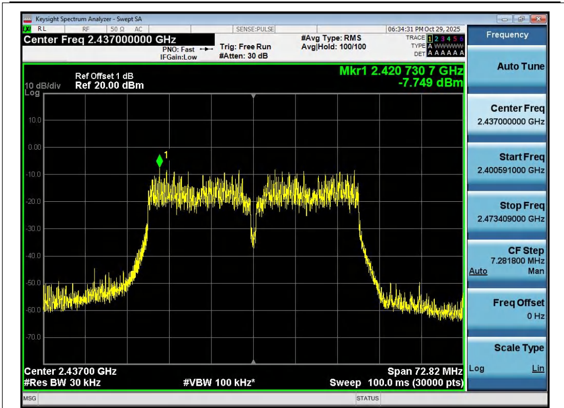
11N40SISO-Ant1-2437-PASS
