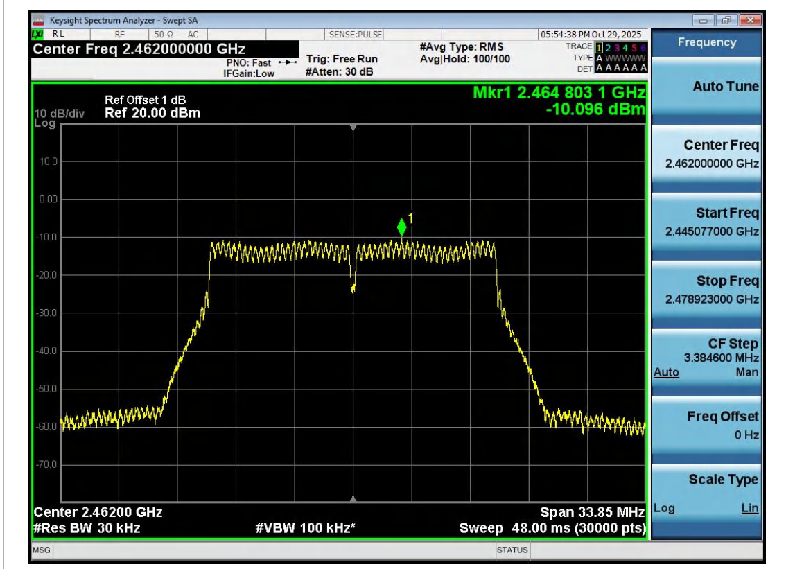
11G-Ant1-2462-PASS
