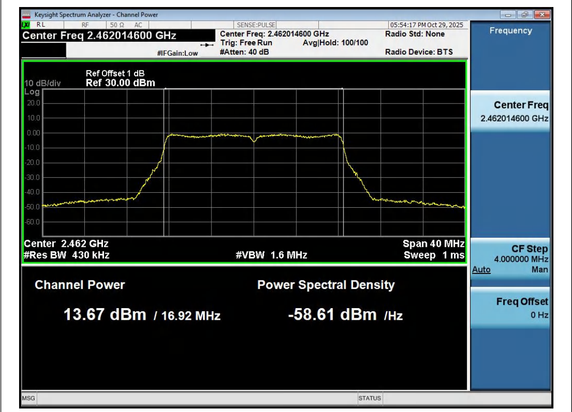
11G-Ant1-2462-PASS
