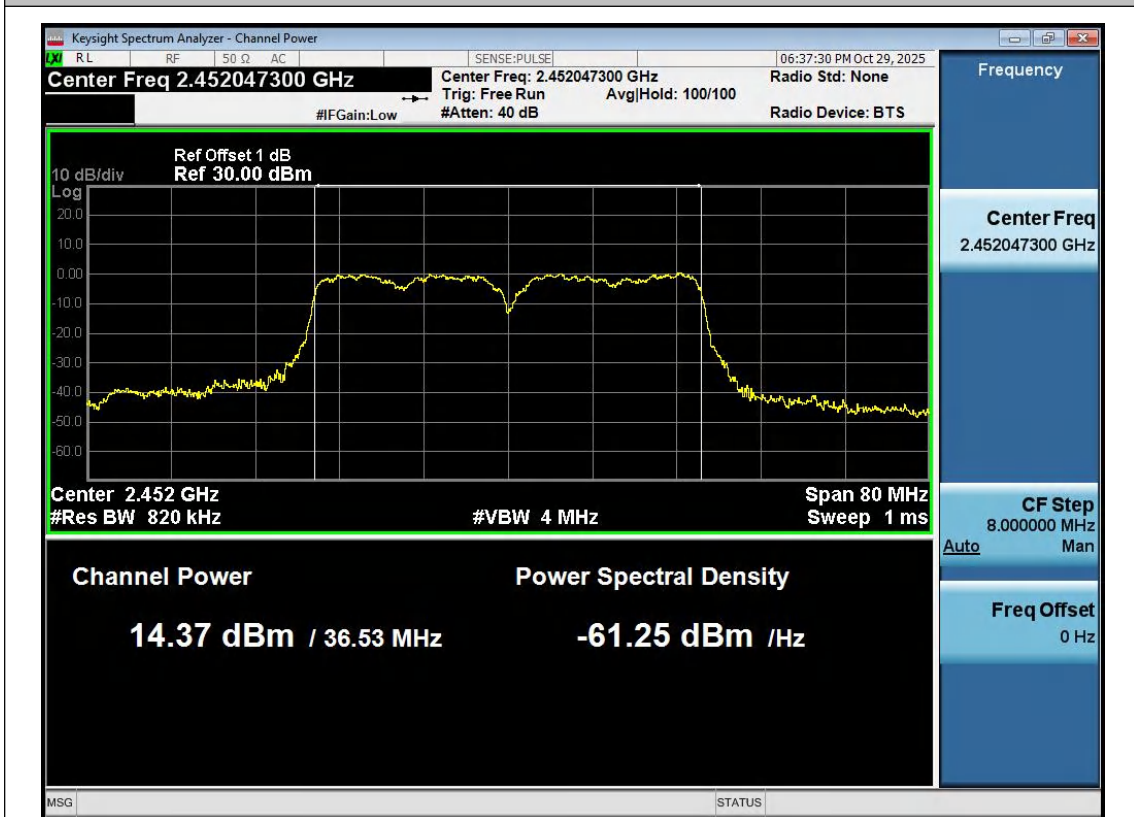
11N40SISO-Ant1-2452-PASS
