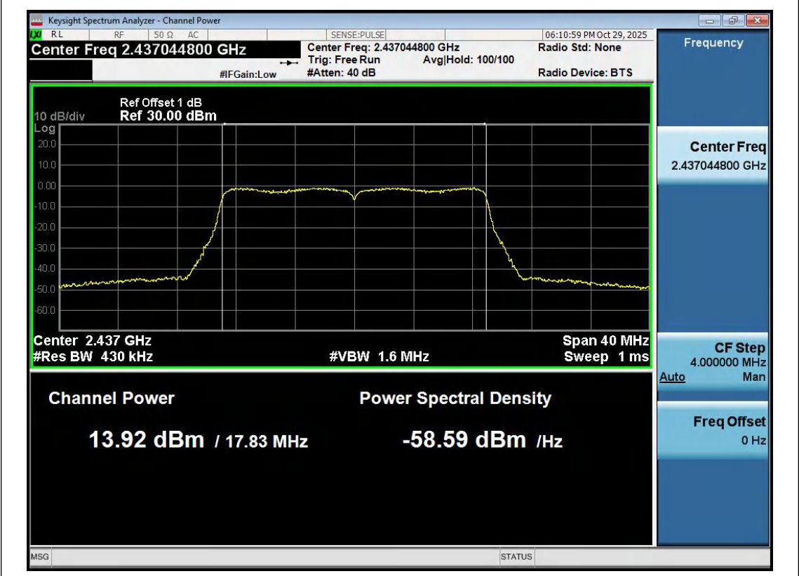
11N20SISO-Ant1-2437-PASS
