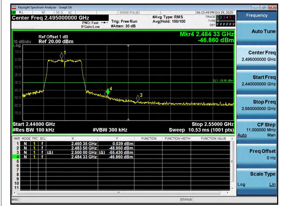
11N20SISO-Ant1-2462-PASS
