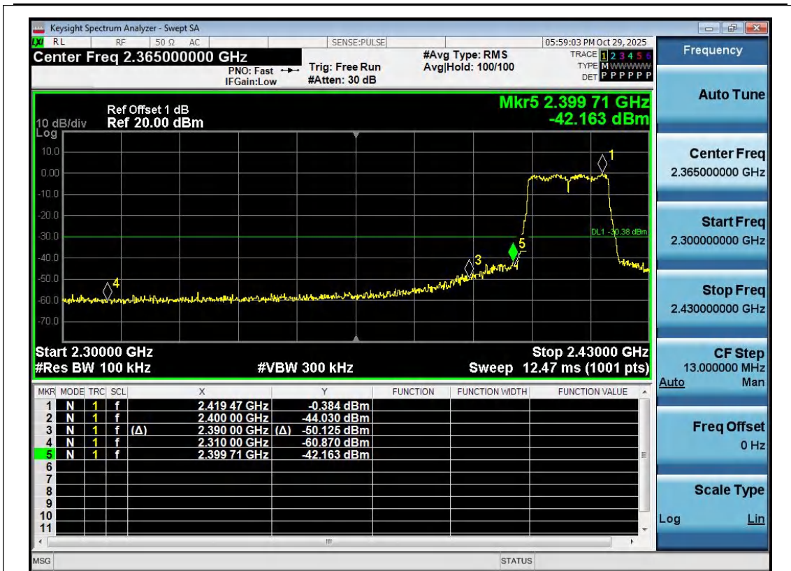
11N20SISO-Ant1-2412-PASS
