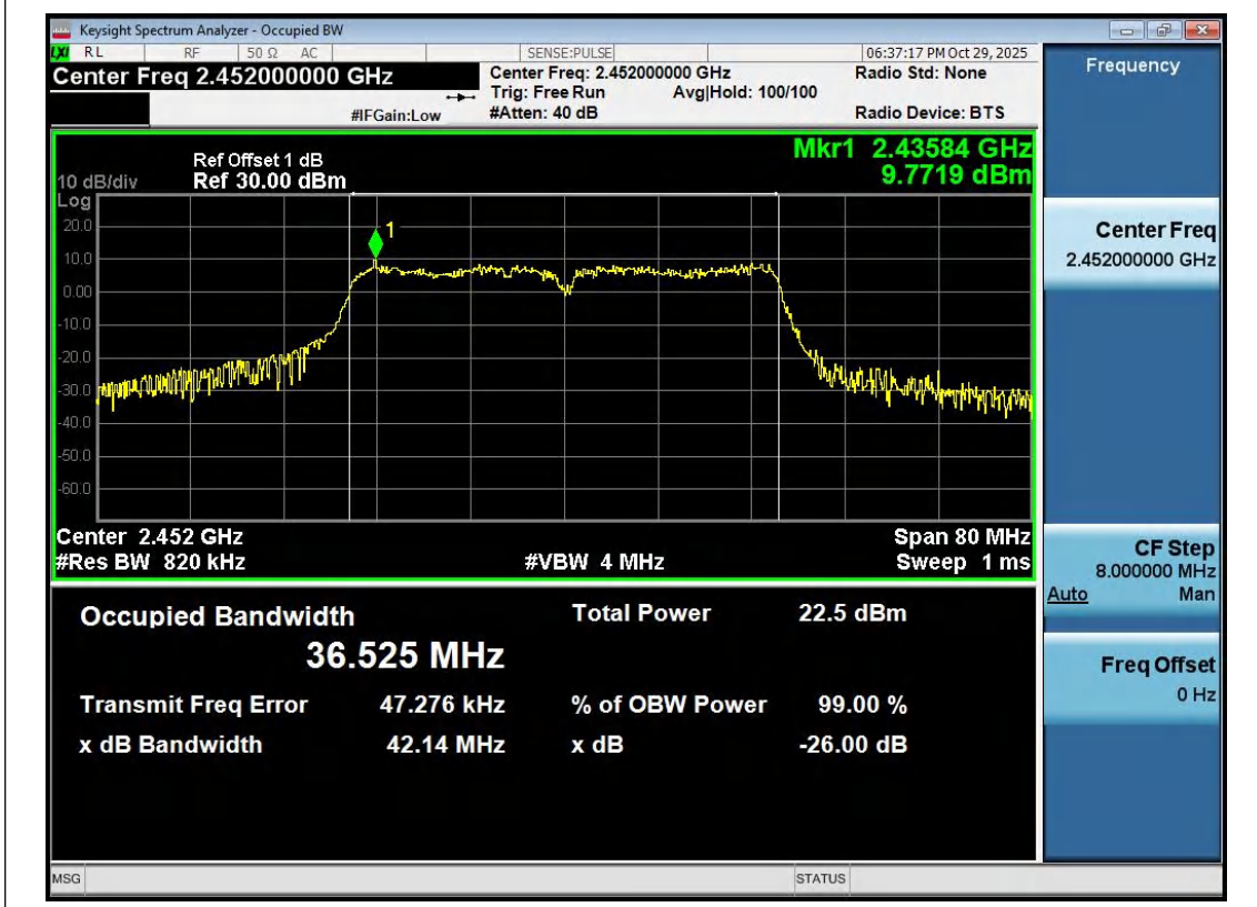
11N40SISO-Ant1-2452
