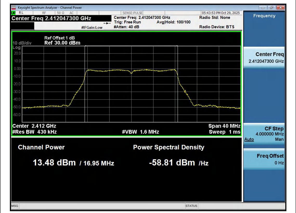
11G-Ant1-2412-PASS
