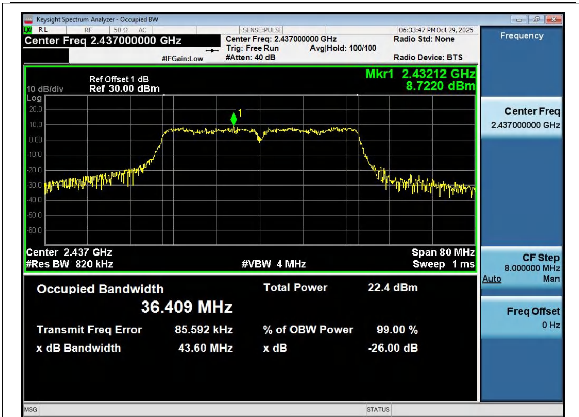
11N40SISO-Ant1-2437
