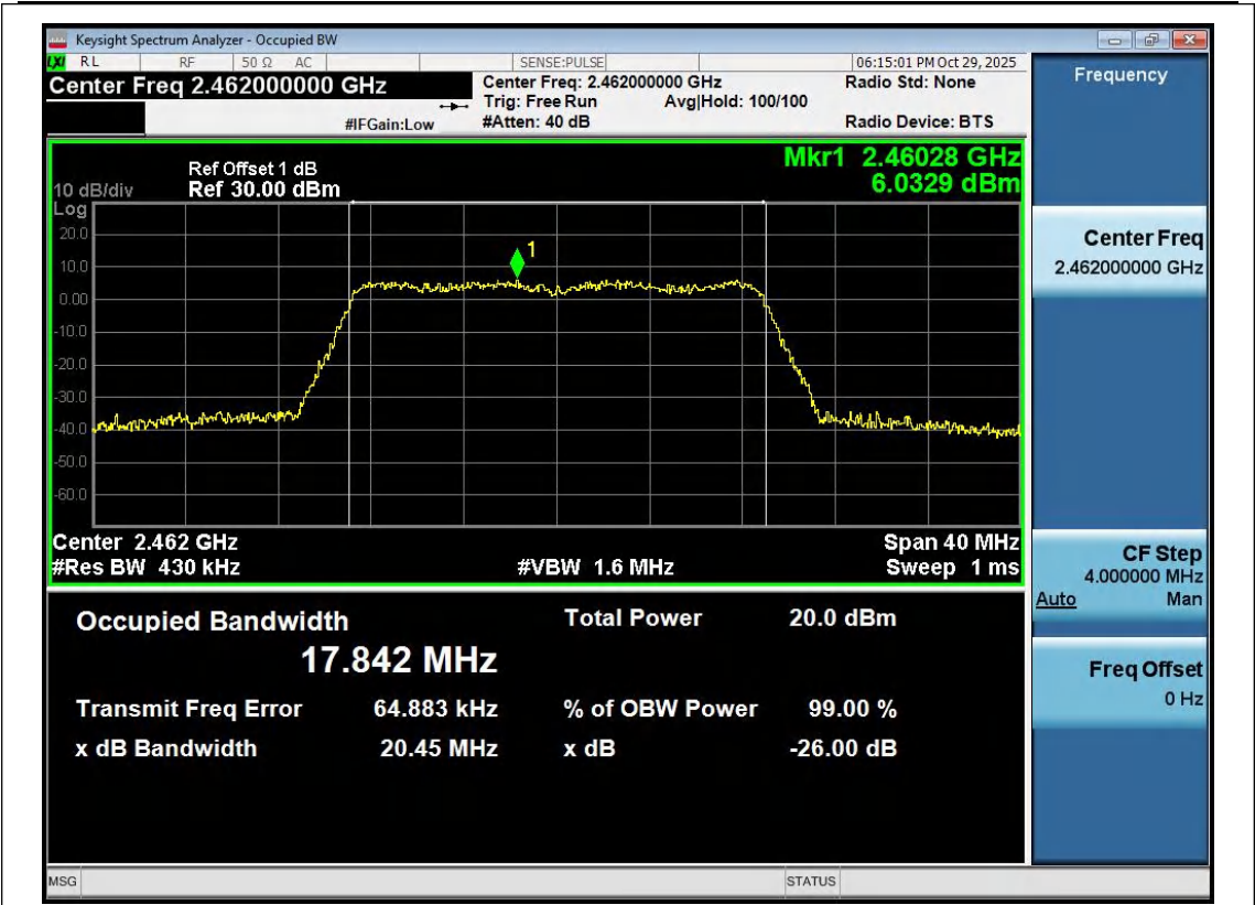
11N20SISO-Ant1-2462
