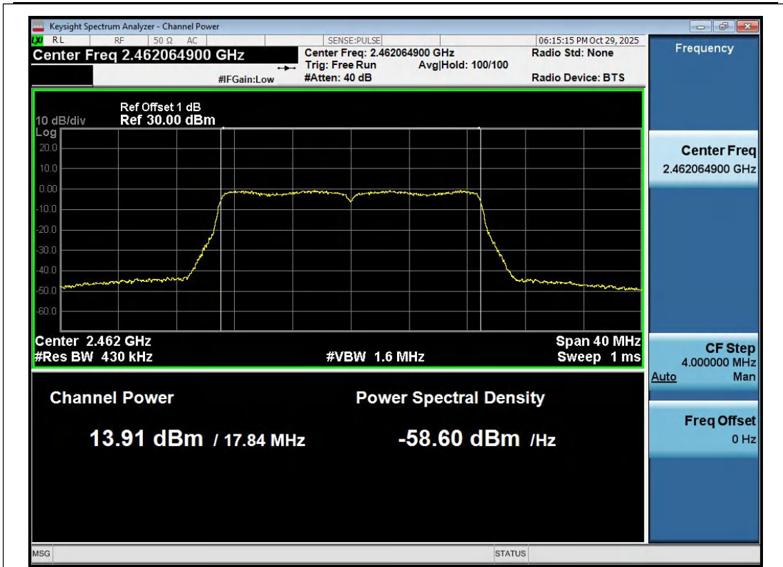
11N20SISO-Ant1-2462-PASS
