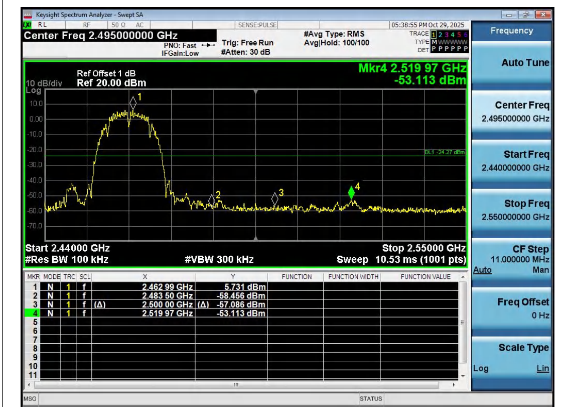
11B-Ant1-2462-PASS
