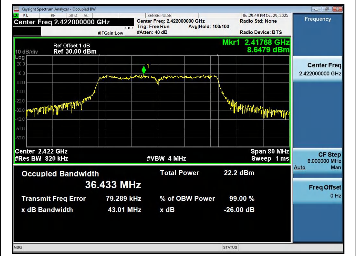
11N40SISO-Ant1-2422
