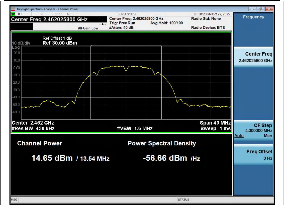
11B-Ant1-2462-PASS
