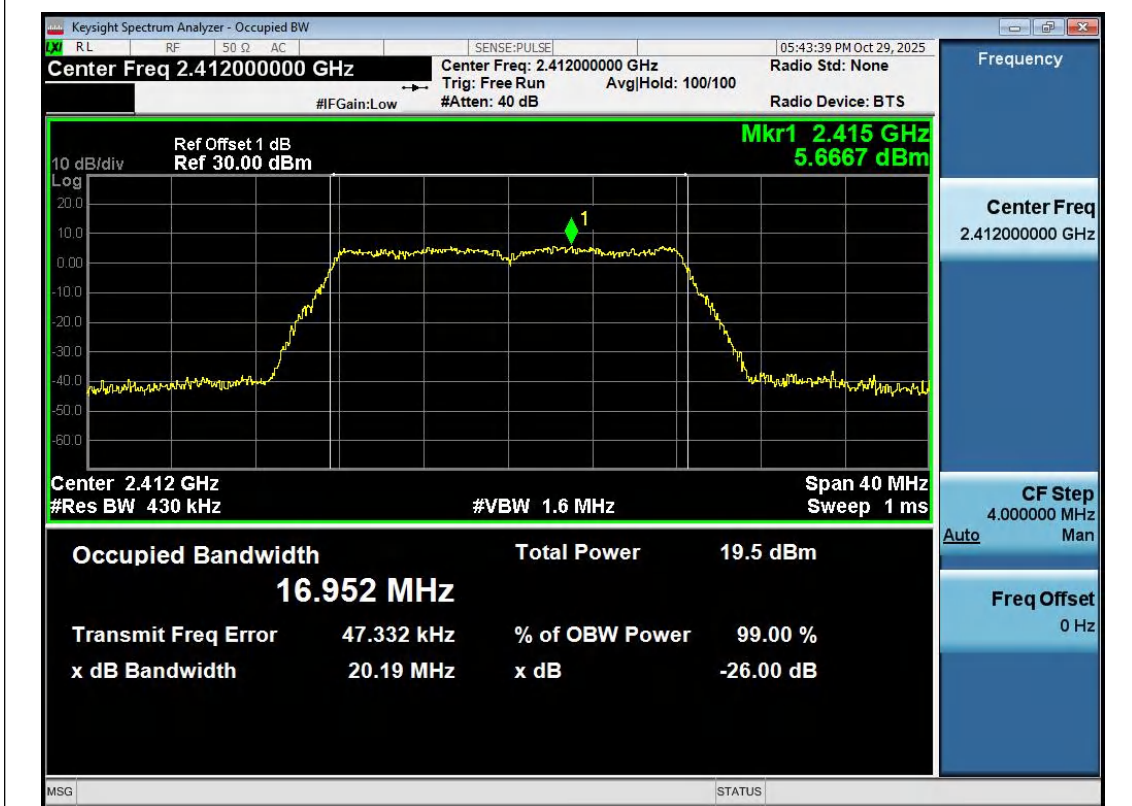
11G-Ant1-2412
