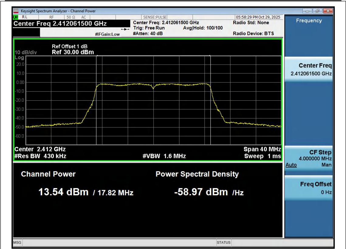
11N20SISO-Ant1-2412-PASS
