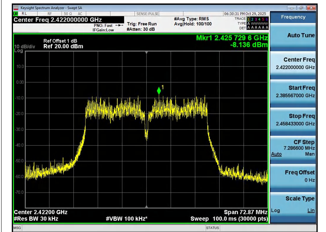
11N40SISO-Ant1-2422-PASS
