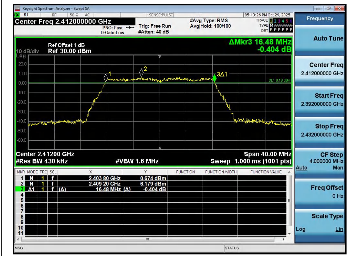
11G-Ant1-2412-PASS
