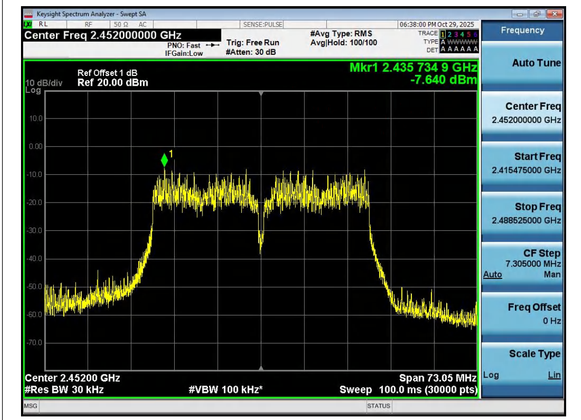
11N40SISO-Ant1-2452-PASS
