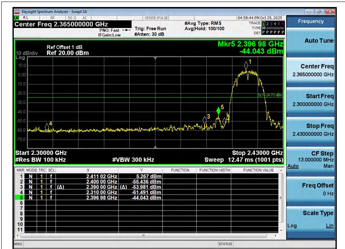
11B-Ant1-2412-PASS
