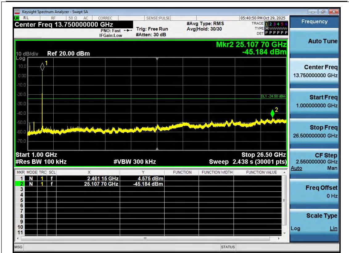
11B-Ant1-2462-1000~26500-PASS
