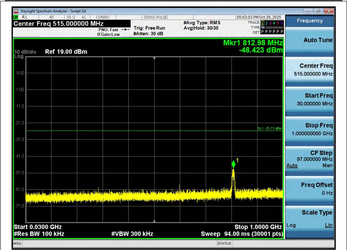
11B-Ant1-2437-30~1000-PASS
