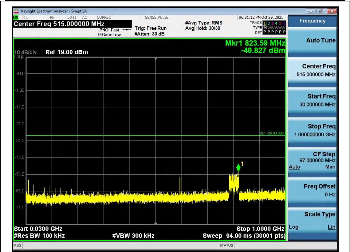
11N40SISO-Ant1-2422-30~1000-PASS
