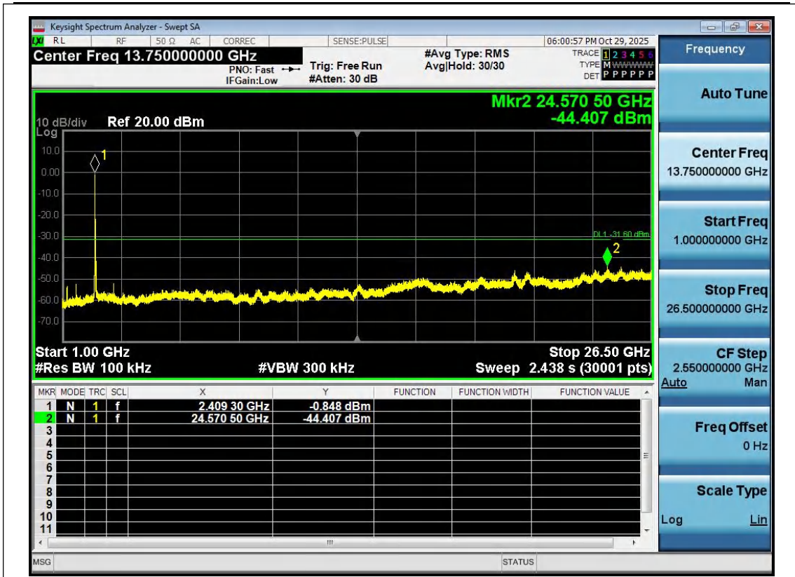
11N20SISO-Ant1-2412-1000~26500-PASS
