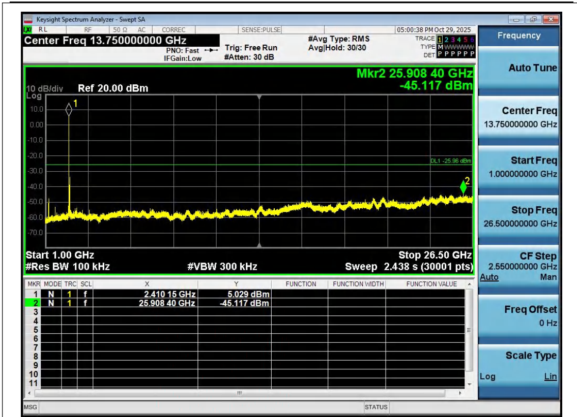
11B-Ant1-2412-1000~26500-PASS
