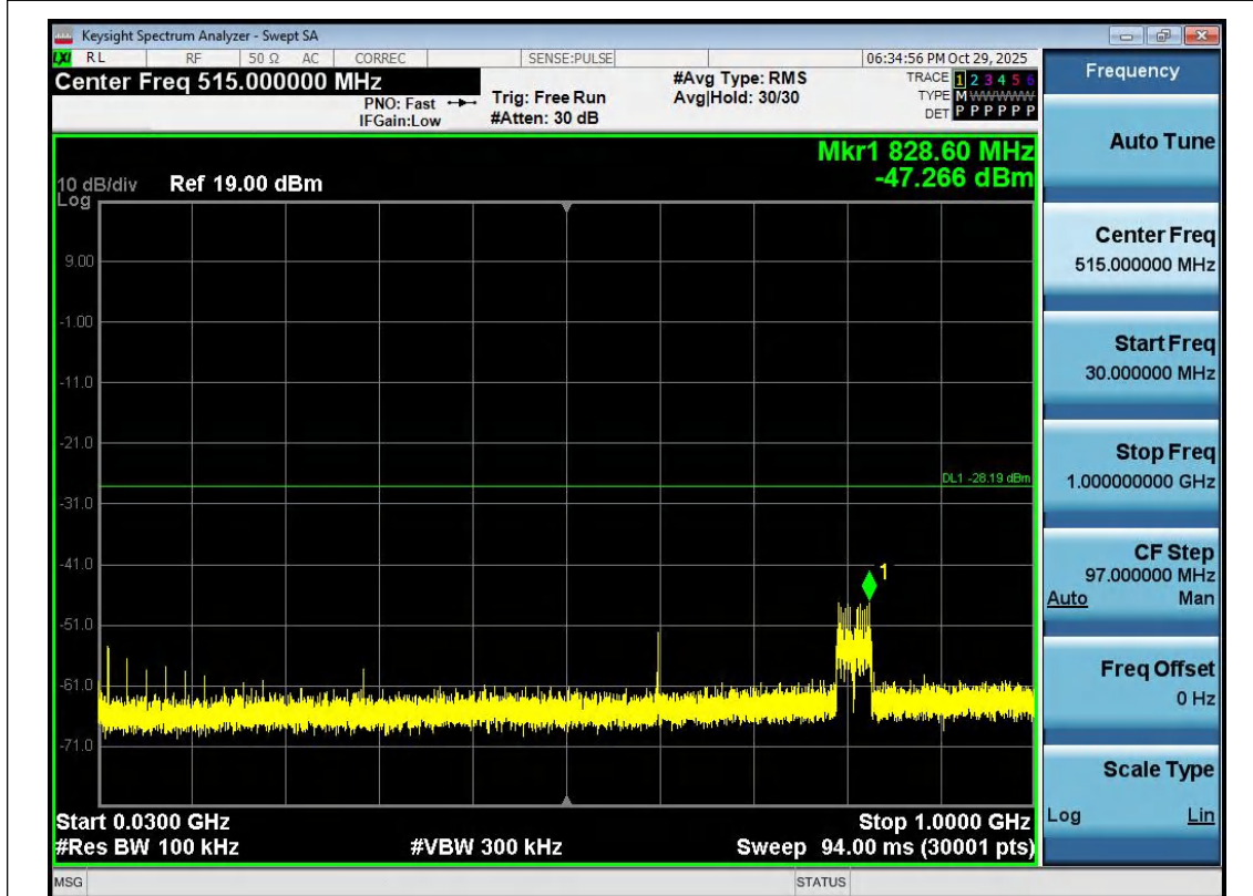
11N40SISO-Ant1-2437-30~1000-PASS
