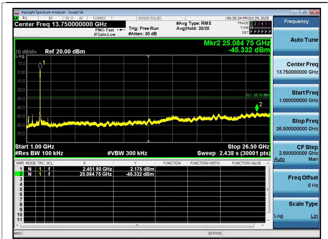
11N40SISO-Ant1-2437-1000~26500-PASS
