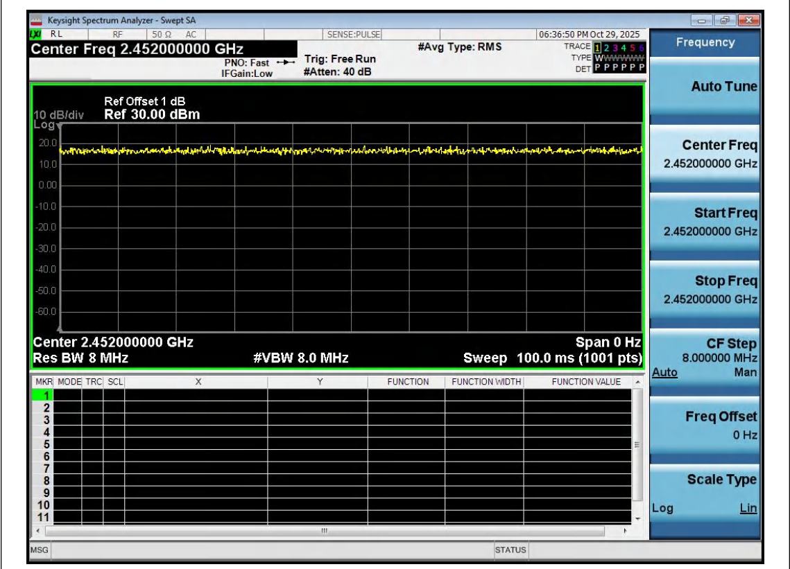
NTNV-11N40SISO-Ant1-2452
