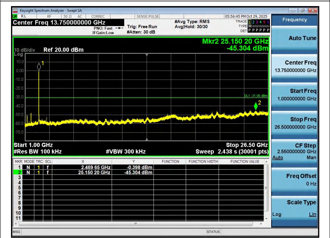
11G-Ant1-2462-1000~26500-PASS
