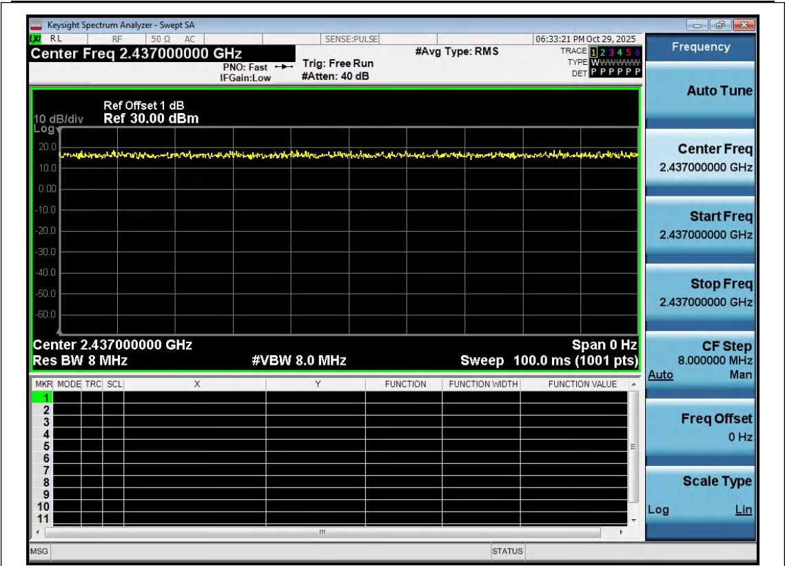
NTNV-11N40SISO-Ant1-2437
