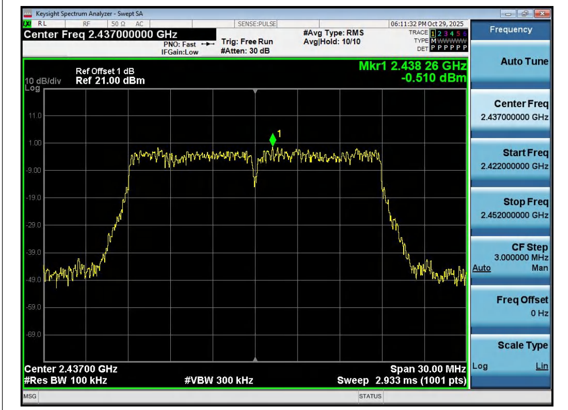
11N20SISO-Ant1-2437-0~Reference-PASS
