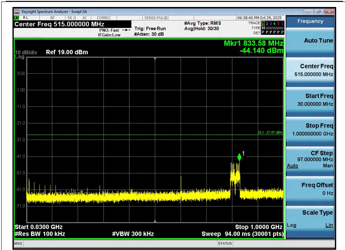
11N40SISO-Ant1-2452-30~1000-PASS
