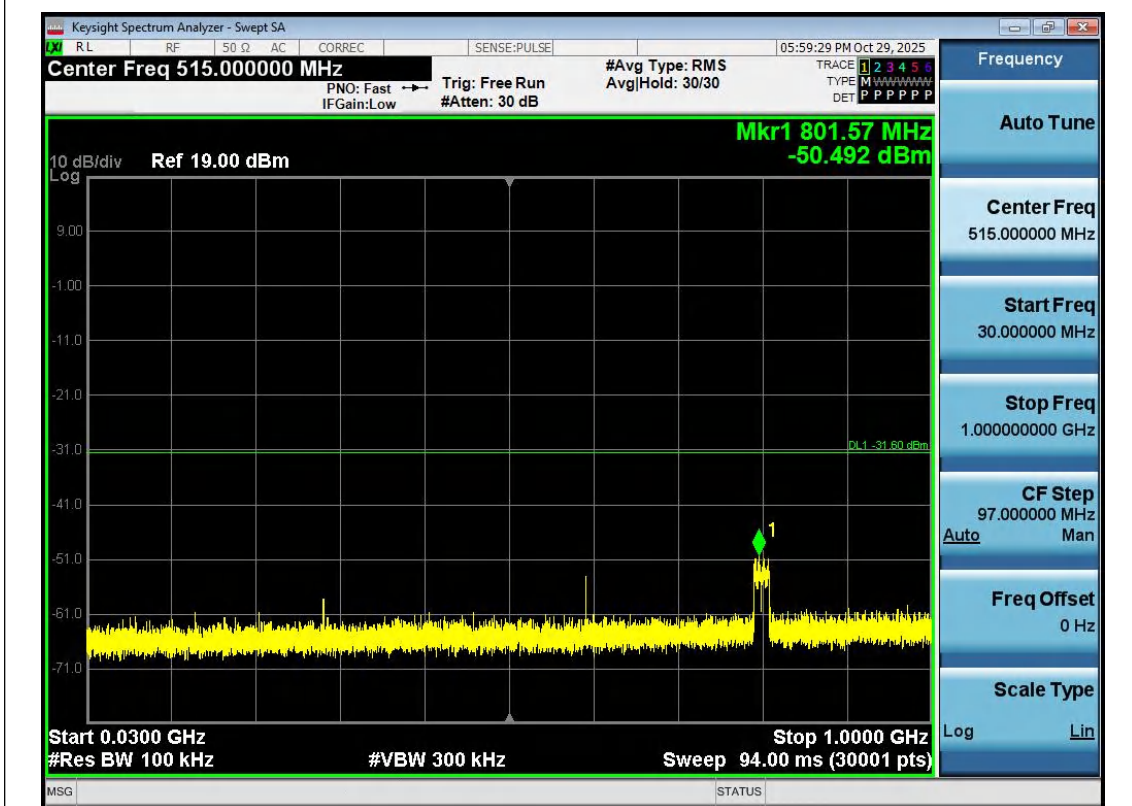
11N20SISO-Ant1-2412-30~1000-PASS
