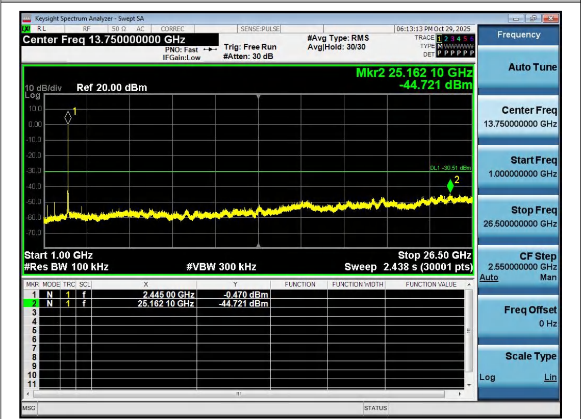
11N20SISO-Ant1-2437-1000~26500-PASS
