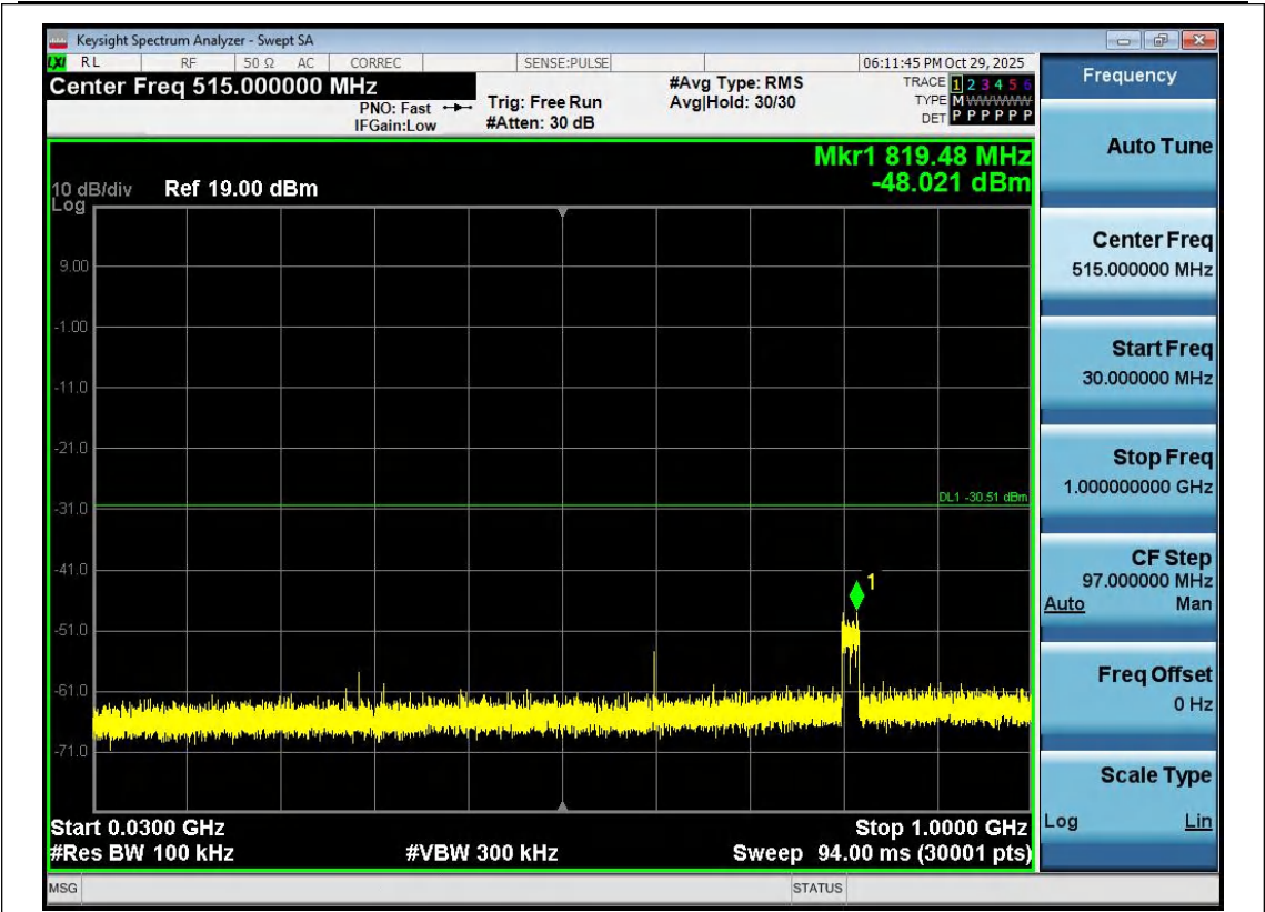
11N20SISO-Ant1-2437-30~1000-PASS
