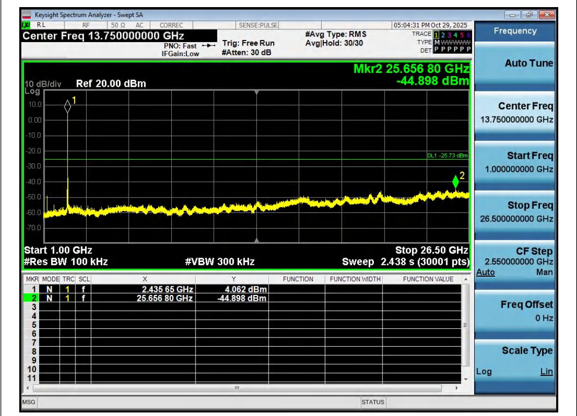
11B-Ant1-2437-1000~26500-PASS
