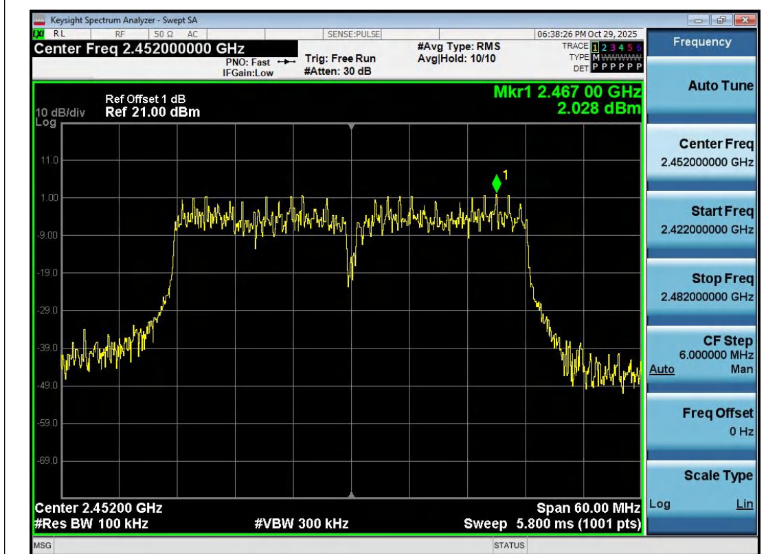
11N40SISO-Ant1-2452-0~Reference-PASS
