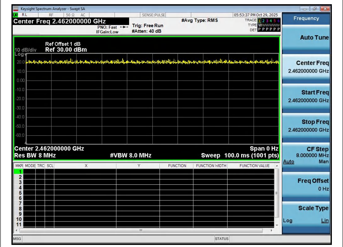
NTNV-11G-Ant1-2462
