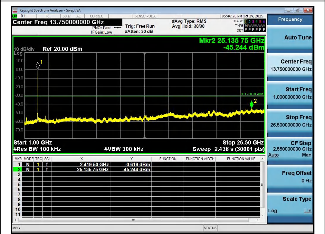
11G-Ant1-2412-1000~26500-PASS
