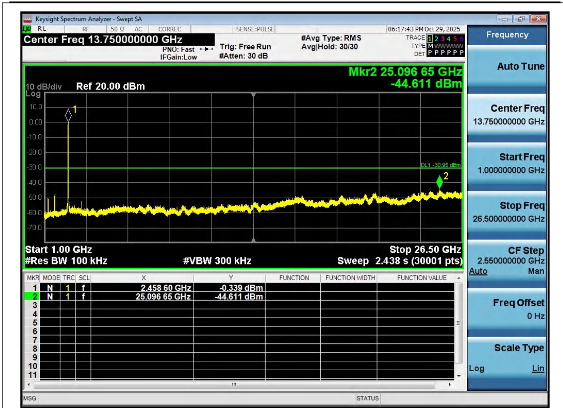
11N20SISO-Ant1-2462-1000~26500-PASS
