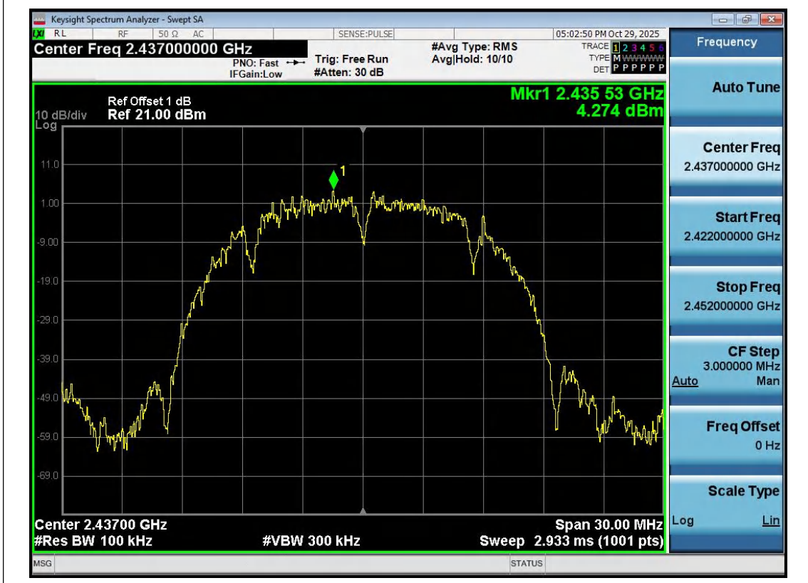
11B-Ant1-2437-0~Reference-PASS
