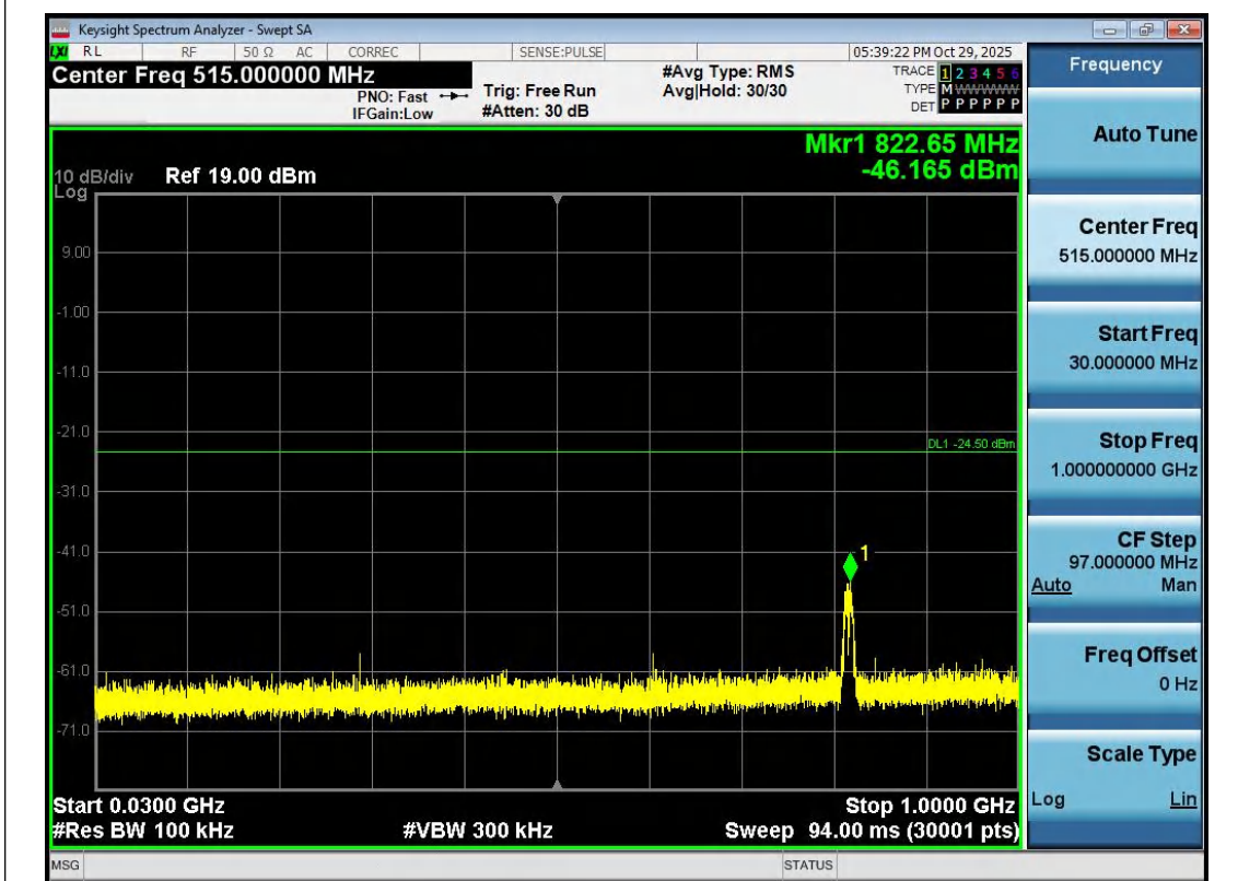
11B-Ant1-2462-30~1000-PASS
