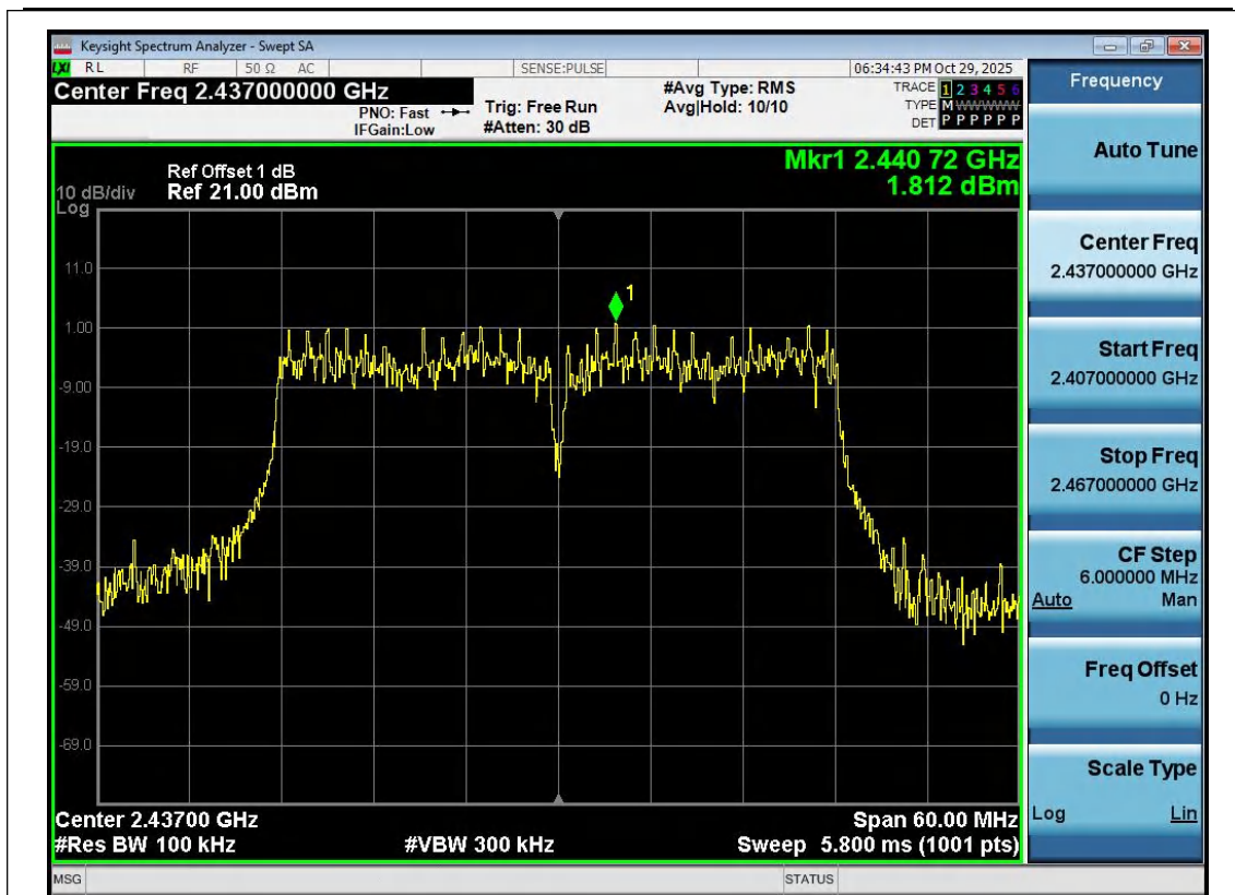
11N40SISO-Ant1-2437-0~Reference-PASS
