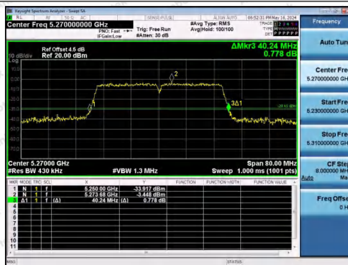
11AC40MIMO-Ant2-5270
