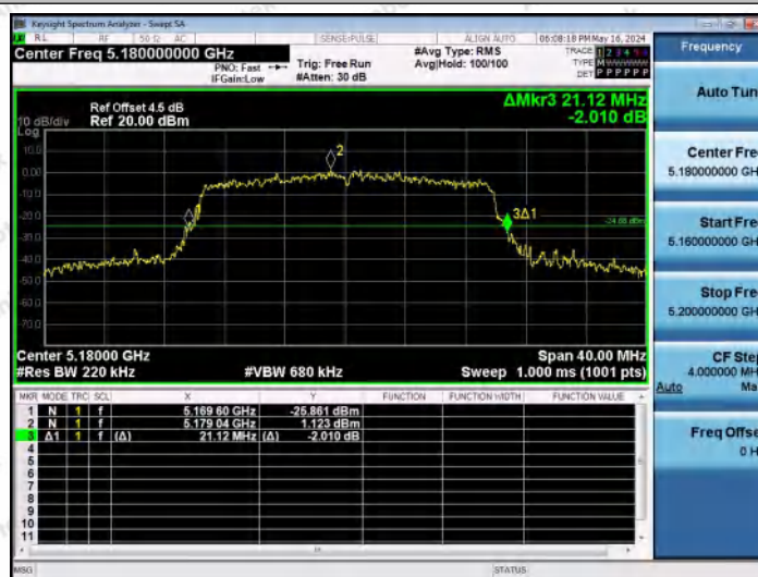
11AX20MIMO-Ant2-5180
