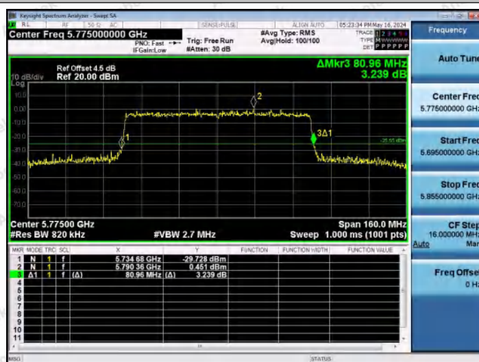
11AX80MIMO-Ant2-5775
