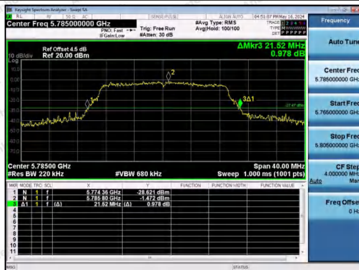
11AC20MIMO-Ant2-5785
