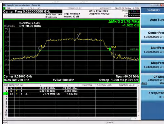
11N20MIMO-Ant2-5320
