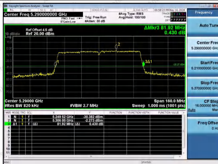
11AC80MIMO-Ant2-5290
