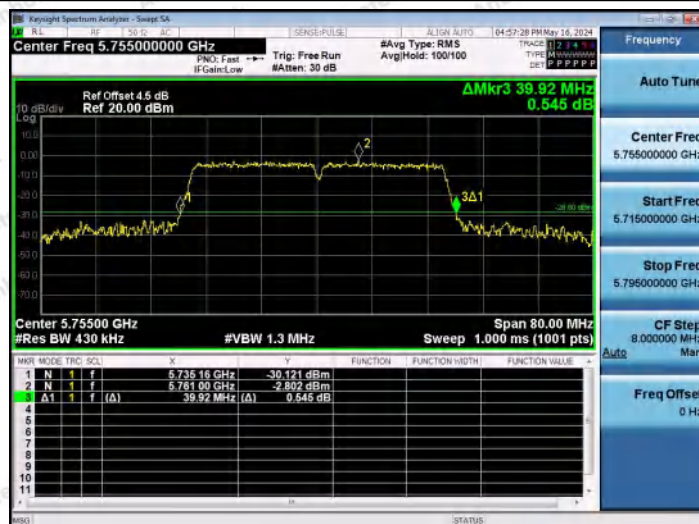
11AC40MIMO-Ant2-5755
