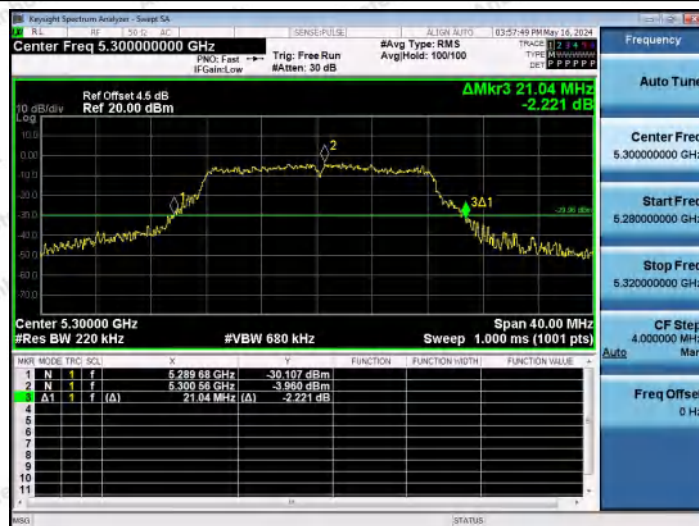
11A-Ant2-5300
