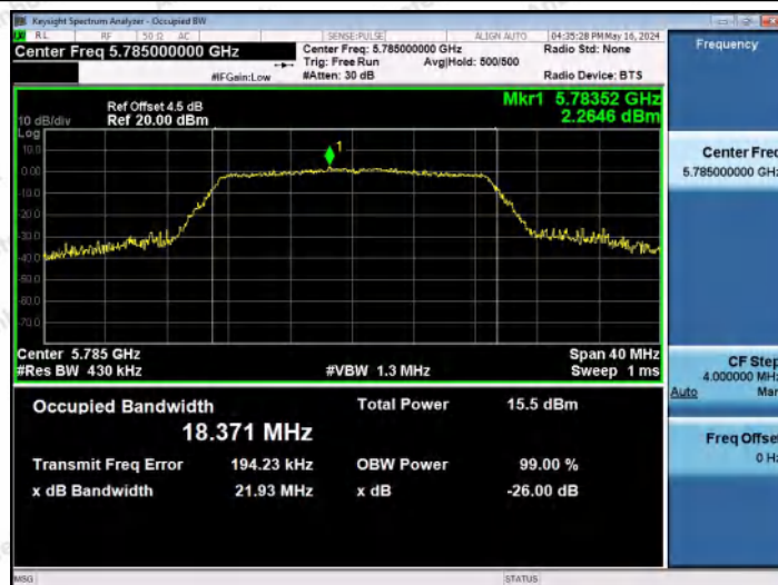
11N20MIMO-Ant2-5785
