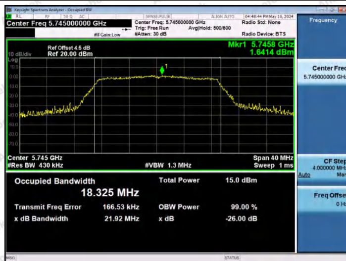
11AC20MIMO-Ant2-5745
