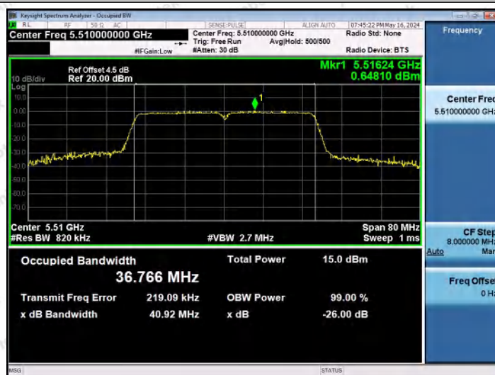
11AC40MIMO-Ant1-5510
