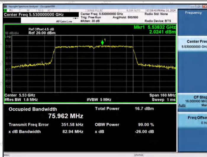
11AC80MIMO-Ant2-5530
