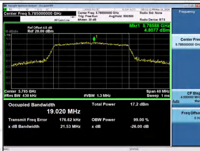
11AX20MIMO-Ant2-5785
