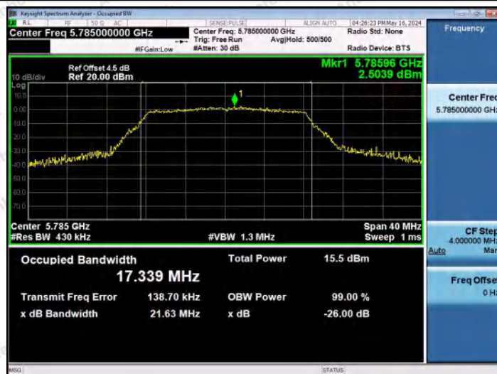
11A-Ant2-5785
