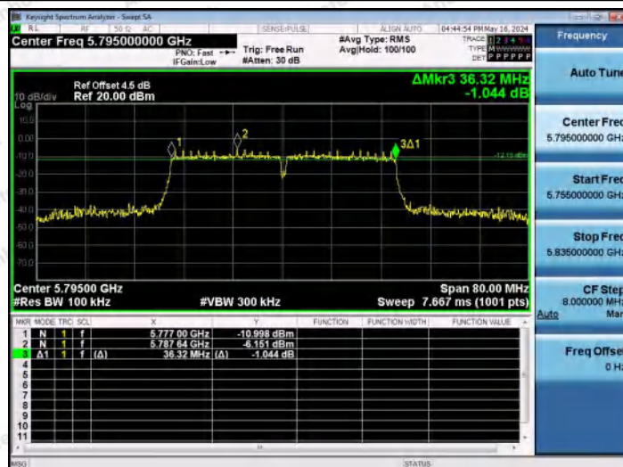
11N40MIMO-Ant2-5795-PASS
