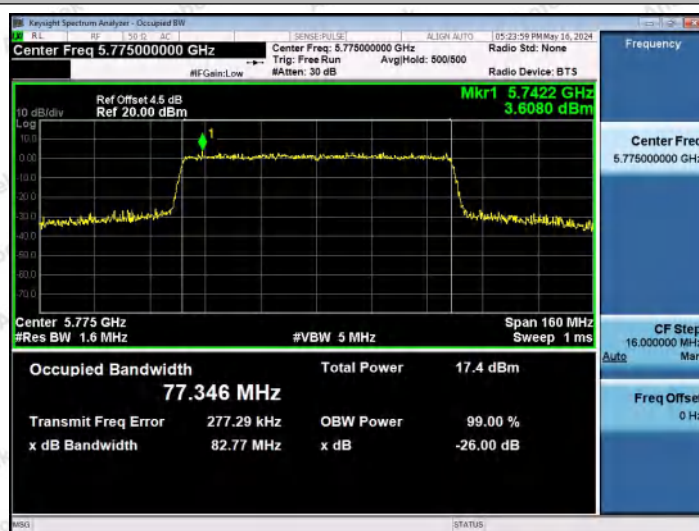
11AX80MIMO-Ant2-5775
