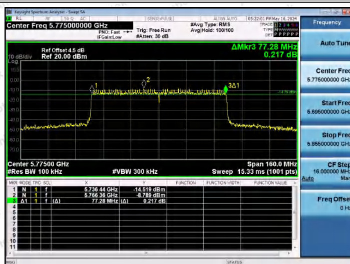
11AX80MIMO-Ant1-5775-PASS
