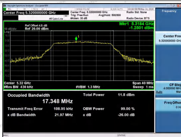
11A-Ant2-5320
