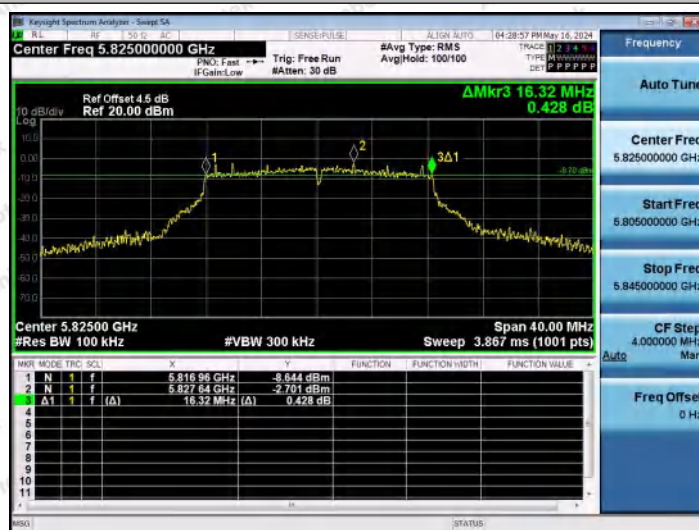
11A-Ant2-5825-PASS
