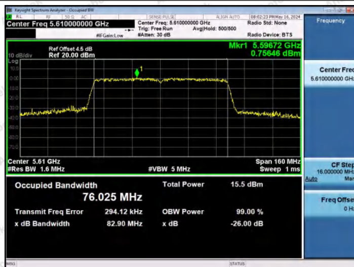
11AC80MIMO-Ant2-5610
