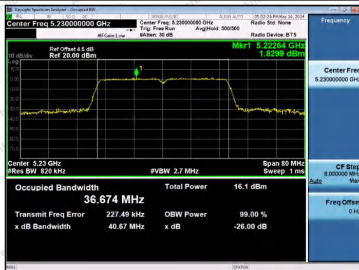
11AC40MIMO-Ant2-5230
