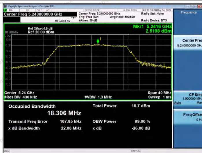
11N20MIMO-Ant2-5240
