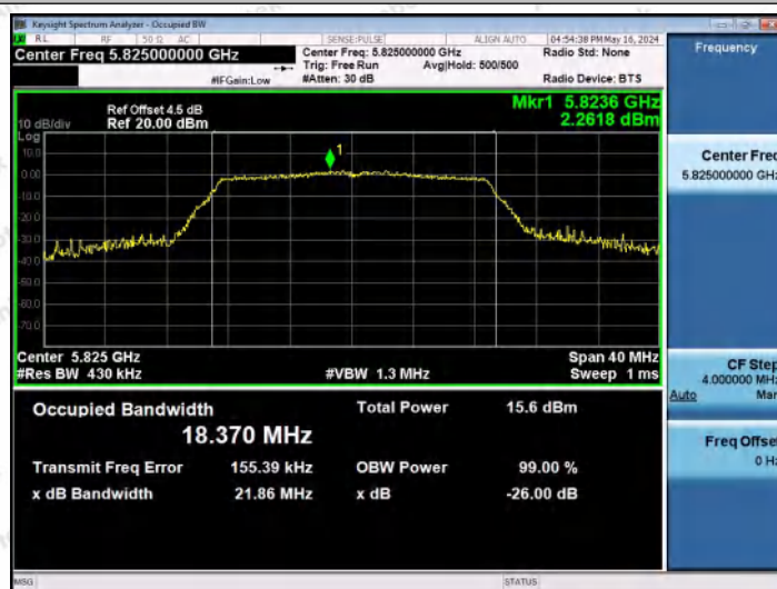
11AC20MIMO-Ant2-5825
