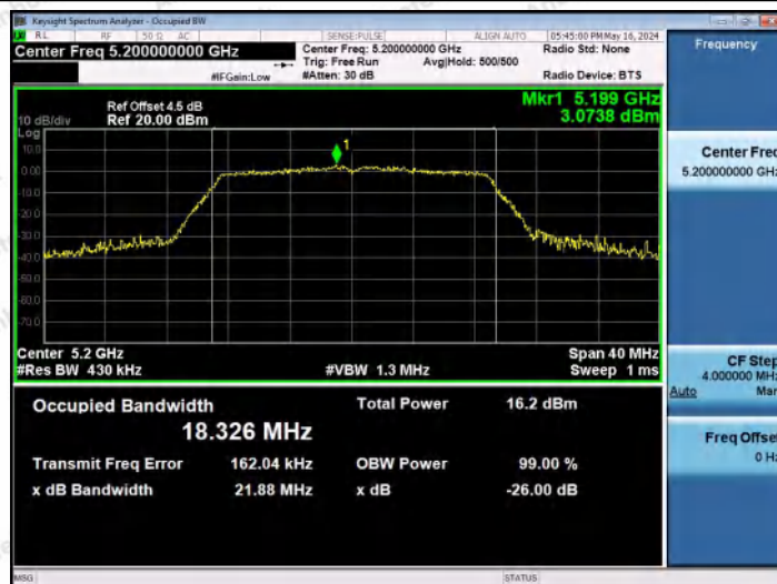
11AC20MIMO-Ant2-5200
