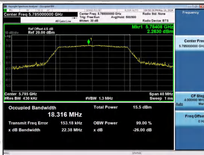
11AC20MIMO-Ant1-5785
