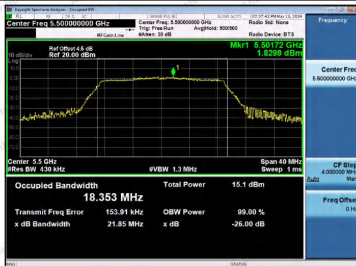
11AC20MIMO-Ant1-5500
