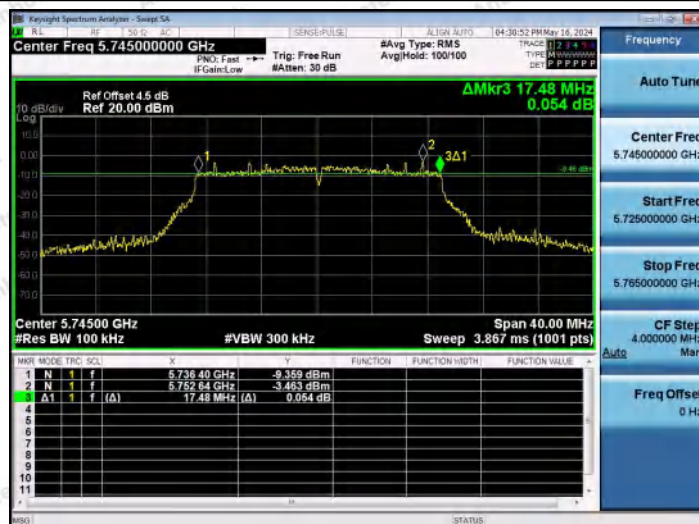
11N20MIMO-Ant1-5745-PASS
