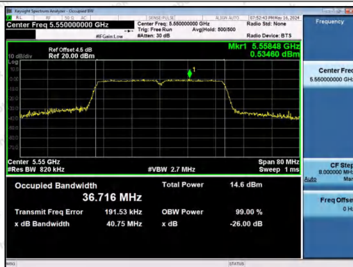
11AC40MIMO-Ant2-5550
