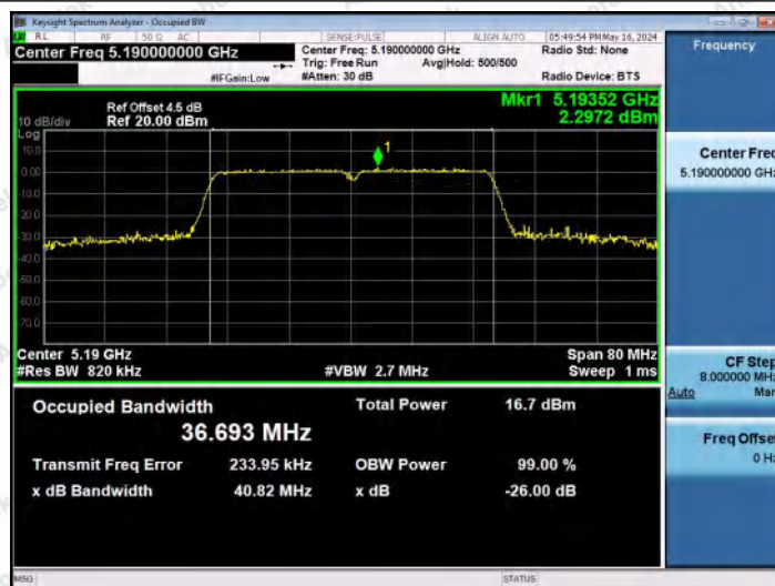
11AC40MIMO-Ant2-5190
