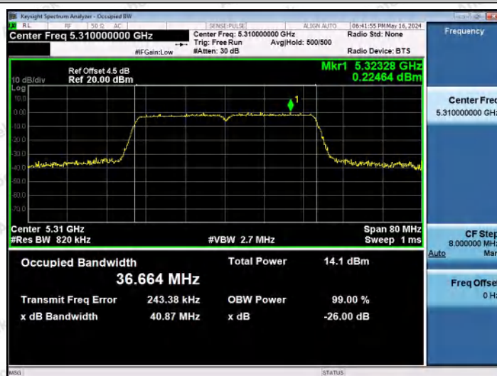
11N40MIMO-Ant2-5310
