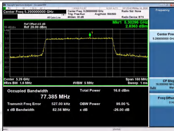
11AX80MIMO-Ant2-5290
