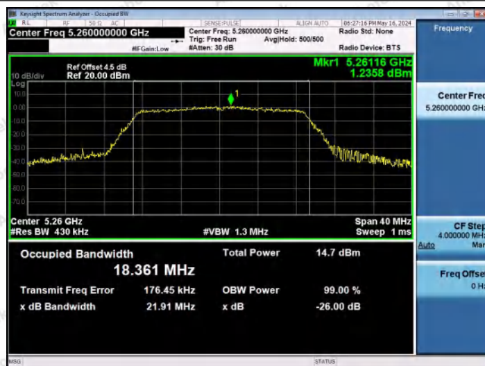
11N20MIMO-Ant2-5260
