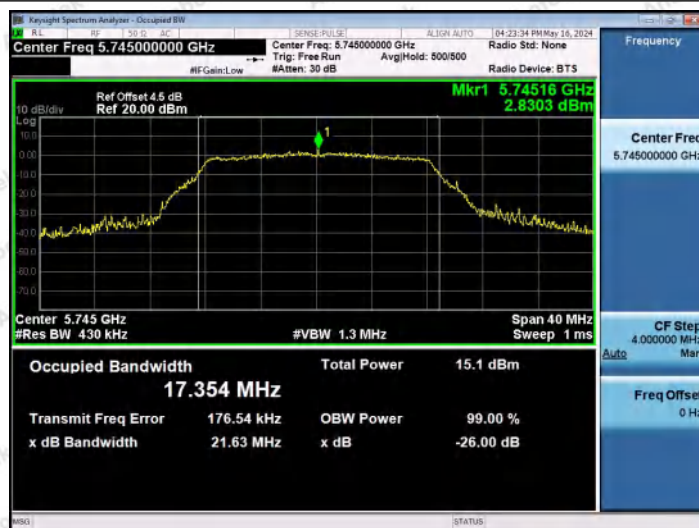
11A-Ant2-5745
