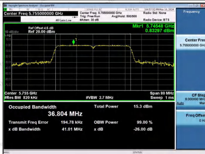
11AC40MIMO-Ant2-5755
