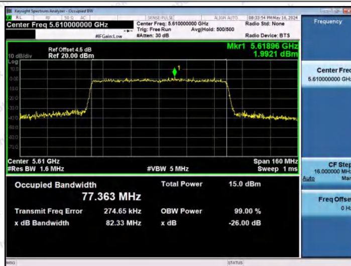
11AX80MIMO-Ant2-5610
