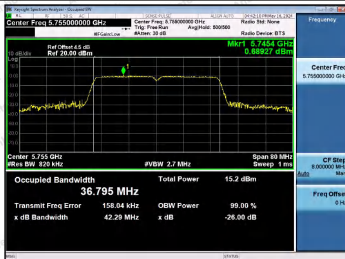
11N40MIMO-Ant2-5755
