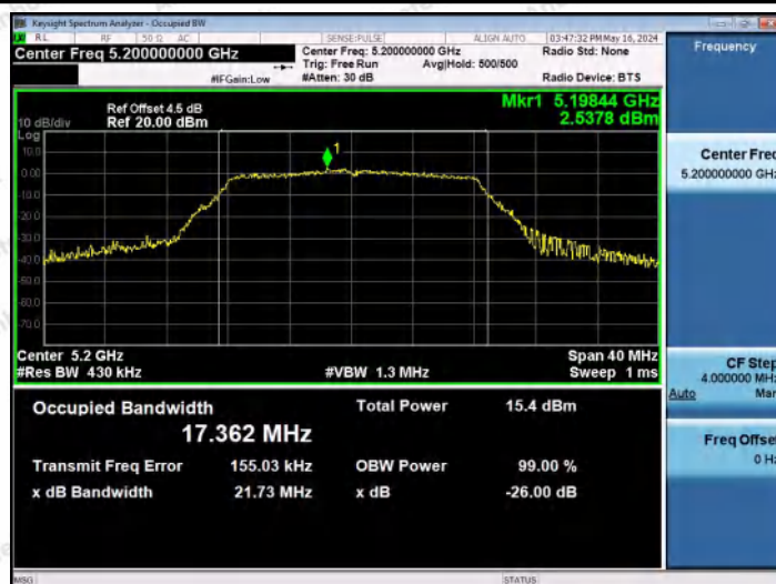
11A-Ant2-5200
