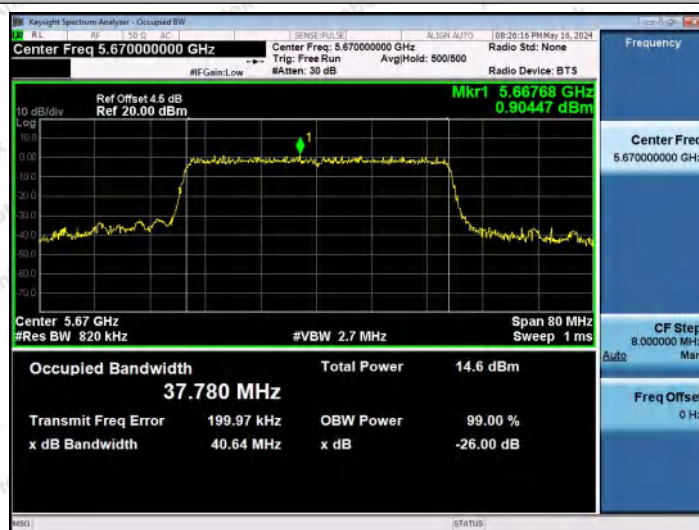
11AX40MIMO-Ant2-5670
