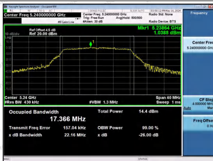
11A-Ant2-5240
