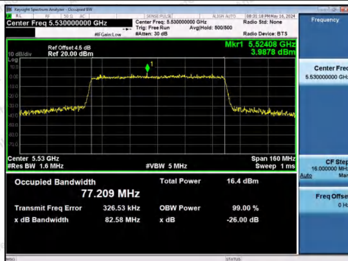
11AX80MIMO-Ant2-5530
