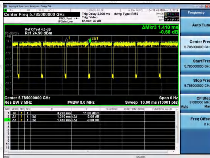
NTNV-11AC20MIMO-Ant2-5785
