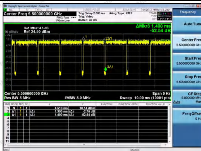
NTVN-11N20MIMO-Ant1-5500
