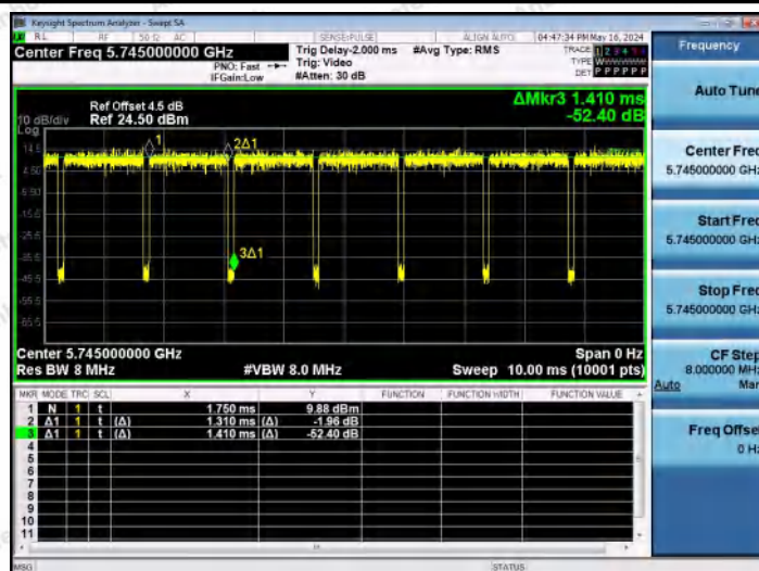
NTNV-11AC20MIMO-Ant1-5745
