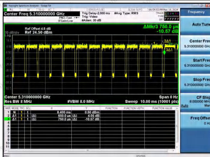
NTNV-11AC40MIMO-Ant1-5310
