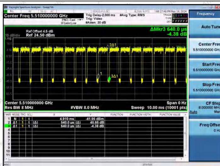
NTNV-11AX40MIMO-Ant2-5510
