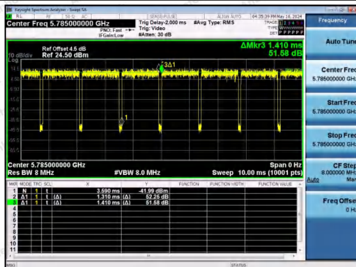
NTNV-11N20MIMO-Ant2-5785
