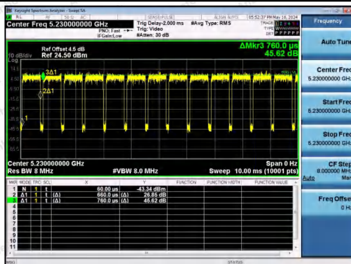
NTNV-11AC40MIMO-Ant2-5230
