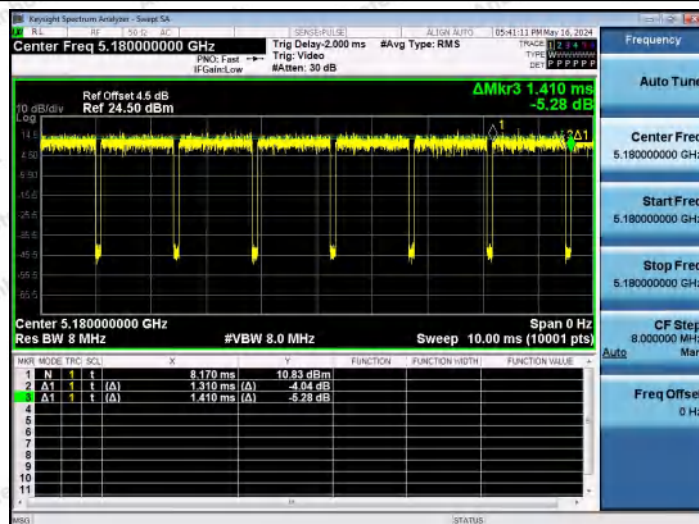
NTNV-11AC20MIMO-Ant1-5180
