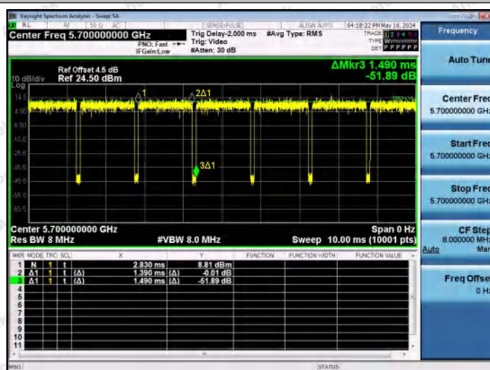
NTNV-11A-Ant1-5700
