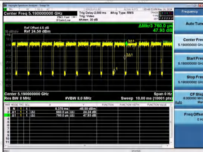
NTNV-11AC40MIMO-Ant1-5190
