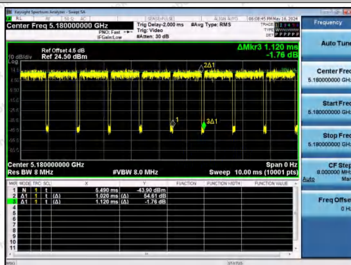
NTNV-11AX20MIMO-Ant2-5180
