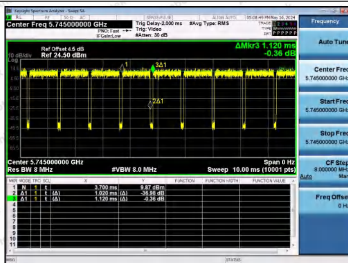
NTNV-11AX20MIMO-Ant2-5745
