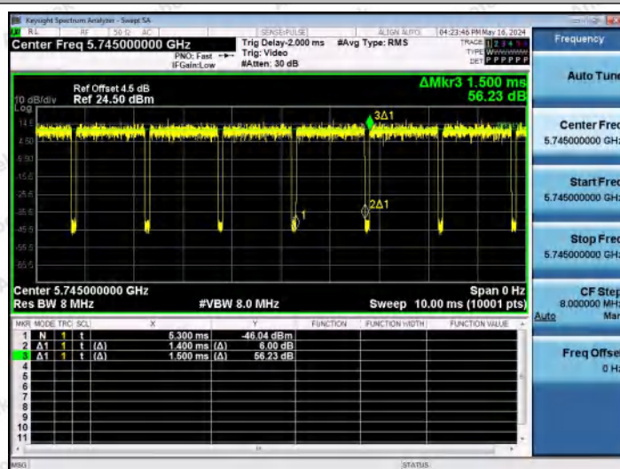
NTNV-11A-Ant2-5745
