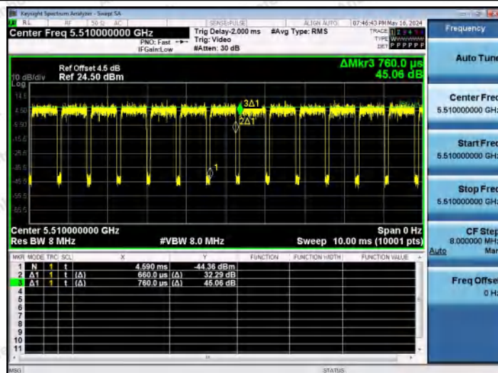
NTNV-11AC40MIMO-Ant2-5510
