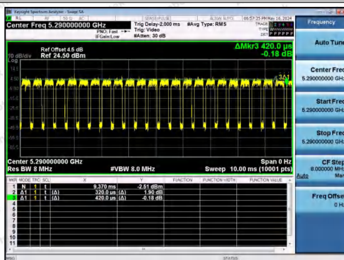
NTNV-11AC80MIMO-Ant1-5290
