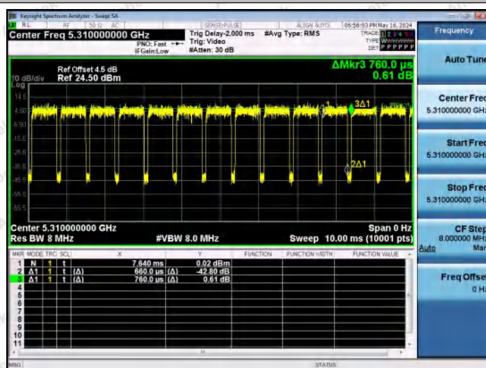
NTNV-11AC40MIMO-Ant2-5310
