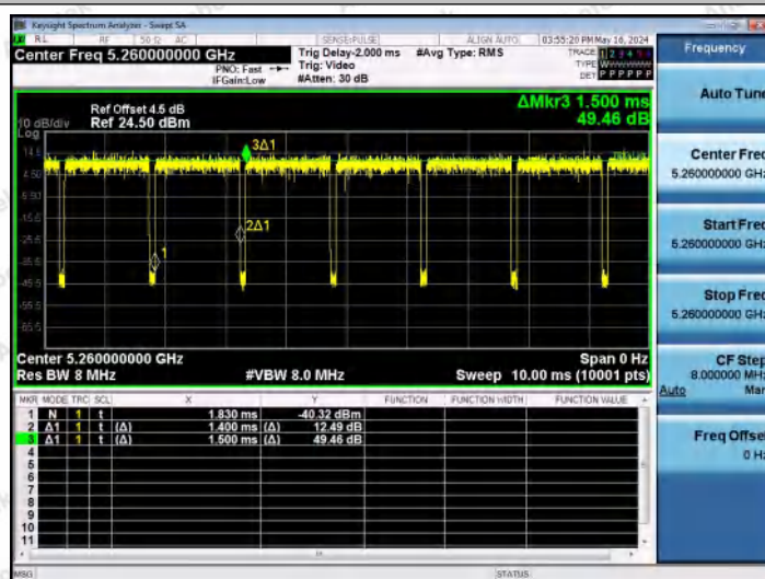
NTNV-11A-Ant2-5260
