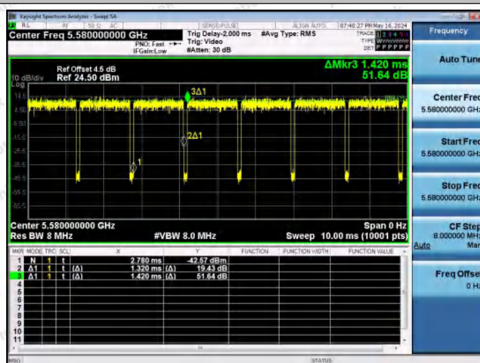
NTNV-11AC20MIMO-Ant1-5580
