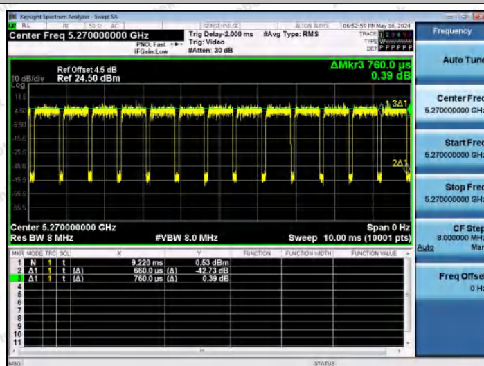
NTNV-11AC40MIMO-Ant2-5270
