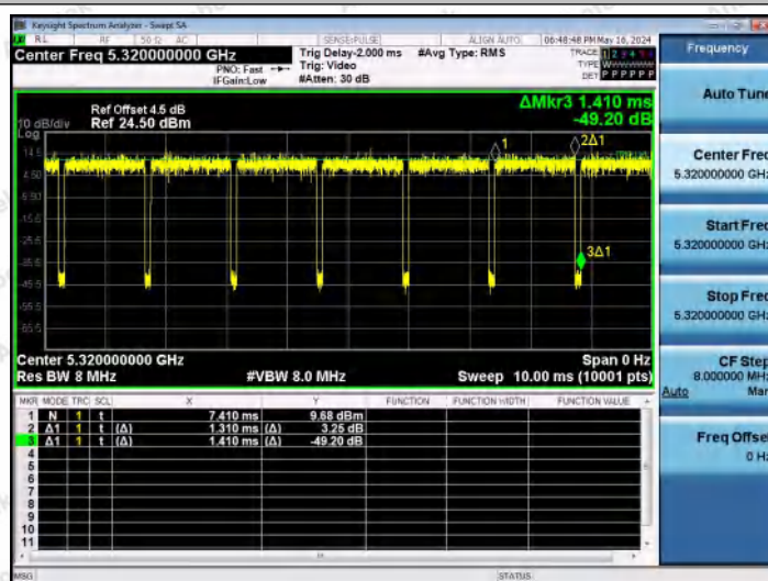
NTNV-11AC20MIMO-Ant1-5320
