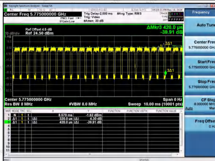
NTNV-11AC80MIMO-Ant2-5775
