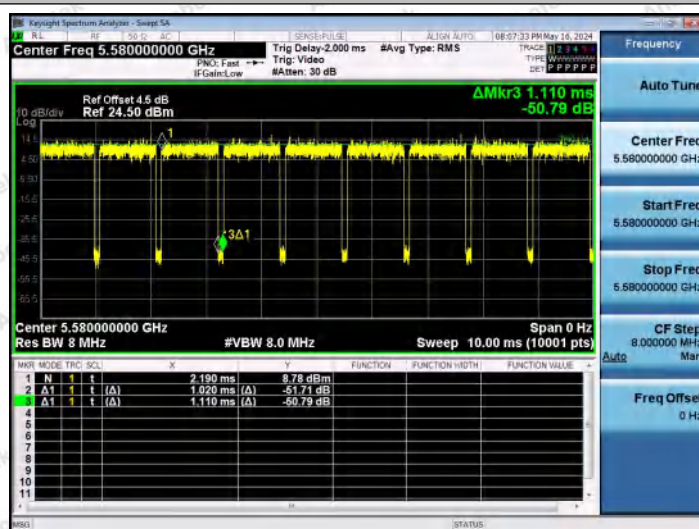
NTNV-11AX20MIMO-Ant2-5580
