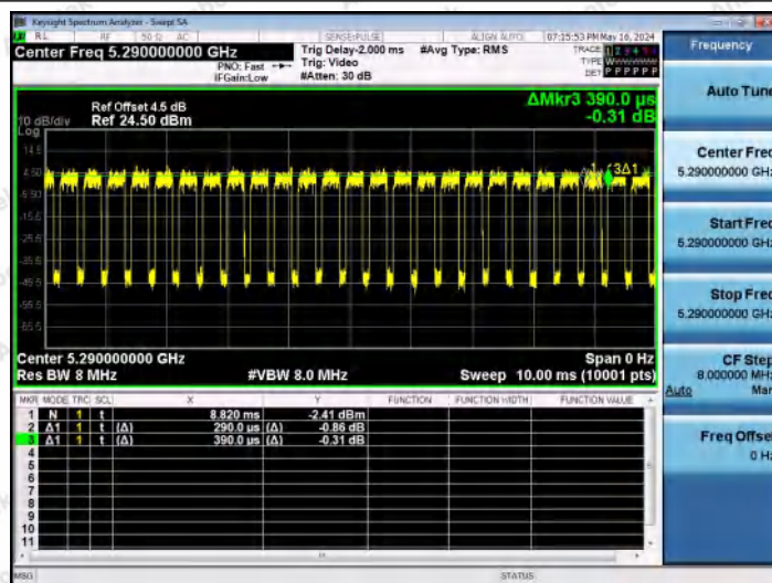
NTNV-11AX80MIMO-Ant2-5290
