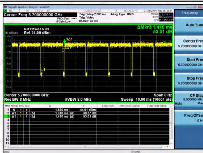
NTVN-11N20MIMO-Ant2-5700
