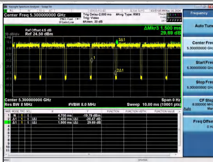
NTNV-11A-Ant1-5300
