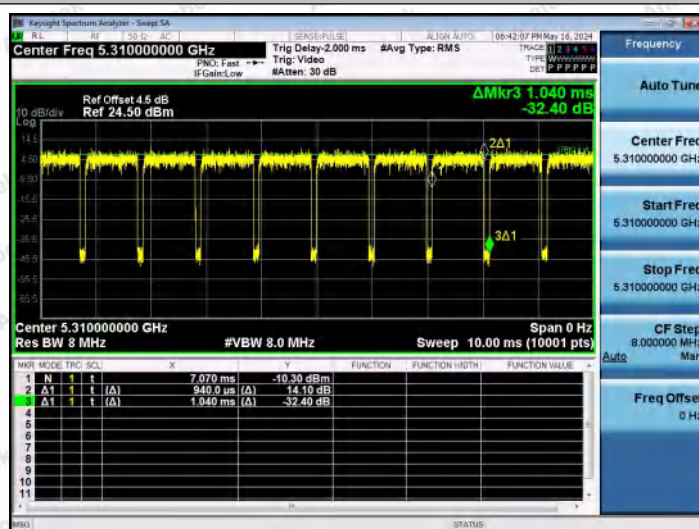
NTNV-11N40MIMO-Ant2-5310
