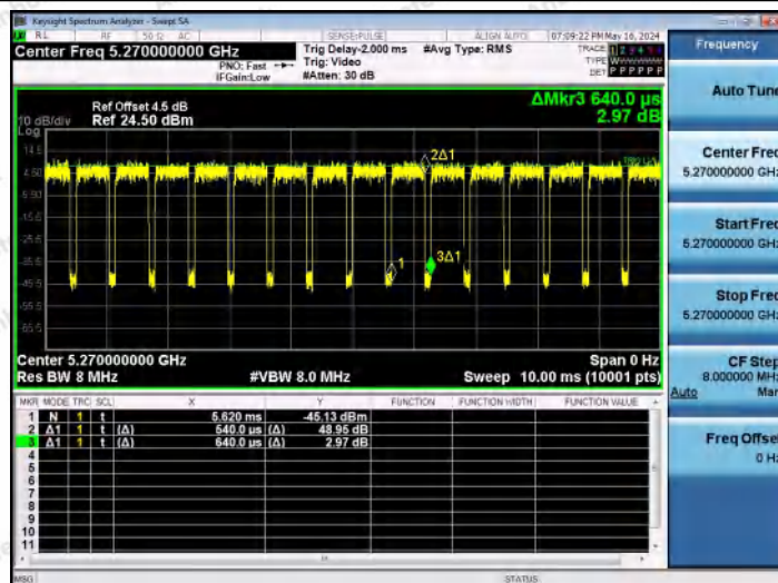
NTNV-11AX40MIMO-Ant2-5270
