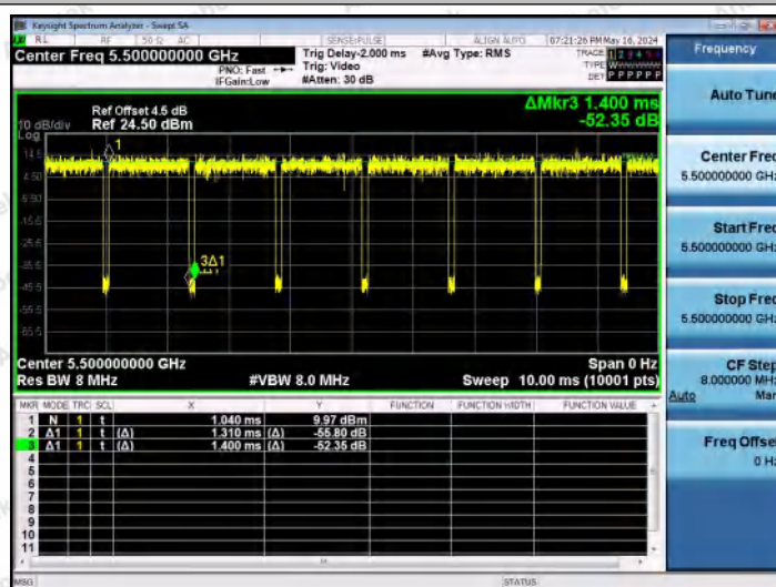
NTVN-11N20MIMO-Ant2-5500
