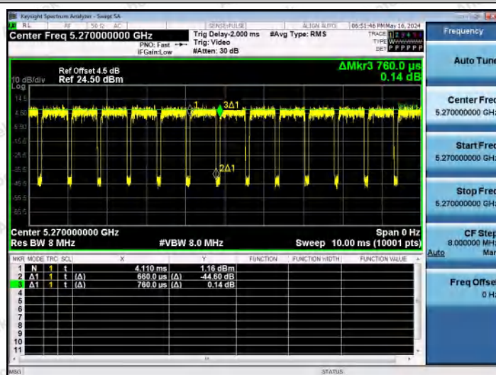
NTNV-11AC40MIMO-Ant1-5270
