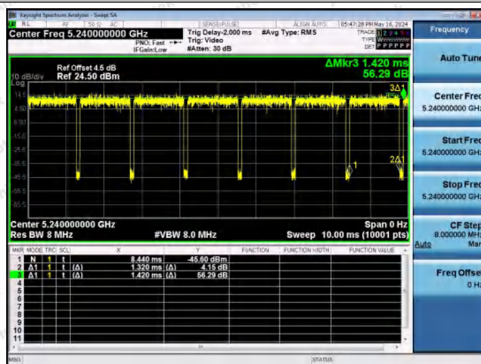
NTNV-11AC20MIMO-Ant2-5240
