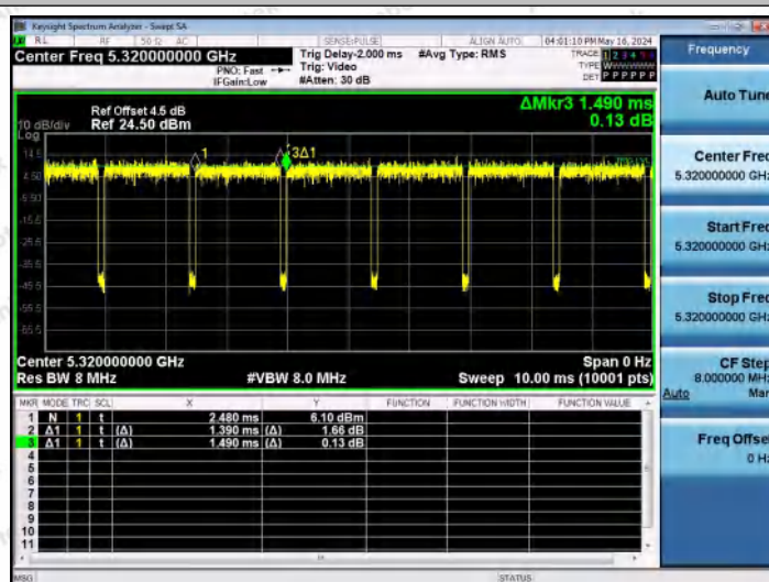
NTNV-11A-Ant2-5320
