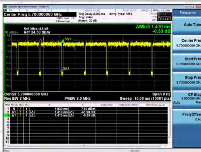
NTVN-11N20MIMO-Ant1-5700
