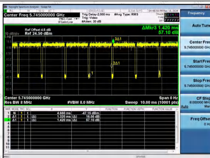
NTNV-11AC20MIMO-Ant2-5745
