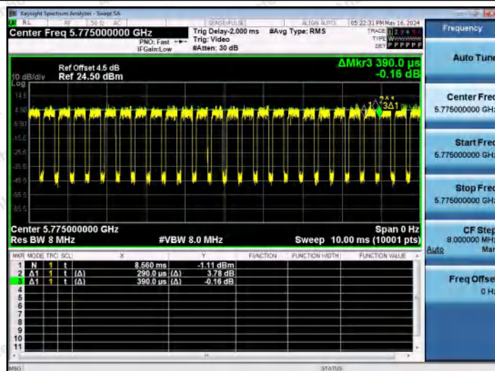
NTNV-11AX80MIMO-Ant1-5775
