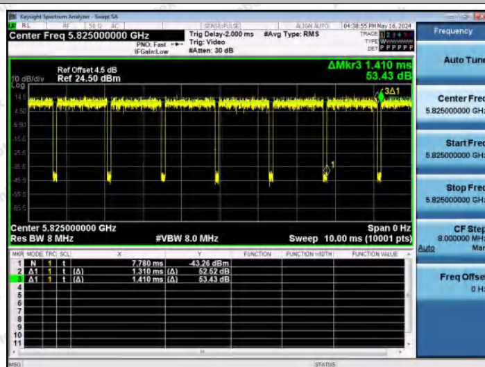
NTNV-11N20MIMO-Ant2-5825
