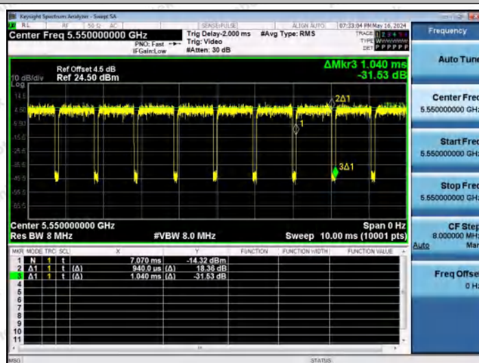
NTVN-11N40MIMO-Ant2-5550
