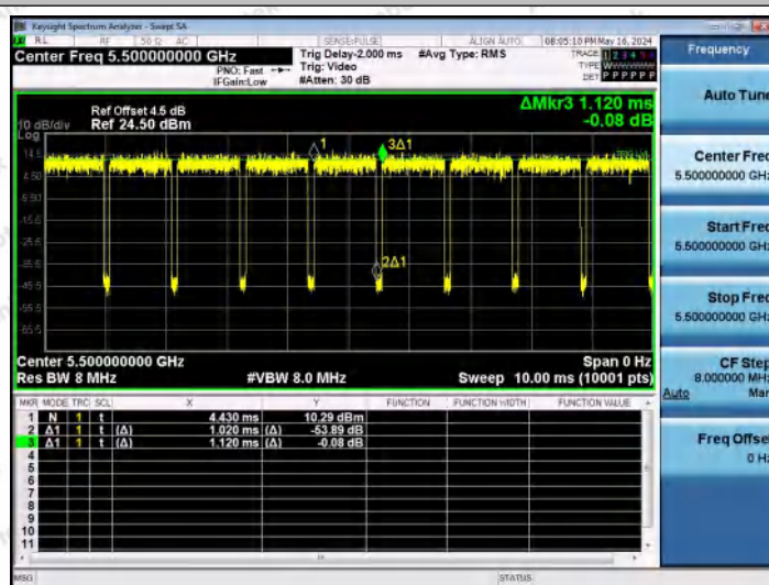
NTNV-11AX20MIMO-Ant2-5500
