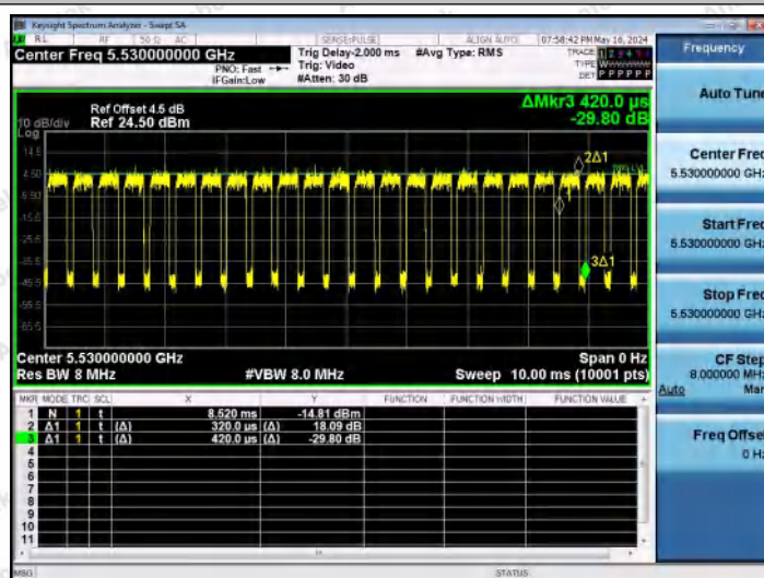
NTNV-11AC80MIMO-Ant1-5530
