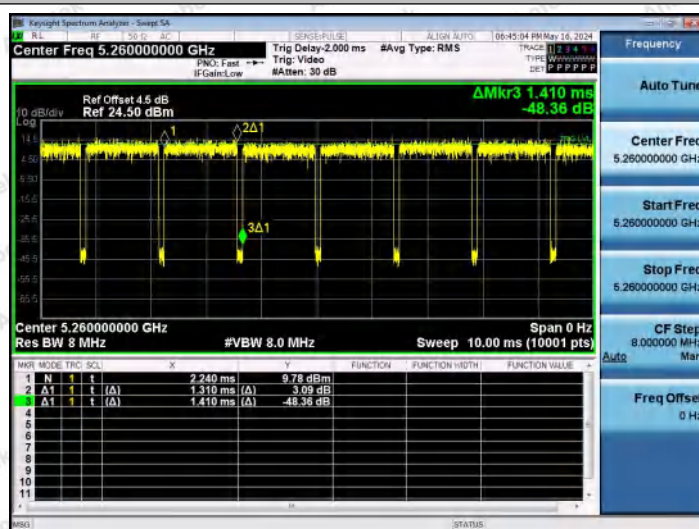
NTNV-11AC20MIMO-Ant2-5260
