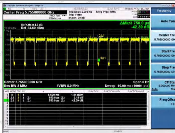
NTNV-11AC40MIMO-Ant1-5755
