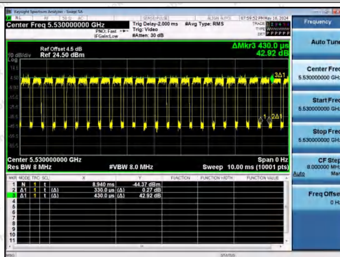
NTNV-11AC80MIMO-Ant2-5530
