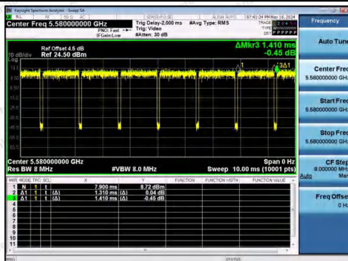
NTNV-11AC20MIMO-Ant2-5580
