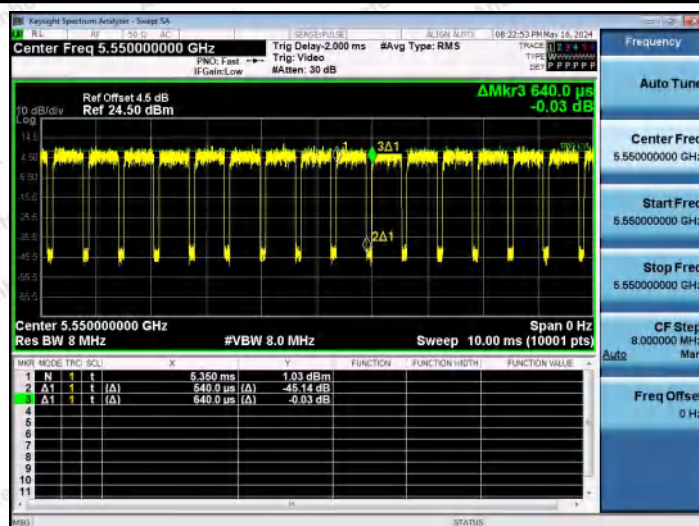
NTNV-11AX40MIMO-Ant2-5550
