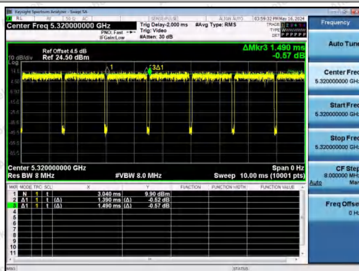
NTNV-11A-Ant1-5320
