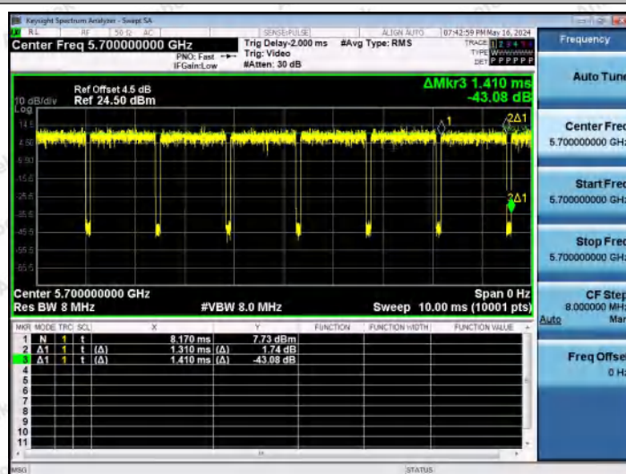
NTNV-11AC20MIMO-Ant1-5700
