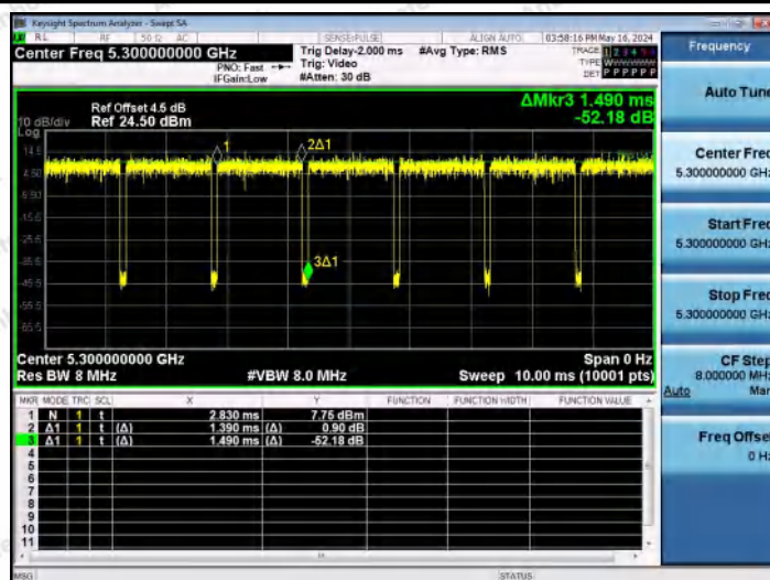
NTNV-11A-Ant2-5300
