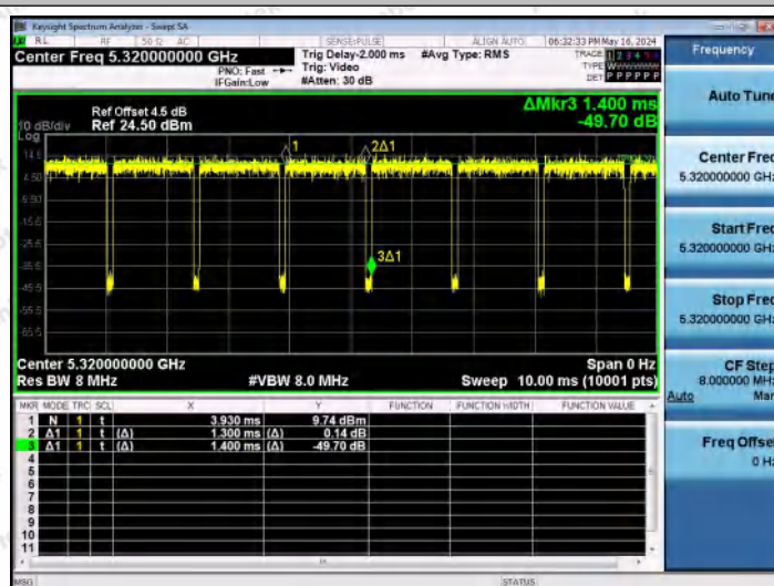
NTNV-11N20MIMO-Ant2-5320
