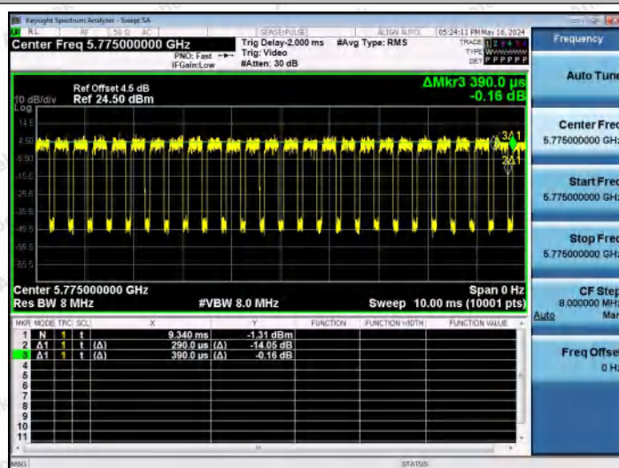
NTNV-11AX80MIMO-Ant2-5775
