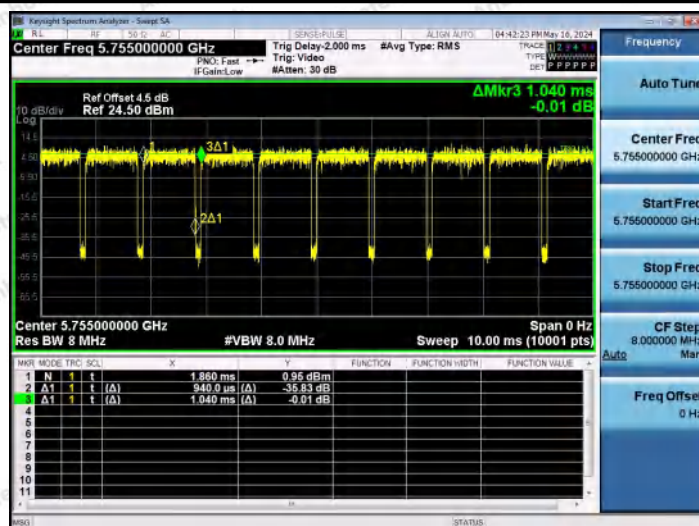
NTVN-11N40MIMO-Ant2-5755
