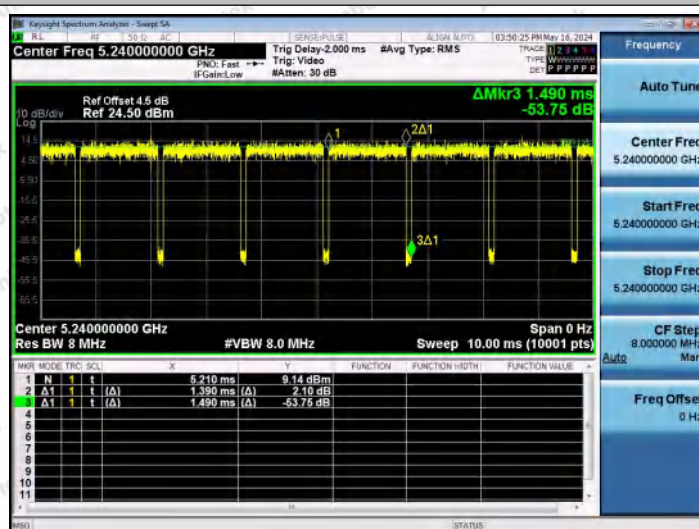
NTNV-11A-Ant2-5240
