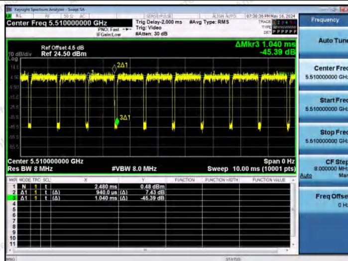
NTVN-11N40MIMO-Ant2-5510
