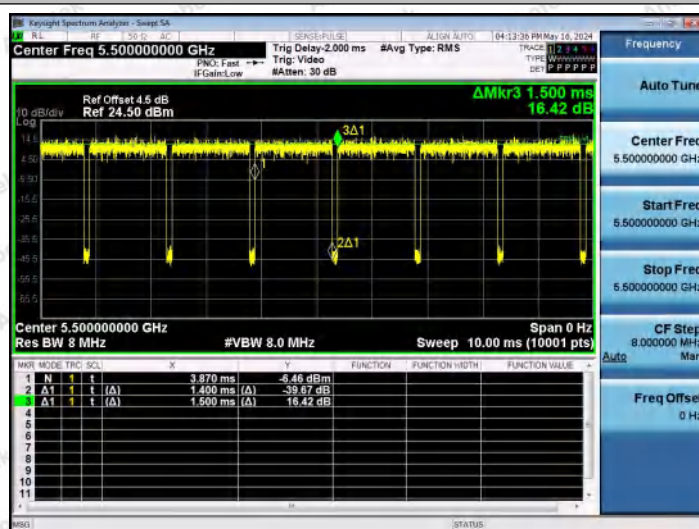
NTNV-11A-Ant2-5500
