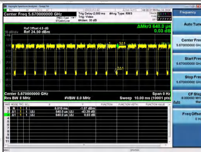
NTNV-11AX40MIMO-Ant2-5670
