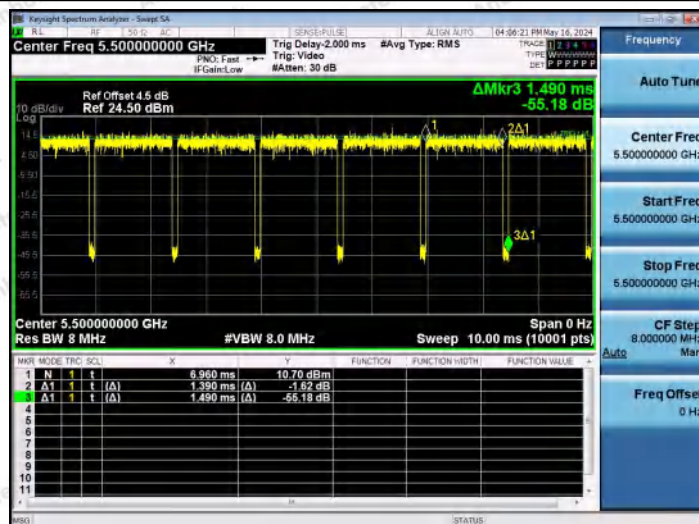
NTNV-11A-Ant1-5500
