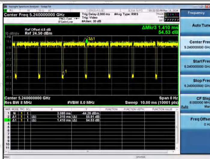
NTNV-11N20MIMO-Ant2-5240
