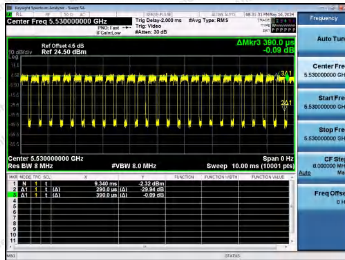
NTNV-11AX80MIMO-Ant2-5530
