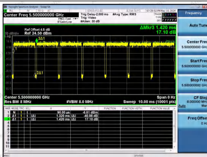
NTNV-11AC20MIMO-Ant2-5500
