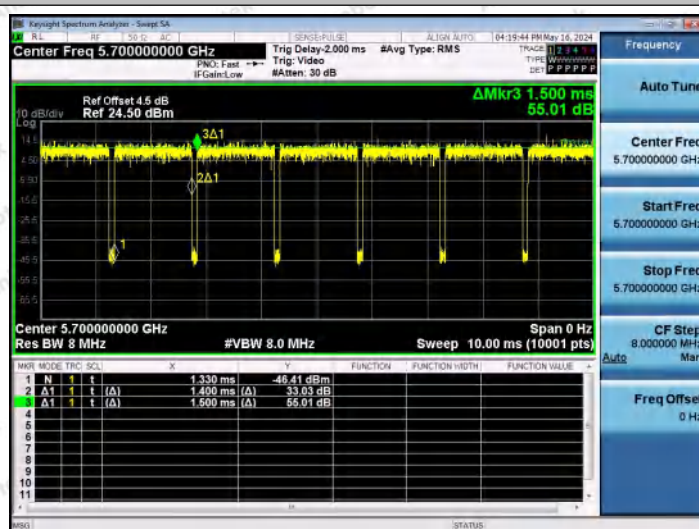
NTNV-11A-Ant2-5700
