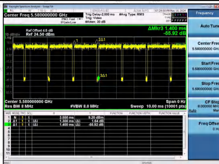
NTVN-11N20MIMO-Ant2-5580
