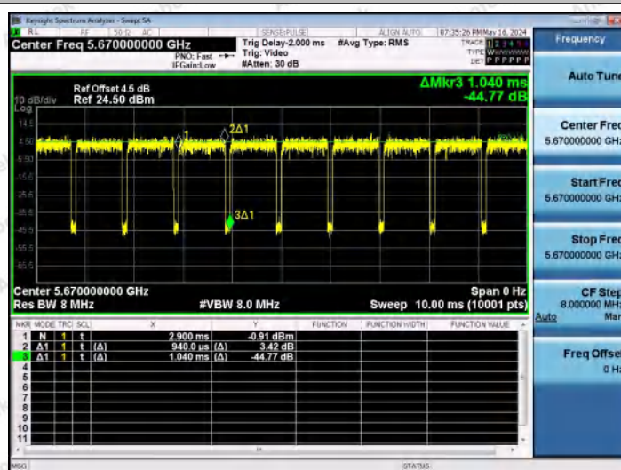
NTNV-11N40MIMO-Ant2-5670
