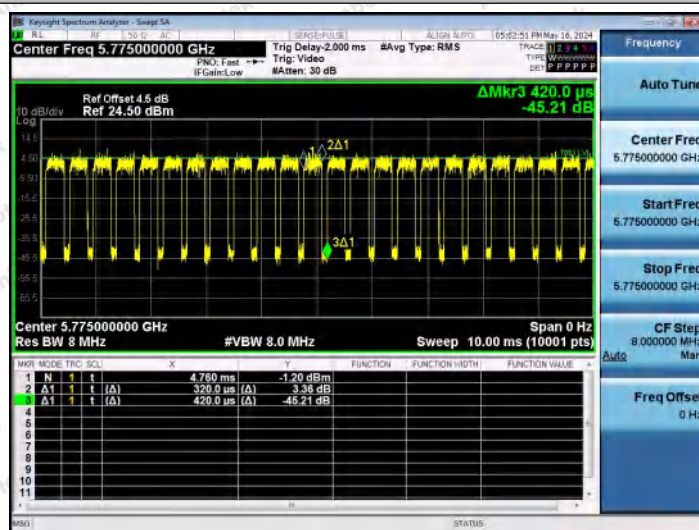
NTNV-11AC80MIMO-Ant1-5775
