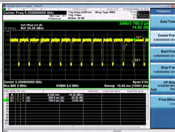
NTNV-11AC40MIMO-Ant2-5550
