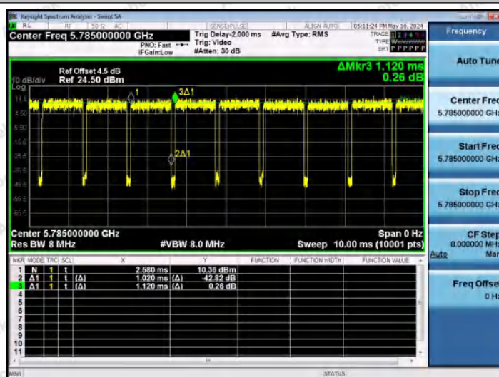
NTNV-11AX20MIMO-Ant2-5785
