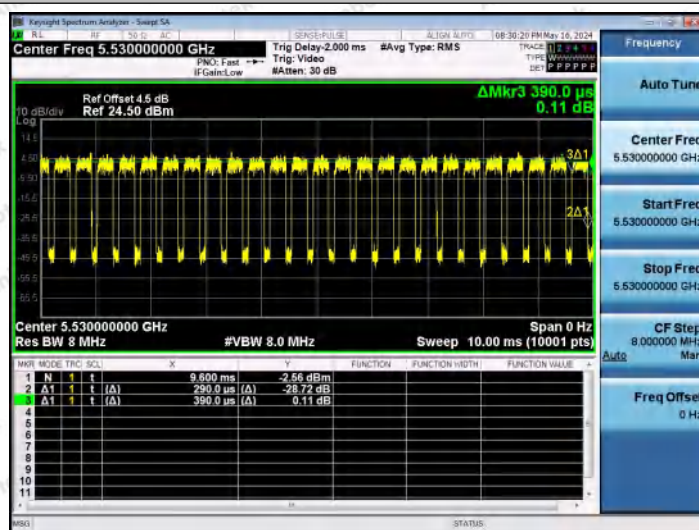
NTNV-11AX80MIMO-Ant1-5530
