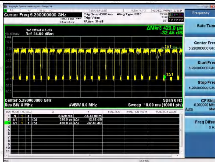
NTNV-11AC80MIMO-Ant2-5290
