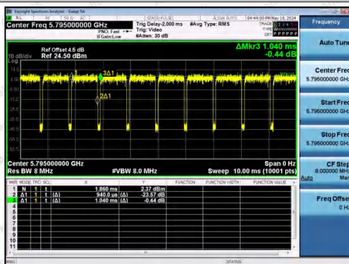
NTVN-11N40MIMO-Ant1-5795
