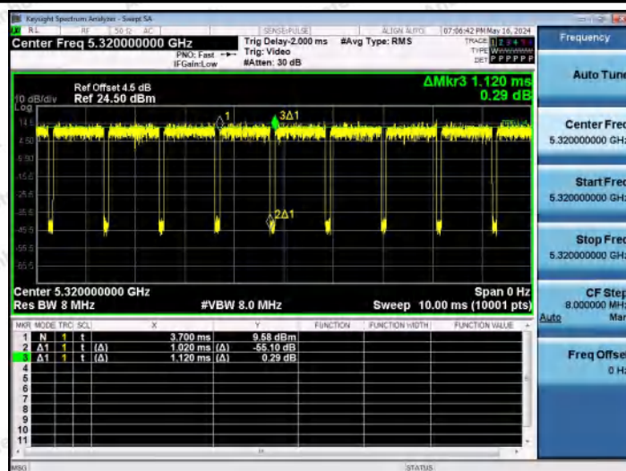
NTNV-11AX20MIMO-Ant2-5320
