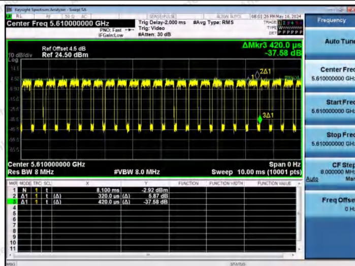
NTNV-11AC80MIMO-Ant1-5610
