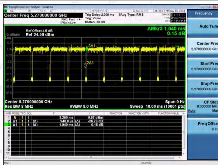
NTNV-11N40MIMO-Ant2-5270
