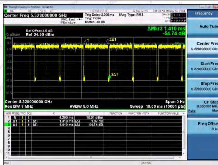
NTNV-11AC20MIMO-Ant2-5320
