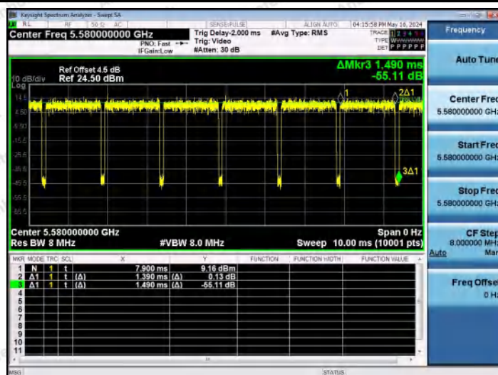
NTNV-11A-Ant2-5580
