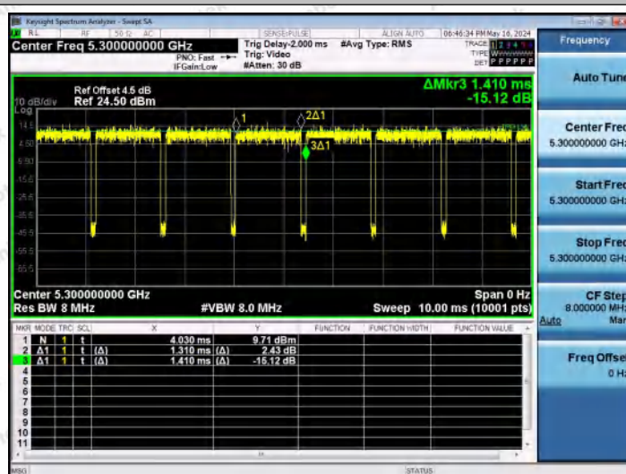
NTNV-11AC20MIMO-Ant1-5300
