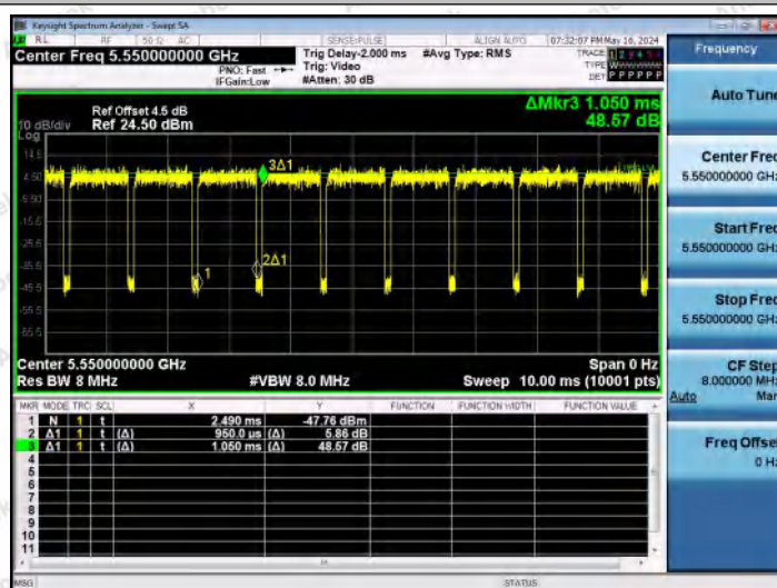
NTVN-11N40MIMO-Ant1-5550
