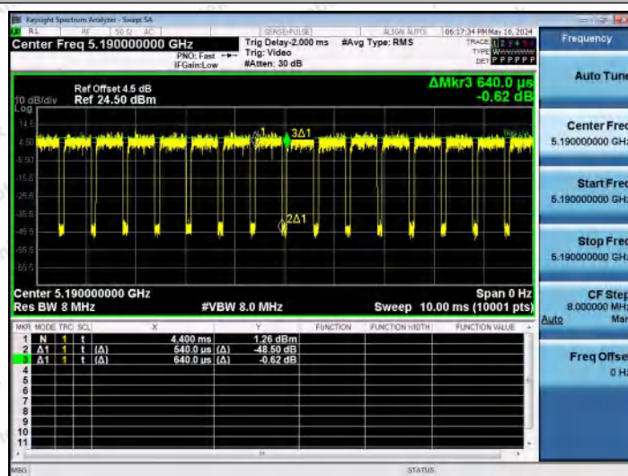
NTNV-11AX40MIMO-Ant2-5190
