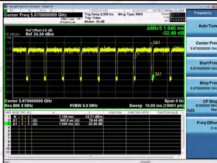
NTNV-11N40MIMO-Ant1-5670
