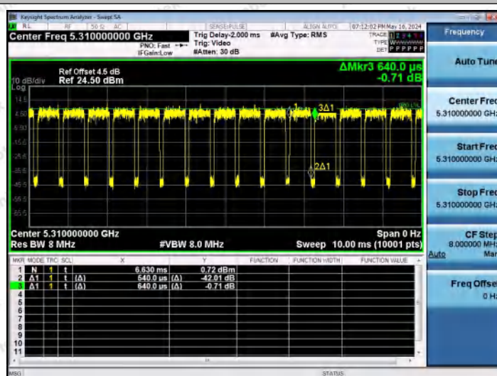
NTNV-11AX40MIMO-Ant2-5310
