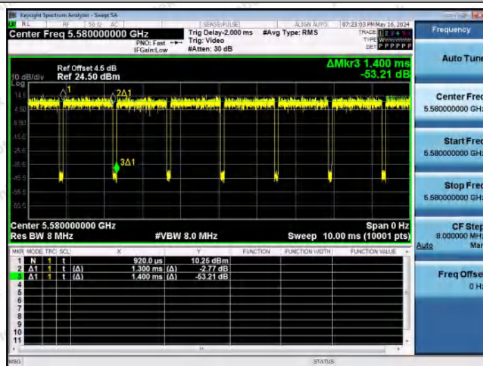
NTVN-11N20MIMO-Ant1-5580
