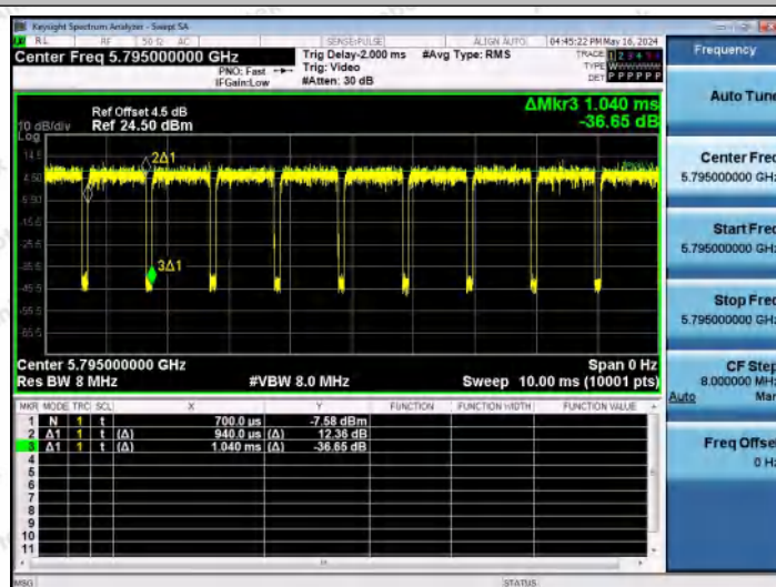
NTVN-11N40MIMO-Ant2-5795
