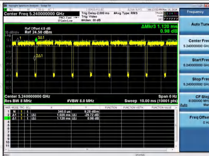
NTNV-11AX20MIMO-Ant2-5240
