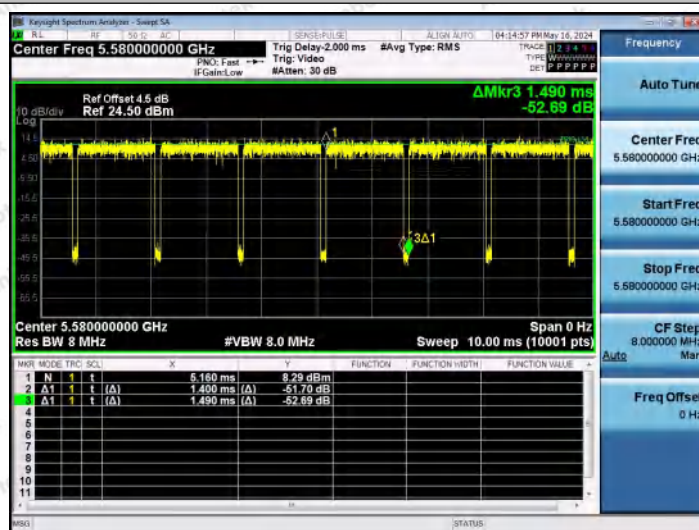
NTNV-11A-Ant1-5580
