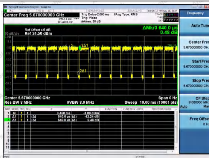
NTNV-11AX40MIMO-Ant1-5670
