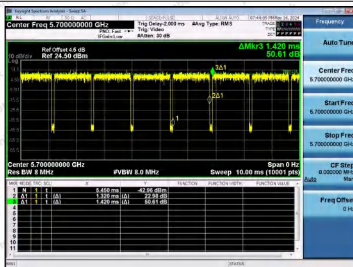
NTNV-11AC20MIMO-Ant2-5700
