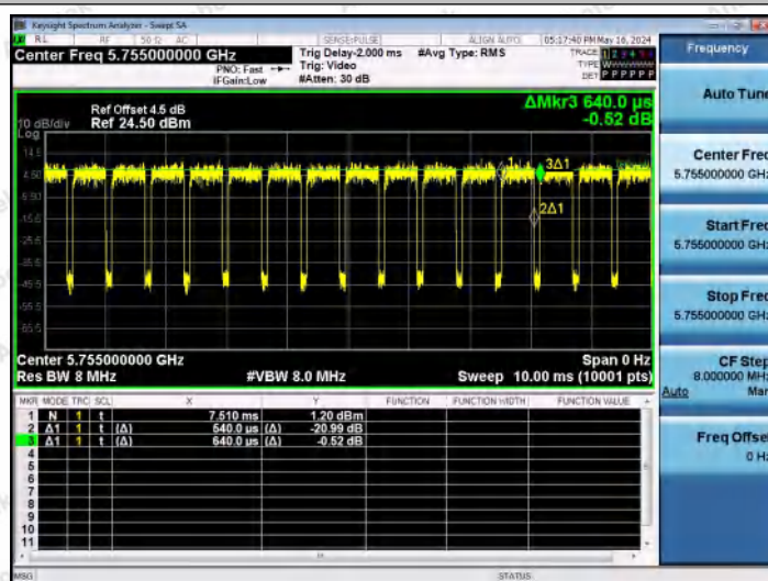
NTNV-11AX40MIMO-Ant2-5755
