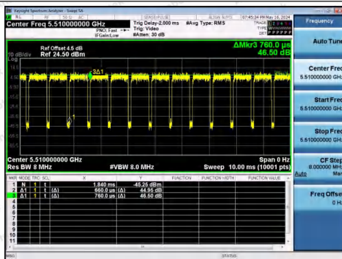
NTNV-11AC40MIMO-Ant1-5510
