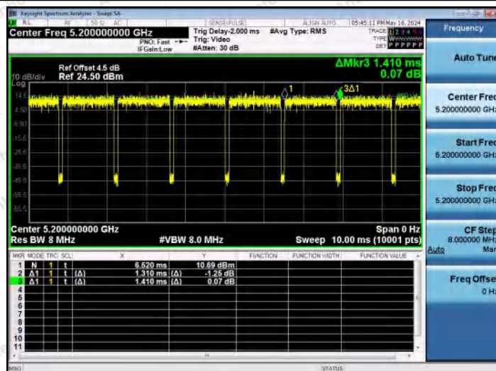
NTNV-11AC20MIMO-Ant2-5200
