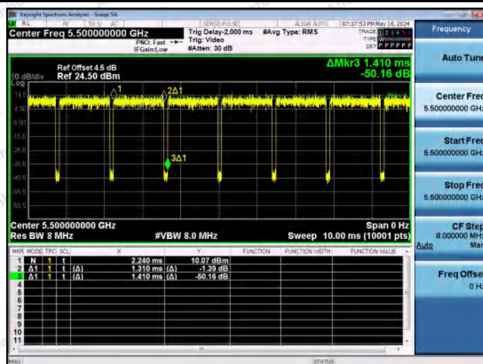
NTNV-11AC20MIMO-Ant1-5500
