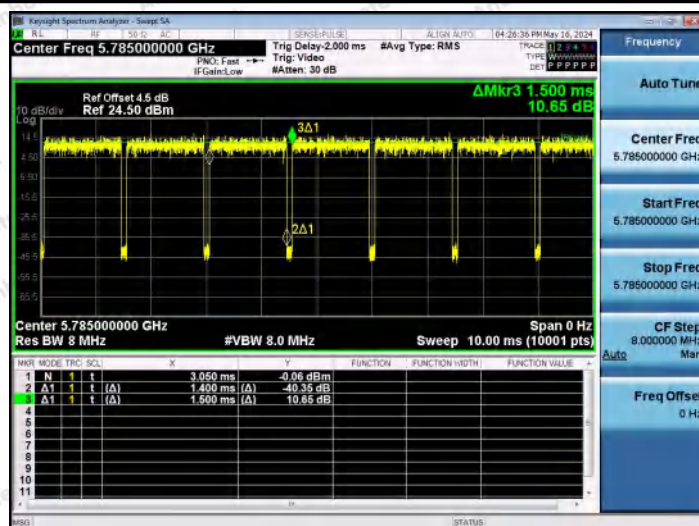
NTNV-11A-Ant2-5785
