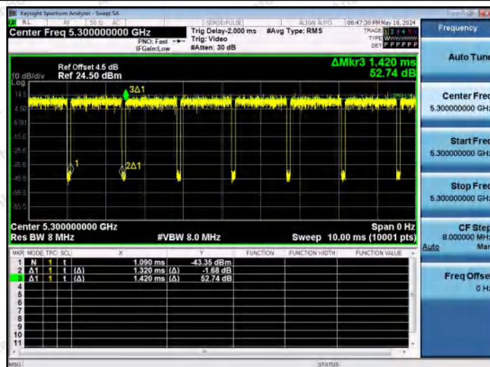
NTNV-11AC20MIMO-Ant2-5300
