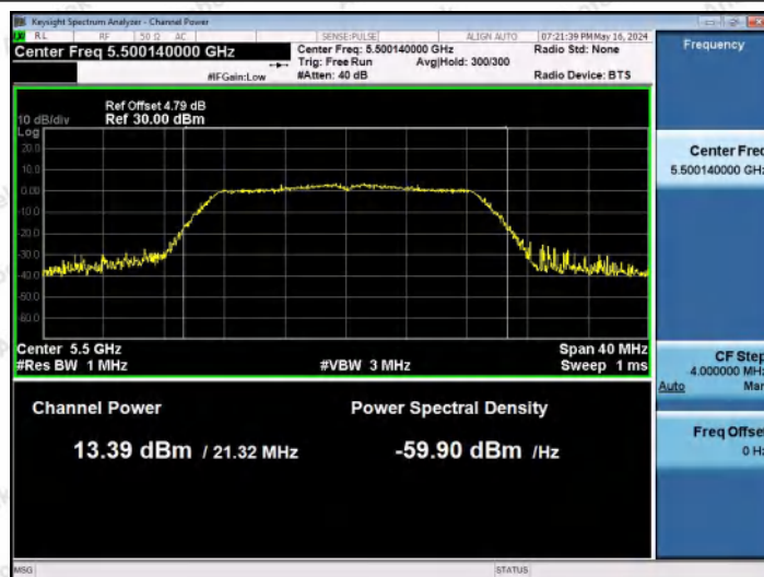
11N20MIMO-Ant2-5500-PASS
