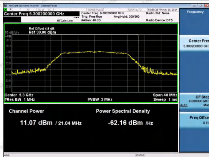
11A-Ant2-5300-PASS
