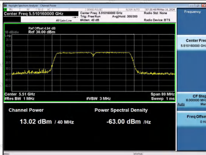
11N40MIMO-Ant2-5510-PASS
