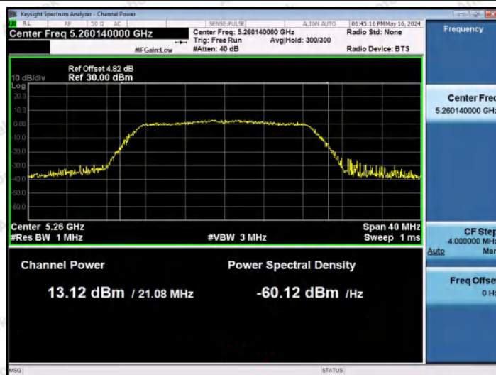
11AC20MIMO-Ant2-5260-PASS
