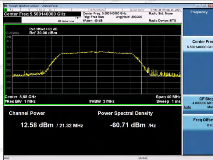
11AC20MIMO-Ant2-5580-PASS
