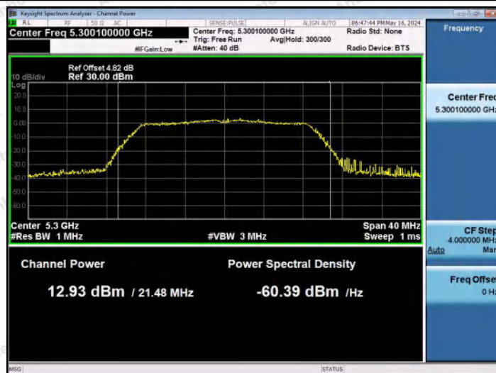
11AC20MIMO-Ant2-5300-PASS
