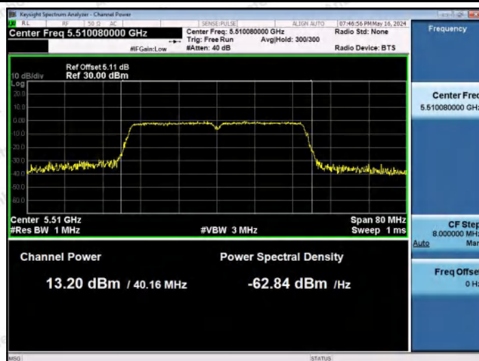
11AC40MIMO-Ant2-5510-PASS
