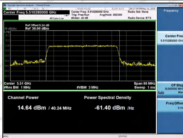
11AX40MIMO-Ant2-5510-PASS
