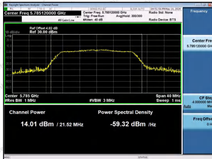
11AC20MIMO-Ant2-5785-PASS
