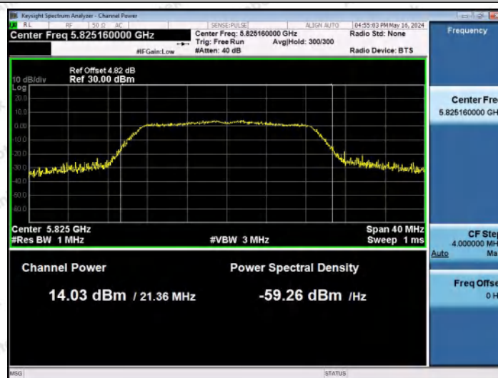
11AC20MIMO-Ant2-5825-PASS
