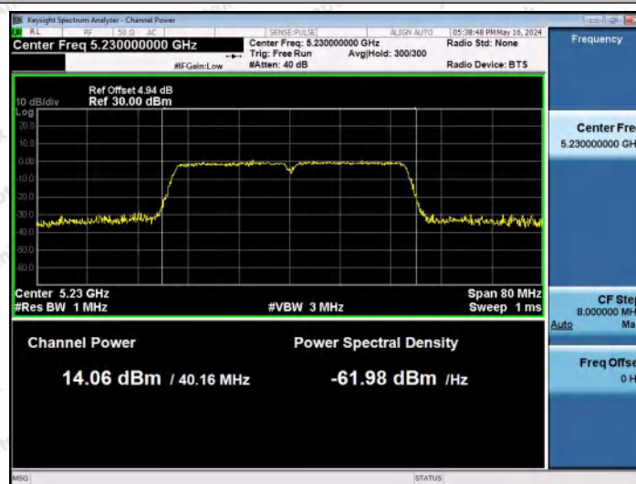
11N40MIMO-Ant1-5230-PASS
