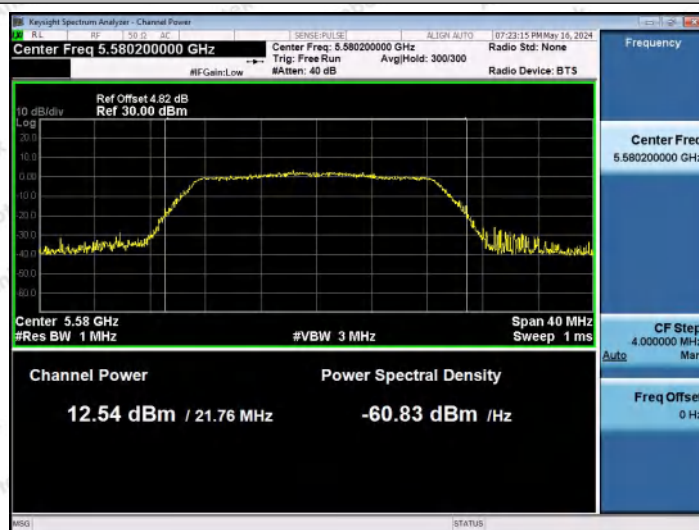
11N20MIMO-Ant1-5580-PASS
