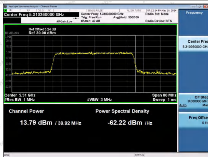
11AX40MIMO-Ant2-5310-PASS
