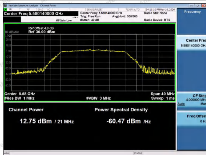
11A-Ant2-5580-PASS
