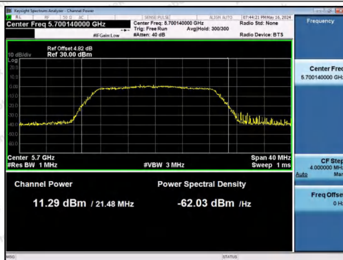
11AC20MIMO-Ant2-5700-PASS
