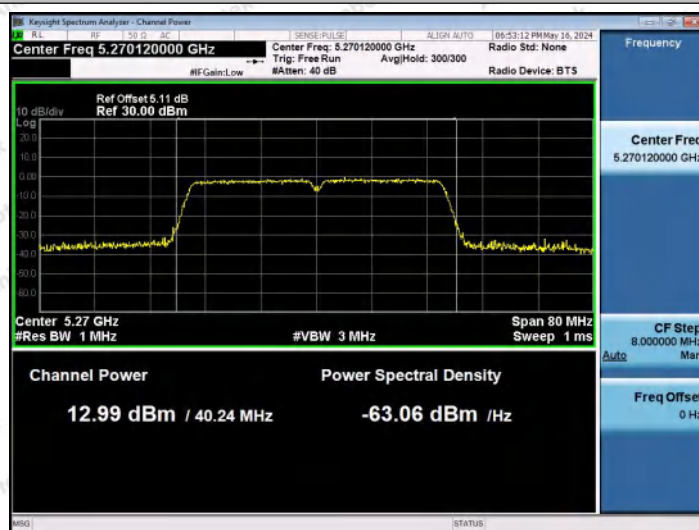
11AC40MIMO-Ant2-5270-PASS
