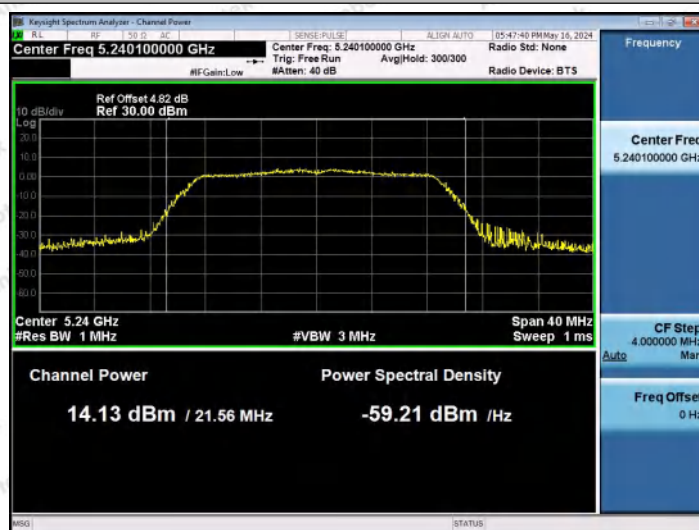
11AC20MIMO-Ant2-5240-PASS
