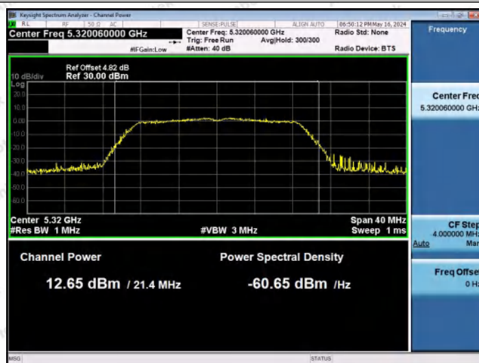
11AC20MIMO-Ant2-5320-PASS
