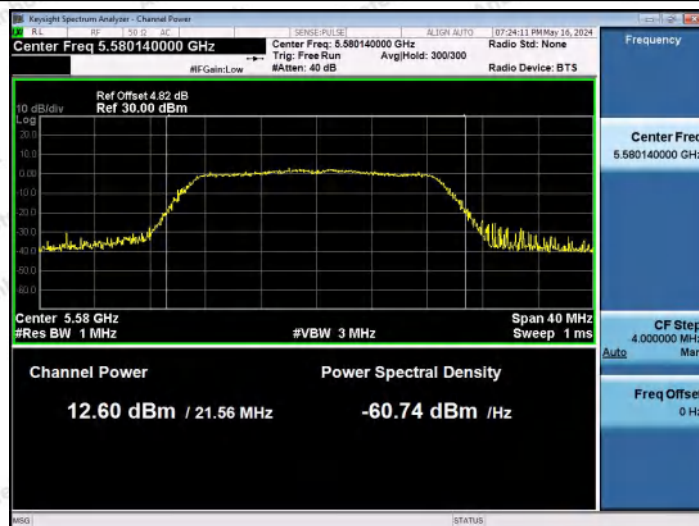
11N20MIMO-Ant2-5580-PASS
