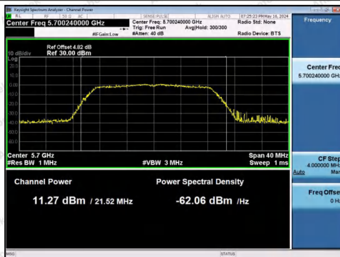
11N20MIMO-Ant1-5700-PASS
