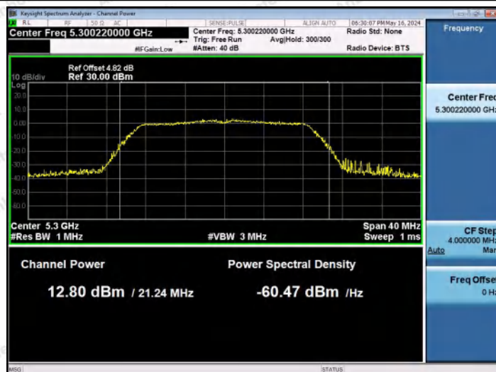
11N20MIMO-Ant2-5300-PASS
