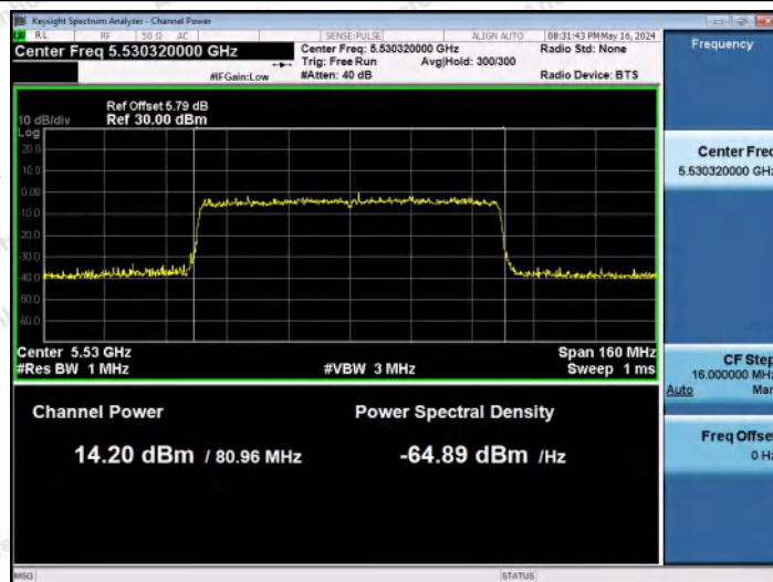
11AX80MIMO-Ant2-5530-PASS
