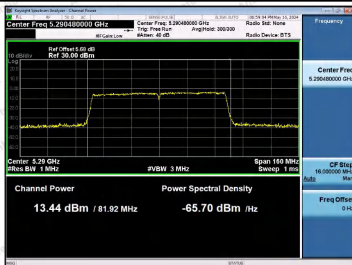
11AC80MIMO-Ant2-5290-PASS
