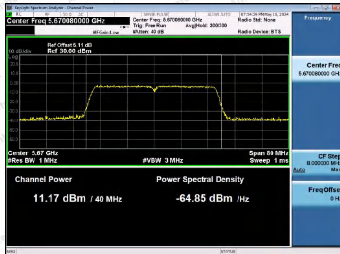
11AC40MIMO-Ant1-5670-PASS
