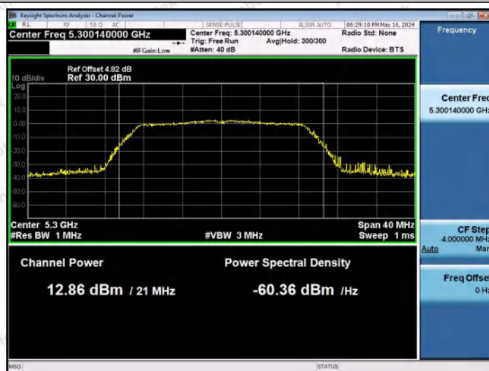
11N20MIMO-Ant1-5300-PASS
