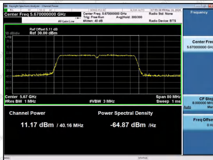
11AC40MIMO-Ant2-5670-PASS
