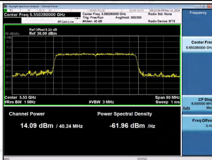
11AX40MIMO-Ant2-5550-PASS
