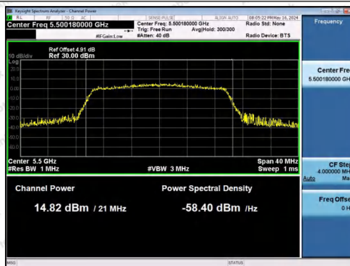
11AX20MIMO-Ant2-5500-PASS
