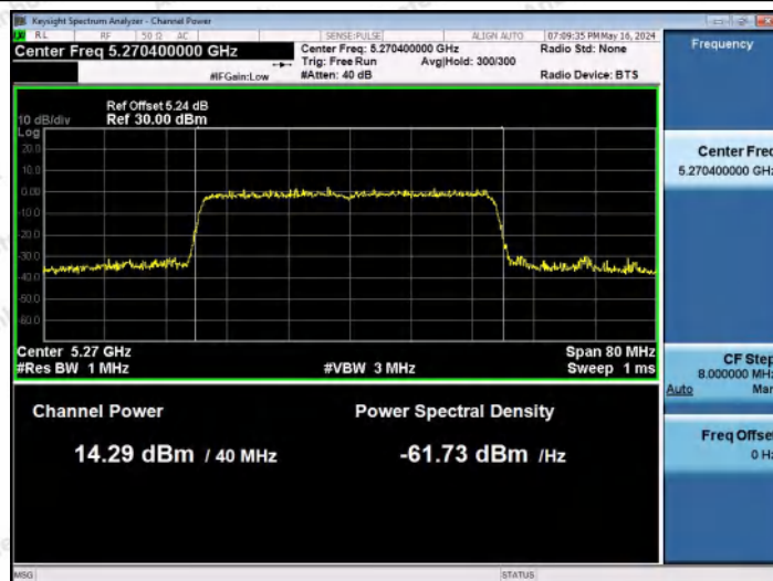
11AX40MIMO-Ant2-5270-PASS
