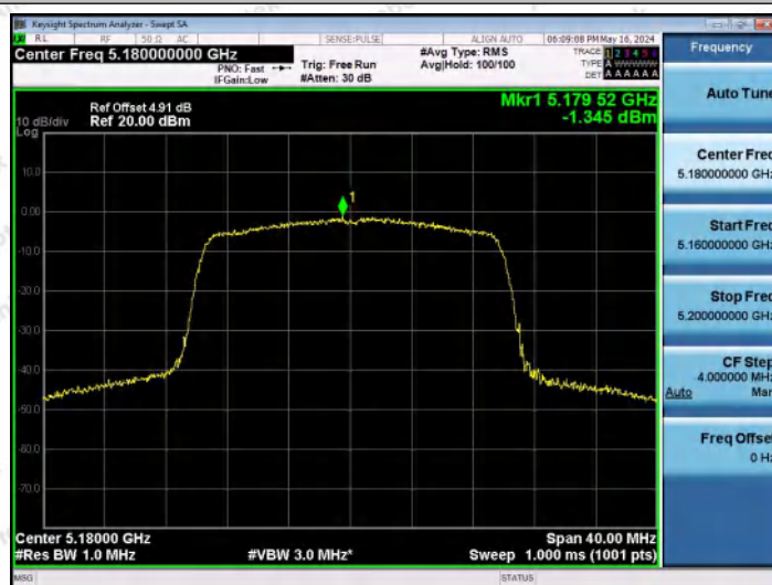
11AX20MIMO-Ant2-5180-PASS
