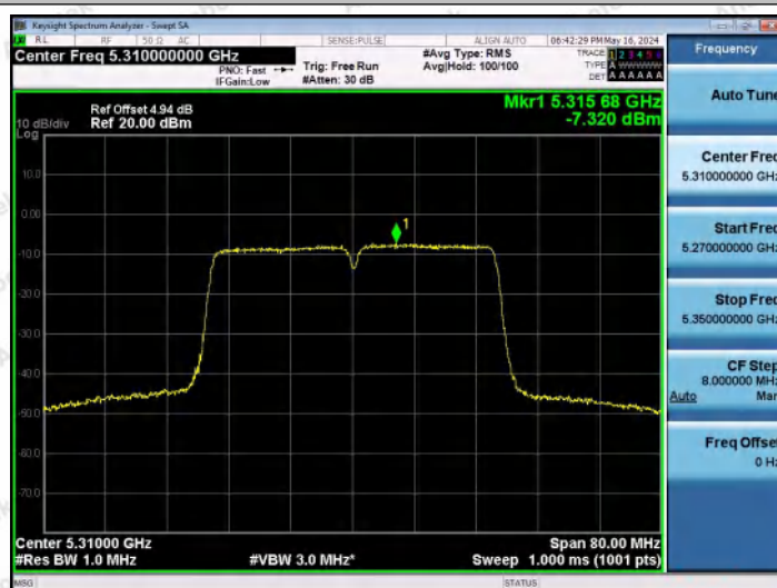
11N40MIMO-Ant2-5310-PASS
