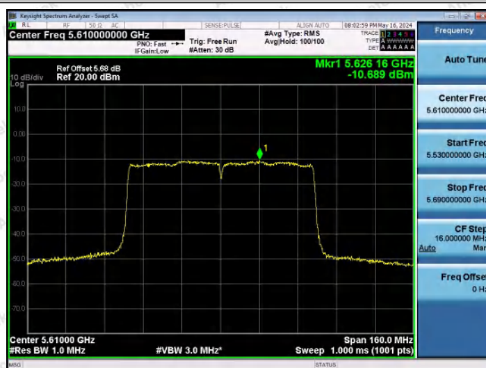
11AC80MIMO-Ant2-5610-PASS
