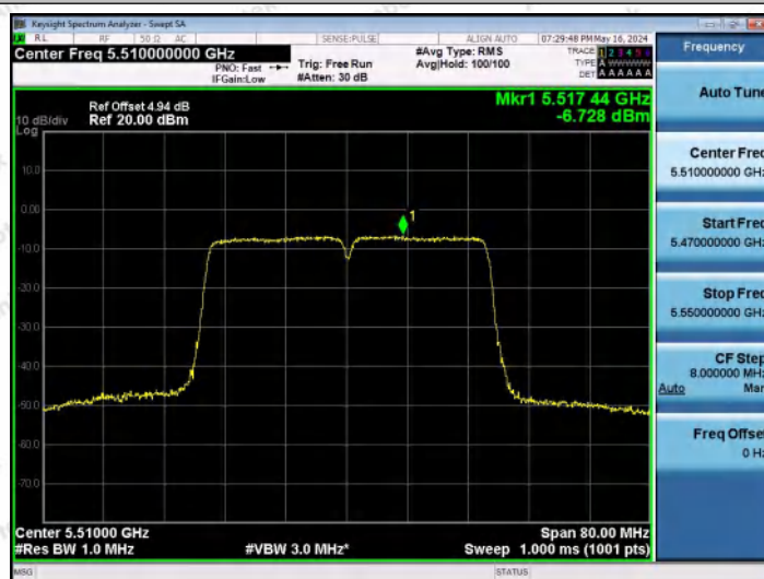
11N40MIMO-Ant1-5510-PASS
