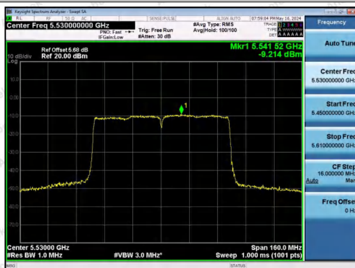
11AC80MIMO-Ant1-5530-PASS
