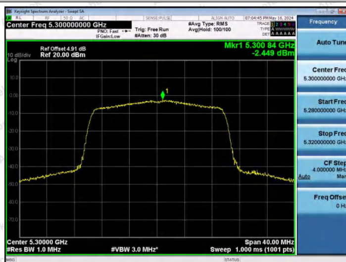
11AX20MIMO-Ant2-5300-PASS
