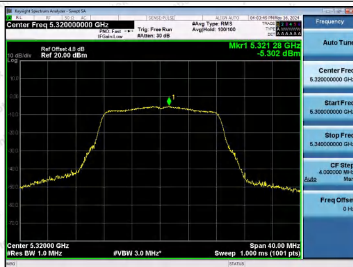
11A-Ant2-5320-PASS
