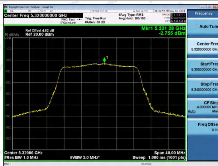
11N20MIMO-Ant2-5320-PASS
