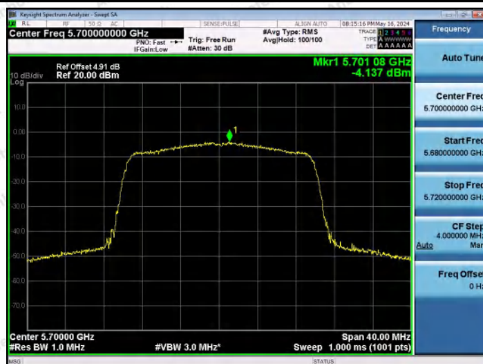
11AX20MIMO-Ant2-5700-PASS
