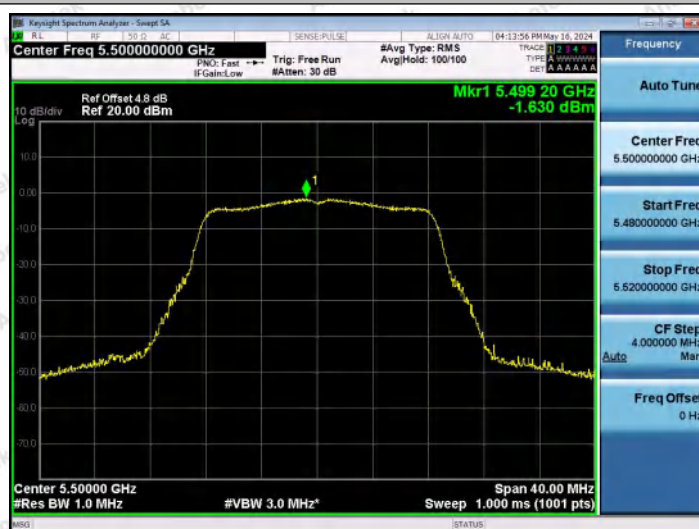
11A-Ant2-5500-PASS
