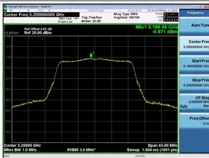
11AC20MIMO-Ant1-5200-PASS
