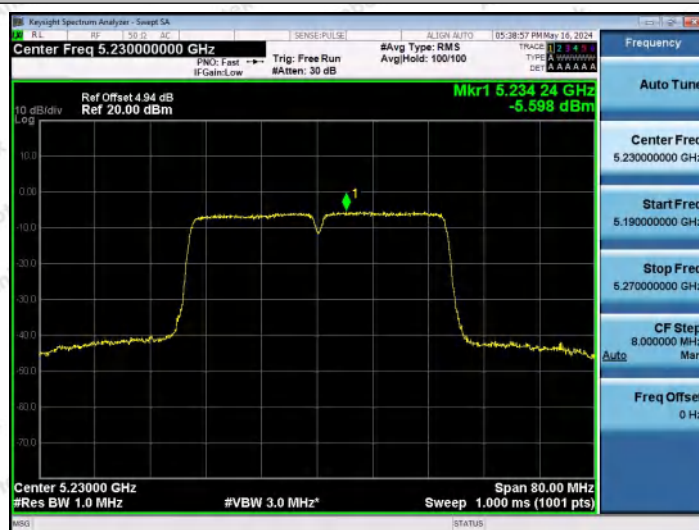
11N40MIMO-Ant1-5230-PASS
