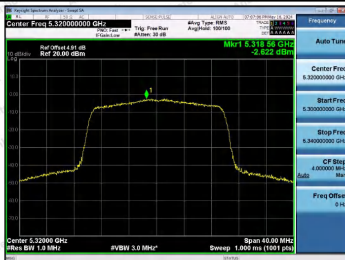
11AX20MIMO-Ant2-5320-PASS
