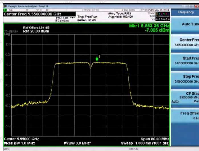
11N40MIMO-Ant2-5550-PASS
