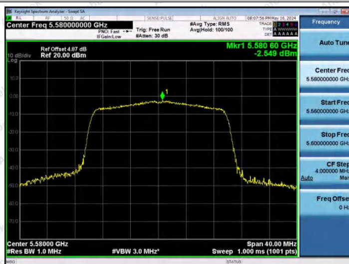
11AX20MIMO-Ant2-5580-PASS
