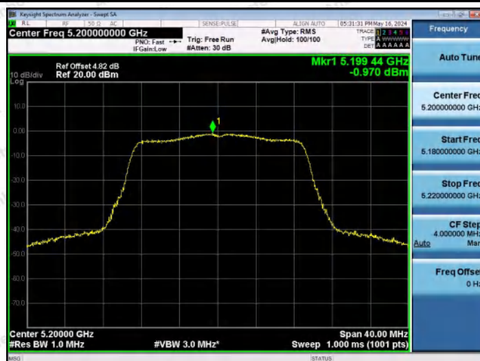
11N20MIMO-Ant2-5200-PASS
