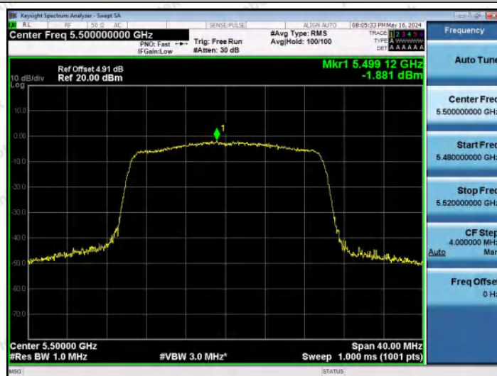
11AX20MIMO-Ant2-5500-PASS
