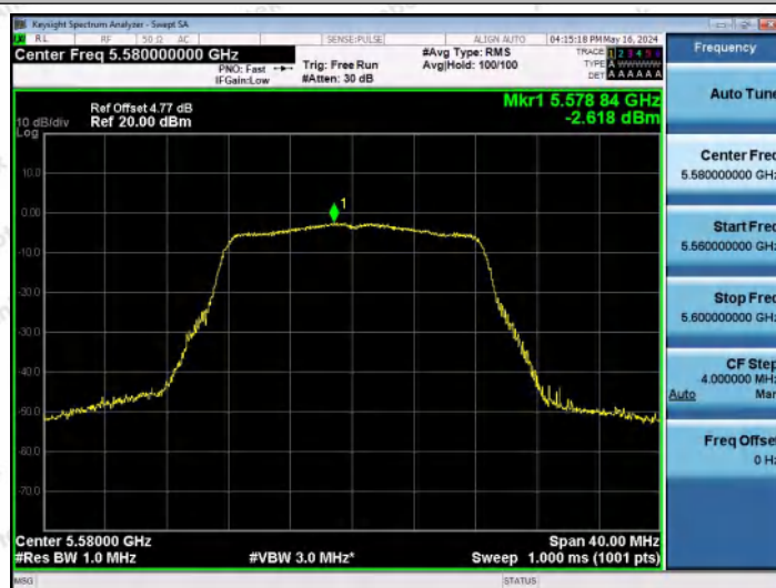
11A-Ant1-5580-PASS
