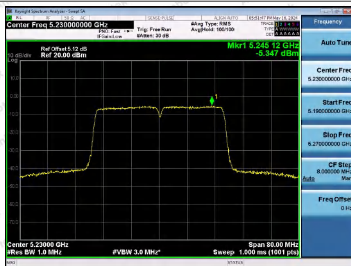
11AC40MIMO-Ant1-5230-PASS
