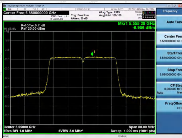
11AC40MIMO-Ant2-5550-PASS
