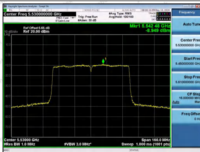
11AC80MIMO-Ant2-5530-PASS
