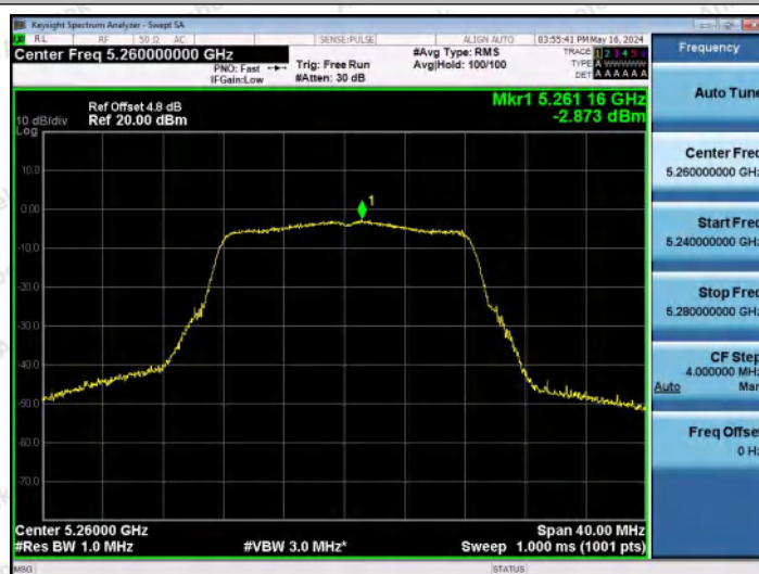
11A-Ant2-5260-PASS
