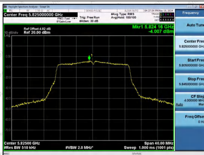
11N20MIMO-Ant1-5825-PASS
