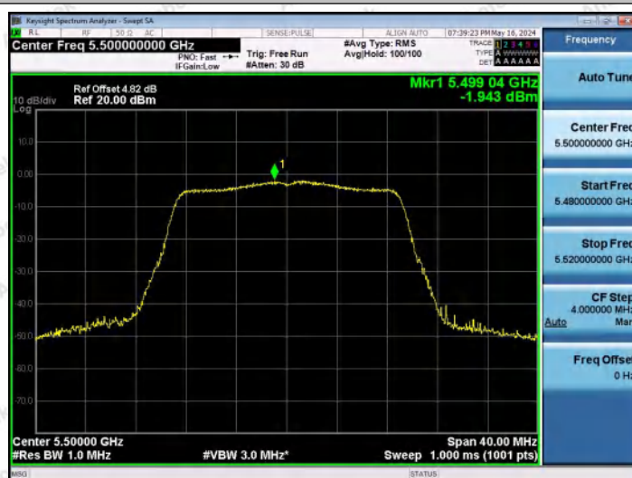
11AC20MIMO-Ant2-5500-PASS
