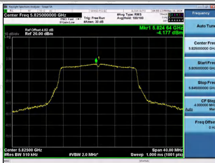
11AC20MIMO-Ant2-5825-PASS
