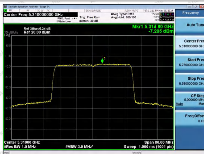
11AX40MIMO-Ant1-5310-PASS
