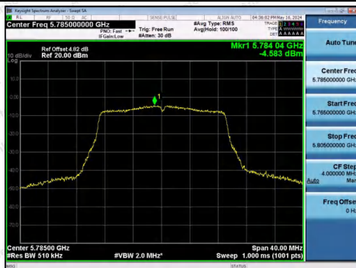
11N20MIMO-Ant2-5785-PASS
