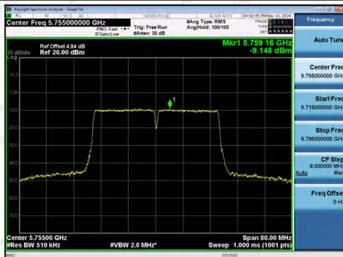
11N40MIMO-Ant2-5755-PASS
