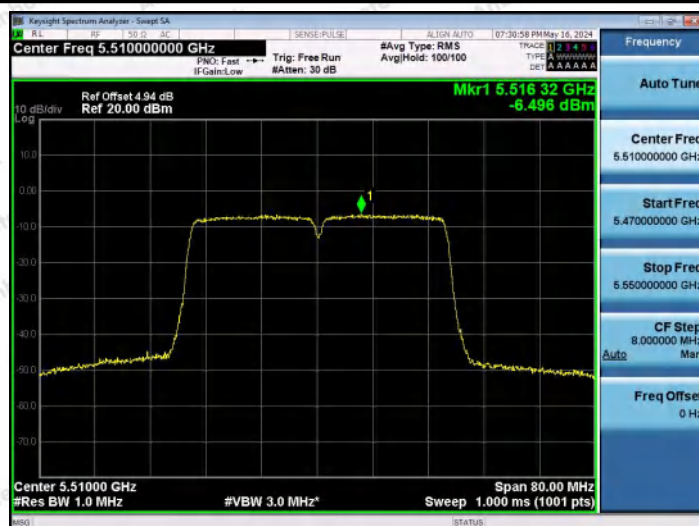
11N40MIMO-Ant2-5510-PASS
