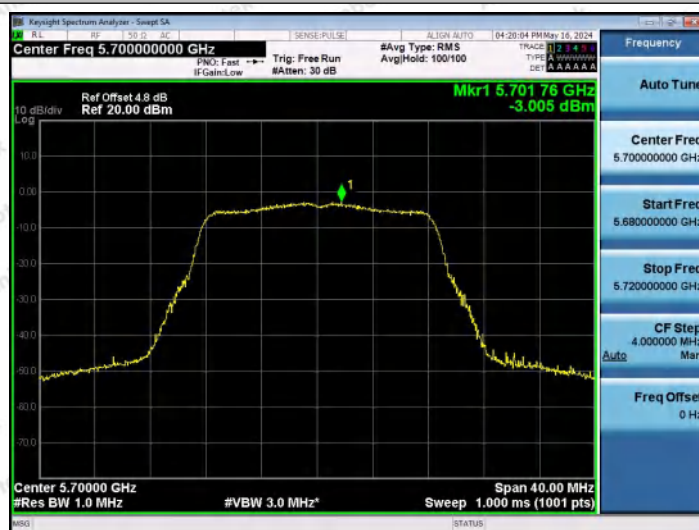
11A-Ant2-5700-PASS
