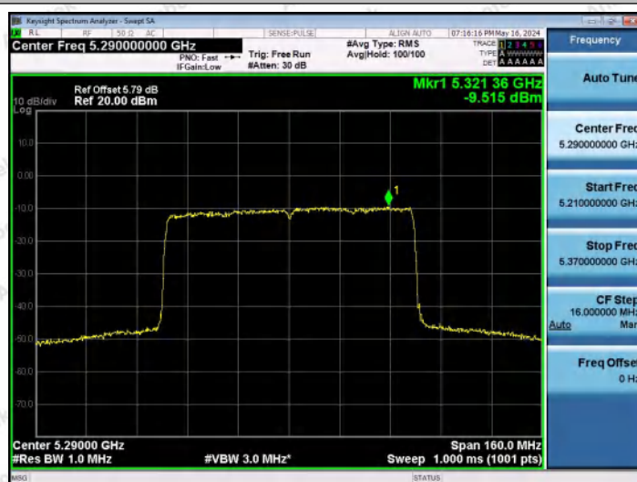
11AX80MIMO-Ant2-5290-PASS
