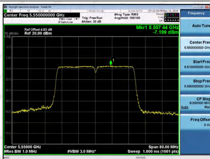
11N40MIMO-Ant1-5550-PASS
