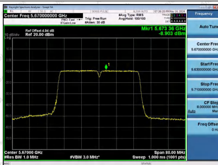
11N40MIMO-Ant2-5670-PASS
