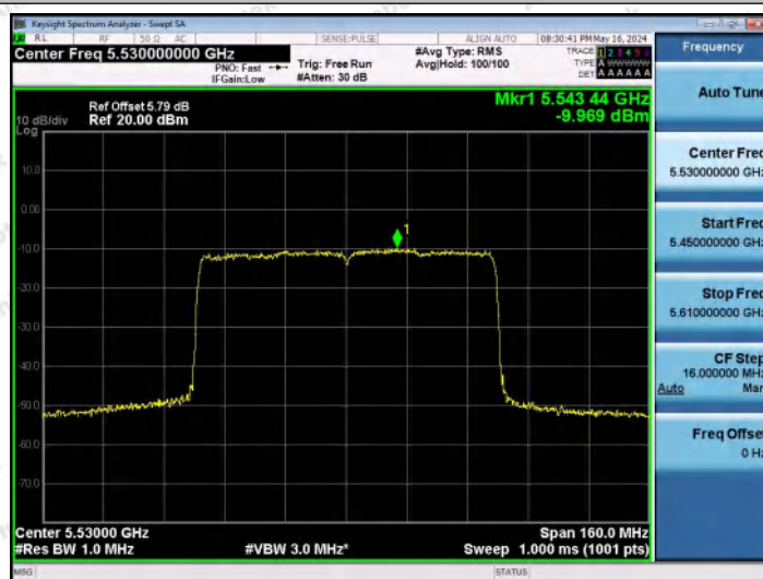
11AX80MIMO-Ant1-5530-PASS
