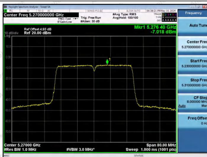
11N40MIMO-Ant1-5270-PASS
