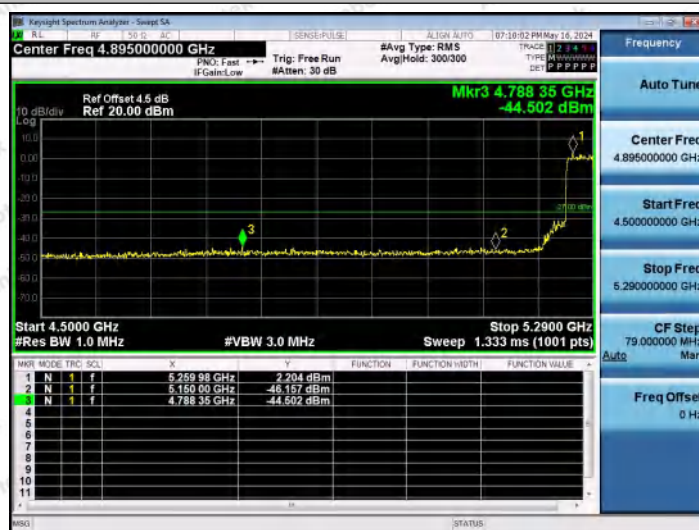
11AX40MIMO-Ant2-5270-PASS
