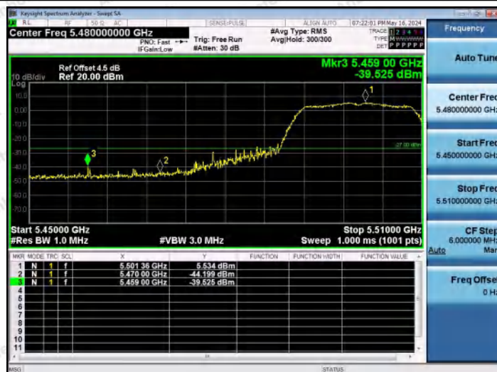
11N20MIMO-Ant2-5500-PASS
