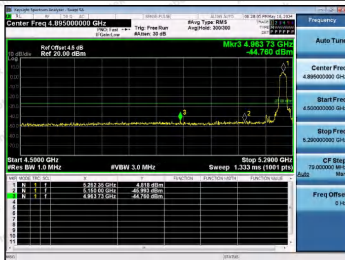
11N20MIMO-Ant2-5260-PASS
