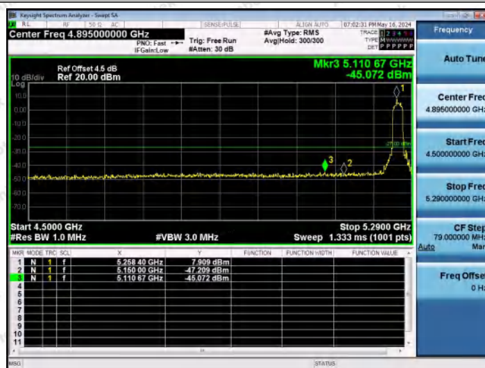
11AX20MIMO-Ant2-5260-PASS
