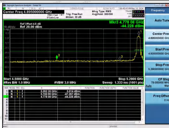
11AC20MIMO-Ant2-5260-PASS
