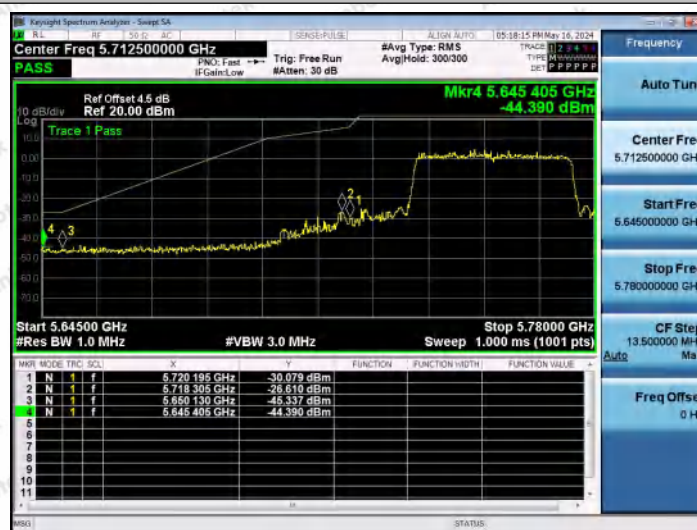
11AX40MIMO-Ant2-5755-PASS
