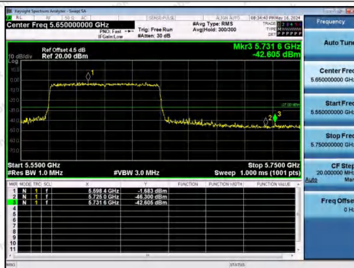
11AX80MIMO-Ant2-5610-PASS
