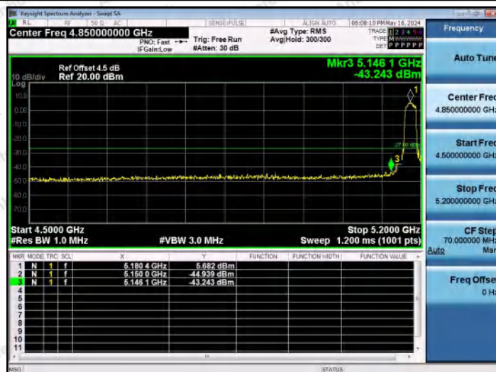
11AX20MIMO-Ant1-5180-PASS
