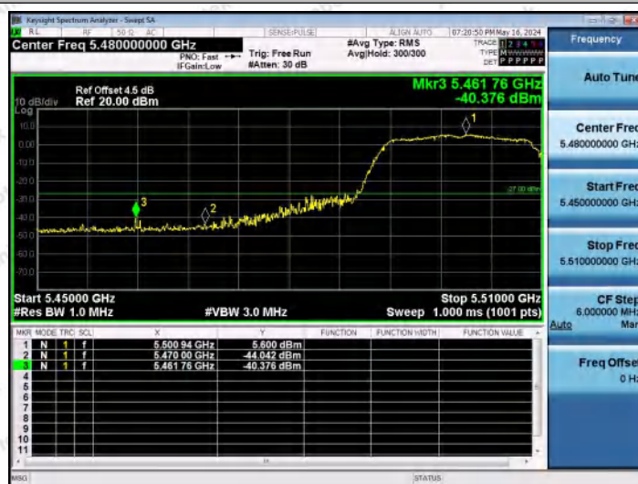
11N20MIMO-Ant1-5500-PASS
