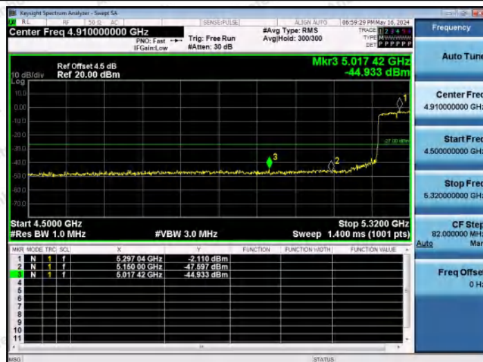
11AC80MIMO-Ant2-5290-PASS
