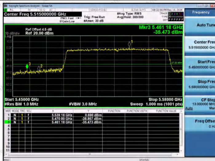
11AX80MIMO-Ant2-5530-PASS
