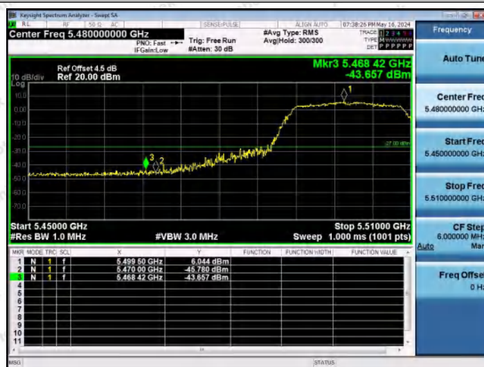
11AC20MIMO-Ant1-5500-PASS
