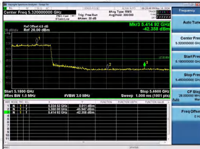
11AX80MIMO-Ant2-5210-PASS
