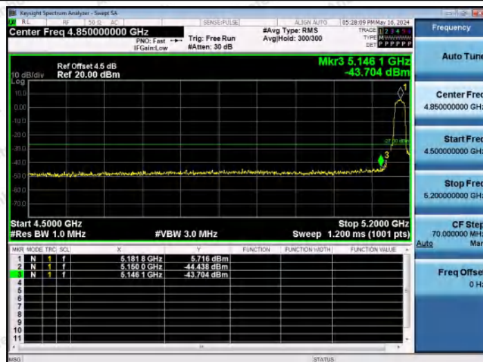
11N20MIMO-Ant1-5180-PASS
