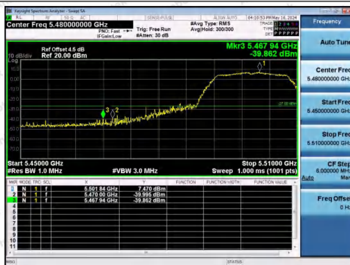
11A-Ant1-5500-PASS
