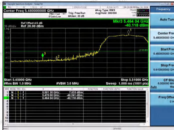
11A-Ant2-5500-PASS
