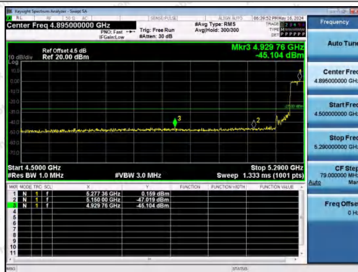
11N40MIMO-Ant2-5270-PASS
