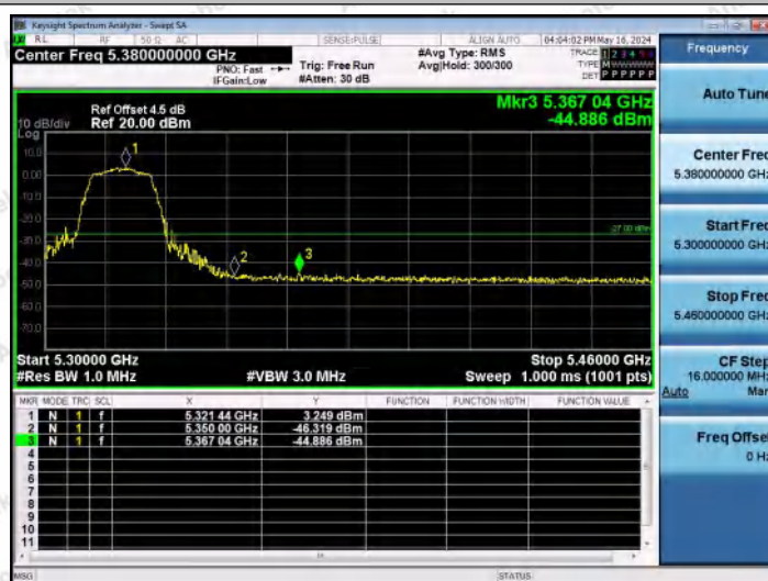
11A-Ant2-5320-PASS
