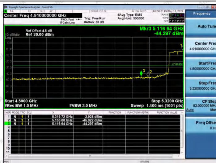
11AC80MIMO-Ant1-5290-PASS
