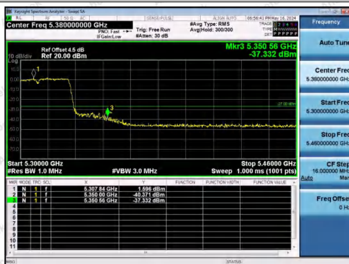
11AC40MIMO-Ant2-5310-PASS
