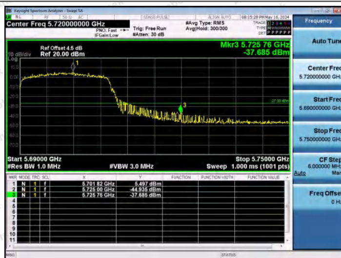
11AX20MIMO-Ant2-5700-PASS
