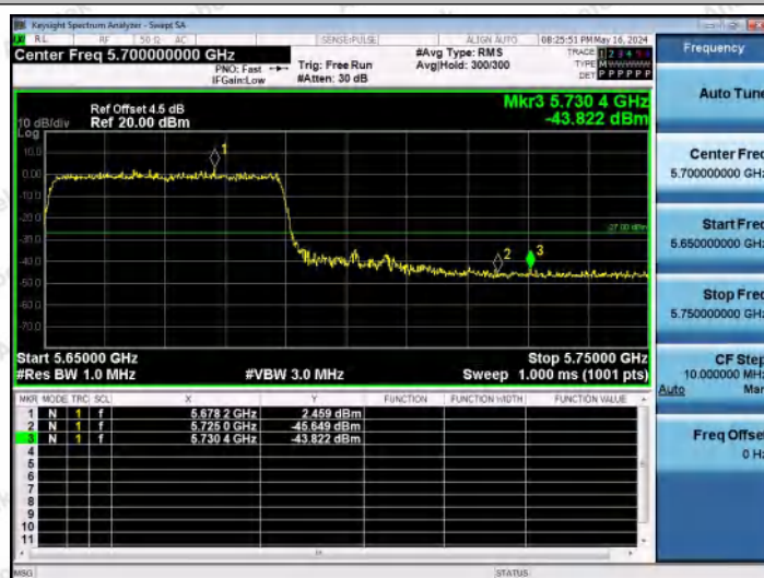
11AX40MIMO-Ant1-5670-PASS
