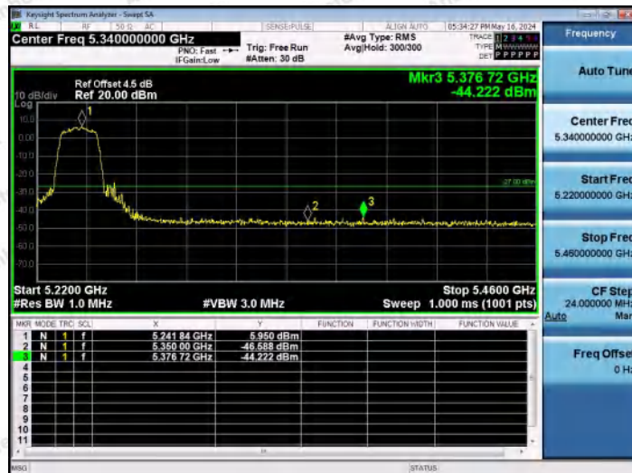
11N20MIMO-Ant2-5240-PASS
