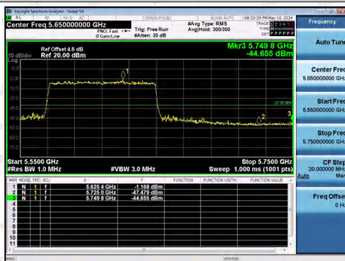
11AX80MIMO-Ant1-5610-PASS
