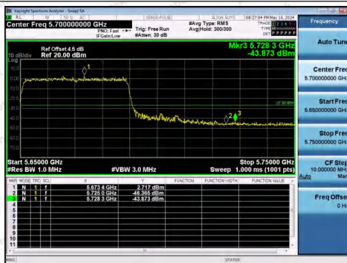
11AX40MIMO-Ant2-5670-PASS
