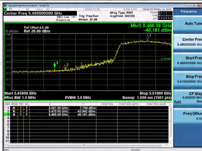
11AX20MIMO-Ant2-5500-PASS
