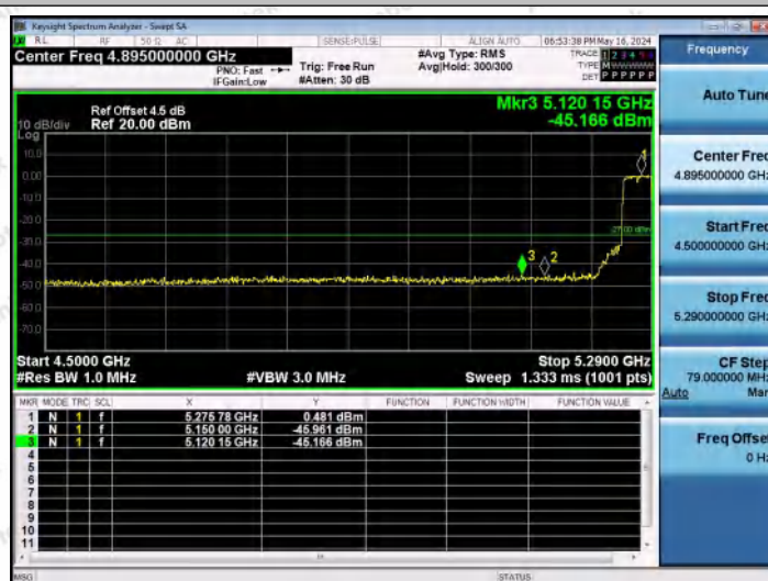
11AC40MIMO-Ant2-5270-PASS
