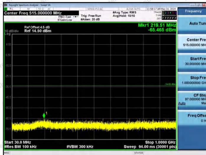
11AX20MIMO-Ant2-2412-30~1000-PASS
