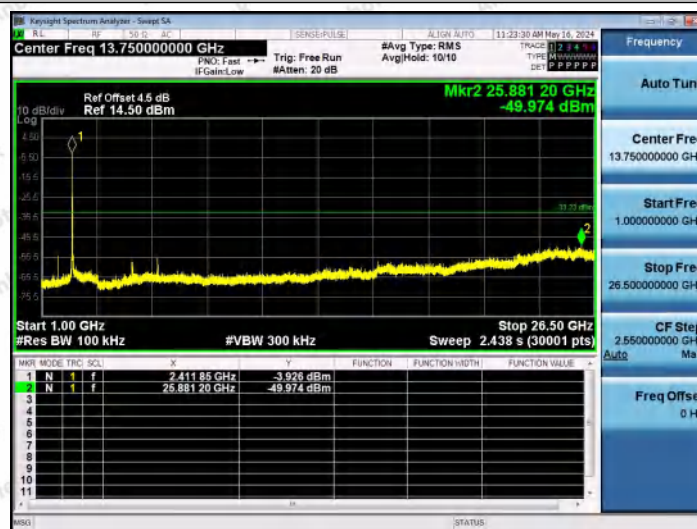
11G-Ant2-2412-1000~26500-PASS
