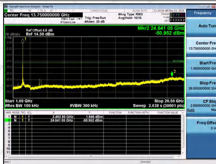
11B-Ant2-2462-1000~26500-PASS
