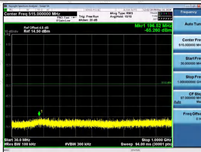
11AX20MIMO-Ant1-2437-30~1000-PASS
