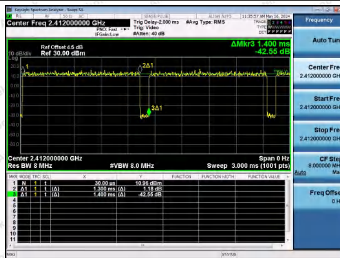
NTNV-11N20MIMO-Ant2-2412
