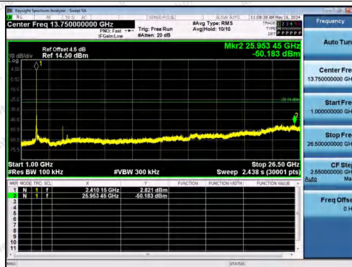
11B-Ant2-2412-1000~26500-PASS
