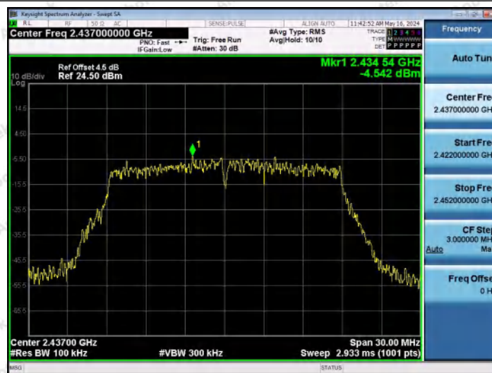
11N20MIMO-Ant2-2437-0~Reference-PASS
