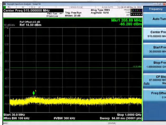
11N20MIMO-Ant2-2412-30~1000-PASS
