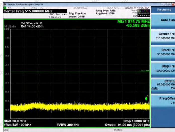
11G-Ant2-2412-30~1000-PASS
