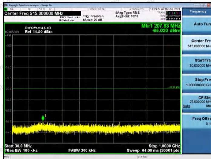
11G-Ant2-2462-30~1000-PASS
