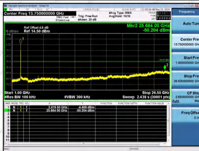
11AX20MIMO-Ant1-2412-1000~26500-PASS
