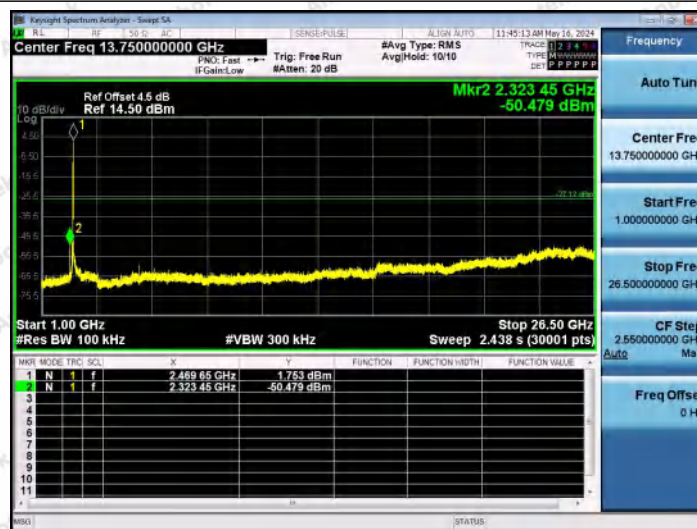
11N20MIMO-Ant1-2462-1000~26500-PASS
