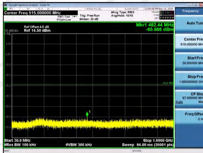
11AX20MIMO-Ant2-2437-30~1000-PASS
