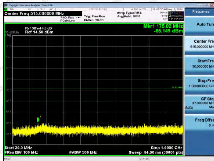
11N20MIMO-Ant2-2437-30~1000-PASS
