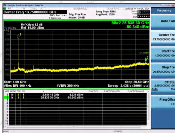
11N20MIMO-Ant2-2437-1000~26500-PASS
