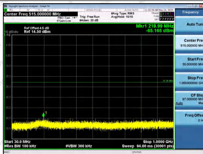
11N20MIMO-Ant1-2412-30~1000-PASS
