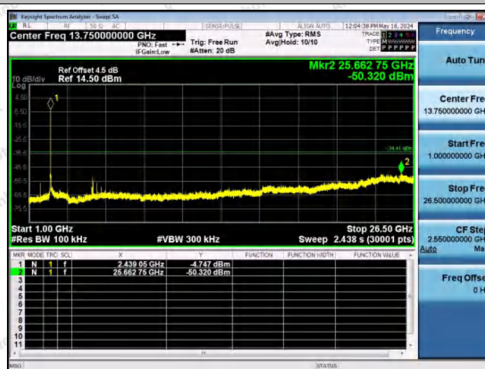
11AX20MIMO-Ant2-2437-1000~26500-PASS
