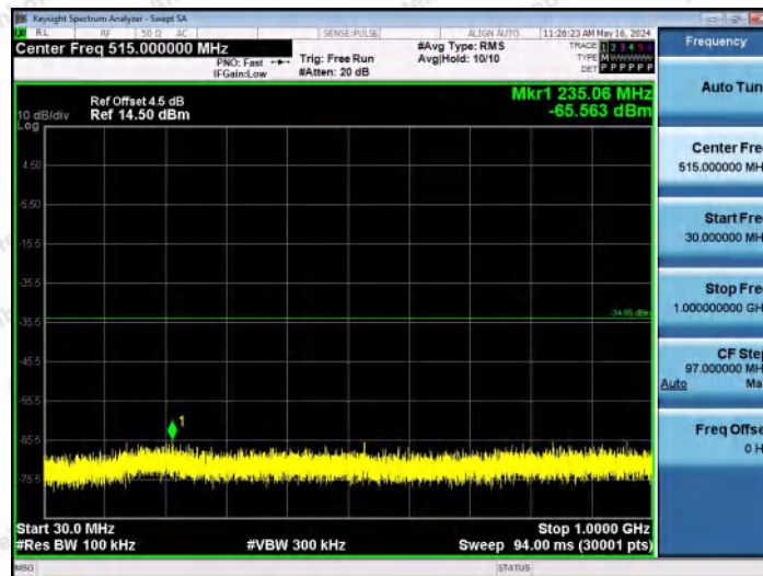
11G-Ant2-2437-30~1000-PASS
