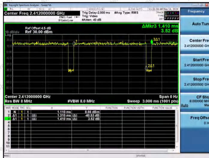
NTNV-11N20MIMO-Ant1-2412
