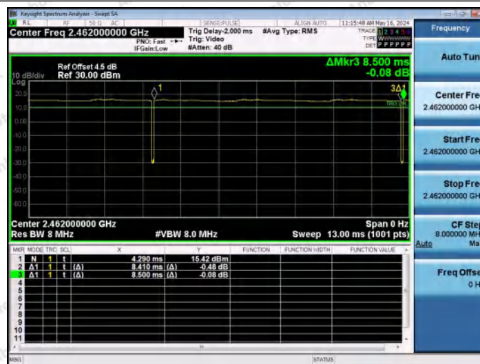
NTNV-11B-Ant2-2462
