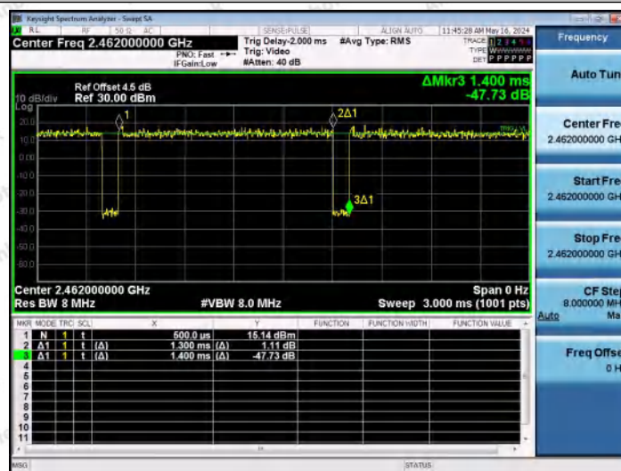
NTNV-11N20MIMO-Ant2-2462
