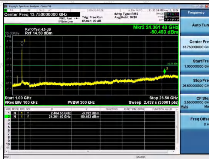
11G-Ant2-2462-1000~26500-PASS
