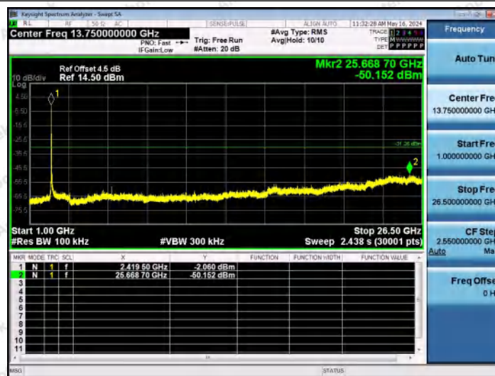
11N20MIMO-Ant1-2412-1000~26500-PASS
