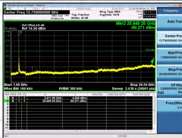
11B-Ant1-2412-1000~26500-PASS
