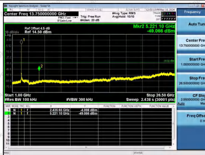
11AX20MIMO-Ant1-2437-1000~26500-PASS
