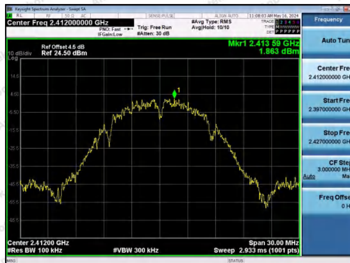
11B-Ant2-2412-0~Reference-PASS
