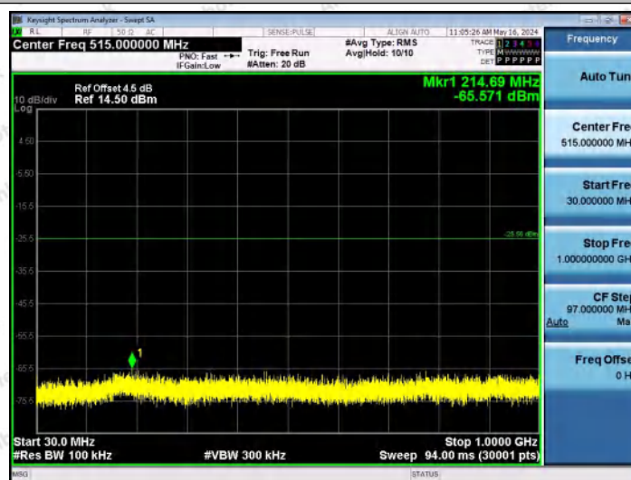
11B-Ant1-2412-30~1000-PASS
