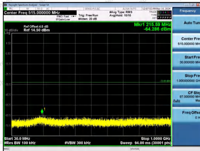
11AX20MIMO-Ant2-2462-30~1000-PASS
