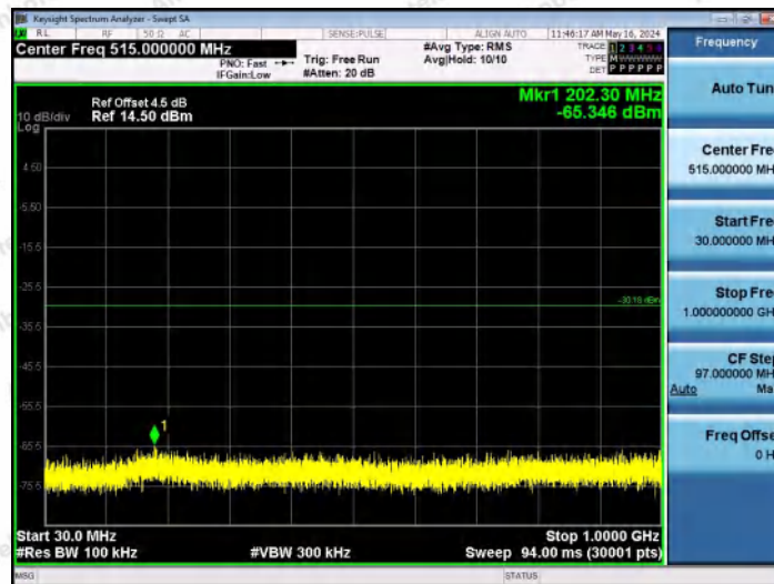
11N20MIMO-Ant2-2462-30~1000-PASS
