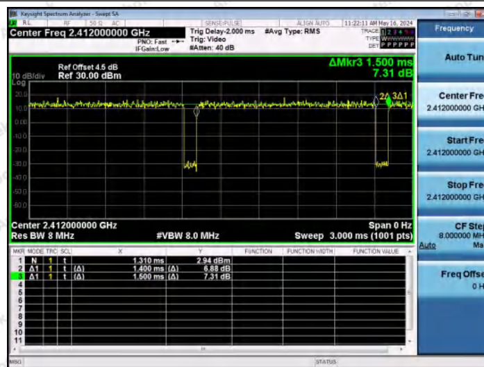
NTNV-11G-Ant2-2412
