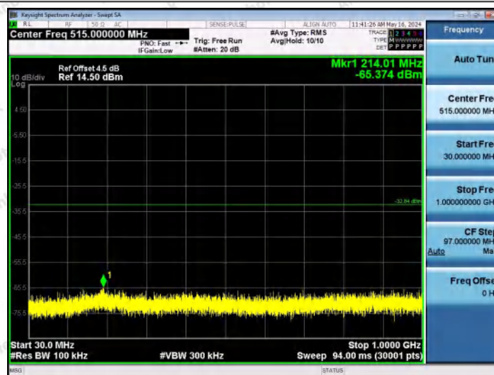
11N20MIMO-Ant1-2437-30~1000-PASS
