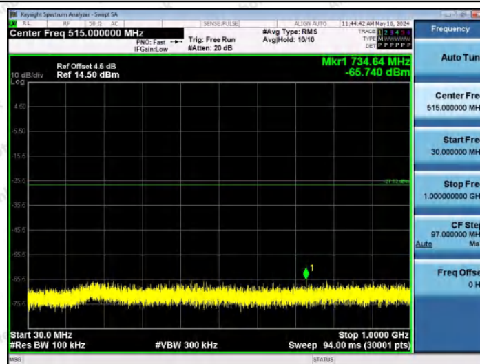
11N20MIMO-Ant1-2462-30~1000-PASS
