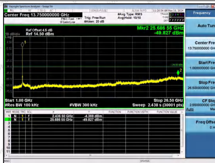
11G-Ant2-2437-1000~26500-PASS
