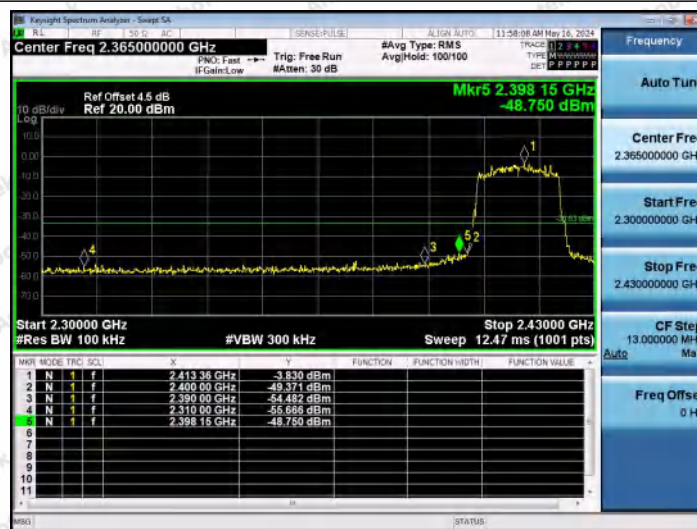
11AX20MIMO-Ant2-2412-PASS
