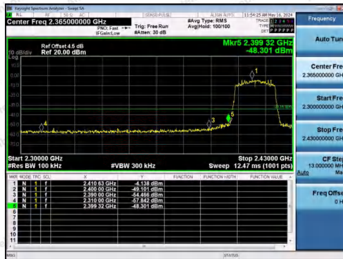
11AX20MIMO-Ant1-2412-PASS
