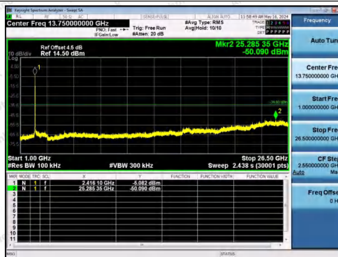
11AX20MIMO-Ant2-2412-1000~26500-PASS
