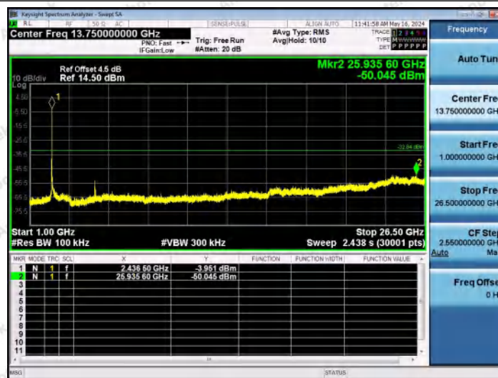
11N20MIMO-Ant1-2437-1000~26500-PASS
