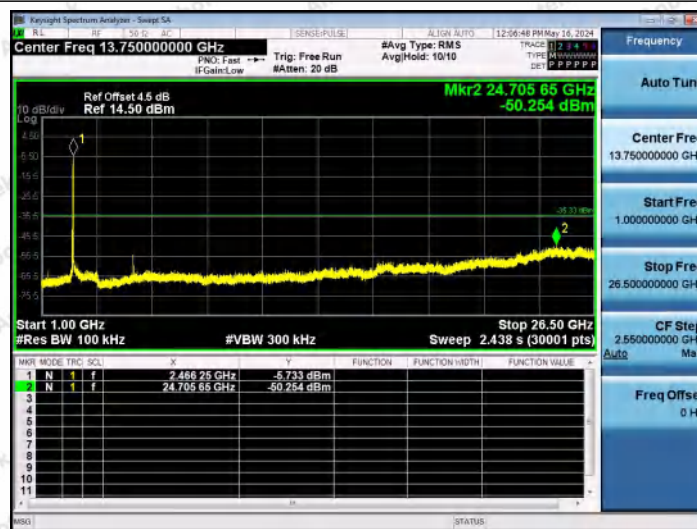
11AX20MIMO-Ant1-2462-1000~26500-PASS
