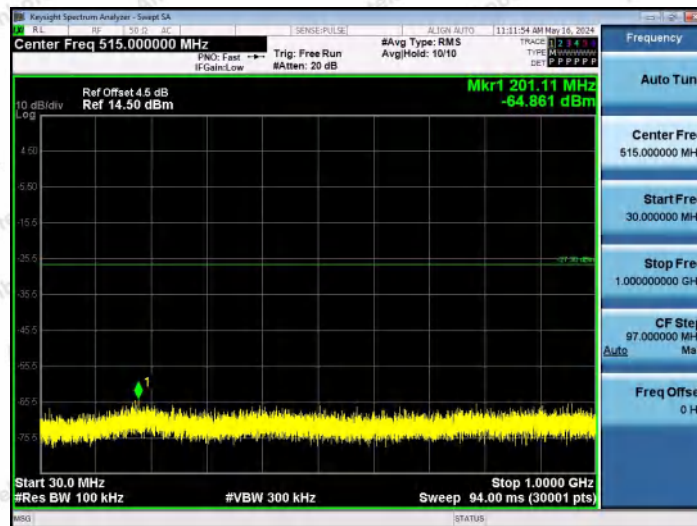
11B-Ant2-2437-30~1000-PASS
