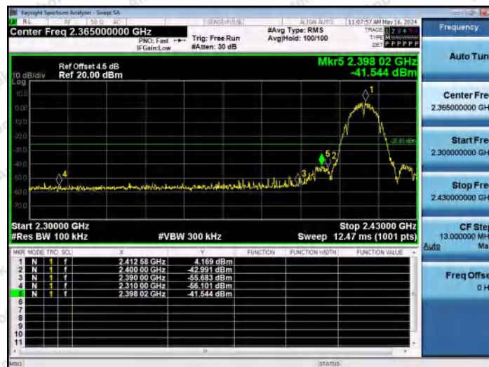
11B-Ant2-2412-PASS
