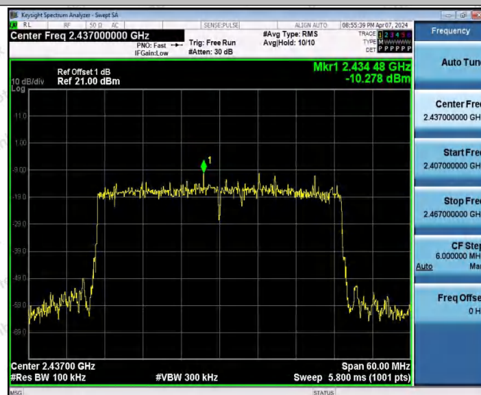
11AX40SISO_Ant2_2437_0~Reference
