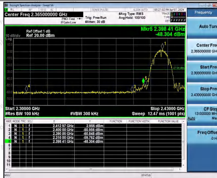
11B_Ant2_Low_2412
