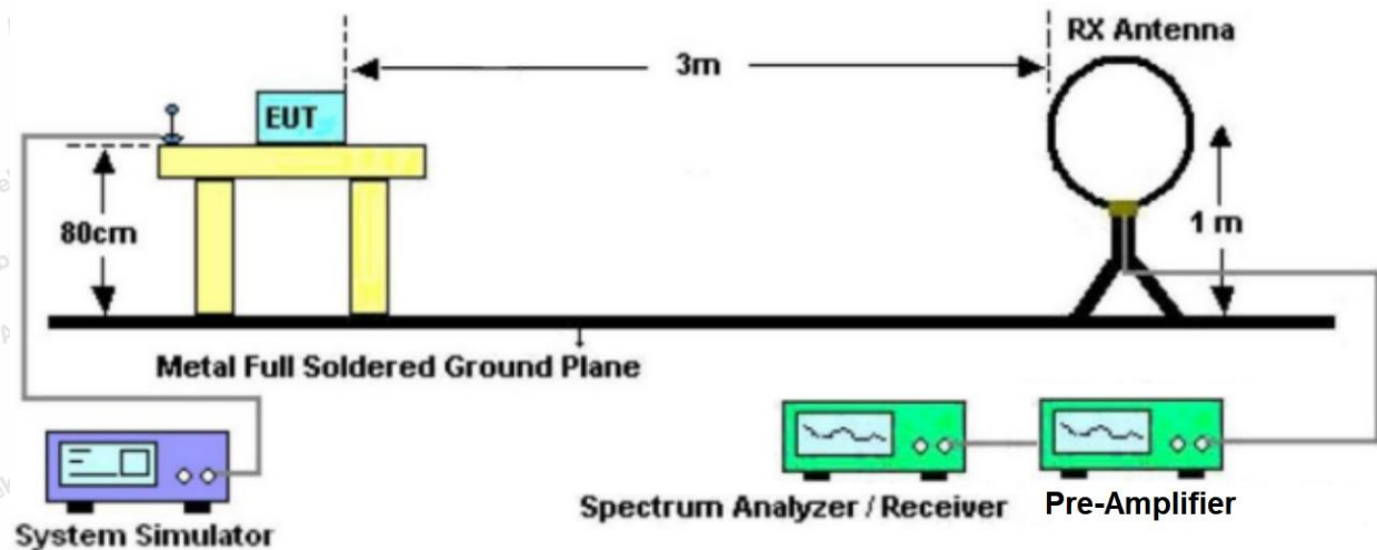
Figure 1. Below 30MHz
