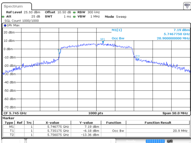
802.11ax20_5745MHz
