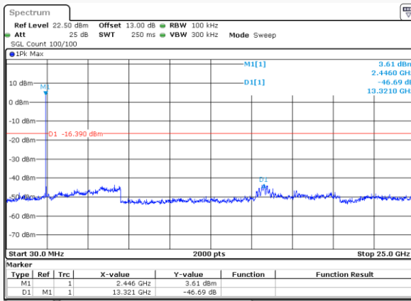
BLE_2M_Middle_Channel
