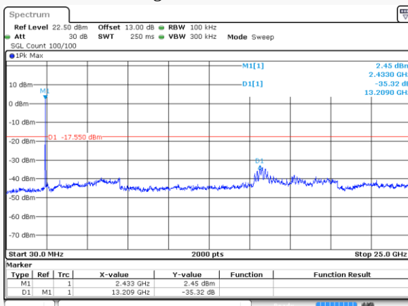
802.11g_2437MHz_Chain 1
