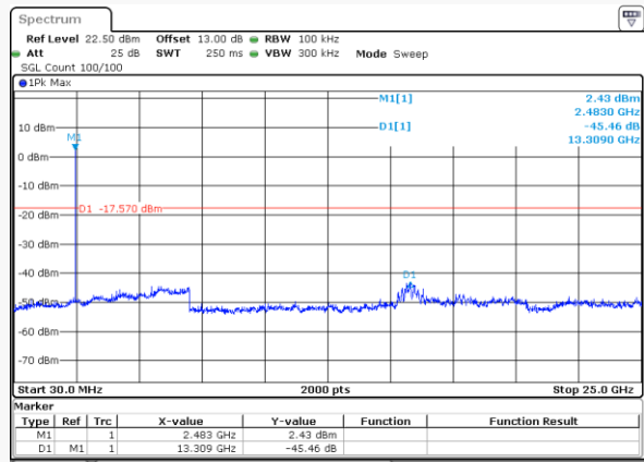
BLE_2M_High_Channel
