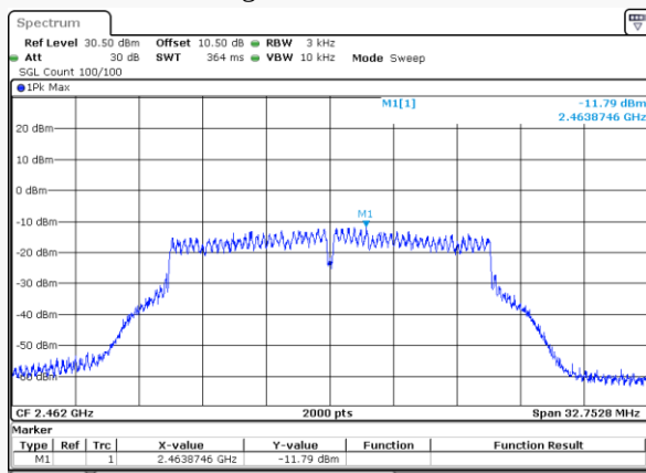
802.11g_2462MHz_Chain 1
