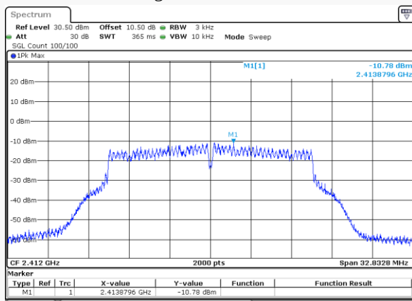
802.11g_2412MHz_Chain 1
