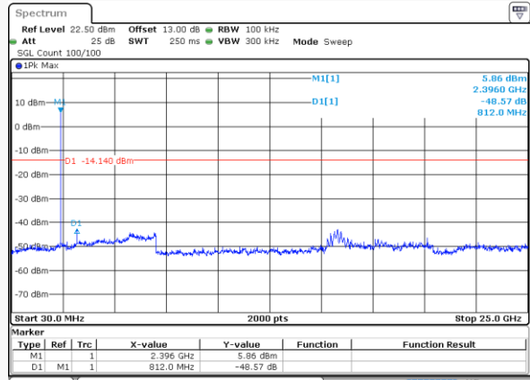
BLE_2M_Low_Channel
