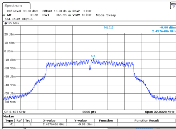
802.11g_2437MHz_Chain 0
