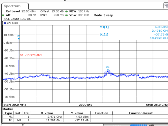
802.11g_2462MHz_Chain 0
