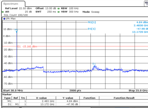
BLE_1M_High_Channel
