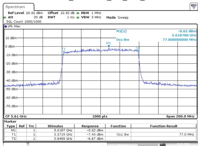
802.11ax80_5610MHz_RU_Full_Chain 0
