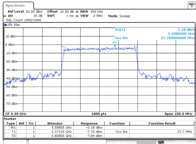
802.11ax40_5590MHz_RU_Full_Chain 1
