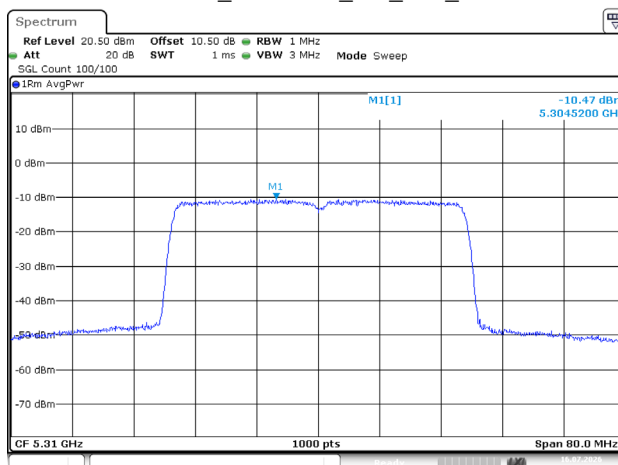
802.11ax40_5310MHz_RU_Full_Chain 0
