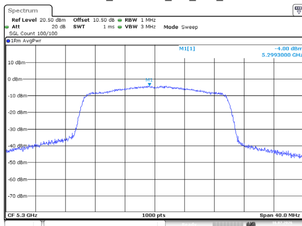
802.11ax20_5300MHz_RU_Full_Chain 1
