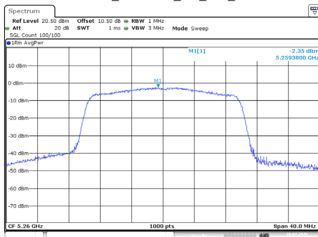
802.11ax20_5260MHz_RU_Full_Chain 0
