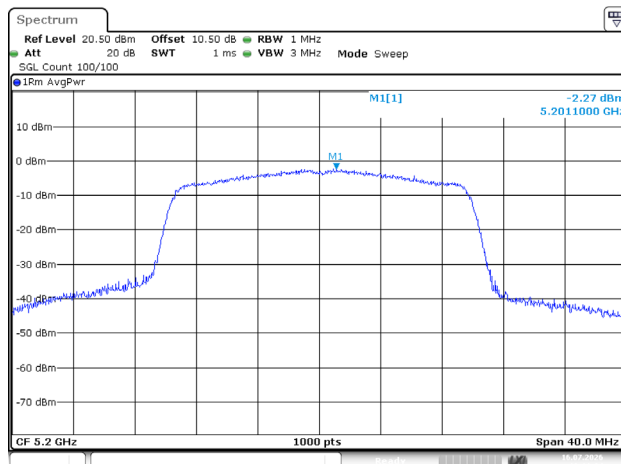
802.11ax20_5200MHz_RU_Full_Chain 1
