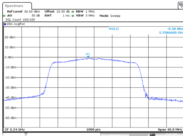
802.11ax20_5240MHz_RU_Full_Chain 0
