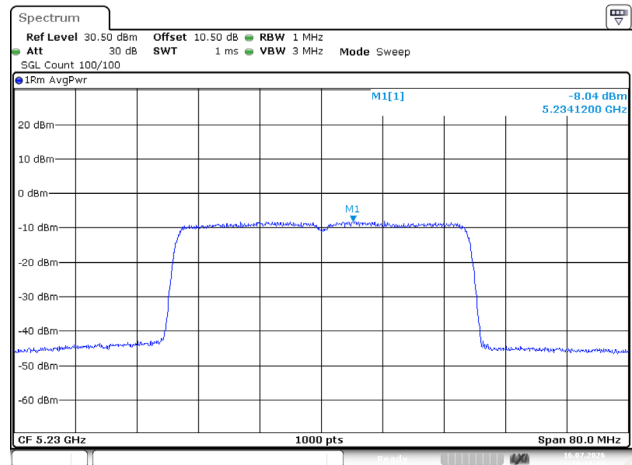
802.11ax40_5230MHz_RU_Full_Chain 0
