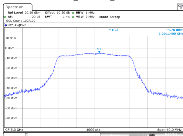
802.11a_5300MHz_Chain 1
