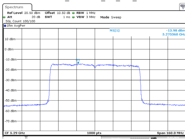
802.11ax80_5290MHz_RU_Full_Chain 0
