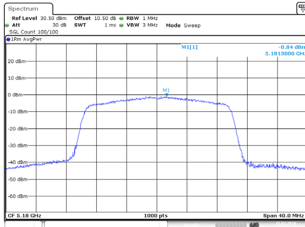
802.11ax20_5180MHz_RU_Full_Chain 0
