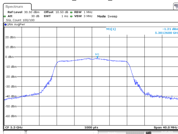
802.11a_5300MHz_Chain 0
