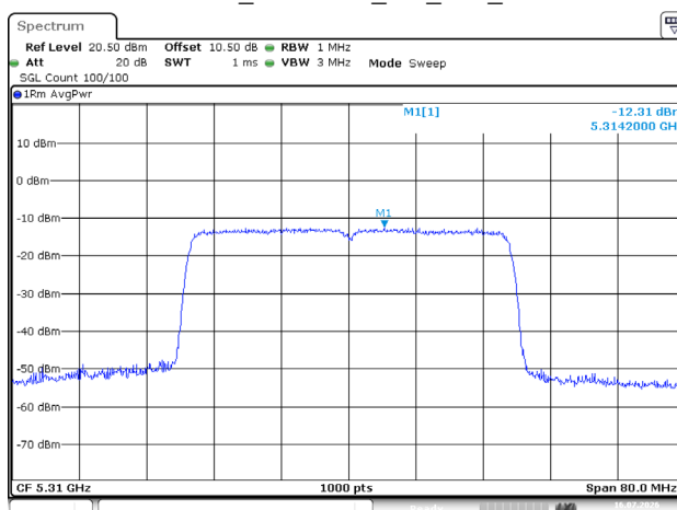
802.11ax40_5310MHz_RU_Full_Chain 1
