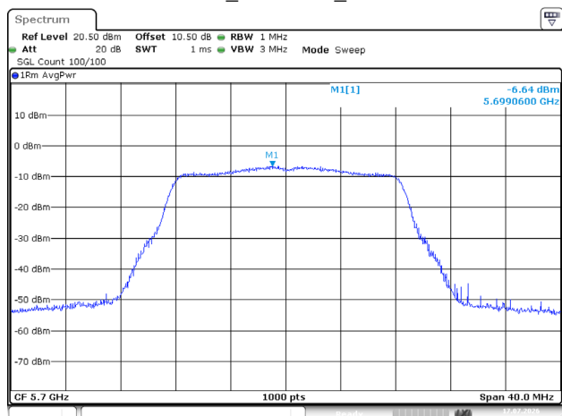
802.11a_5700MHz_Chain 1
