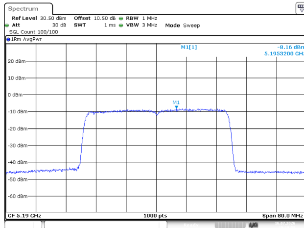
802.11ax40_5190MHz_RU_Full_Chain 0
