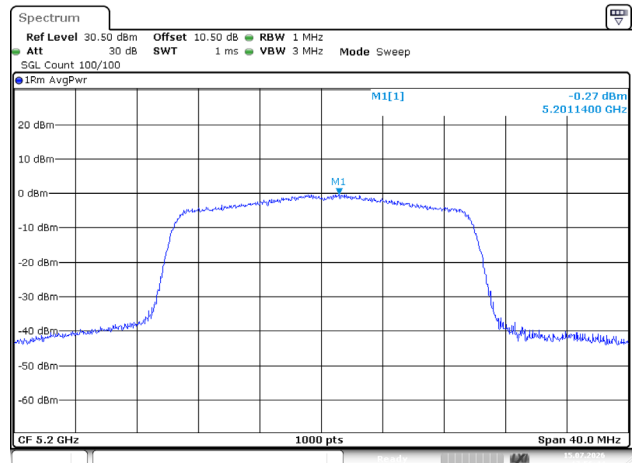
802.11ax20_5200MHz_RU_Full_Chain 0
