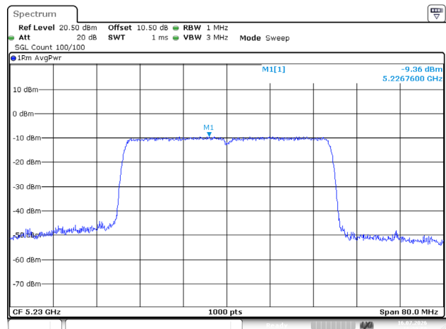
802.11ax40_5230MHz_RU_Full_Chain 1
