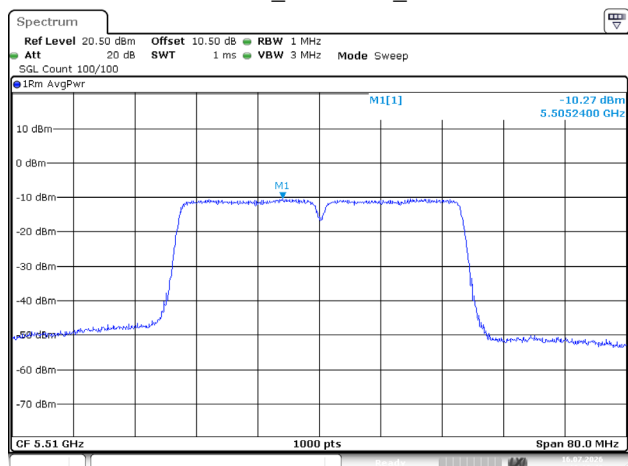
802.11ac40_5510MHz_Chain 0
