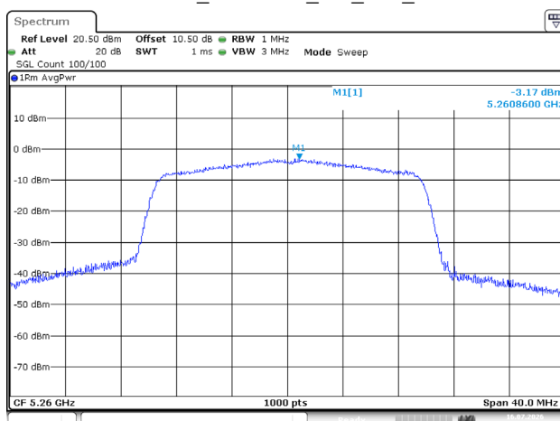
802.11ax20_5260MHz_RU_Full_Chain 1
