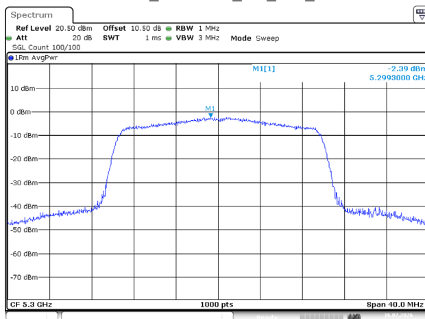
802.11ax20_5300MHz_RU_Full_Chain 0
