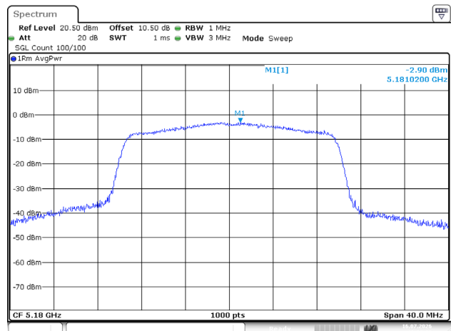
802.11ax20_5180MHz_RU_Full_Chain 1
