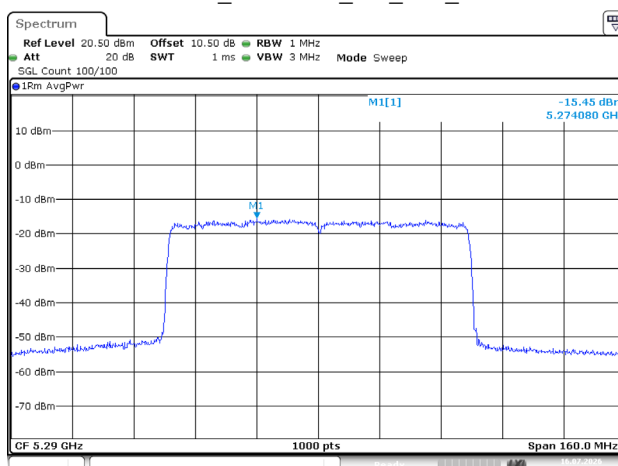
802.11ax80_5290MHz_RU_Full_Chain 1
