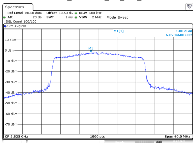
802.11ax20_5825MHz_RU_Full_Chain 0
