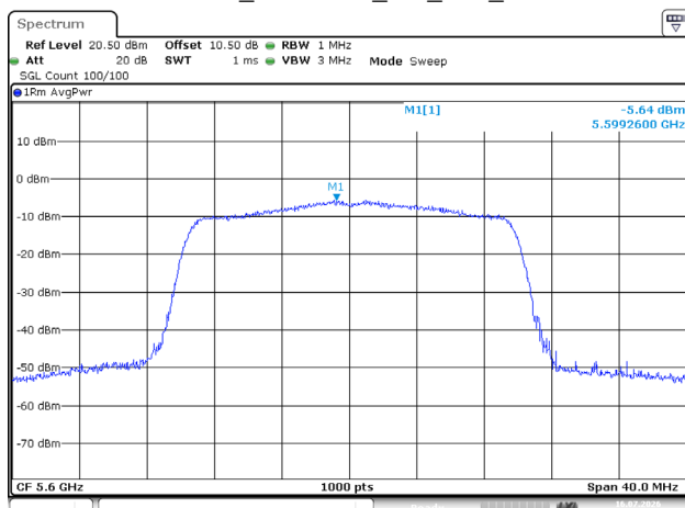
802.11ax20_5600MHz_RU_Full_Chain 0
