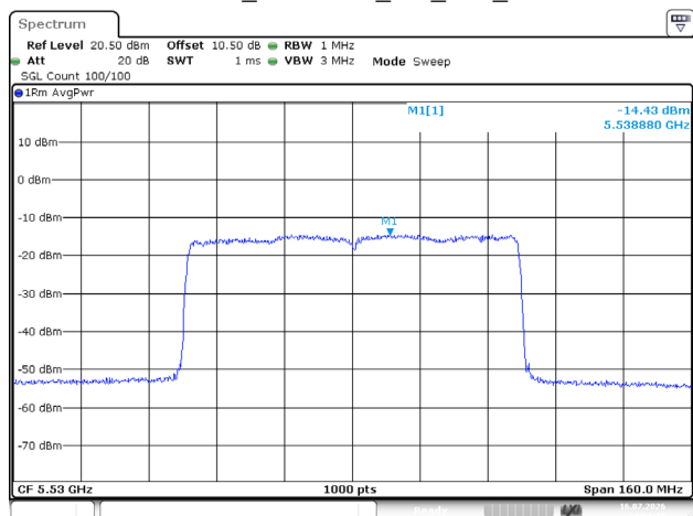
802.11ax80_5530MHz_RU_Full_Chain 0
