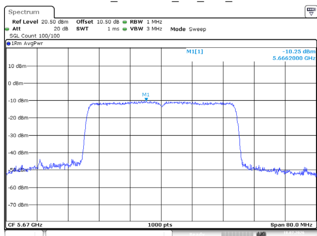
802.11ax40_5670MHz_RU_Full_Chain 1
