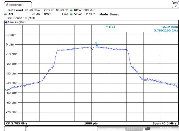
802.11a_5785MHz_Chain 0
