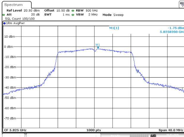
802.11a_5825MHz_Chain 0
