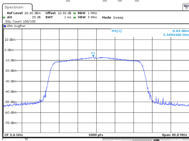
802.11ax20_5600MHz_RU_Full_Chain 1
