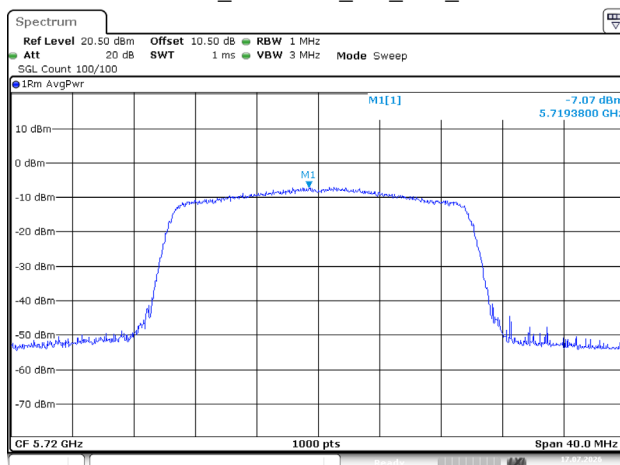
802.11ax20_5720MHz_RU_Full_Chain 1
