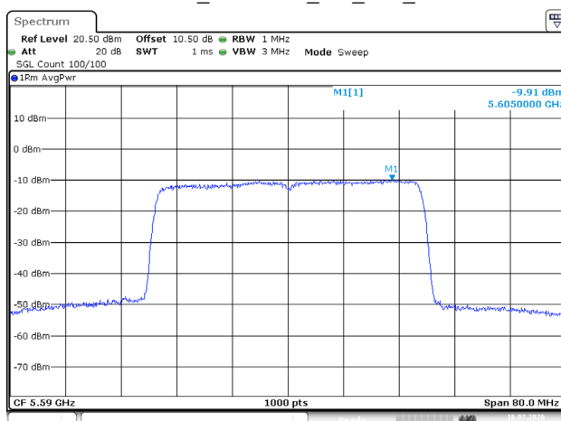
802.11ax40_5590MHz_RU_Full_Chain 0
