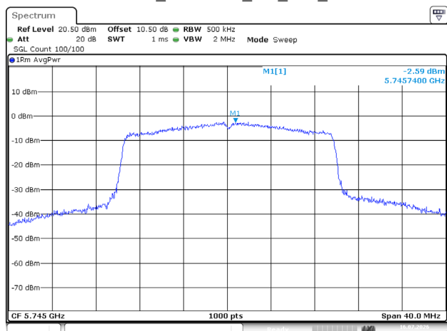
802.11ax20_5745MHz_RU_Full_Chain 0
