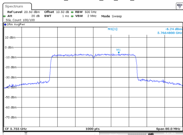
802.11ax40_5755MHz_RU_Full_Chain 0
