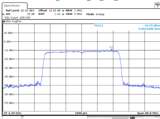
802.11ax40_5590MHz_RU_Full_Chain 1
