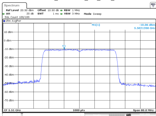
802.11ax40_5510MHz_RU_Full_Chain 1
