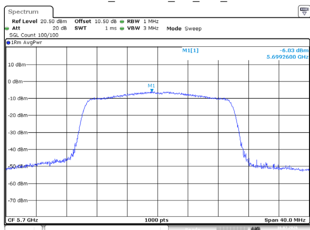
802.11ax20_5700MHz_RU_Full_Chain 0
