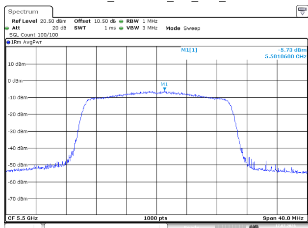
802.11ax20_5500MHz_RU_Full_Chain 1
