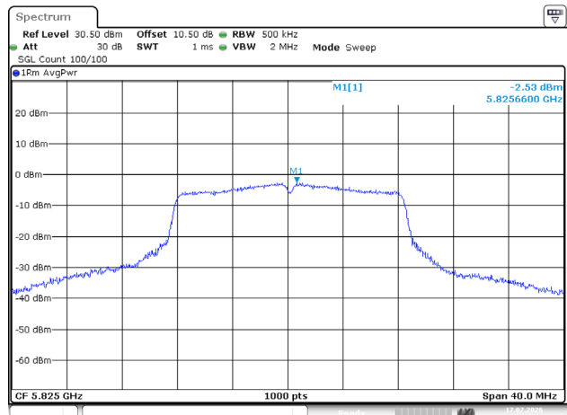
802.11a_5825MHz_Chain 1
