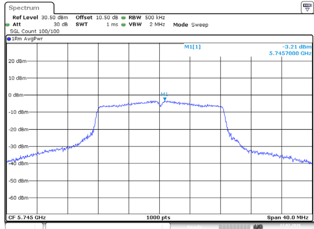
802.11a_5745MHz_Chain 1
