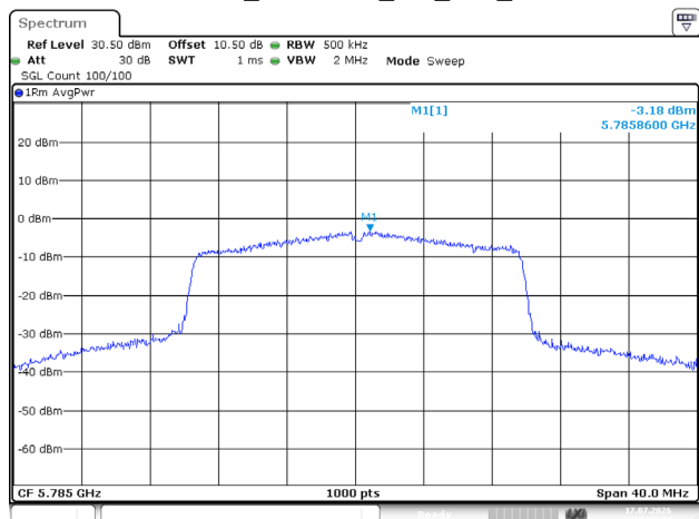
802.11ax20_5785MHz_RU_Full_Chain 1
