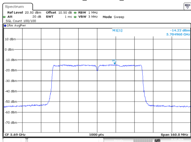
802.11ac80_5690MHz_Chain 0
