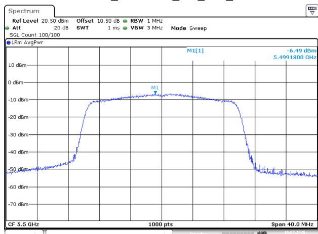
802.11ax20_5500MHz_RU_Full_Chain 0
