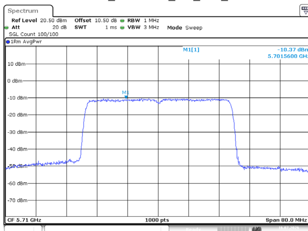
802.11ax40_5710MHz_RU_Full_Chain 0
