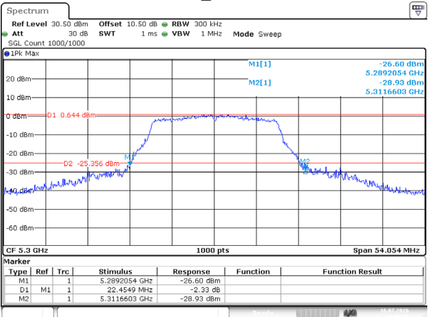
802.11a_5300MHz
