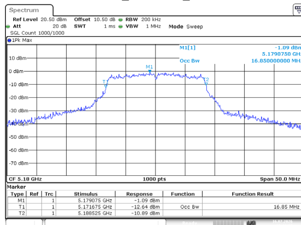
802.11a_5180MHz_Chain 1
