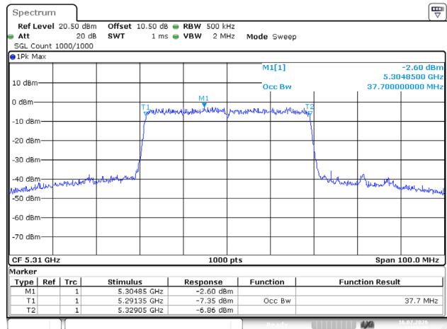
802.11ax40_5310MHz_RU_Full_Chain 0
