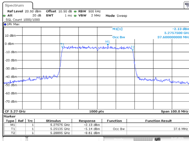
802.11ax40_5270MHz_RU_Full_Chain 0
