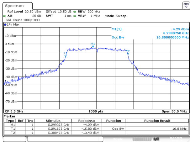
802.11a_5300MHz_Chain 1
