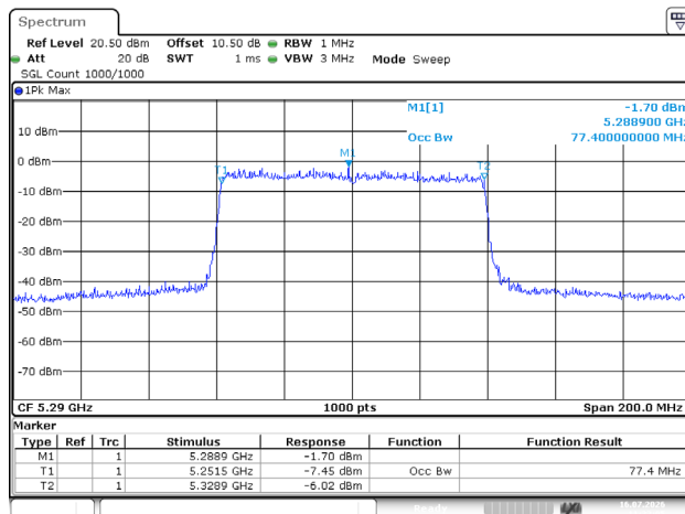
802.11ax80_5290MHz_RU_Full_Chain 0
