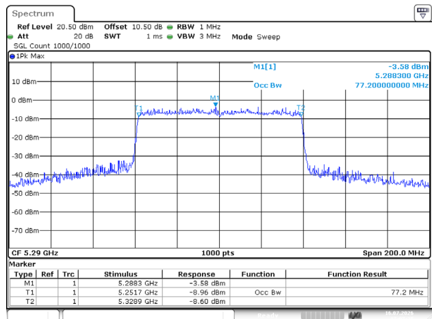
802.11ax80_5290MHz_RU_Full_Chain 1
