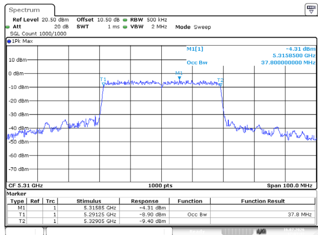
802.11ax40_5310MHz_RU_Full_Chain 1
