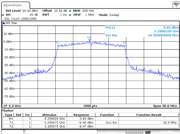
802.11ax20_5300MHz_RU_Full_Chain 0
