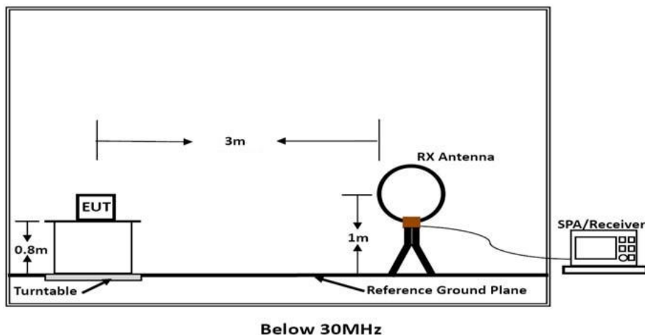
Below 30MHz
