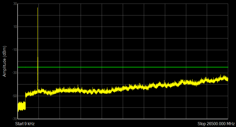
Band7 QAM16 BW=15MHz Channel=21100 RB Size=1 Position=#0
