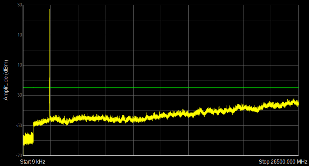
Band7 QPSK BW=10MHz Channel=21100 RB Size=1 Position=#0
