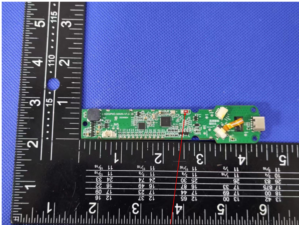
Chip Antenna
