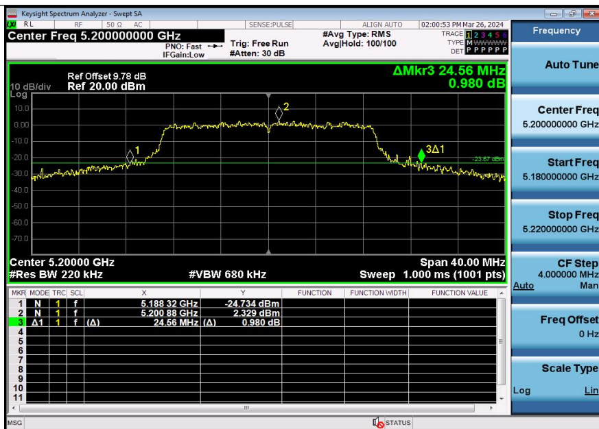
11AC20SISO-Ant1-5200
