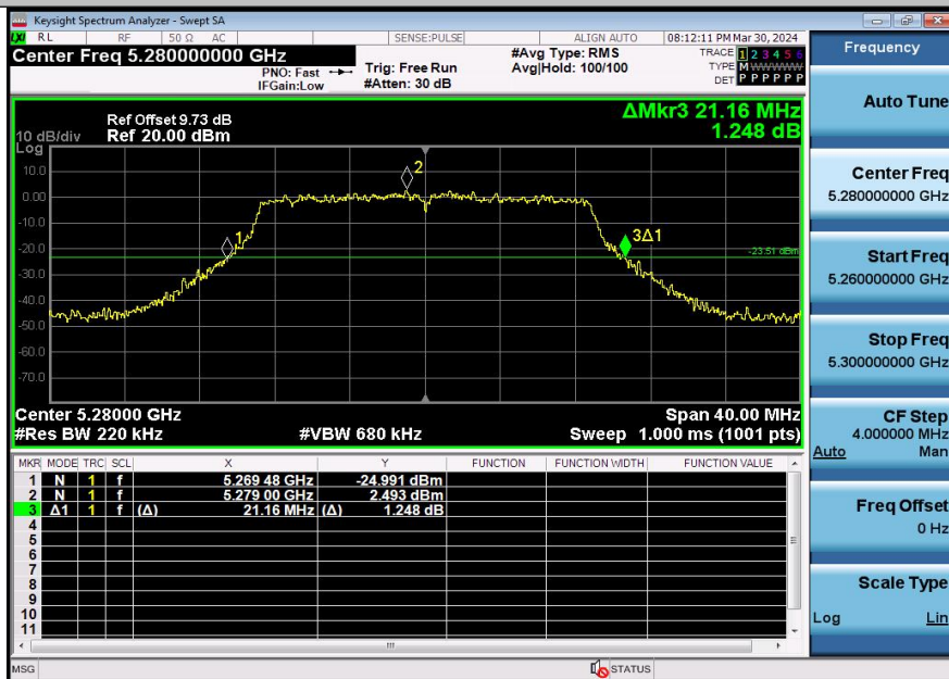
11AC20SISO-Ant1-5280
