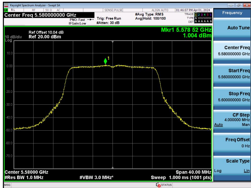
11AX20SISO-Ant1-5580-PASS
