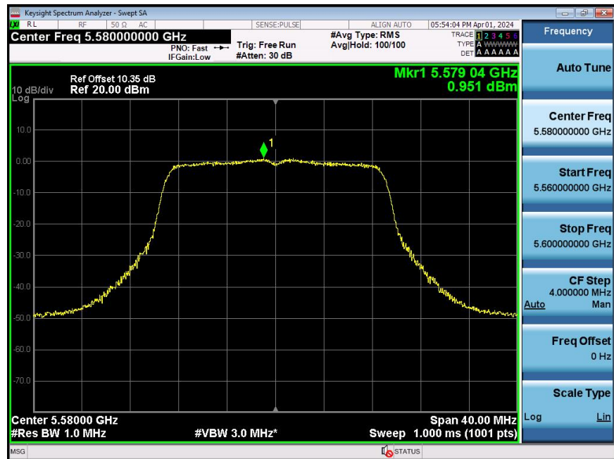
11AX20SISO-Ant2-5580-PASS
