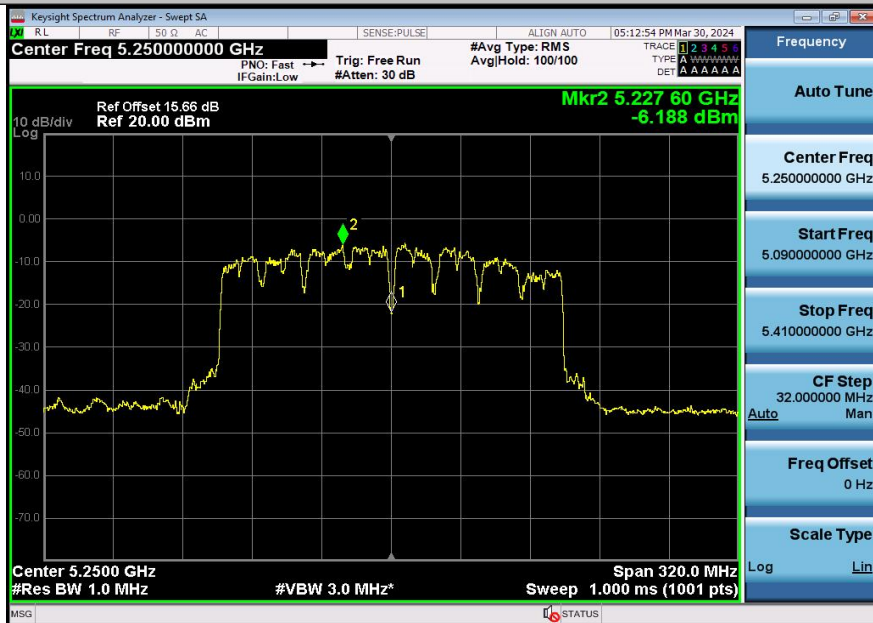
11AC160SISO-Ant2-5250_UNII-1-PASS
